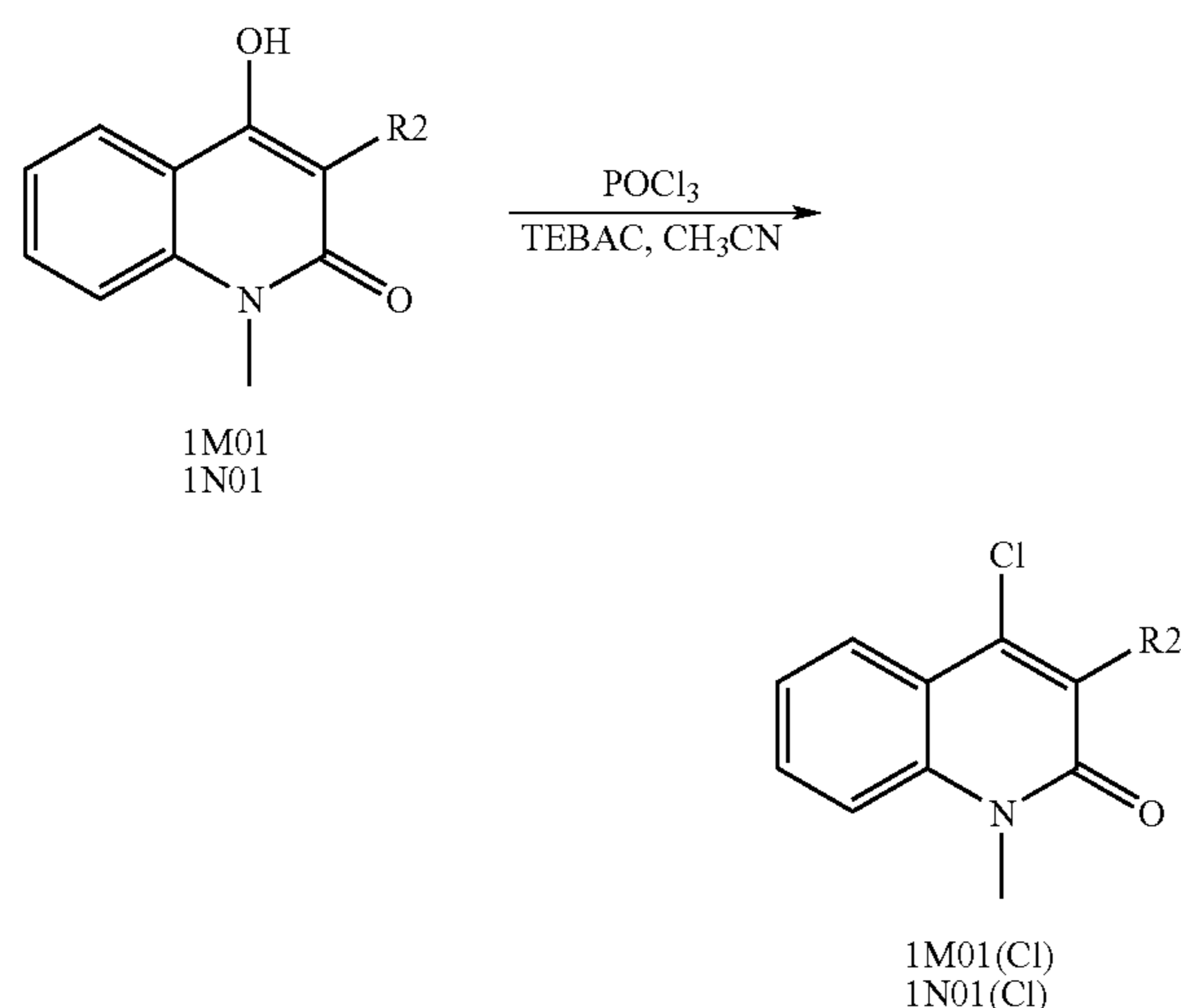
Reaction Scheme 14
