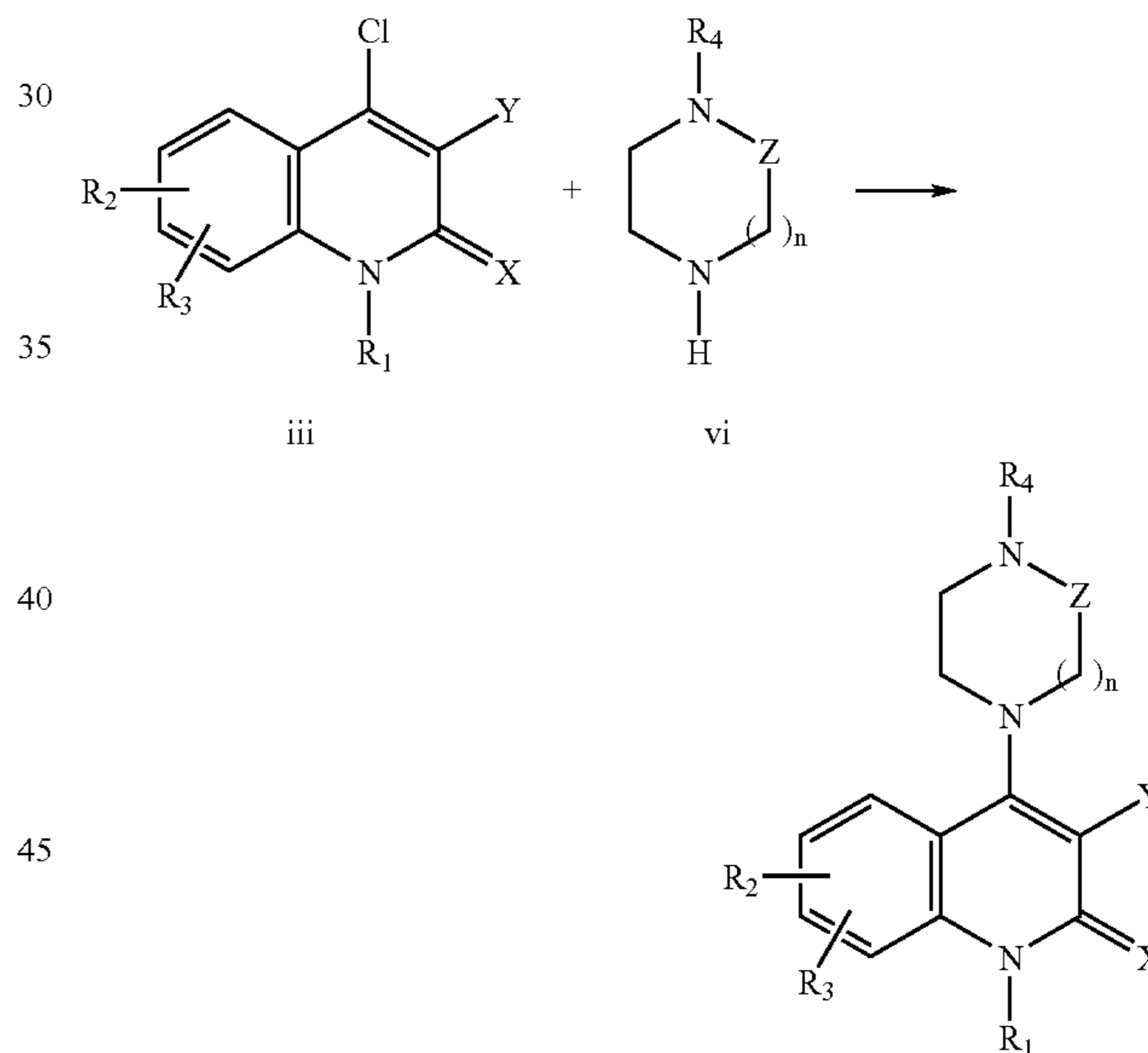
Reaction Scheme 3
