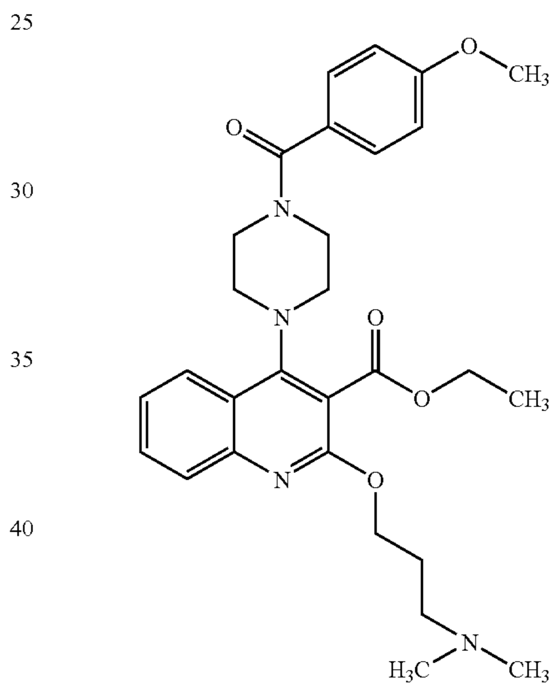
Compound 327
