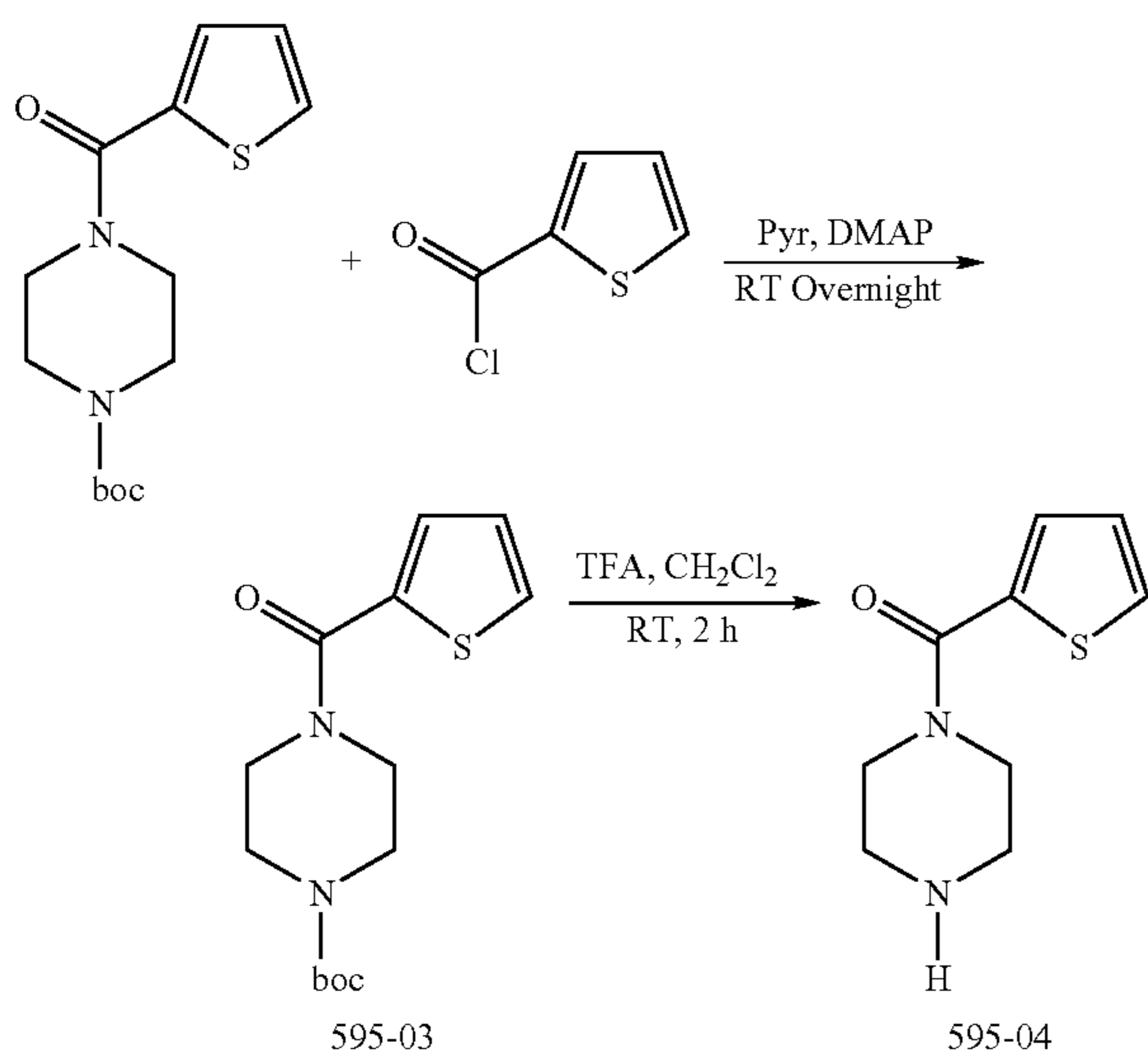
Piperazine-1-yl-thiophen-2-yl-methanone (Referred to as 595-04)
