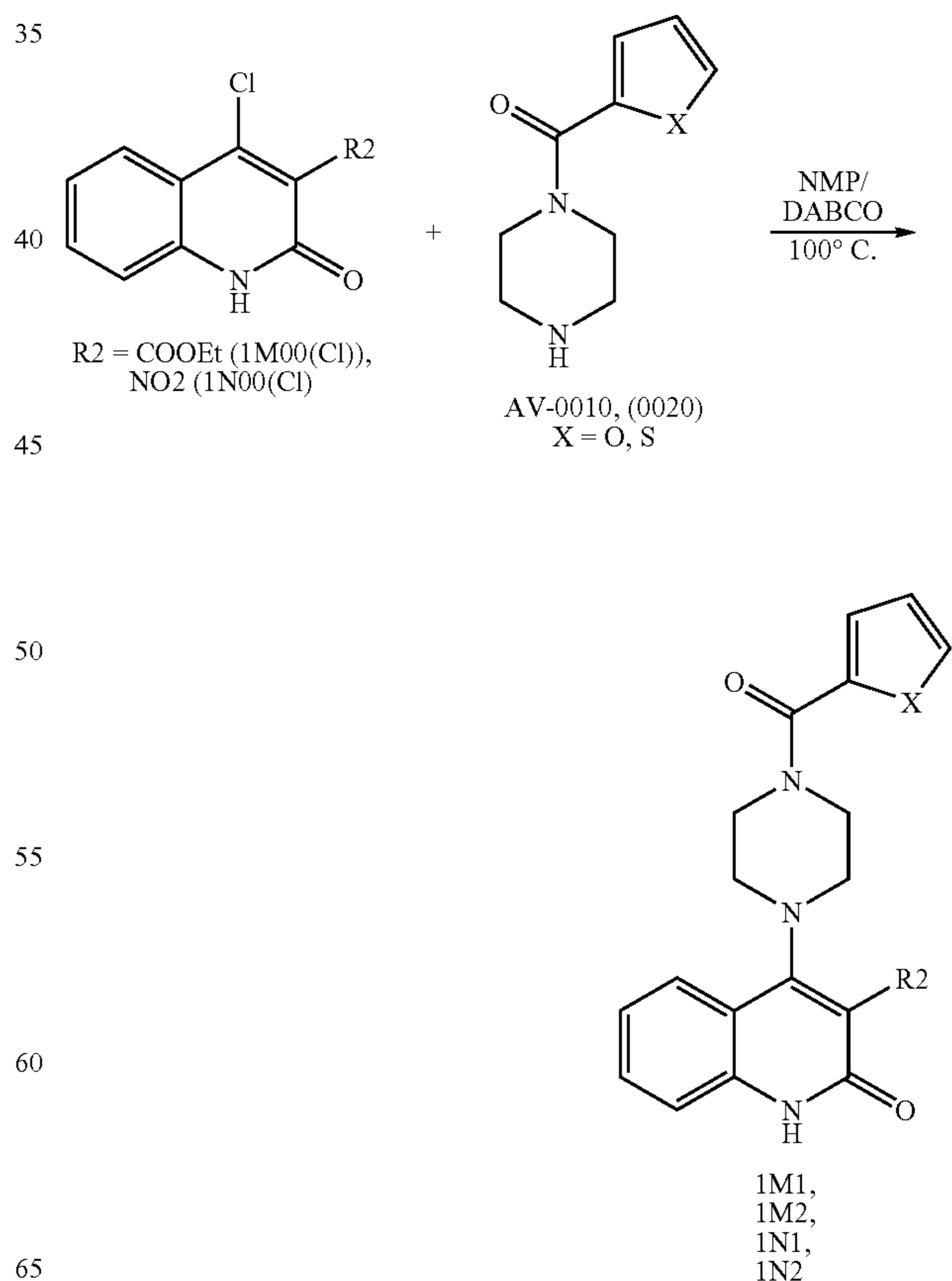
Reaction Scheme 12
