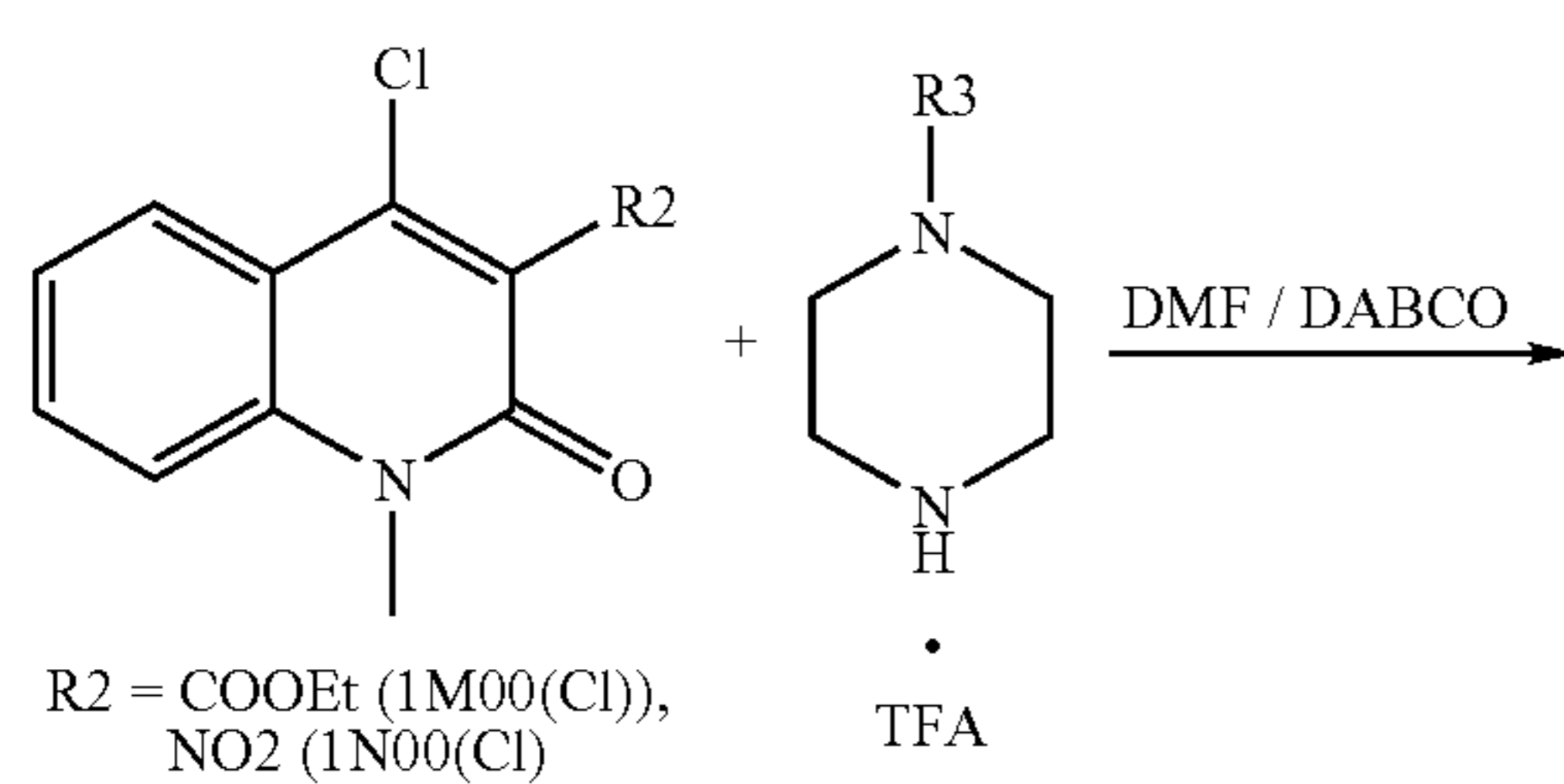
Reaction Scheme 16
