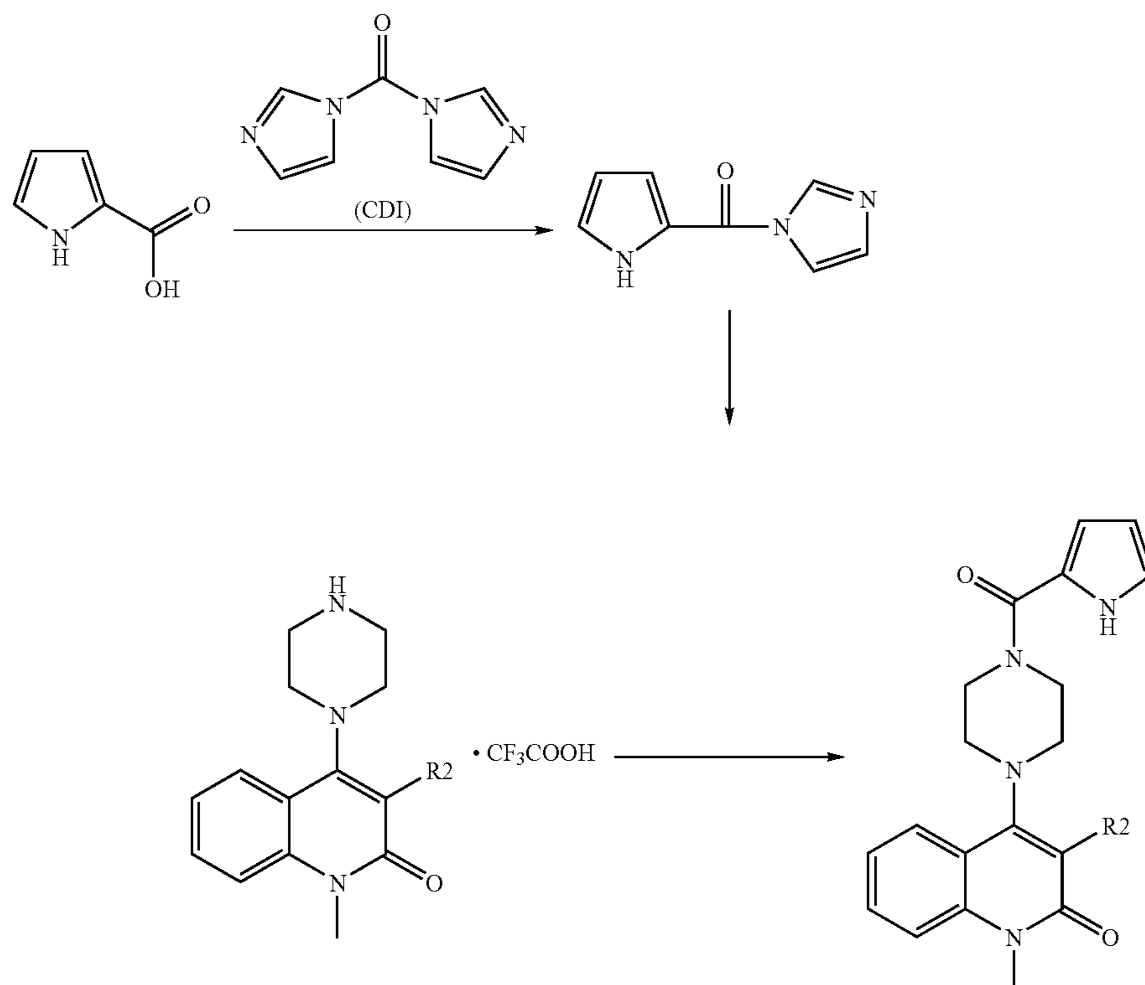
Reaction Scheme 17
