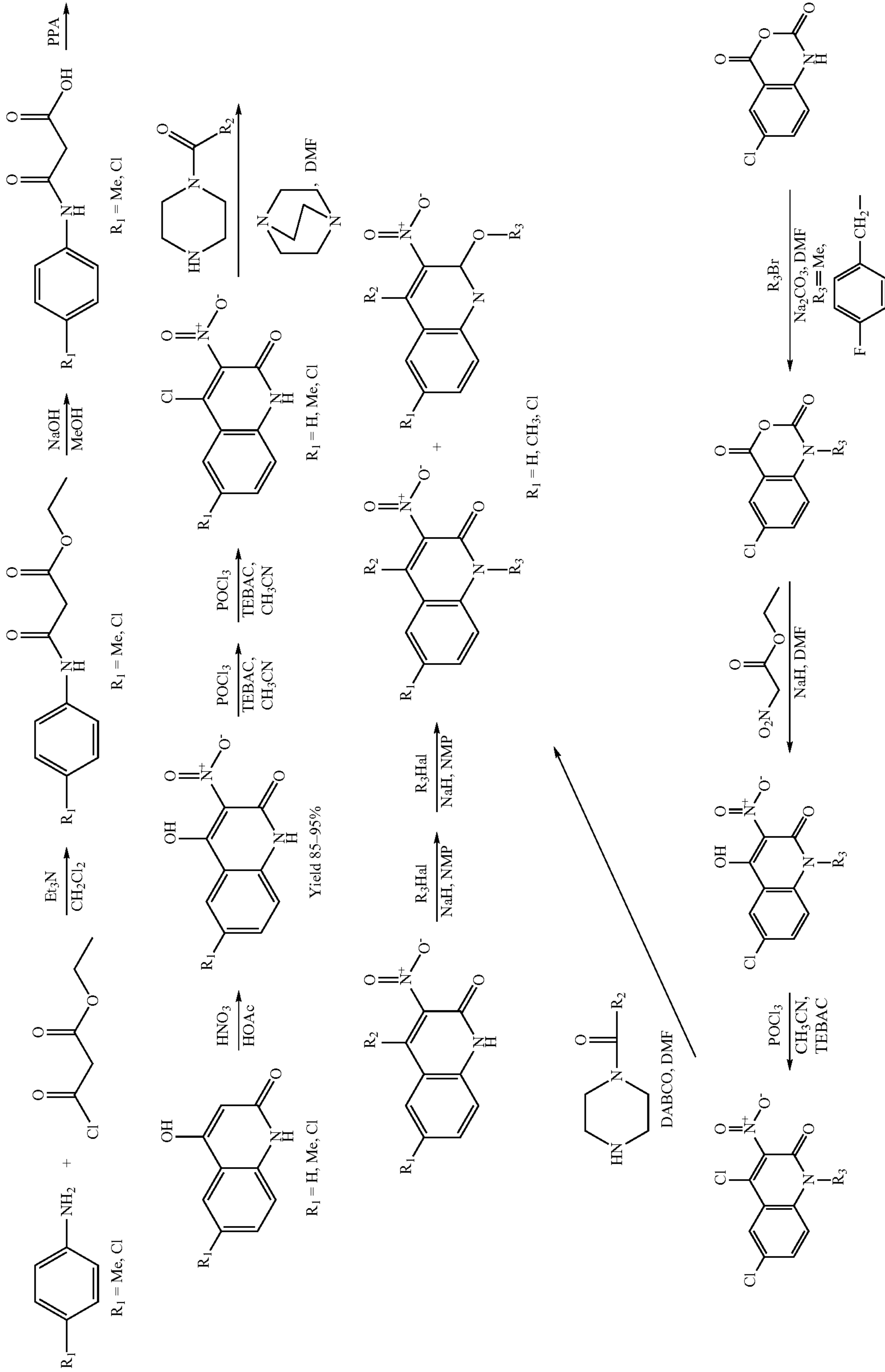
Reaction Scheme 22
