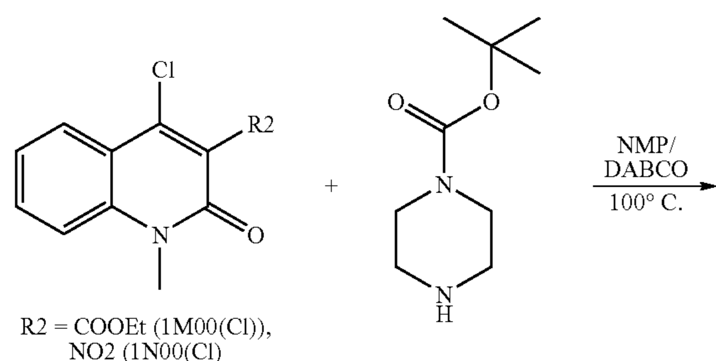
Reaction Scheme 15
