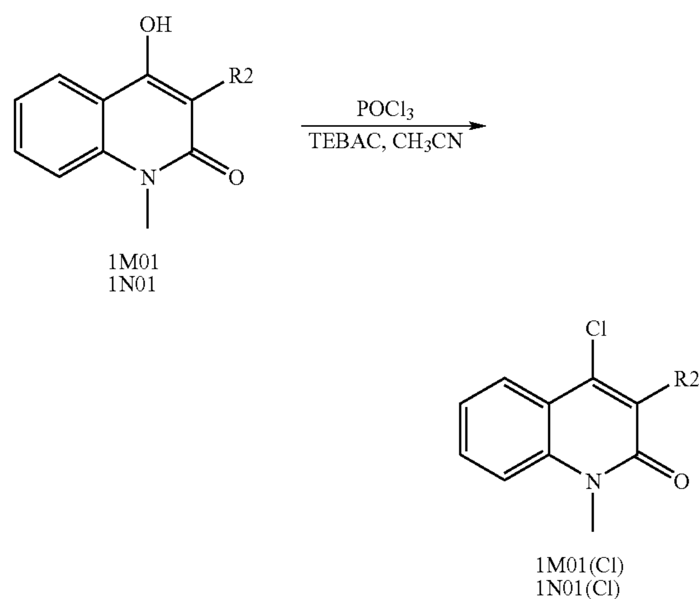
Reaction Scheme 14
