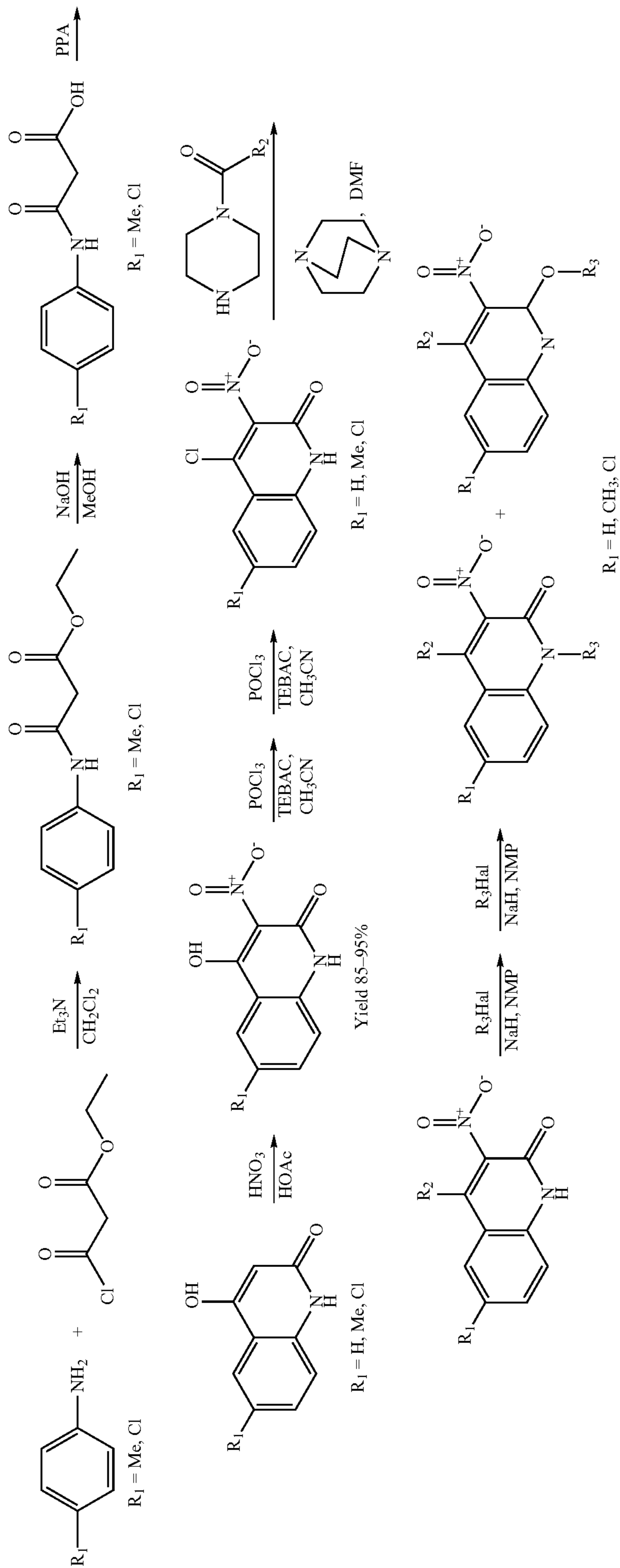
Reaction Scheme 22
