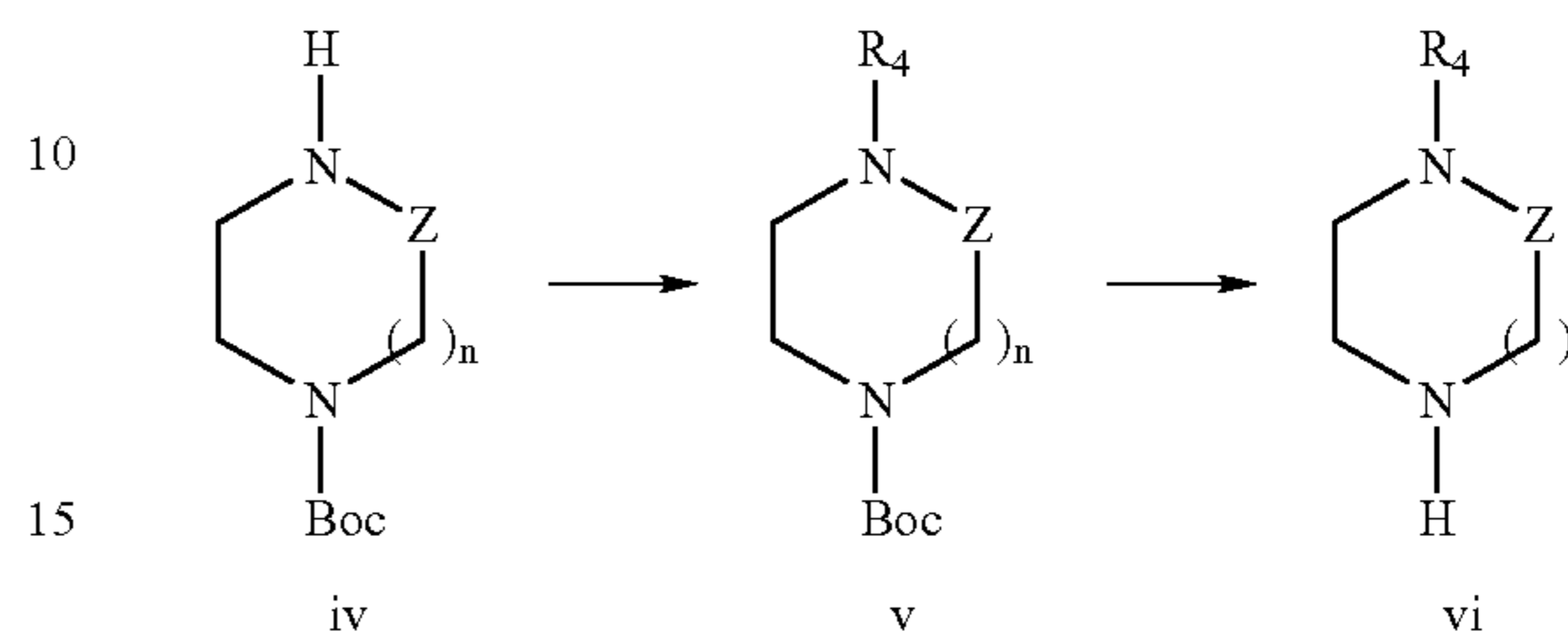
Reaction Scheme 2
