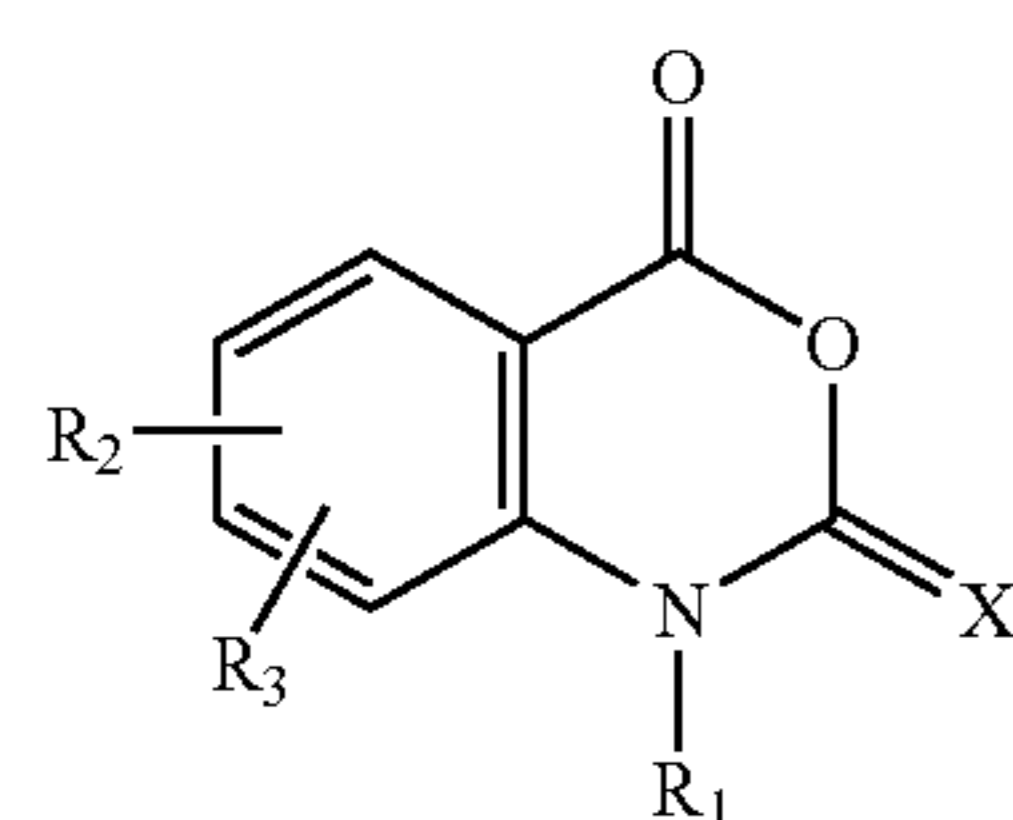
Reaction Scheme 1
