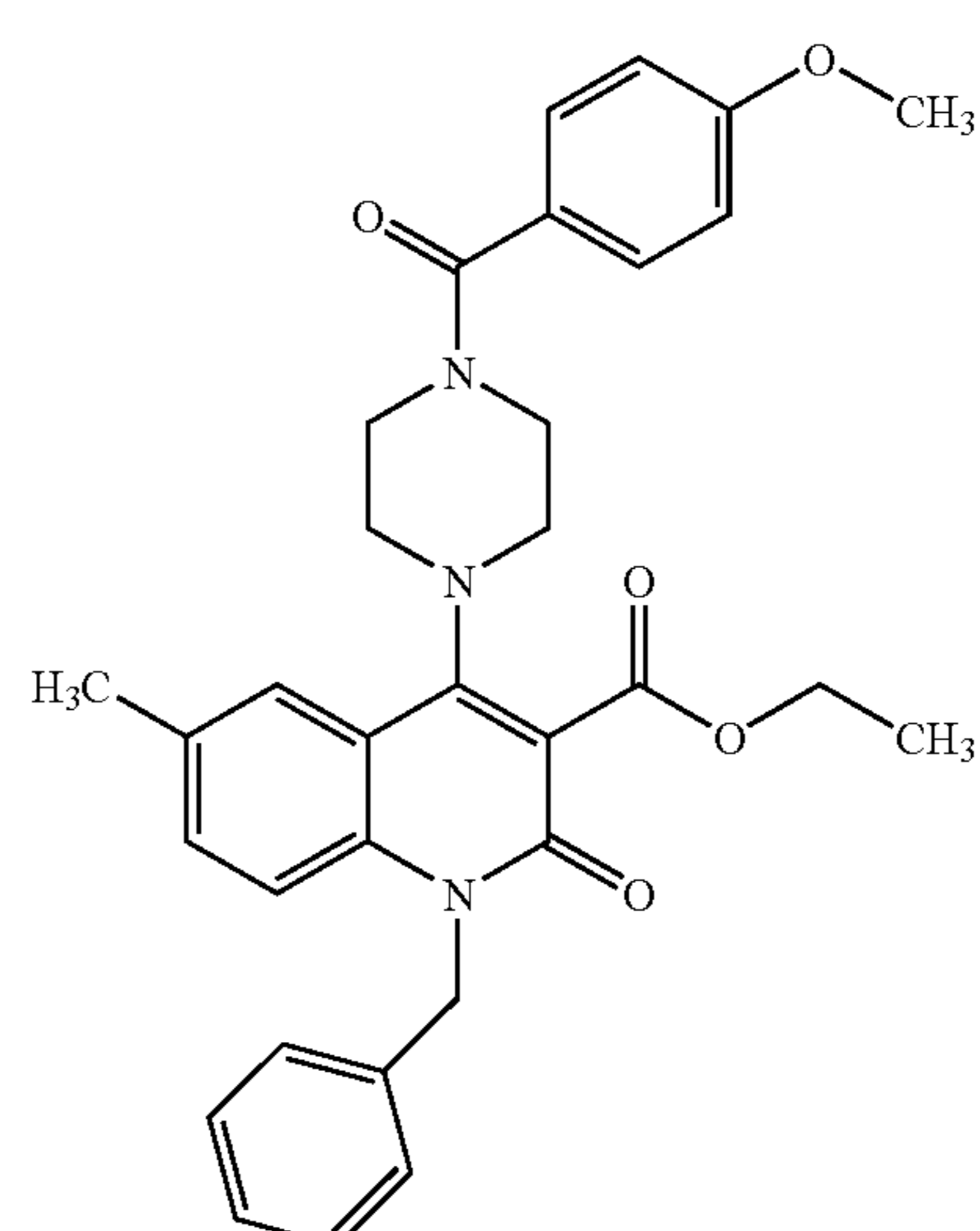
Compound 32
