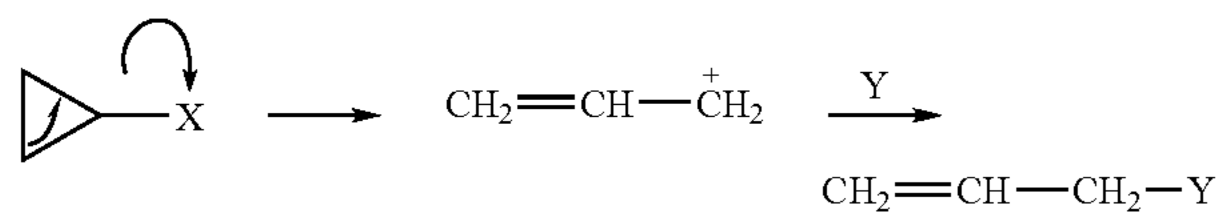
Reaction Scheme 7
