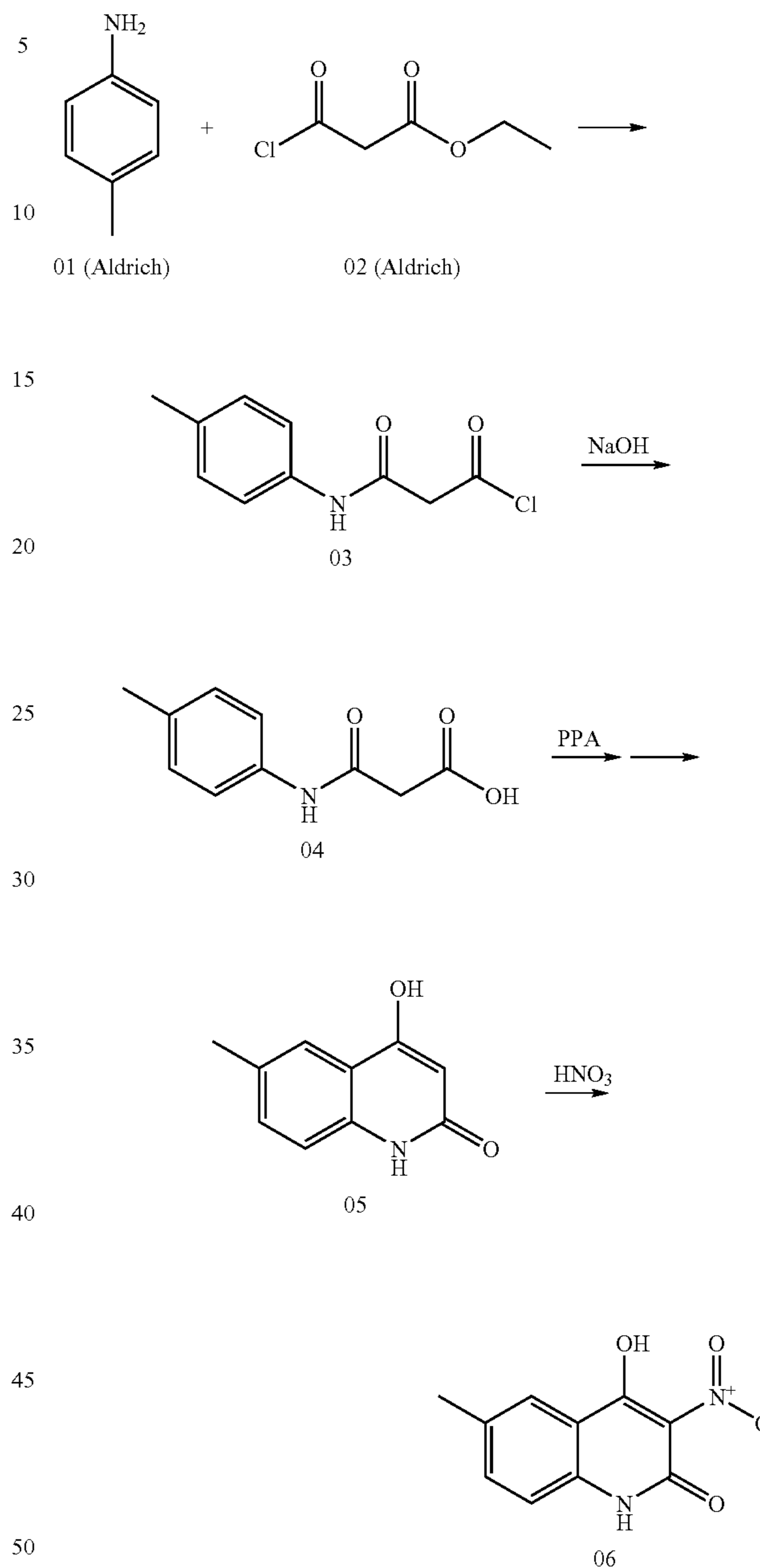
Reaction Scheme 25
