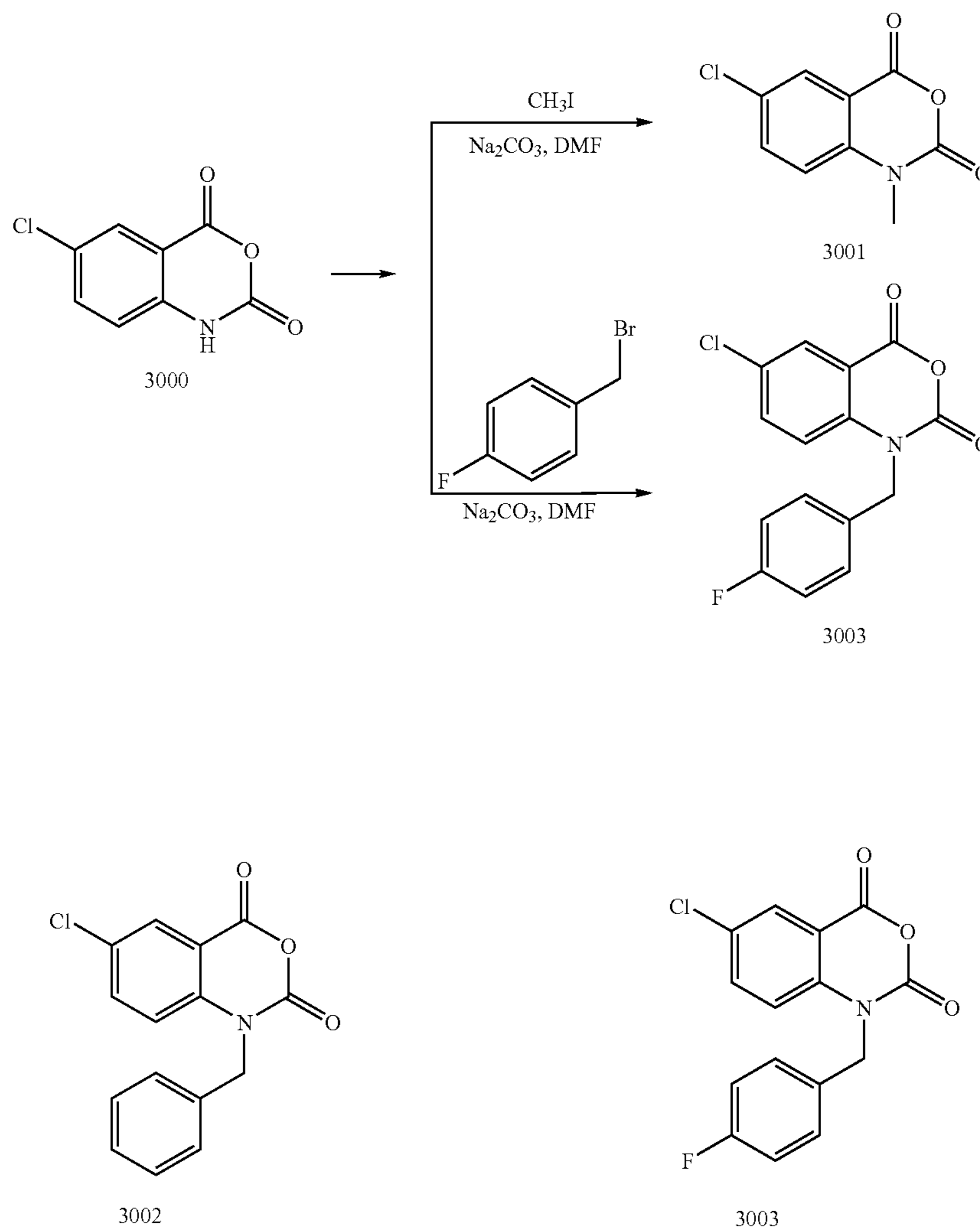
Reaction Scheme 26
