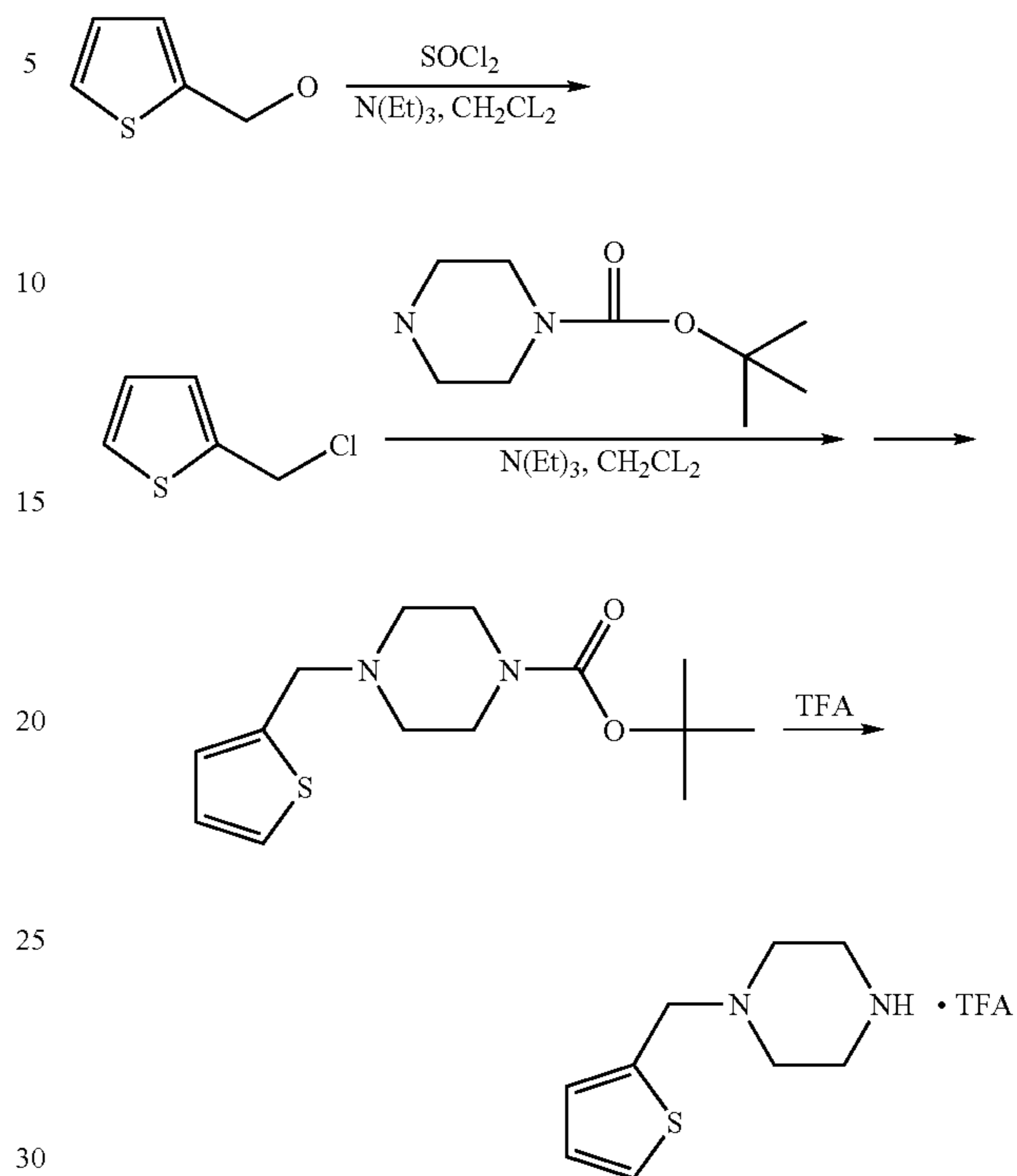
Reaction Scheme 21
