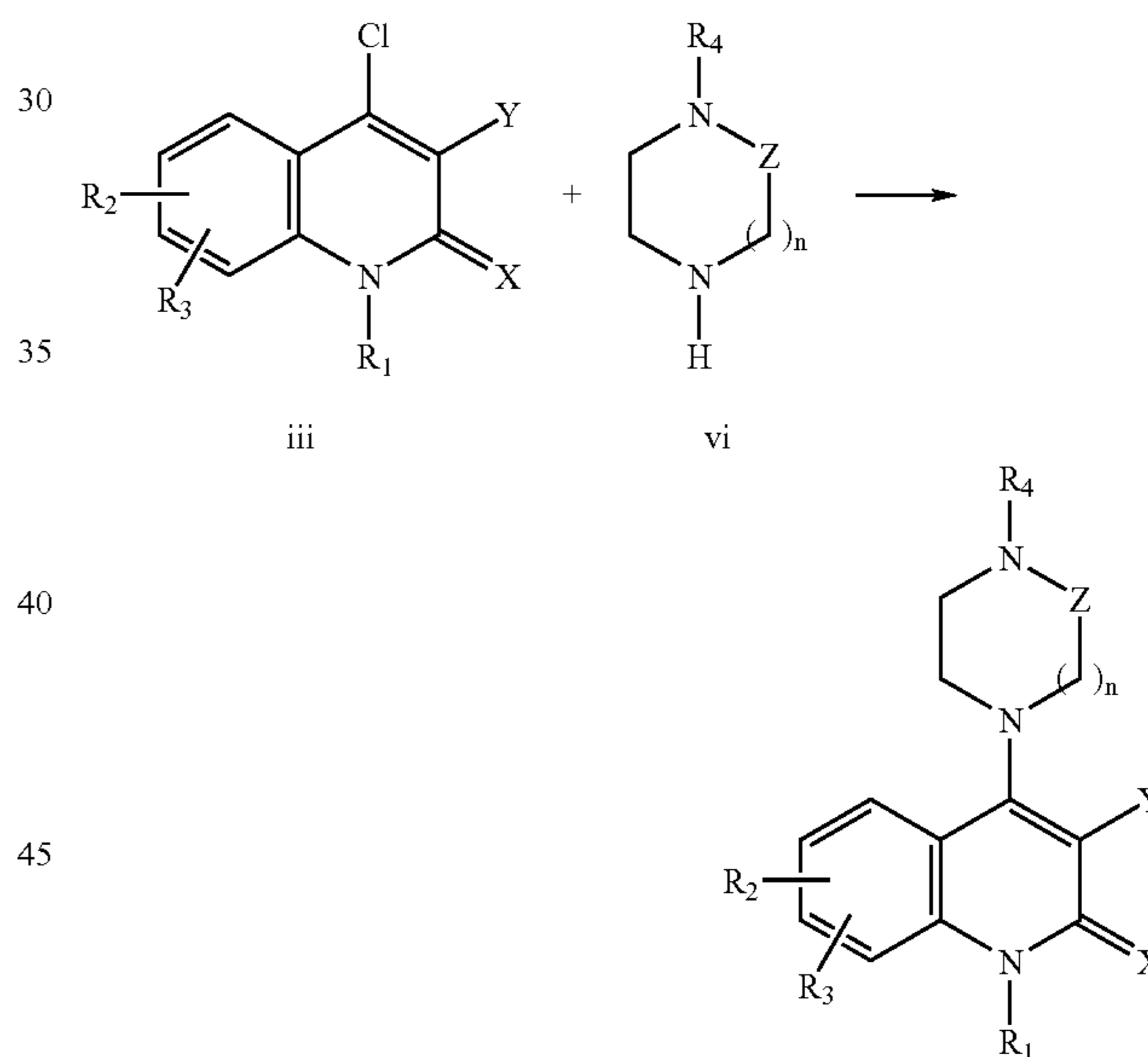
Reaction Scheme 3
