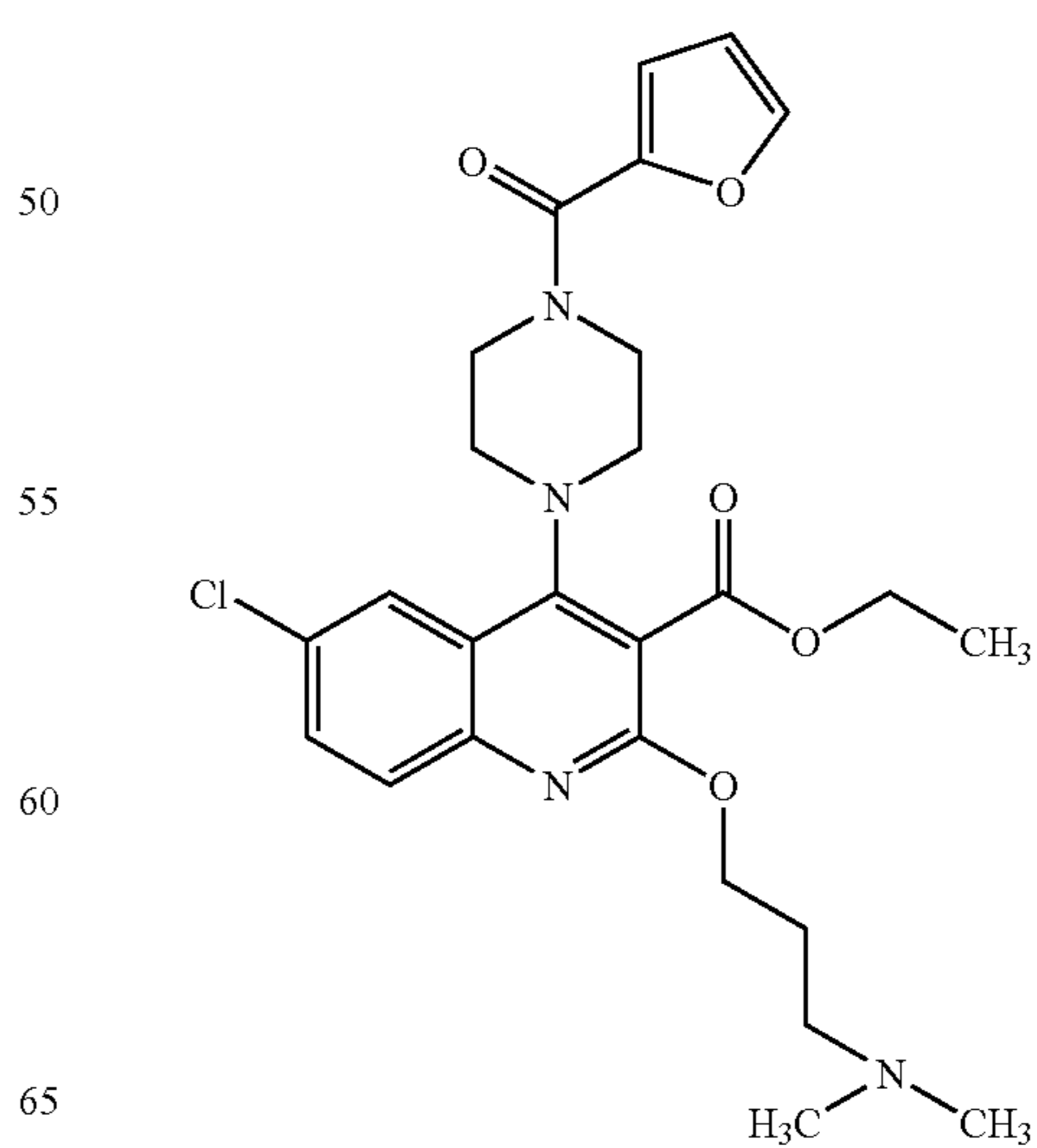
Compound 330
