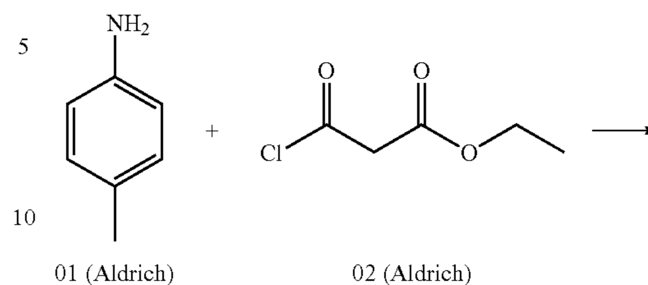
Reaction Scheme 25
