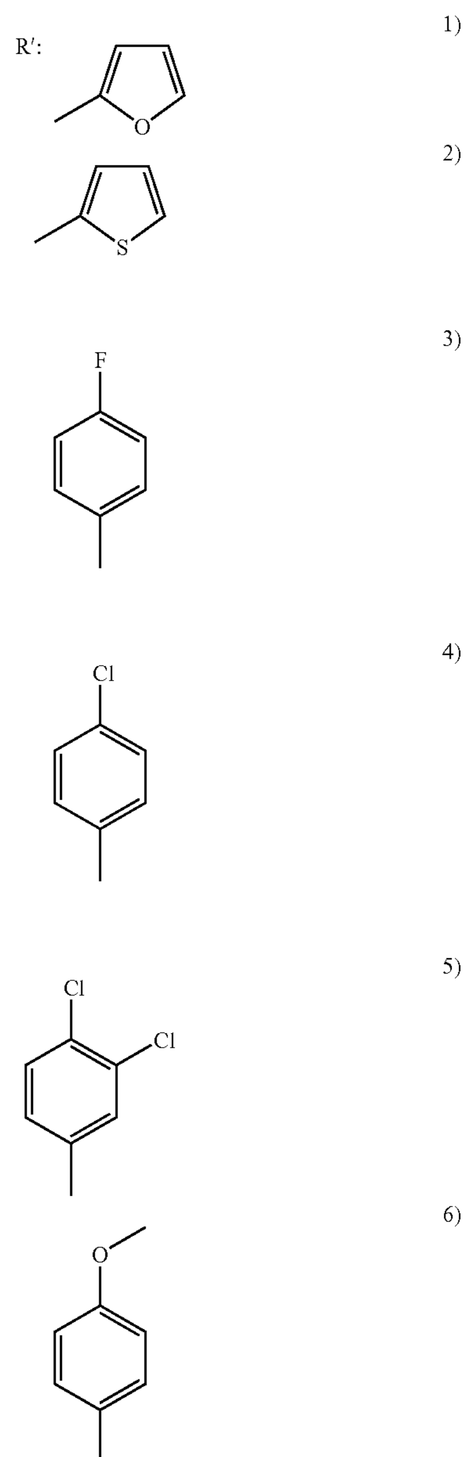
Reaction Scheme 24
