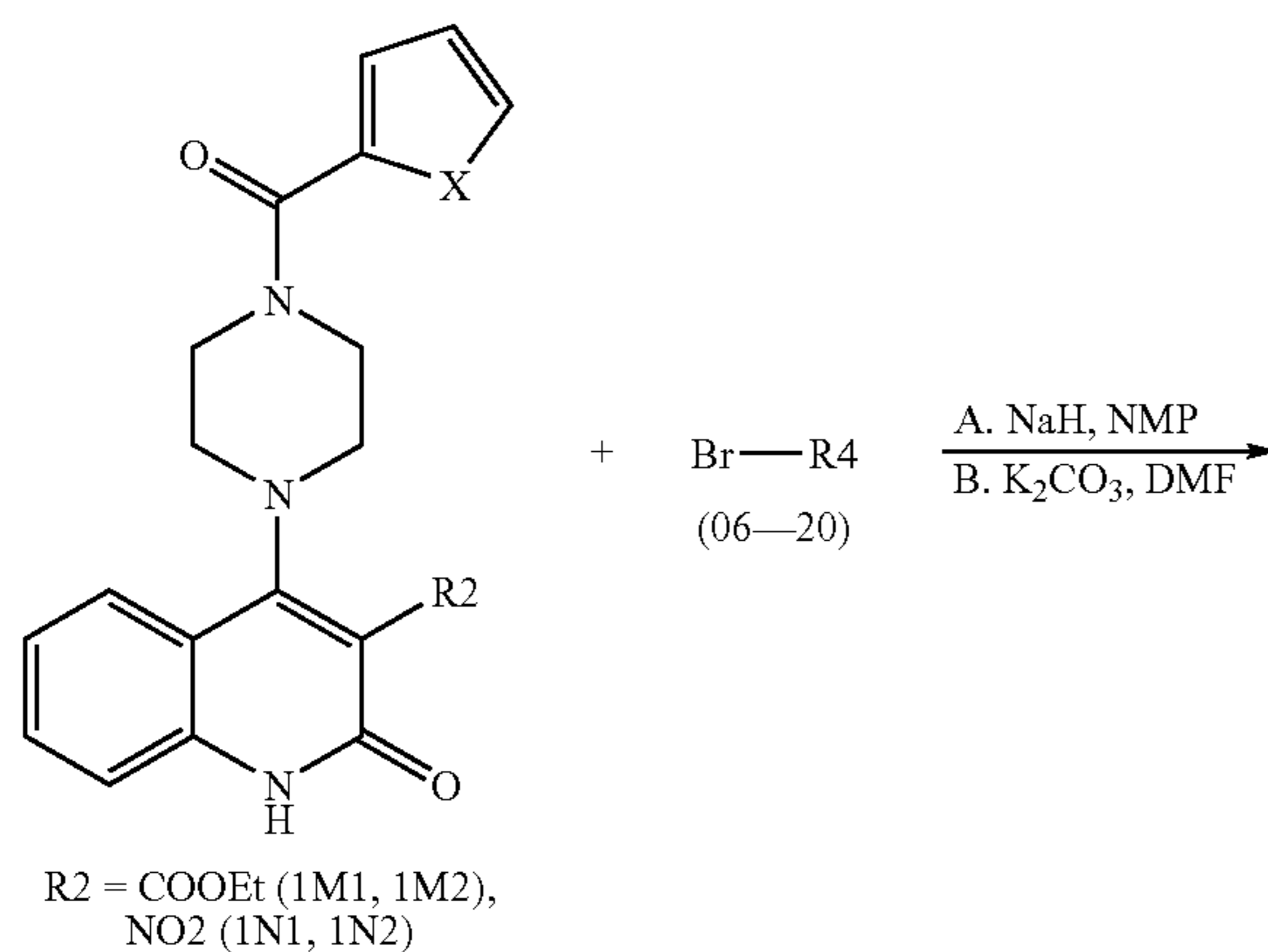
Reaction Scheme 13
