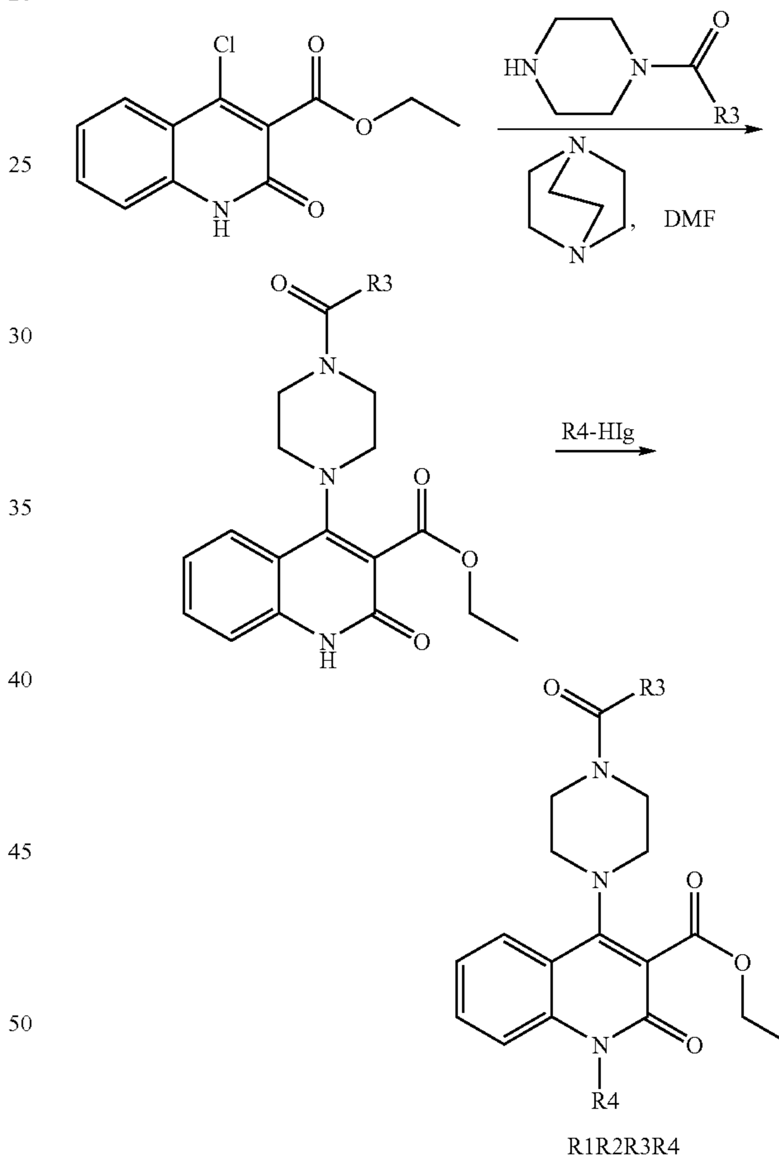
Compound 344
