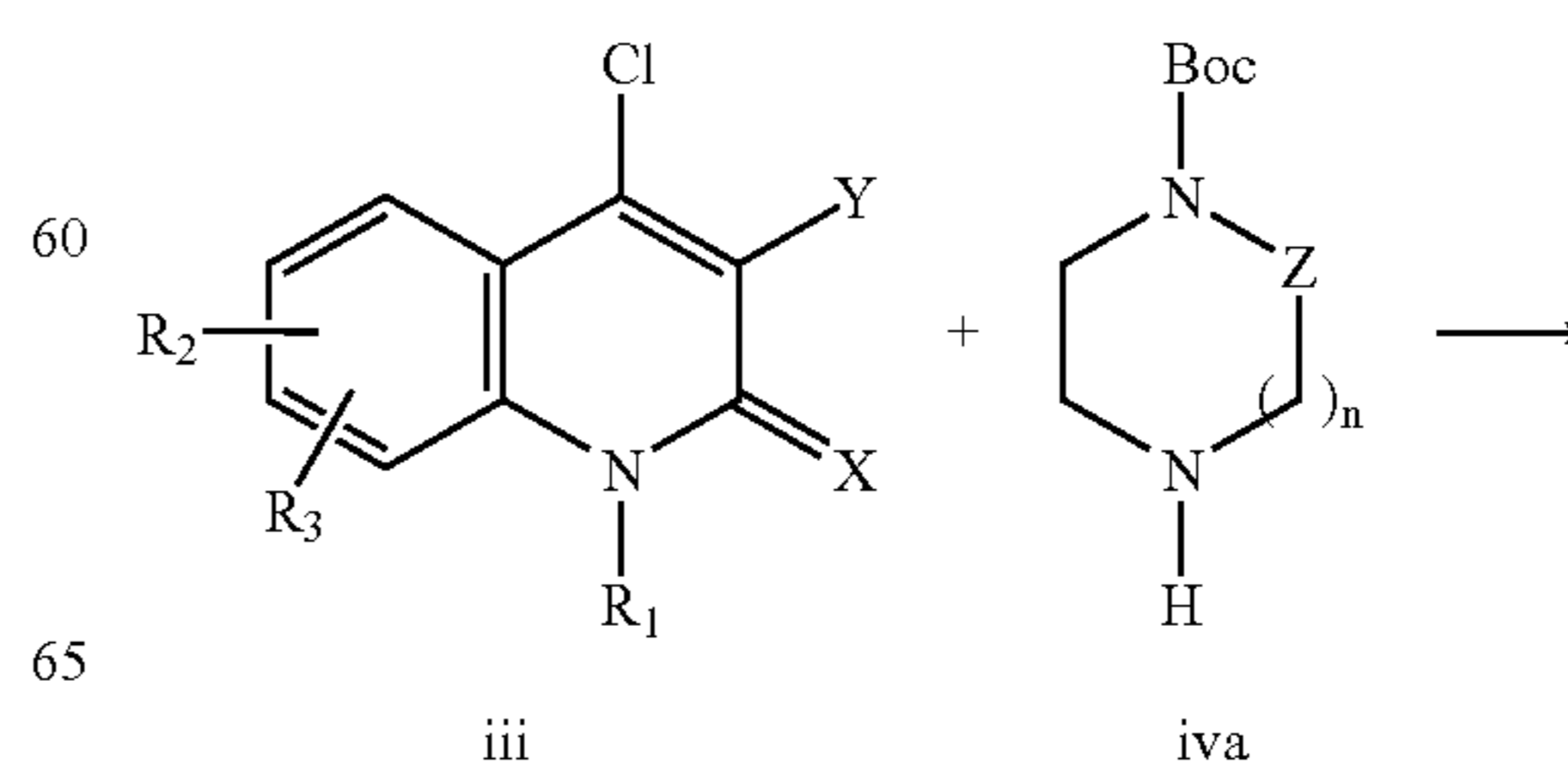
Reaction Scheme 4
