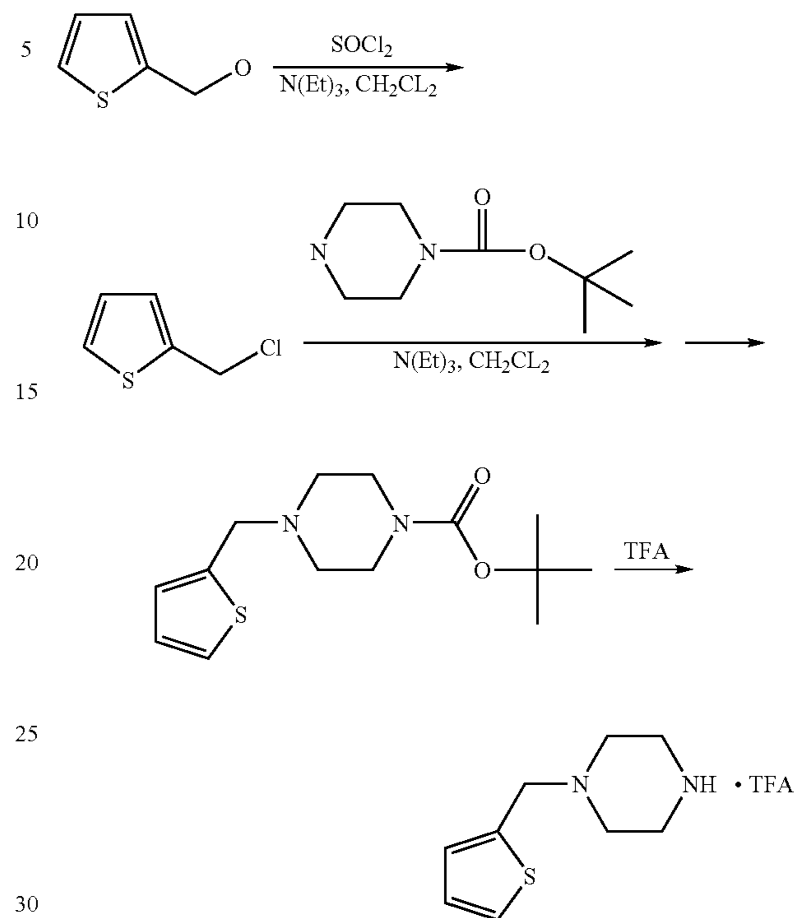
Reaction Scheme 21
