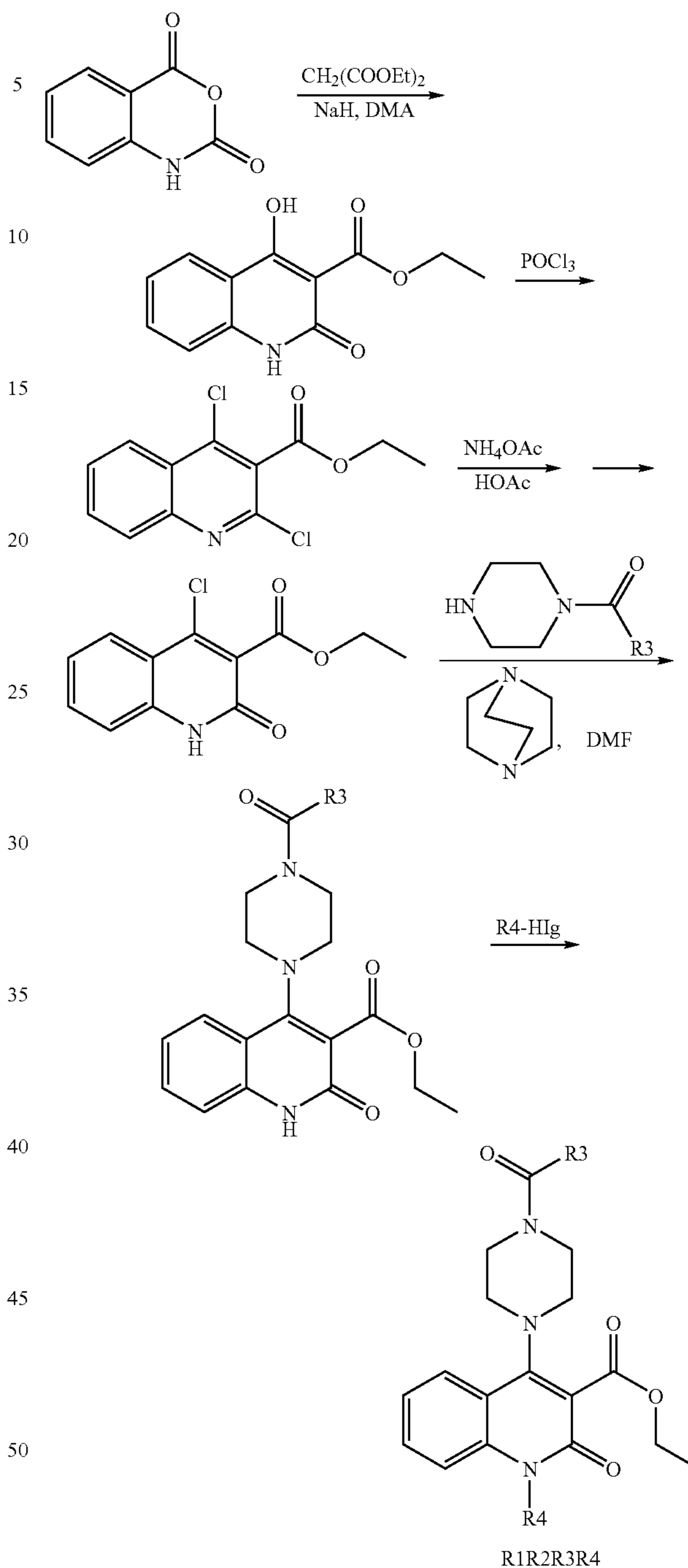
Compound 343
