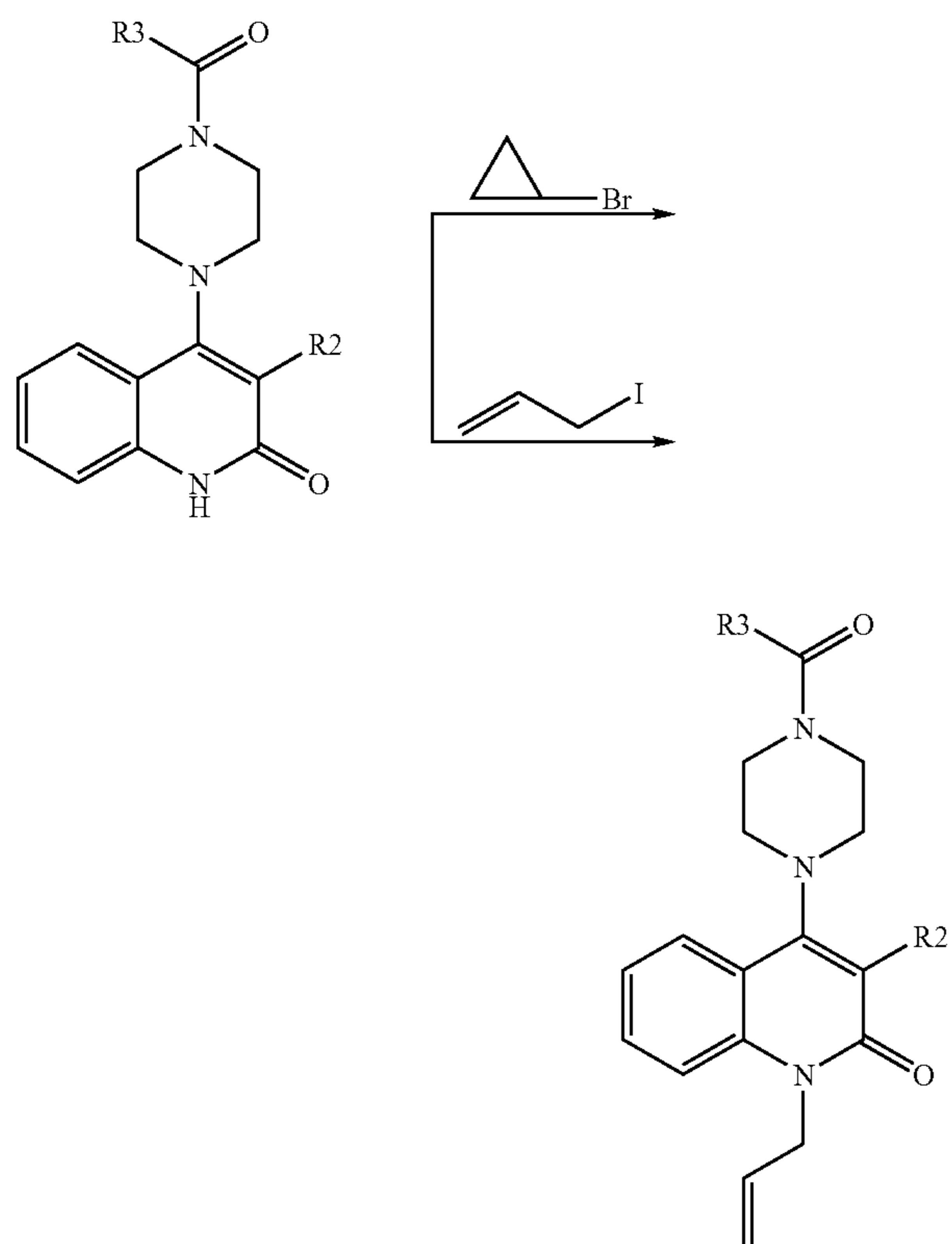
Reaction Scheme 8
