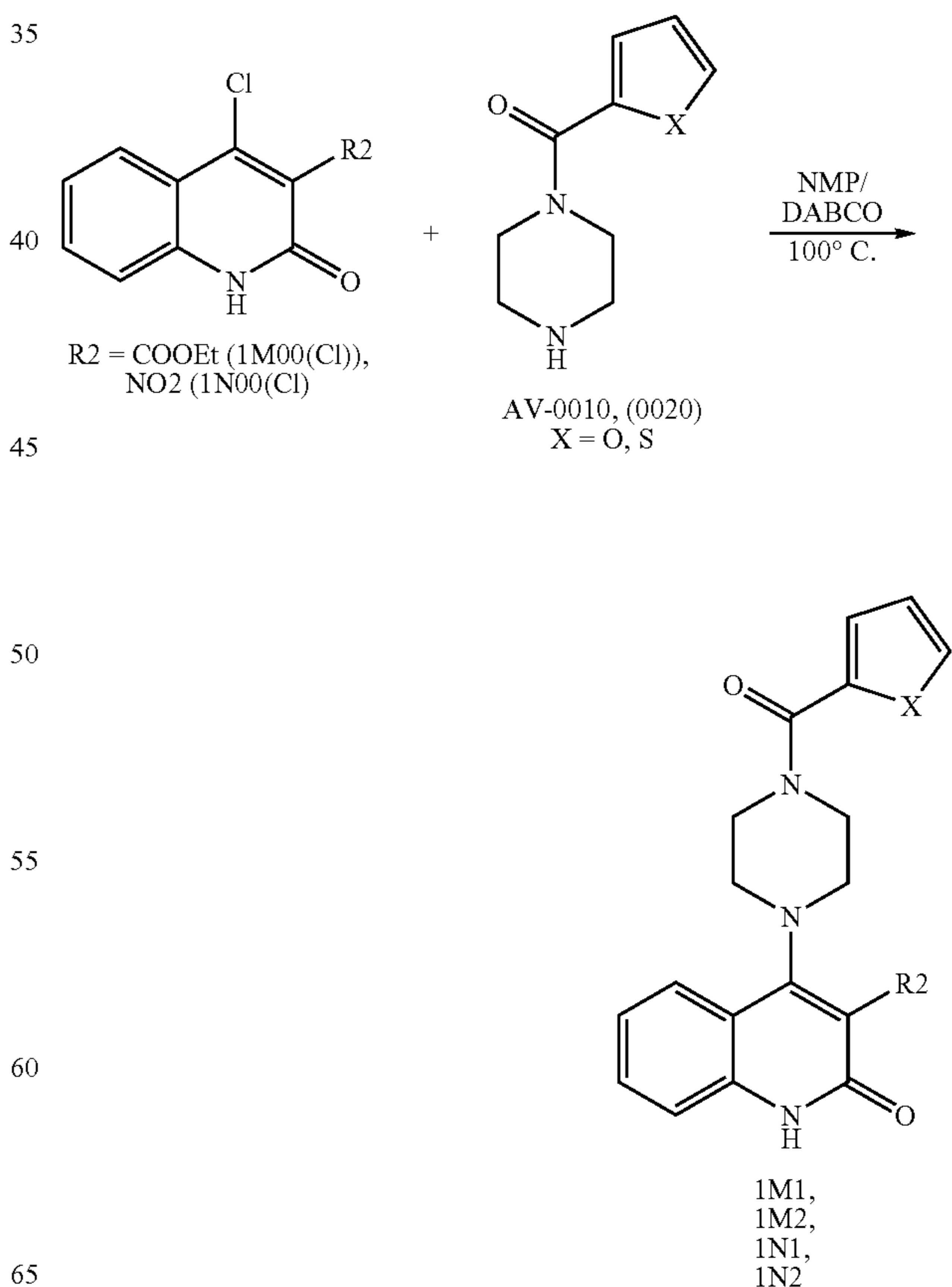
Reaction Scheme 12
