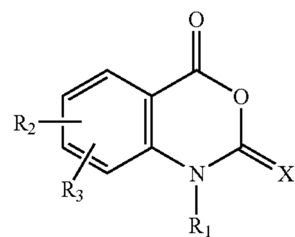
Reaction Scheme 1
