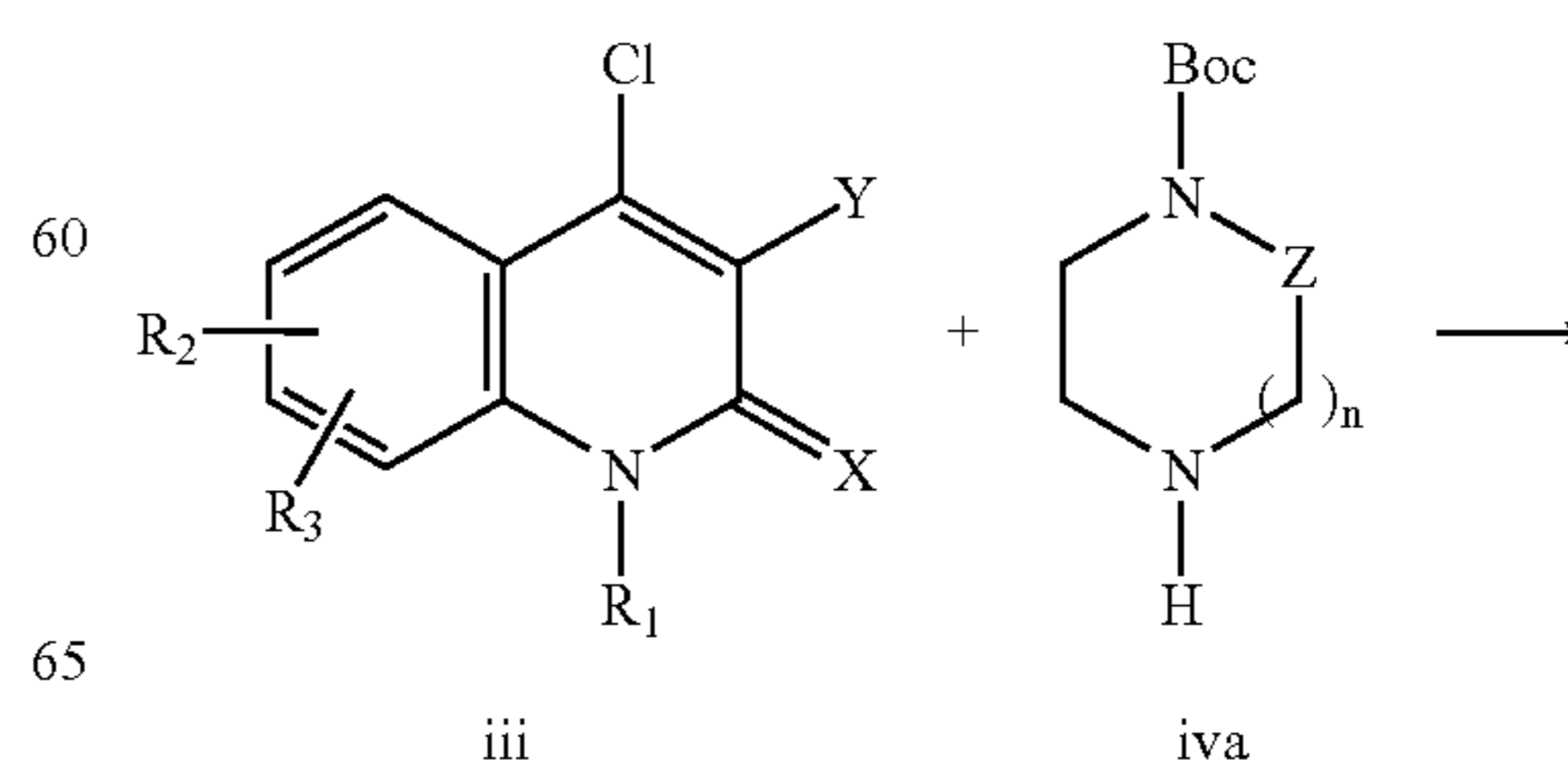
Reaction Scheme 4
