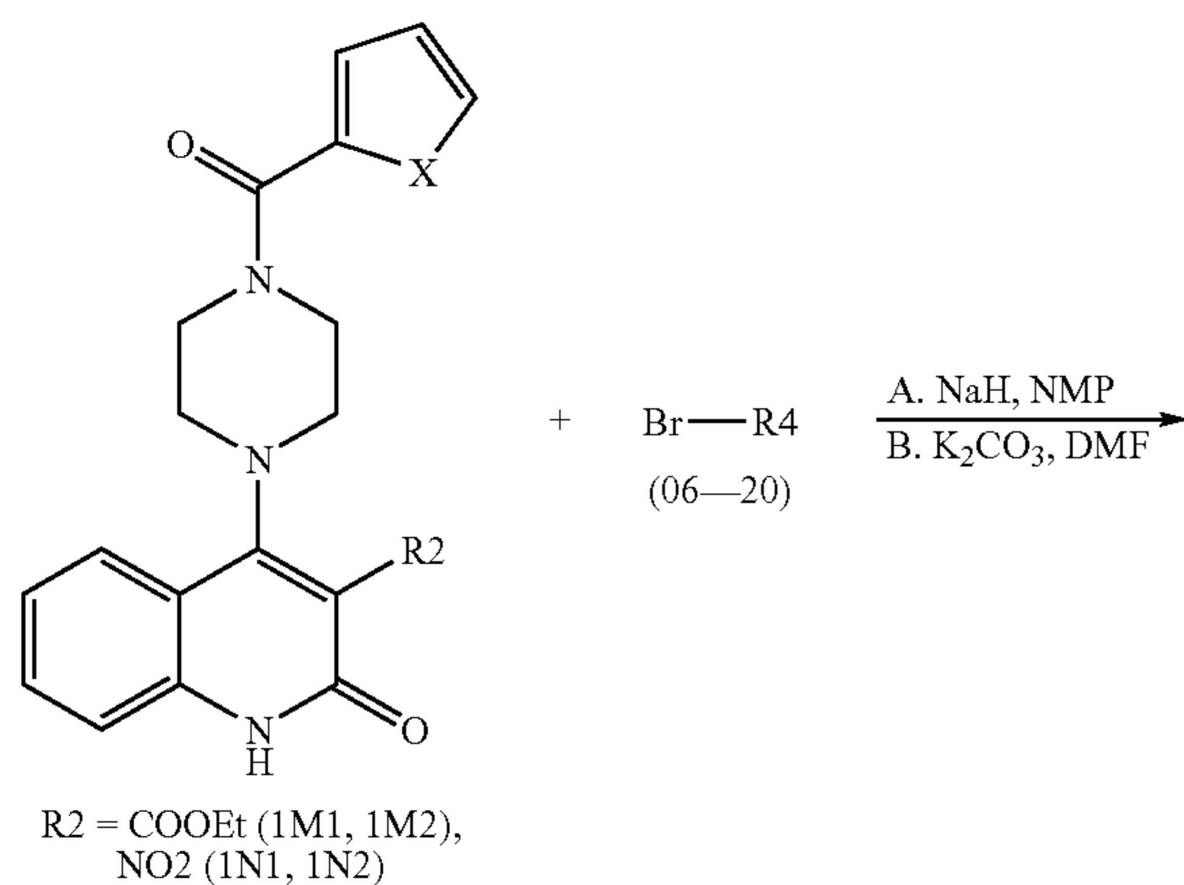
Reaction Scheme 13
