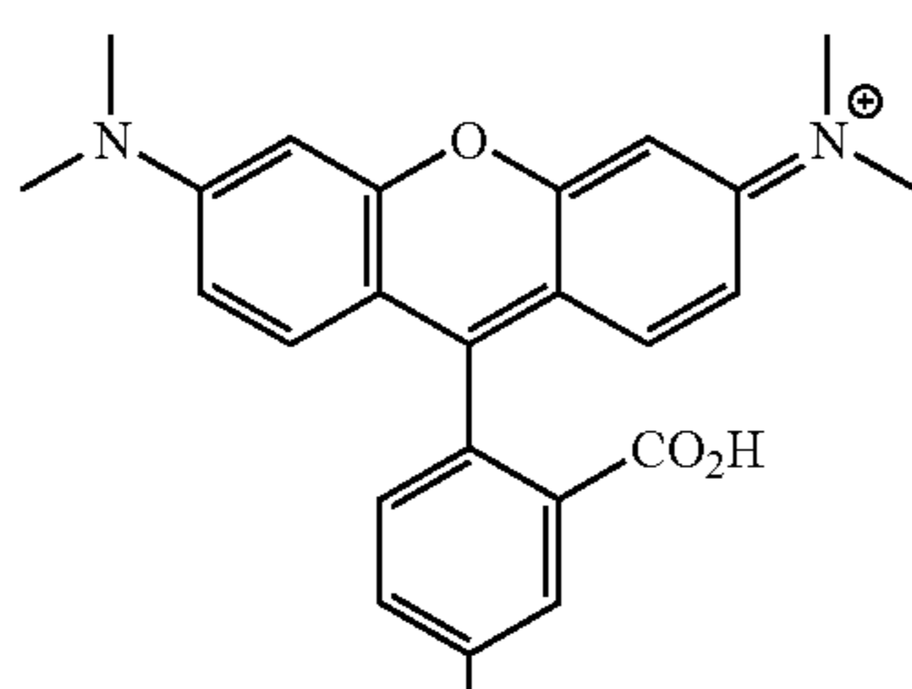
TAMRA
