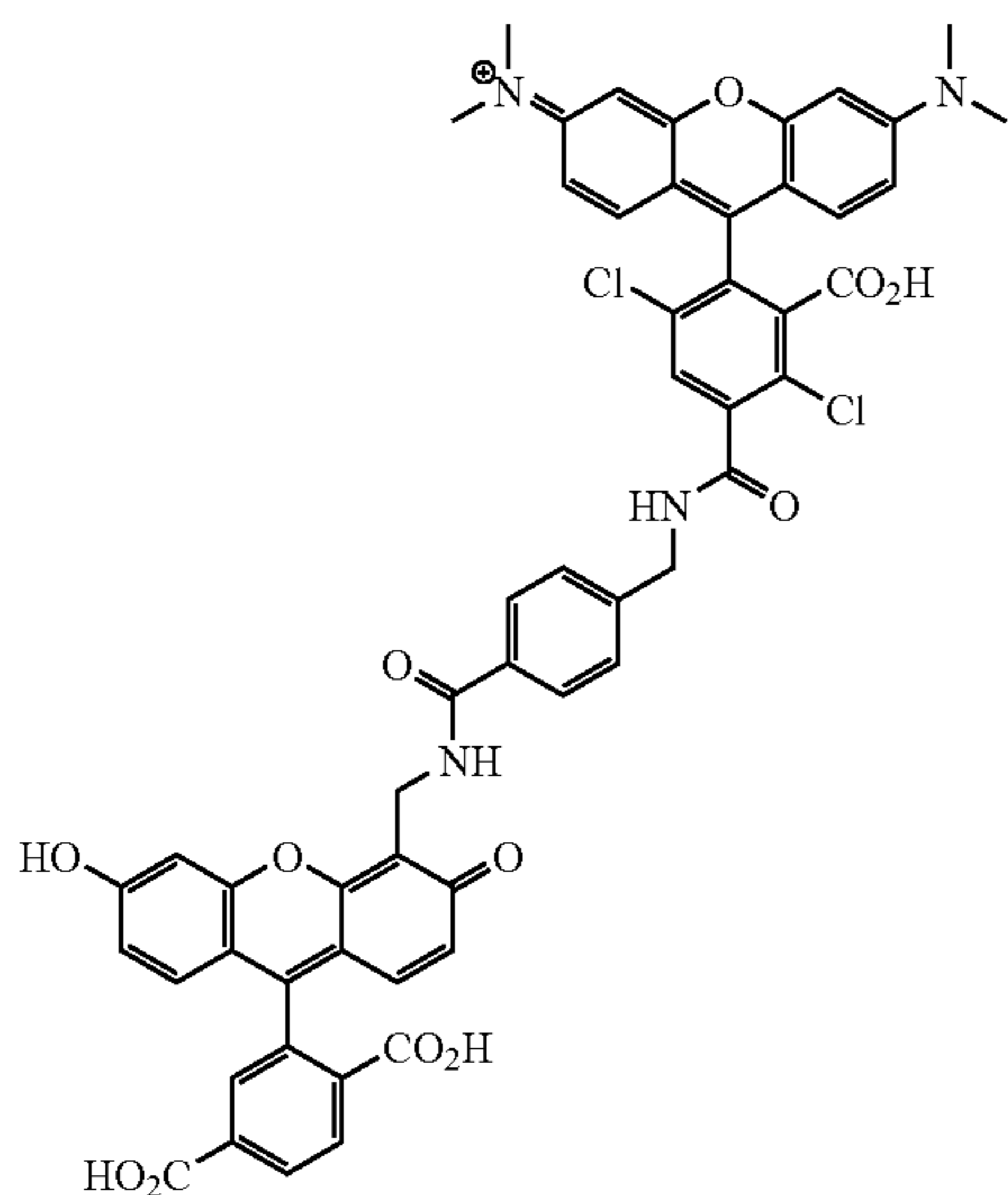
6-CF-B-DTMR-2
