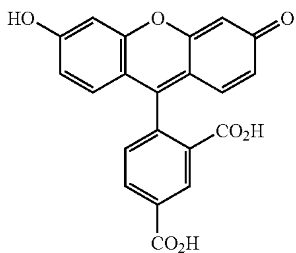
5-carboxyfluorescein
