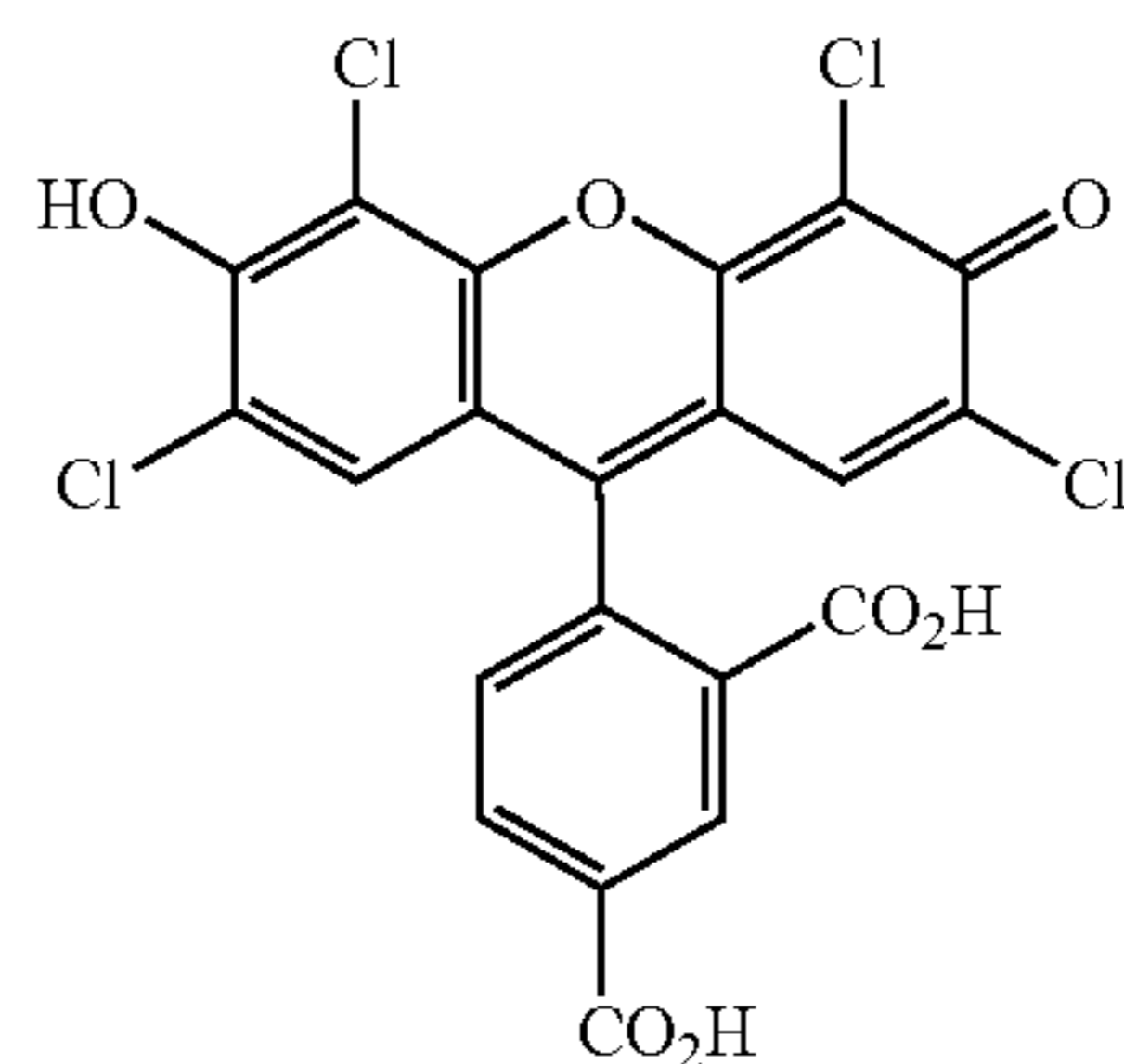
ZOE
