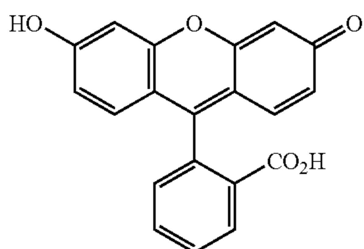
Fluorescein
