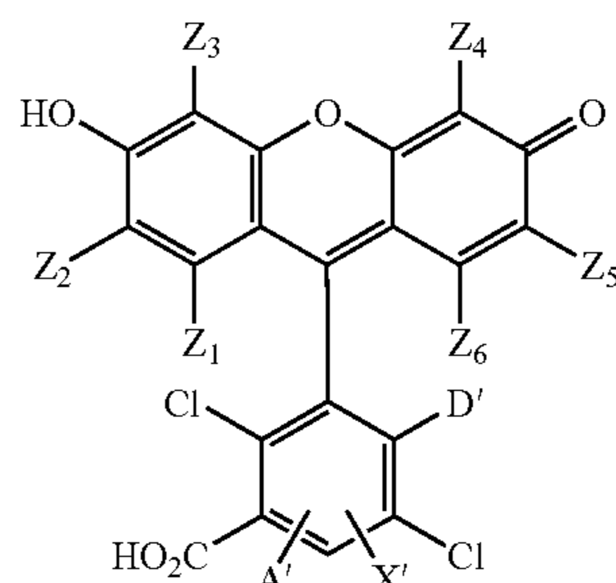
4,7-Dichlorofluorescein (See Pat. No. 5,188,934)
