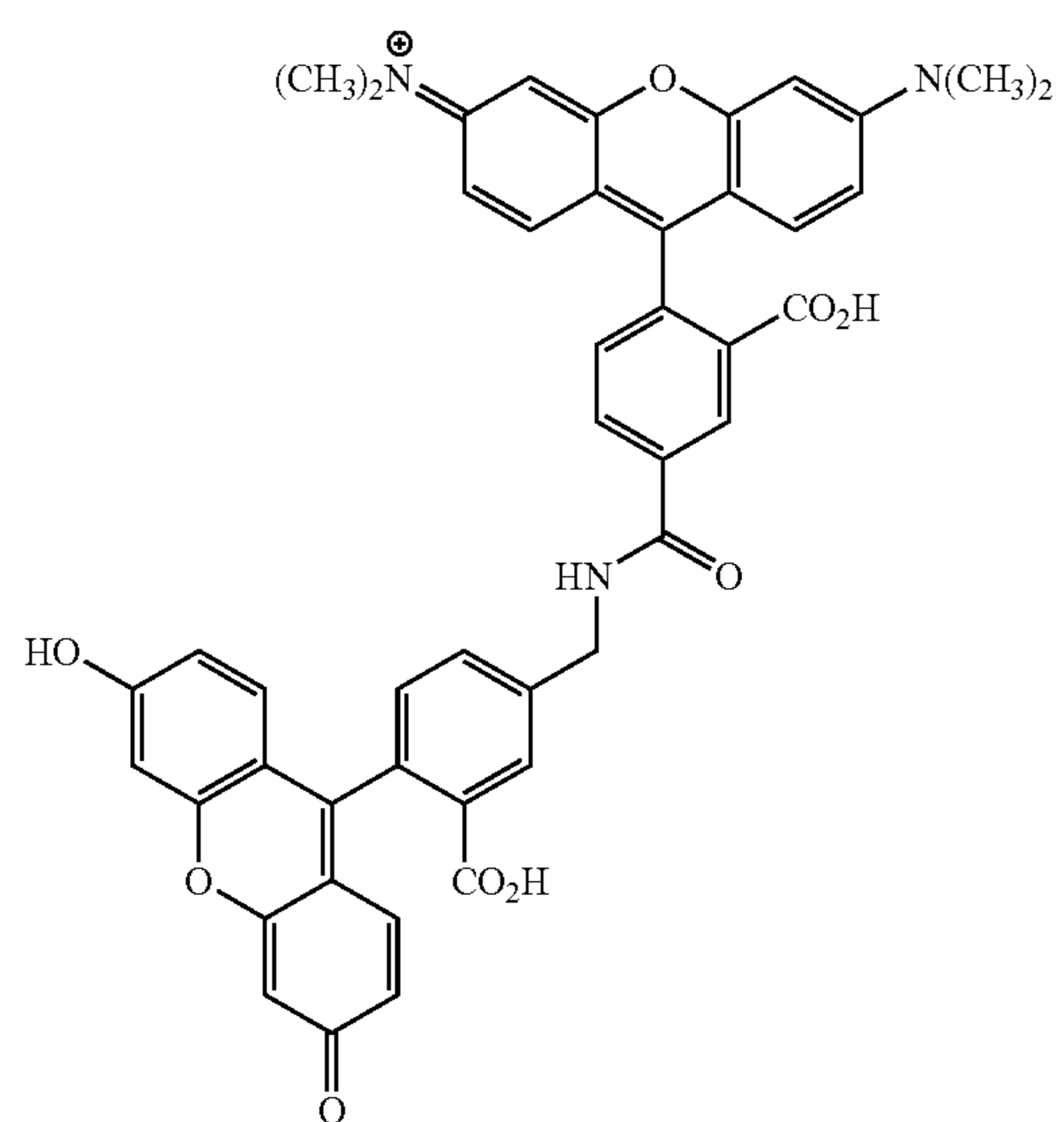
5-TMR-5AMF
