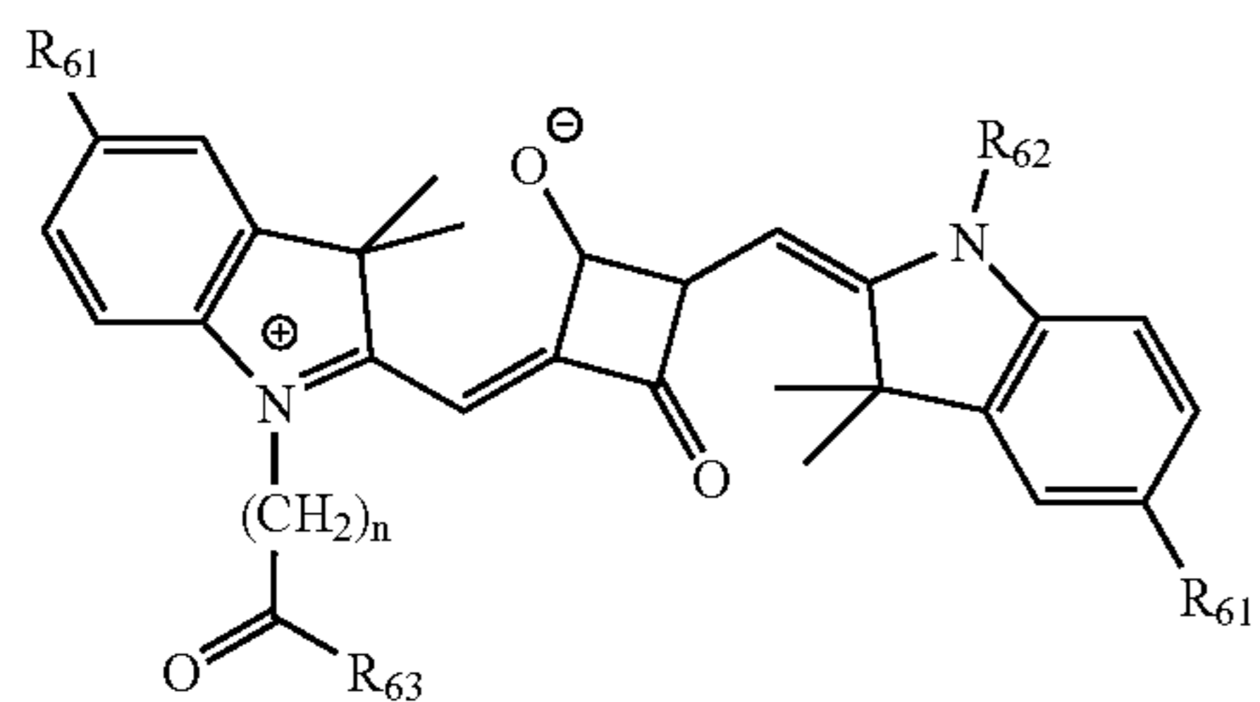
SQUARINE
