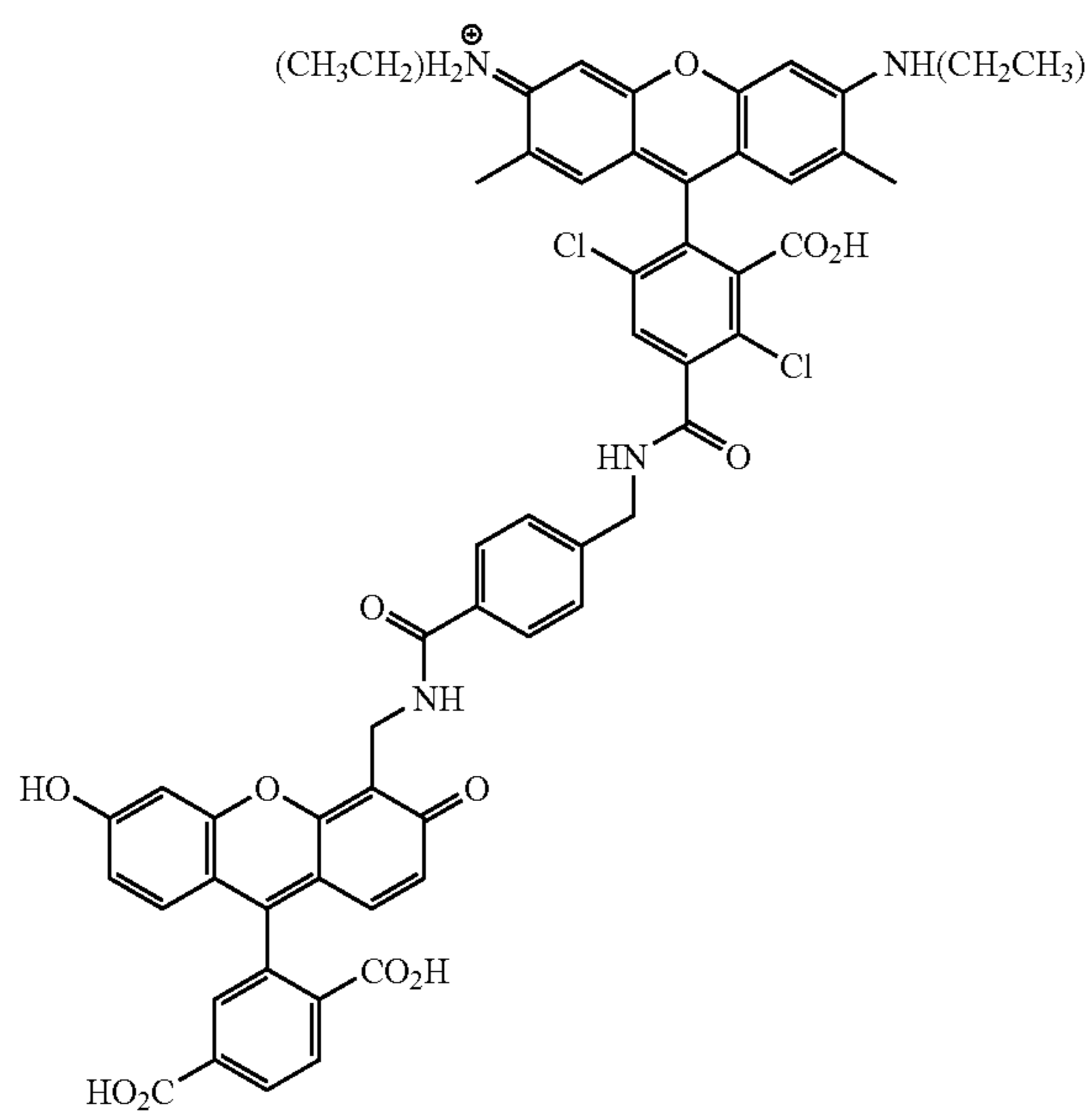
6-CFB-DR6G-2
