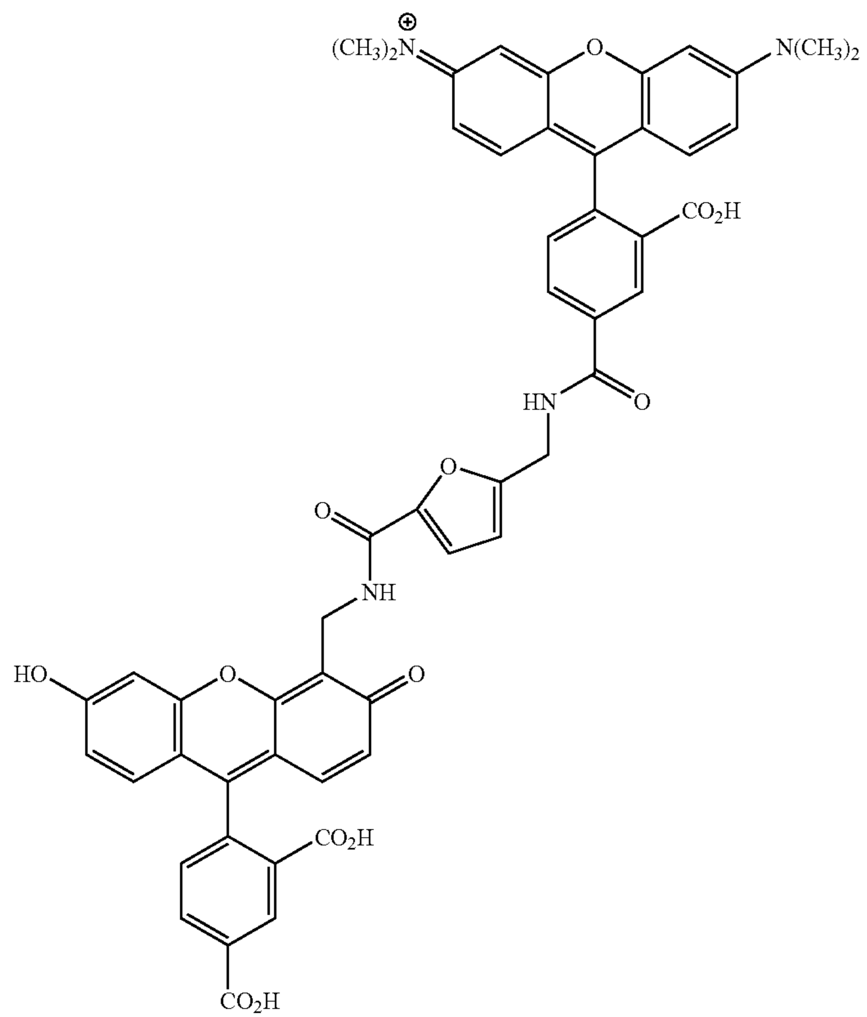
5-TMR-F-CF
