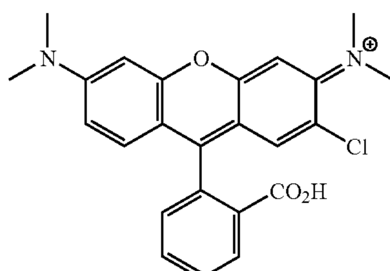
5-carboxyrhodamine
