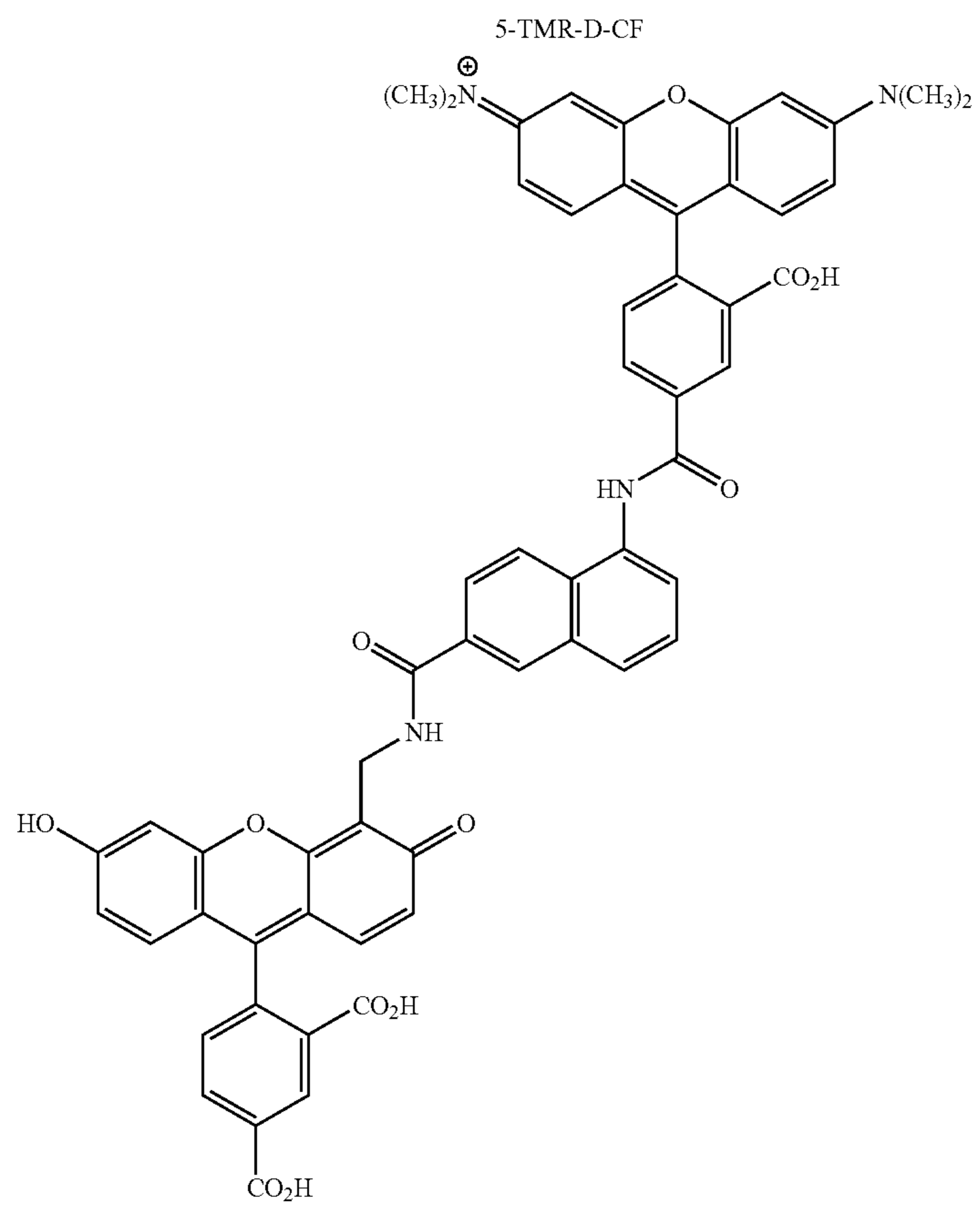
5-TMR-N-CF
