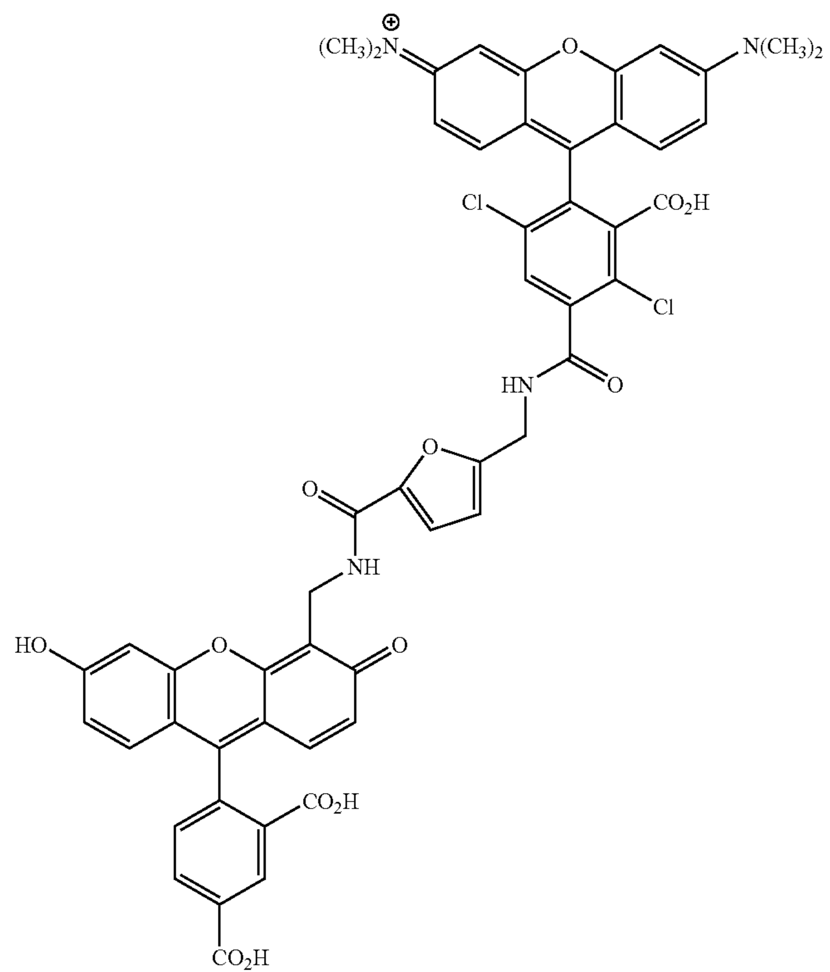
5-DTMR-F-CF
