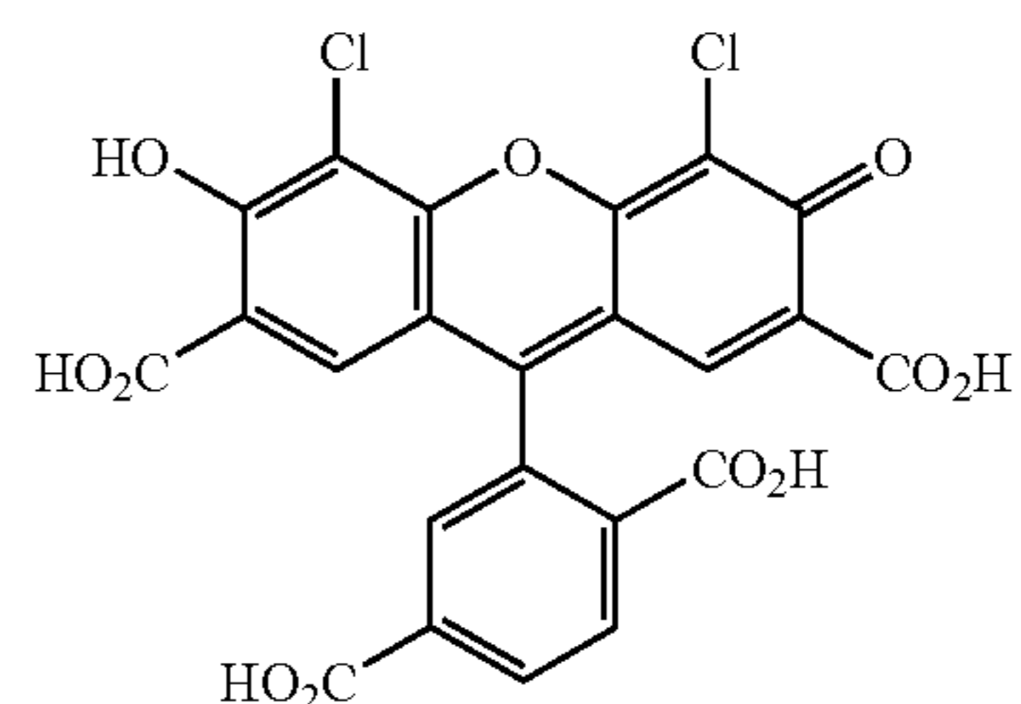
JOE
