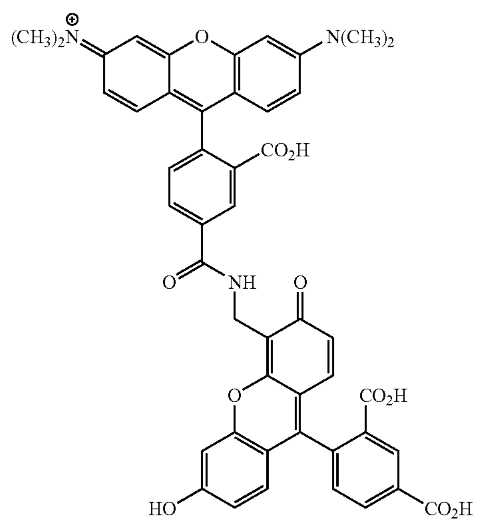
5TMR-CF
