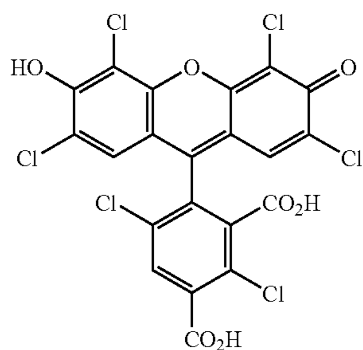
5-carboxy-HEX
