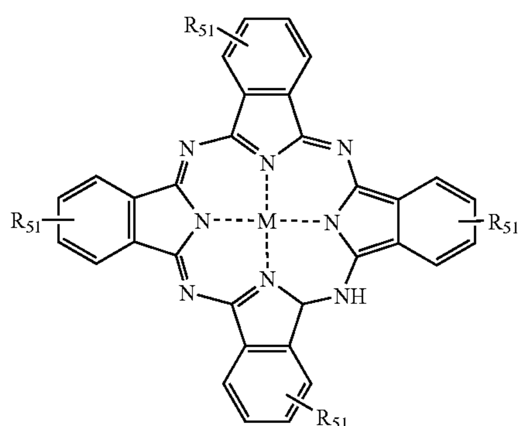
PHTHALOCYANINE
