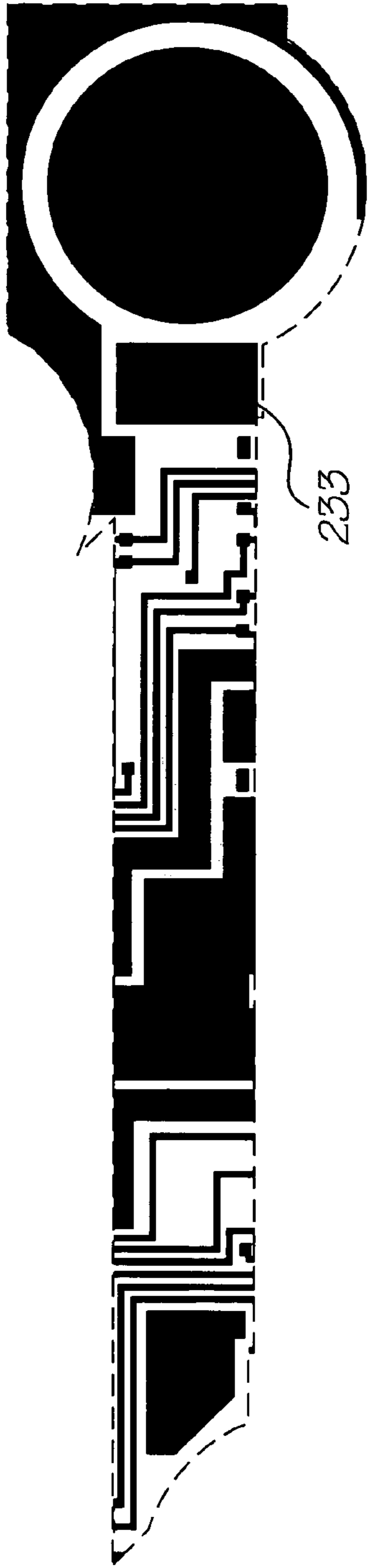
Metal 2 mask
