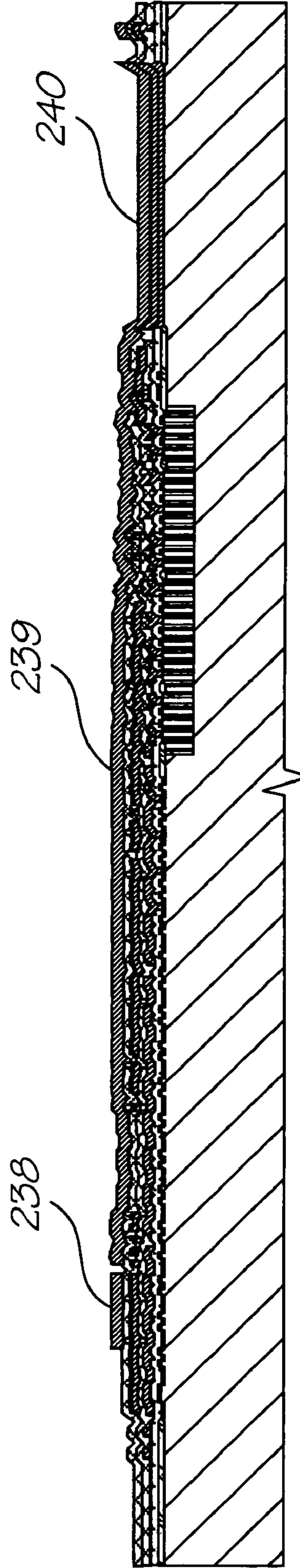
Deposit metal 3
