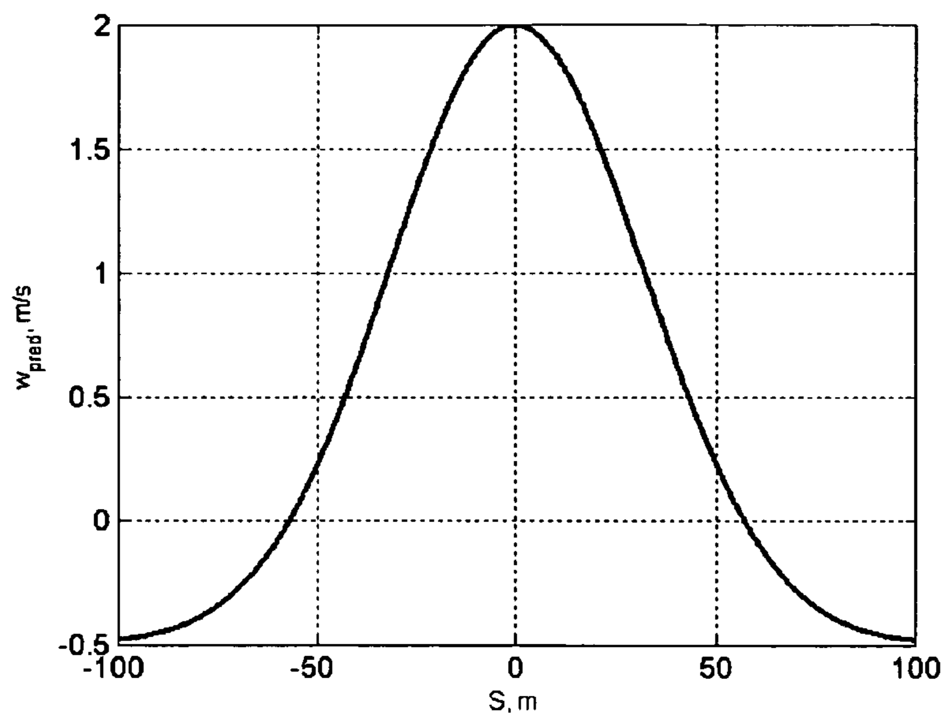
Figure 5. Predicted updraft velocity distribution from equation 17 for w_{up}=2\text{m/s} and r_{up}=45\text{m} .
