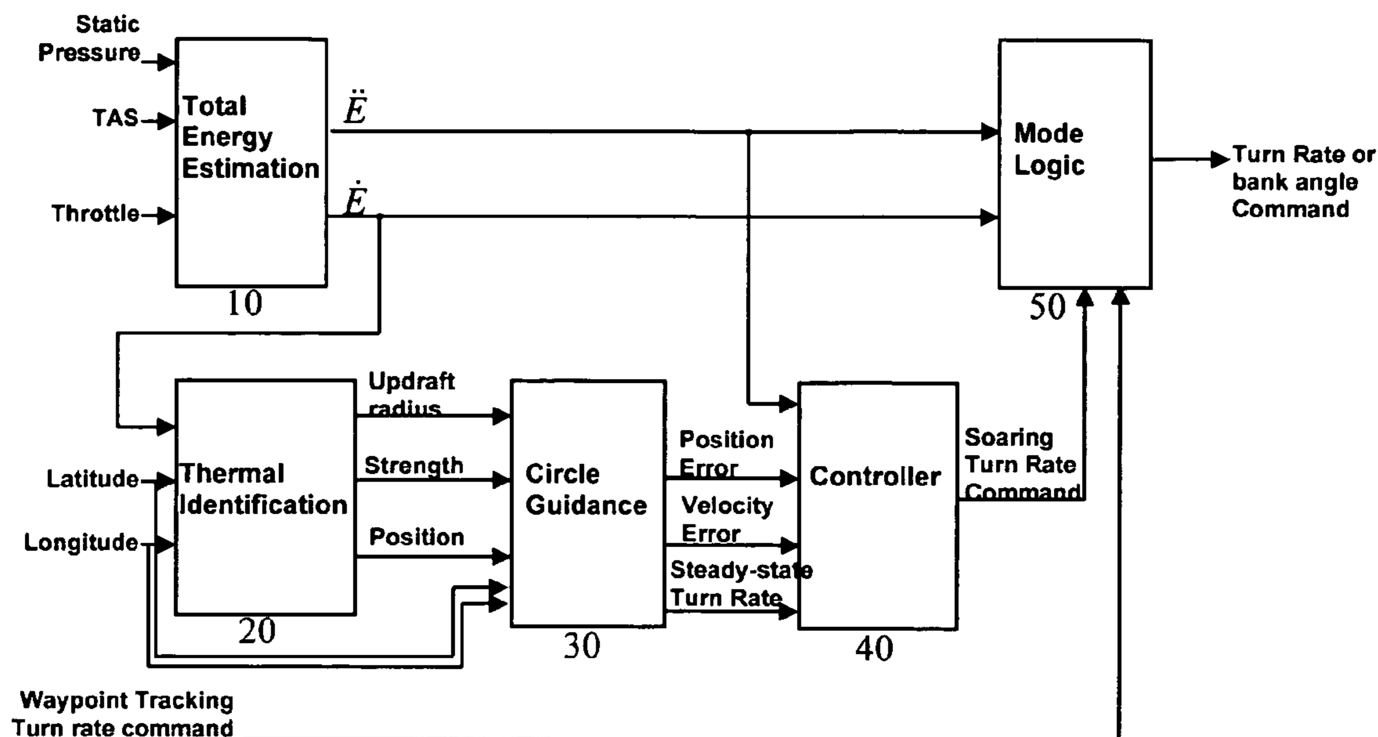
Top level block diagram of the present invention.
