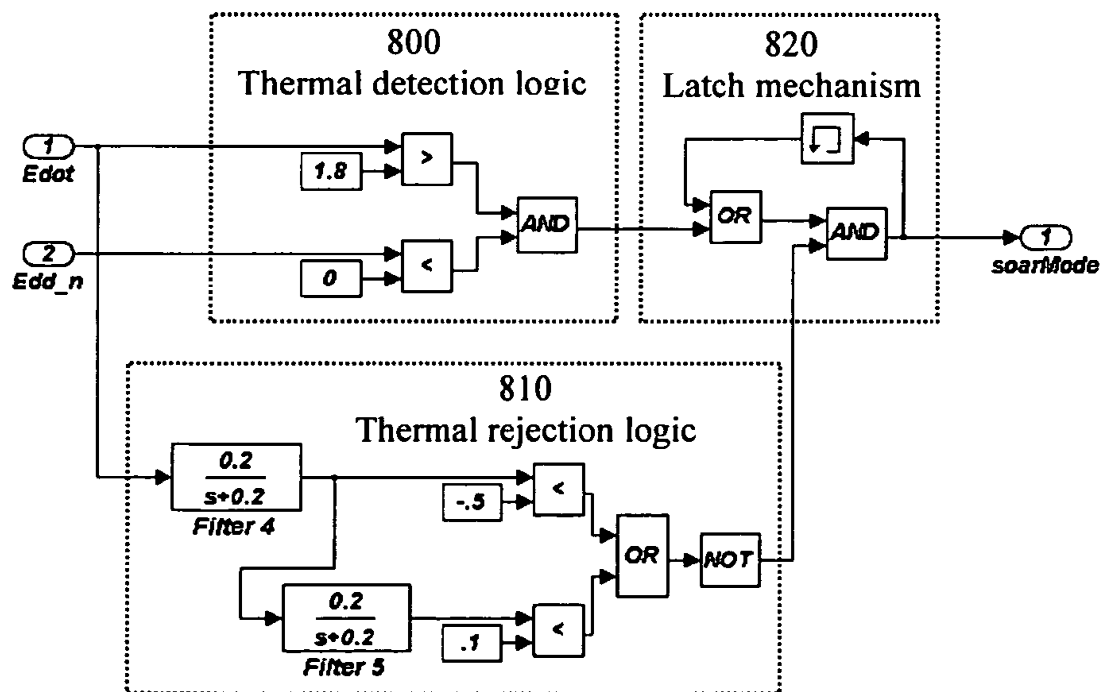
Figure 8. Block diagram of mode logic (block 50).
