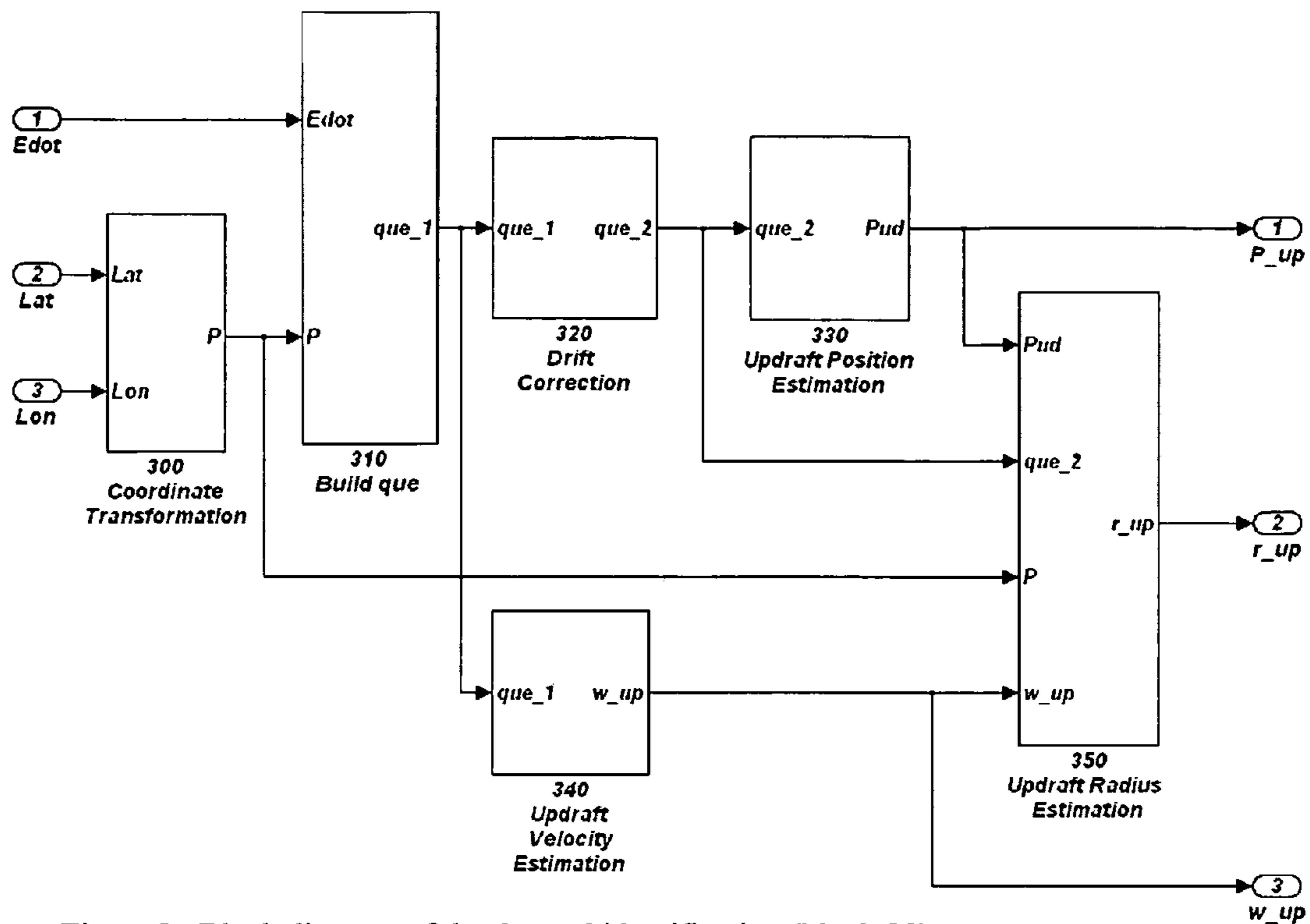
Figure 3. Block diagram of the thermal identification (block 20).
