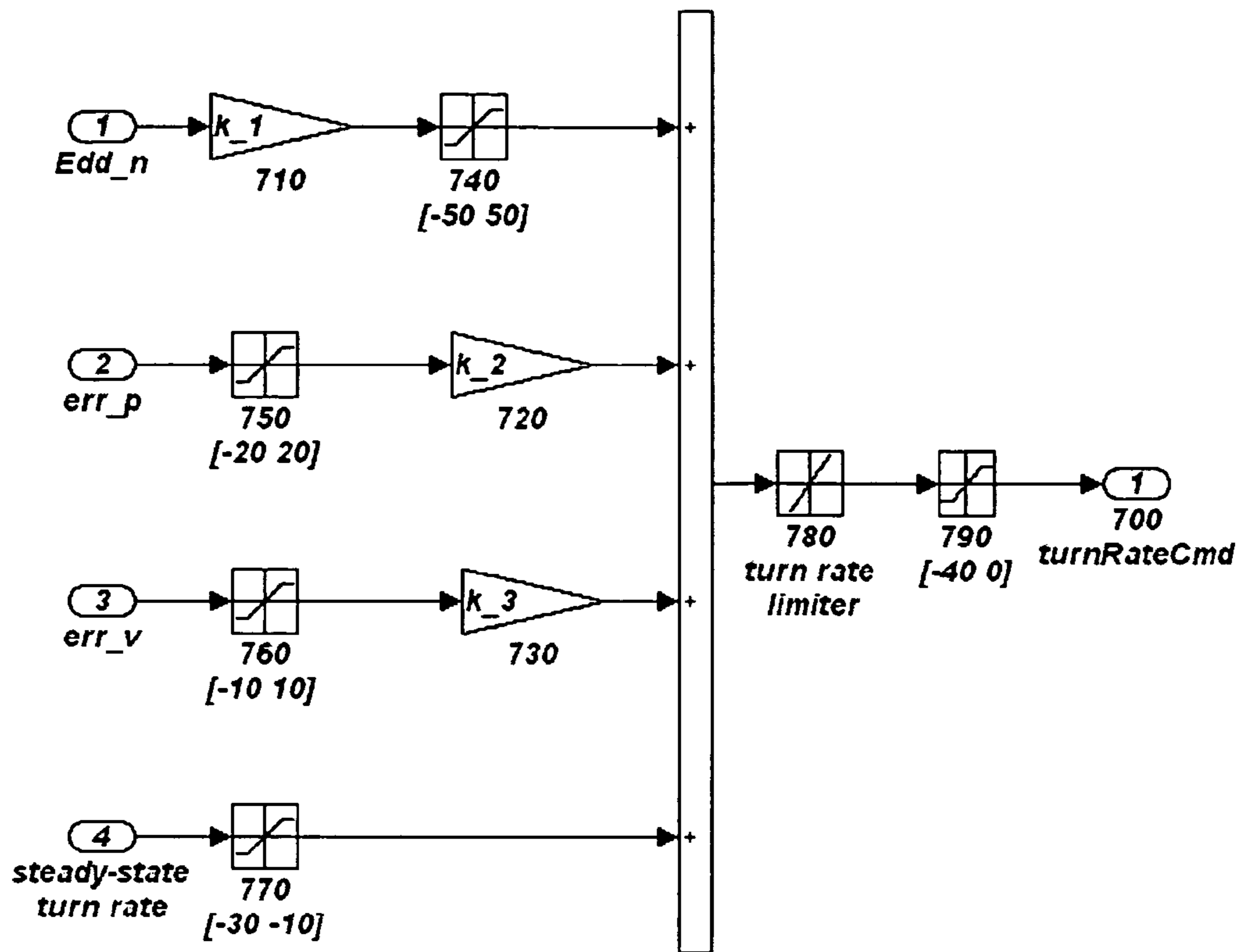
Figure 7. Block diagram of soaring controller (block 40).
