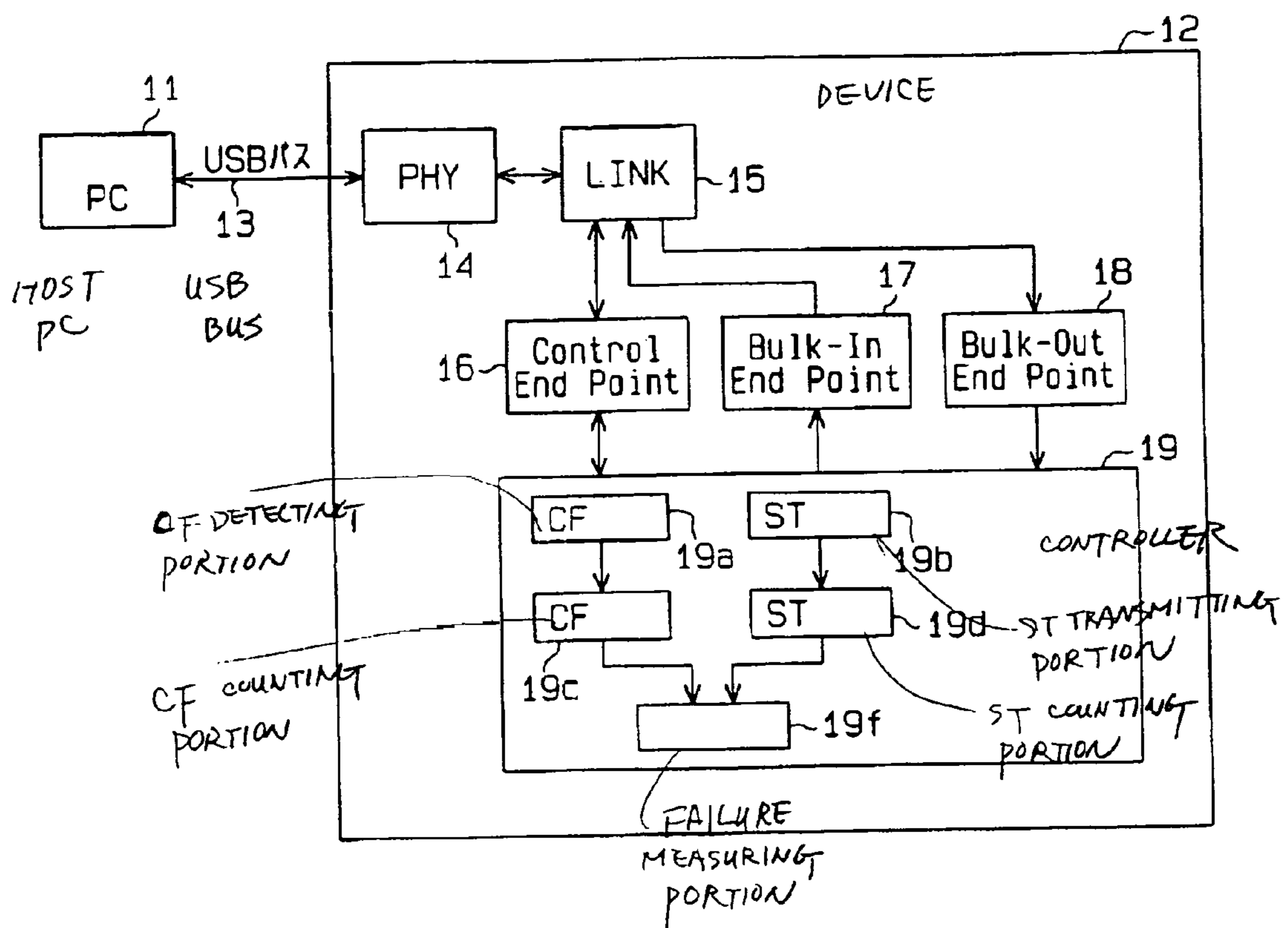
BLOCK DIAGRAM ILLUSTRATING THE THIRD EMBODIMENT
