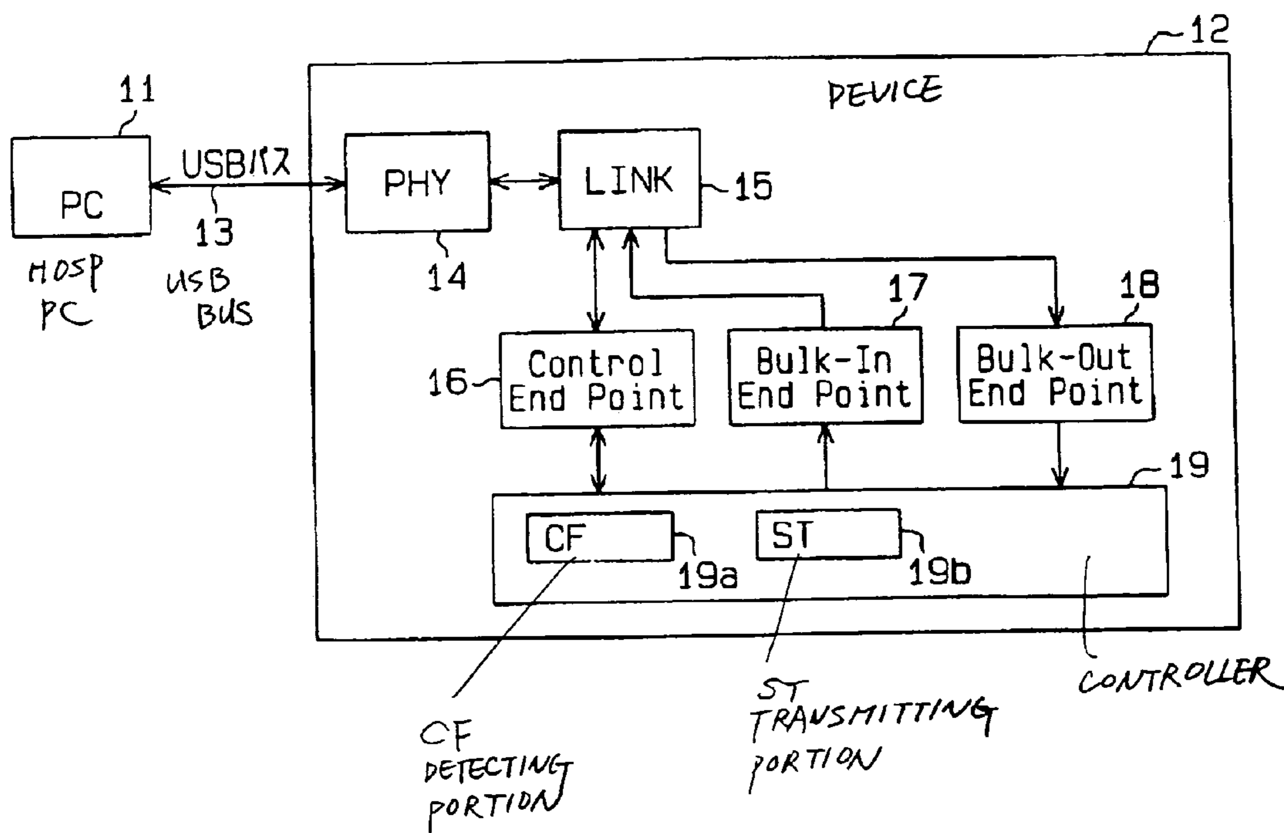
BLOCK DIAGRAM ILLUSTRATING THE FIRST EMBODIMENT
