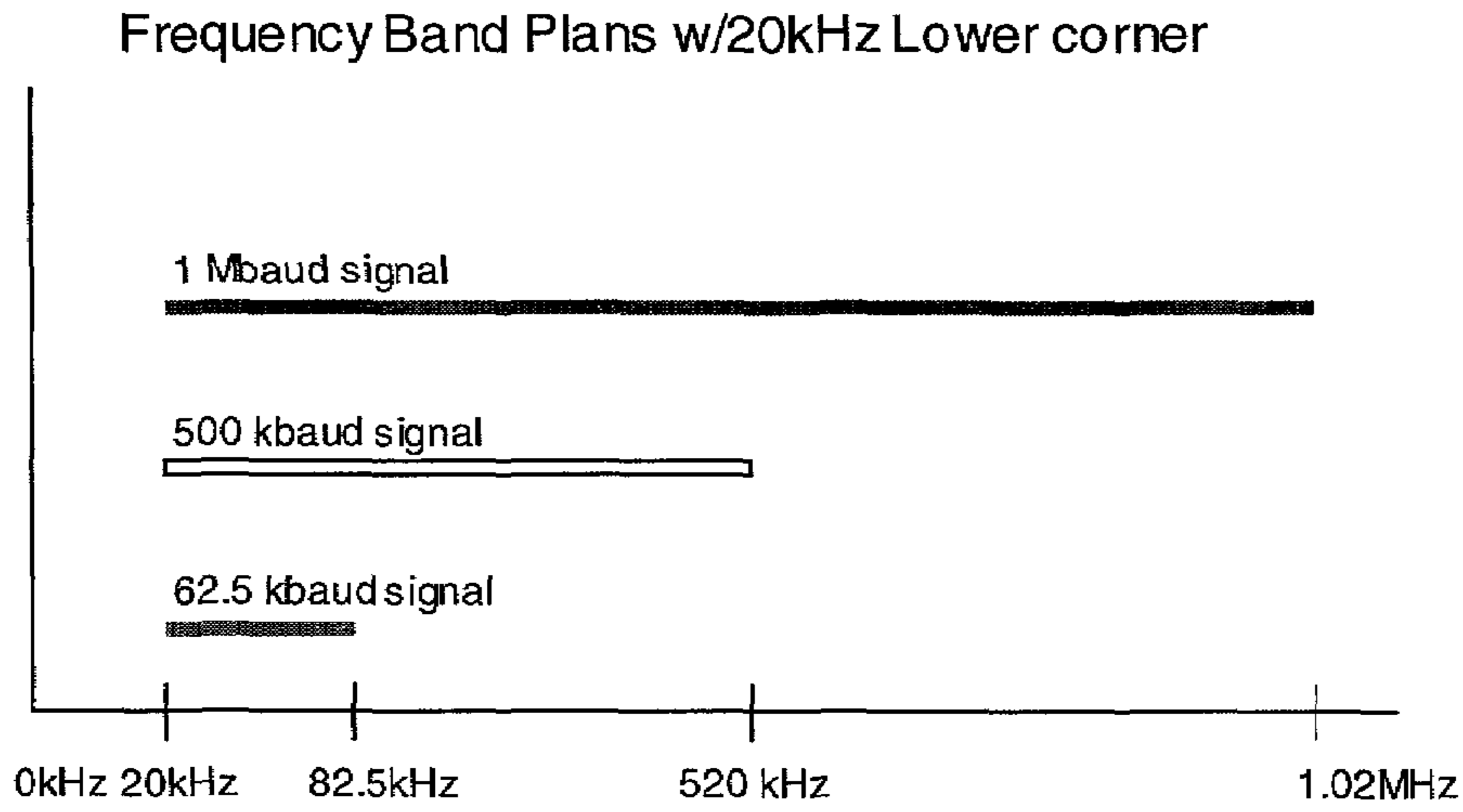
Figure 4 – Example Bandplans with 20kHz lower corner frequency
