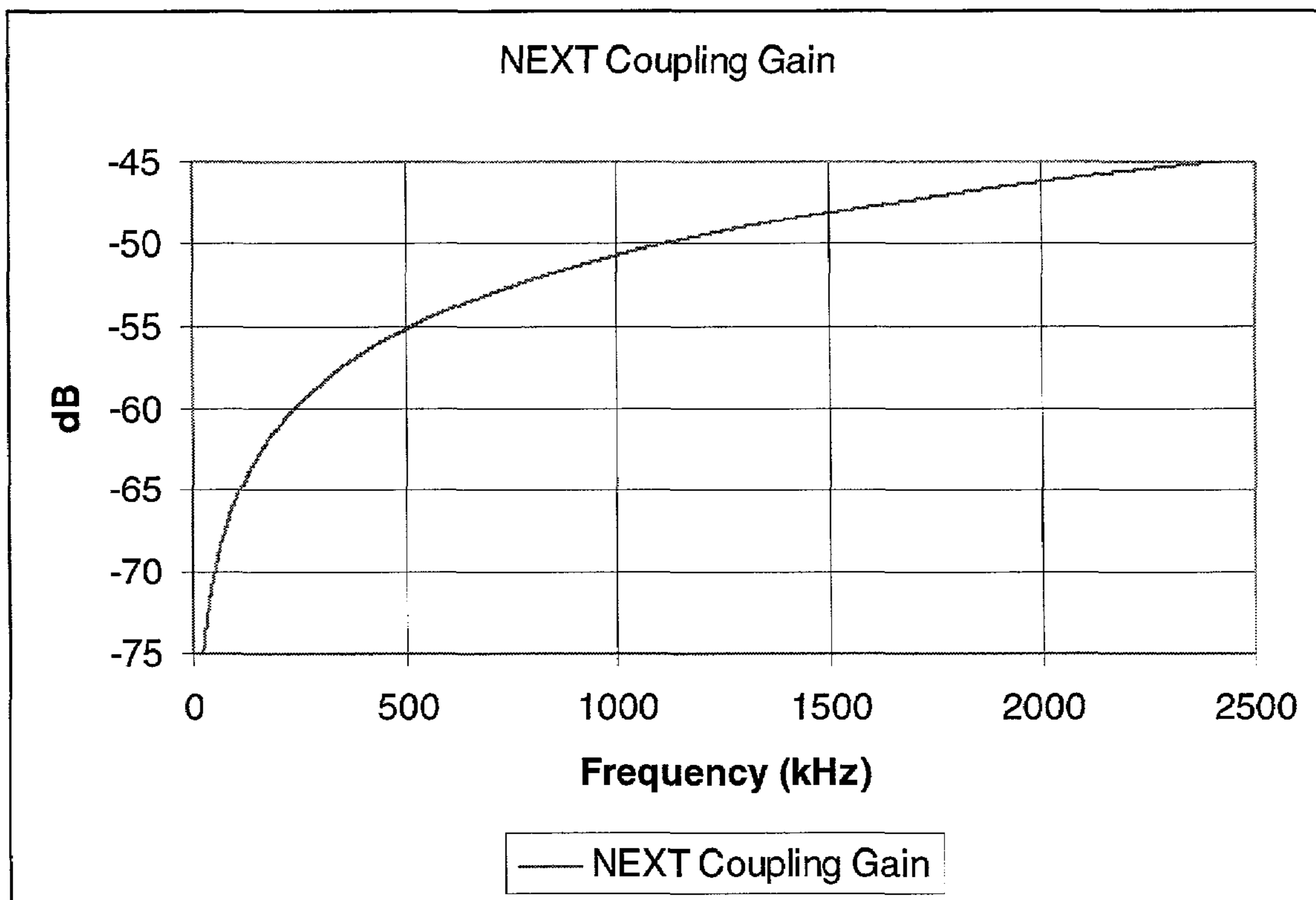
Figure 3 Near End Crosstalk (NEXT) Coupling Gain
