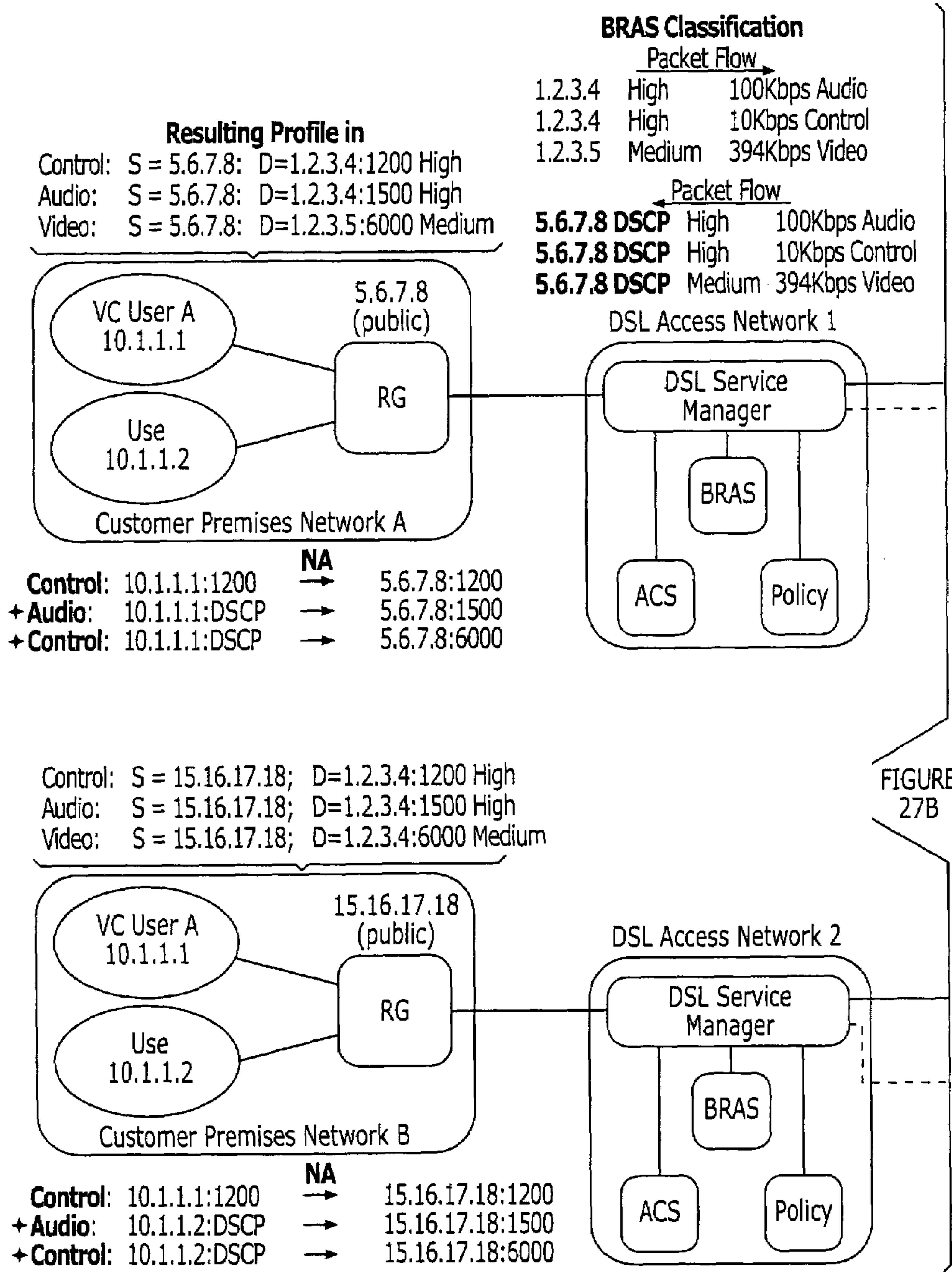
FIGURE 27A
