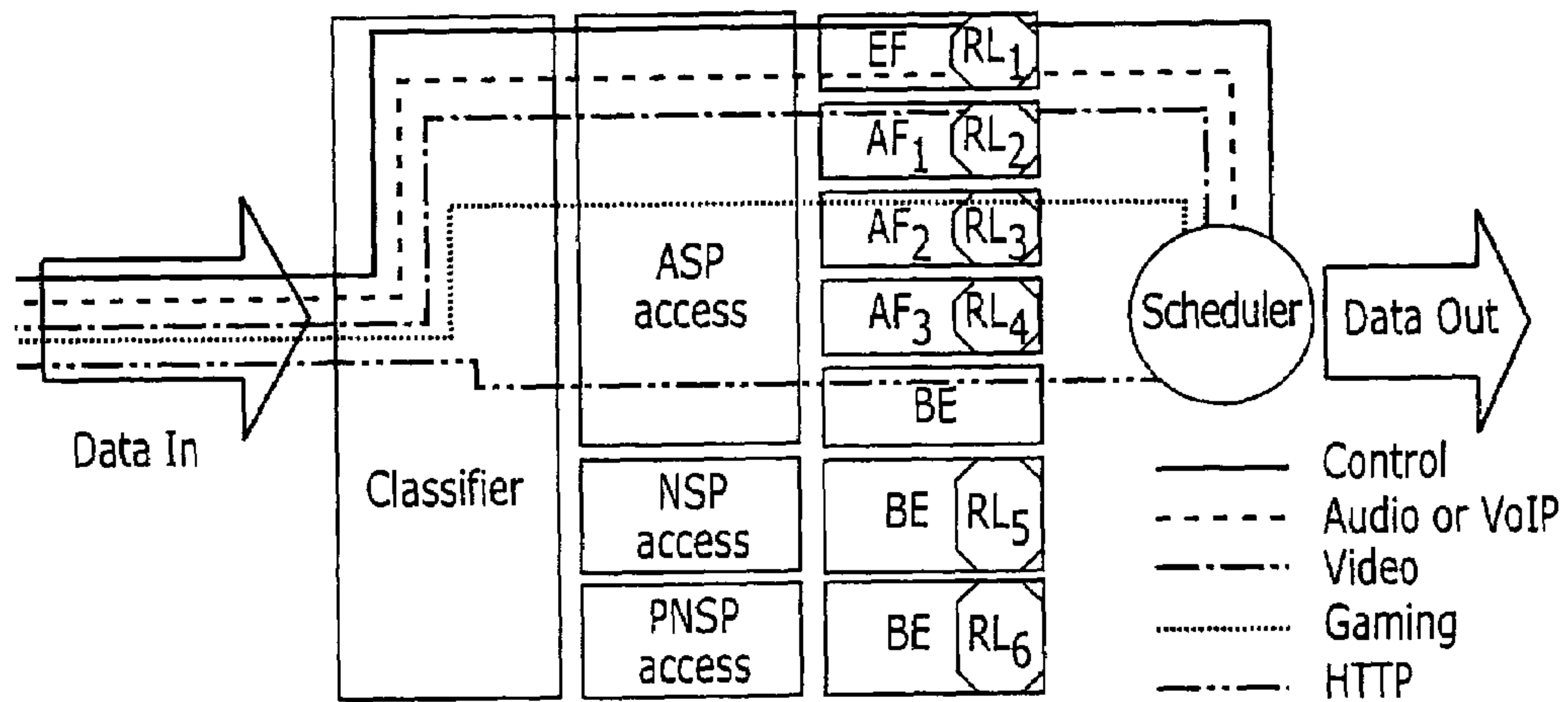
FIGURE 6
