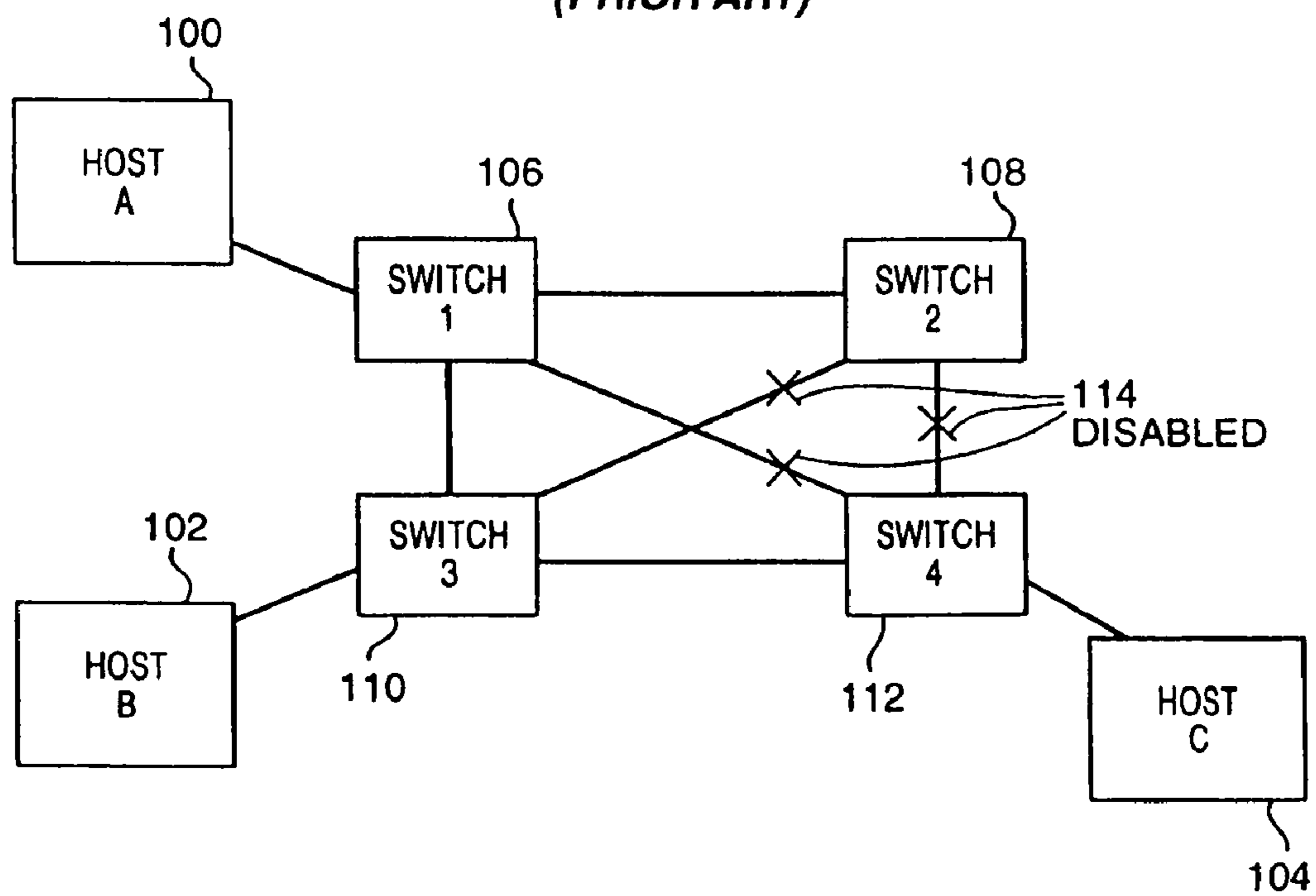
FIG. 2 (PRIOR ART)
