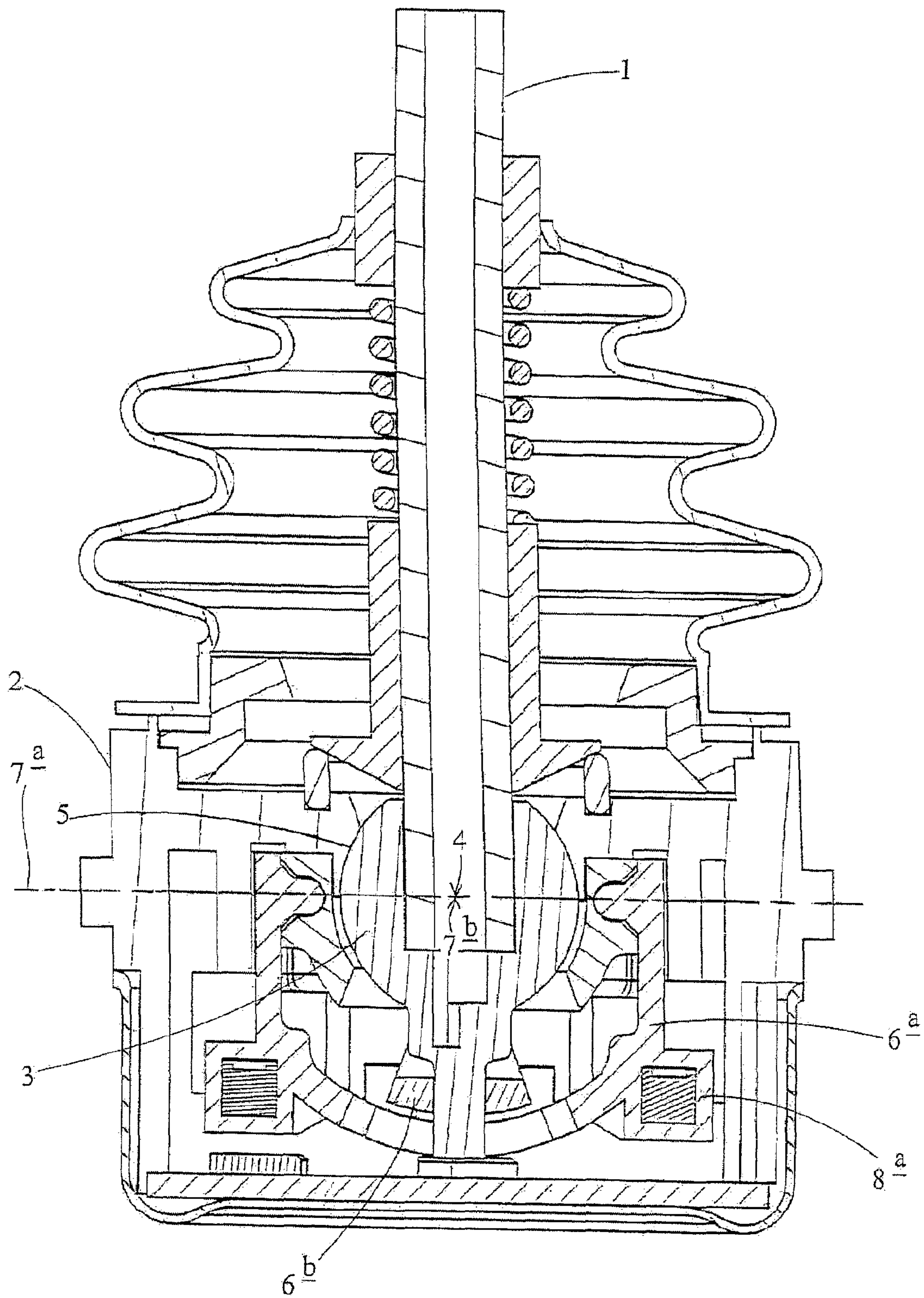
FIG 1 PRIOR ART
