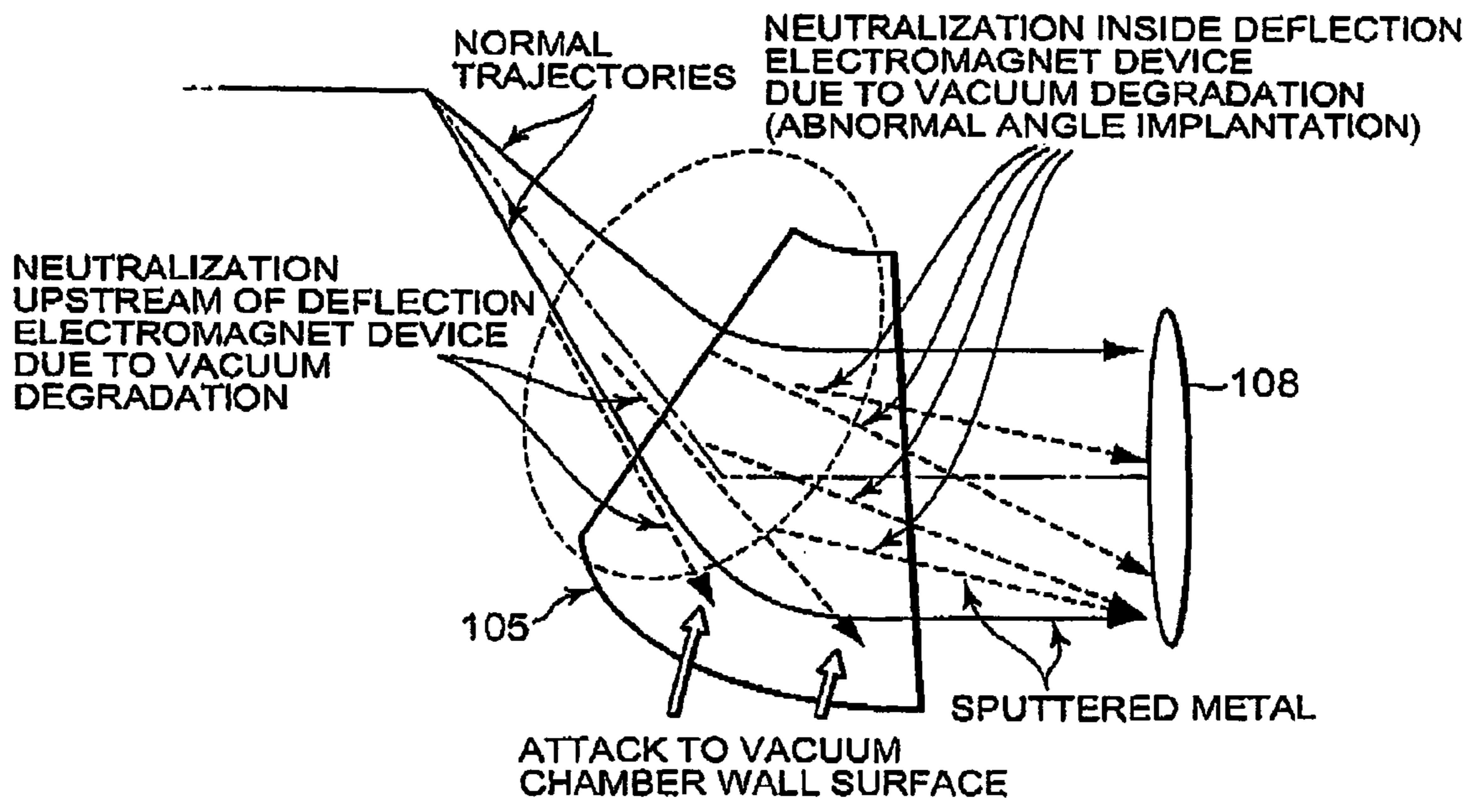
FIG. 2 PRIOR ART
