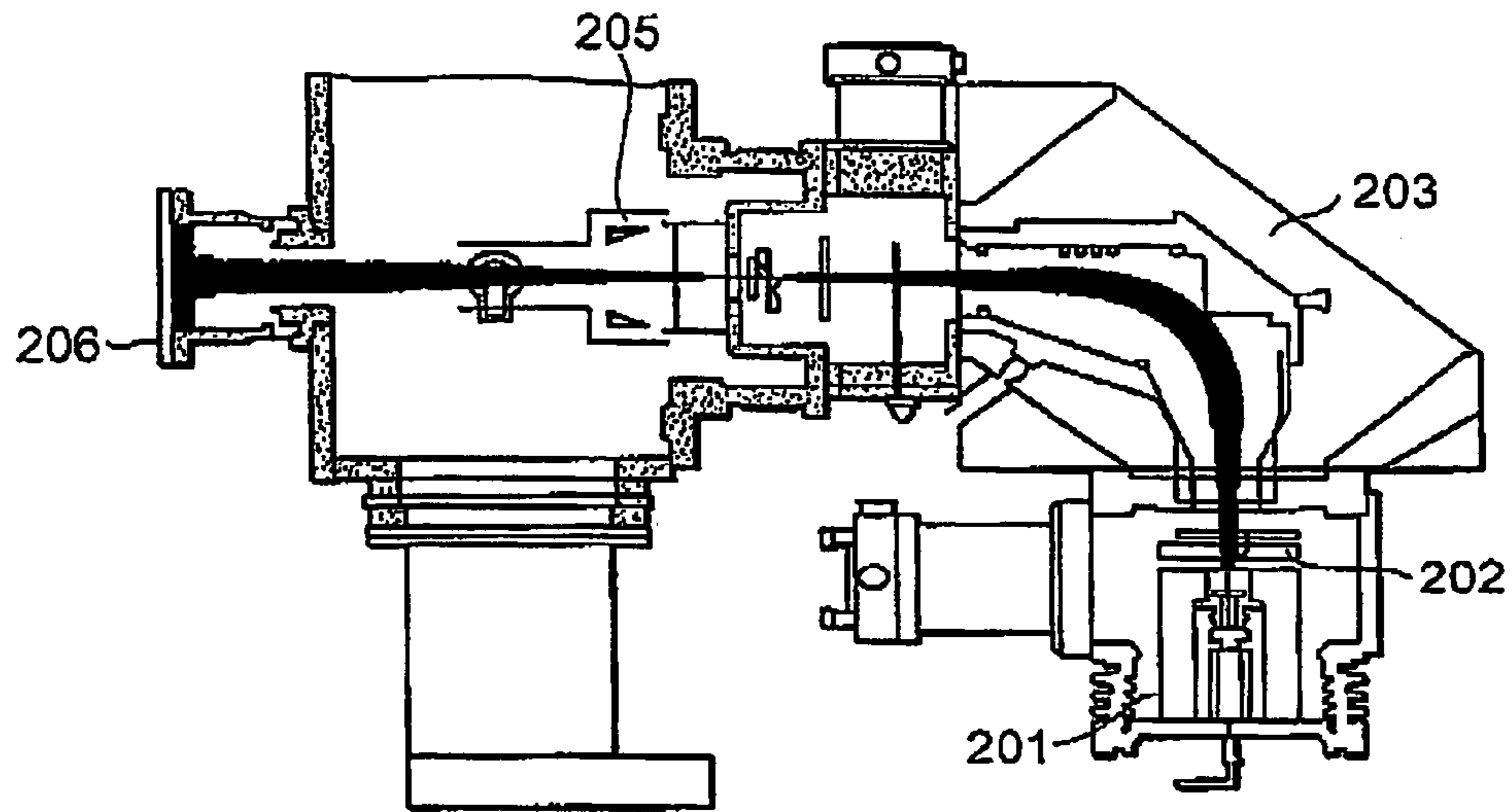
FIG. 3 PRIOR ART
