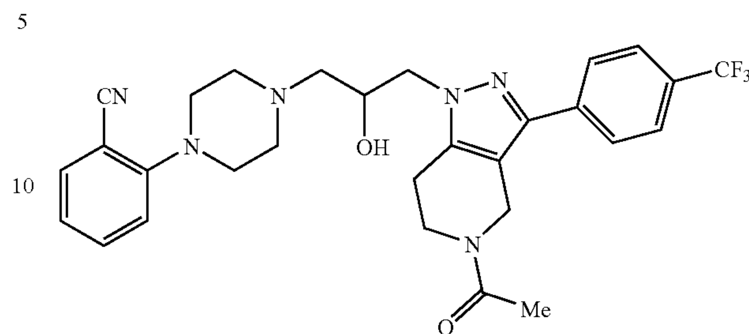
2-(4-{3-[5-Acetyl-3-(4-trifluoromethyl-phenyl)-4,5,6,7-tetrahydro-pyrazolo[4,3-c]pyridin-1-yl]-2-hydroxy-propyl}-piperazin-1-yl)-benzonitrile
