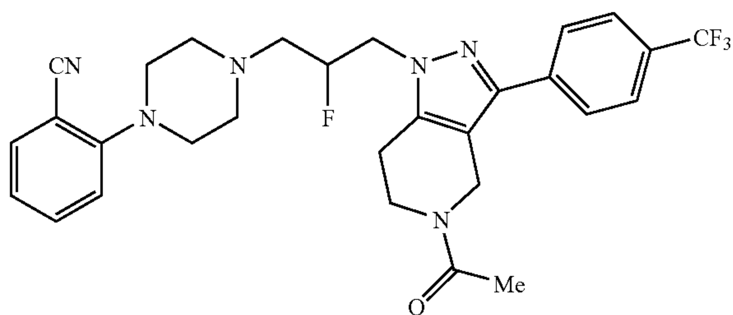
2-(4-{3-[5-Acetyl-3-(4-trifluoromethyl-phenyl)-4,5,6,7-tetrahydro-pyrazolo[4,3-c]pyridin-1-yl]-2-fluoro-propyl}-piperazin-1-yl)-benzonitrile
