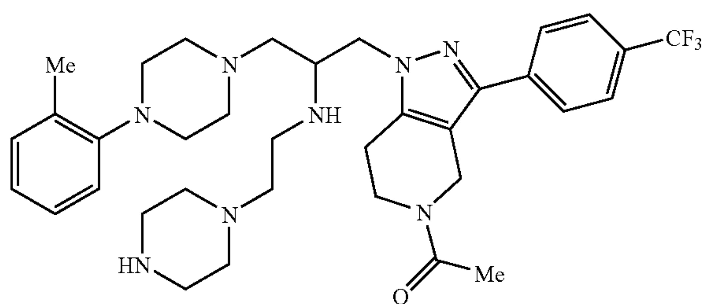
1-[1-[2-(2-piperazin-1-yl-ethylamino)-3-(4-o-tolyl-piperazin-1-yl)-propyl]-3-(4-trifluoromethyl-phenyl)-1,4,6,7-tetrahydro-pyrazolo[4,3-c]pyridin-5-yl]-ethanone
