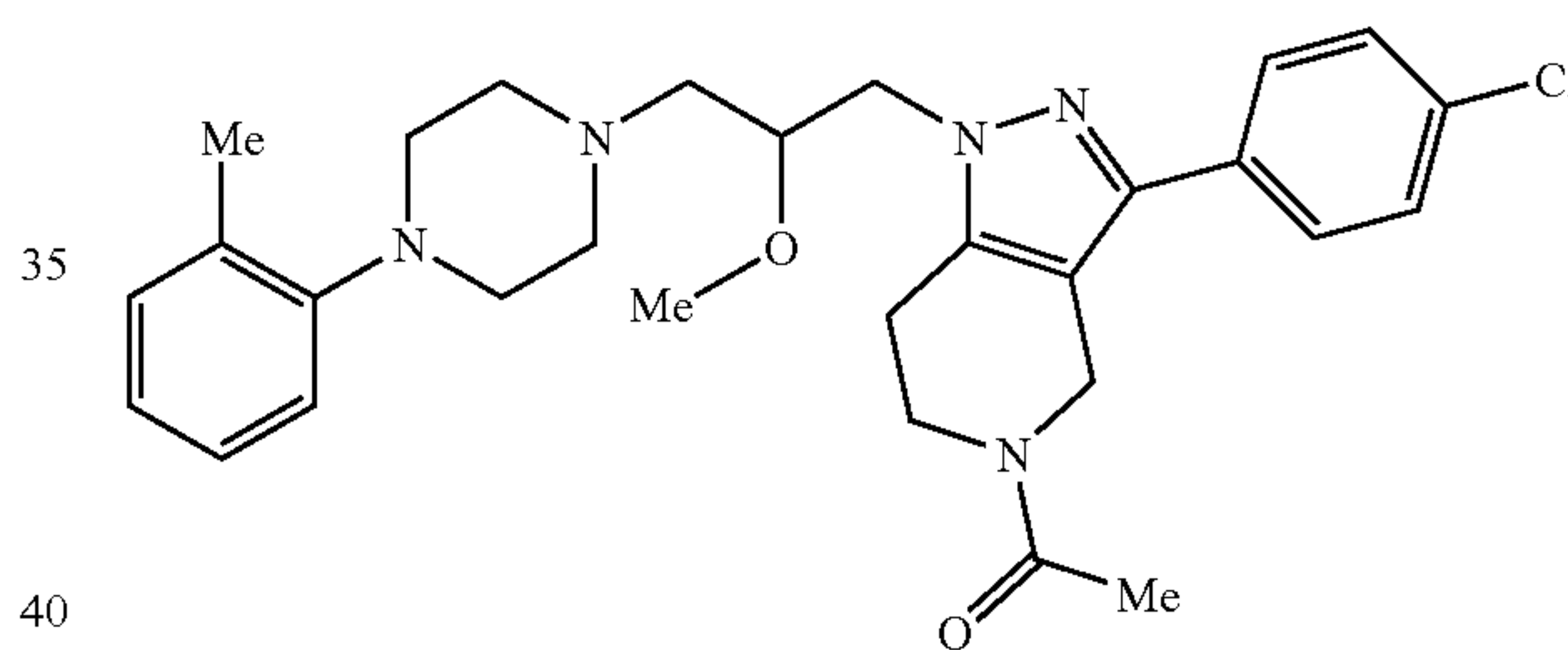
1-[3-(4-Chloro-phenyl)-1-[2-hydroxy-3-(4-o-tolyl-piperazin-1-yl)-propyl]-1,4,6,7-tetrahydro-pyrazolo[4,3-c]pyridin-5-yl]-ethanone
