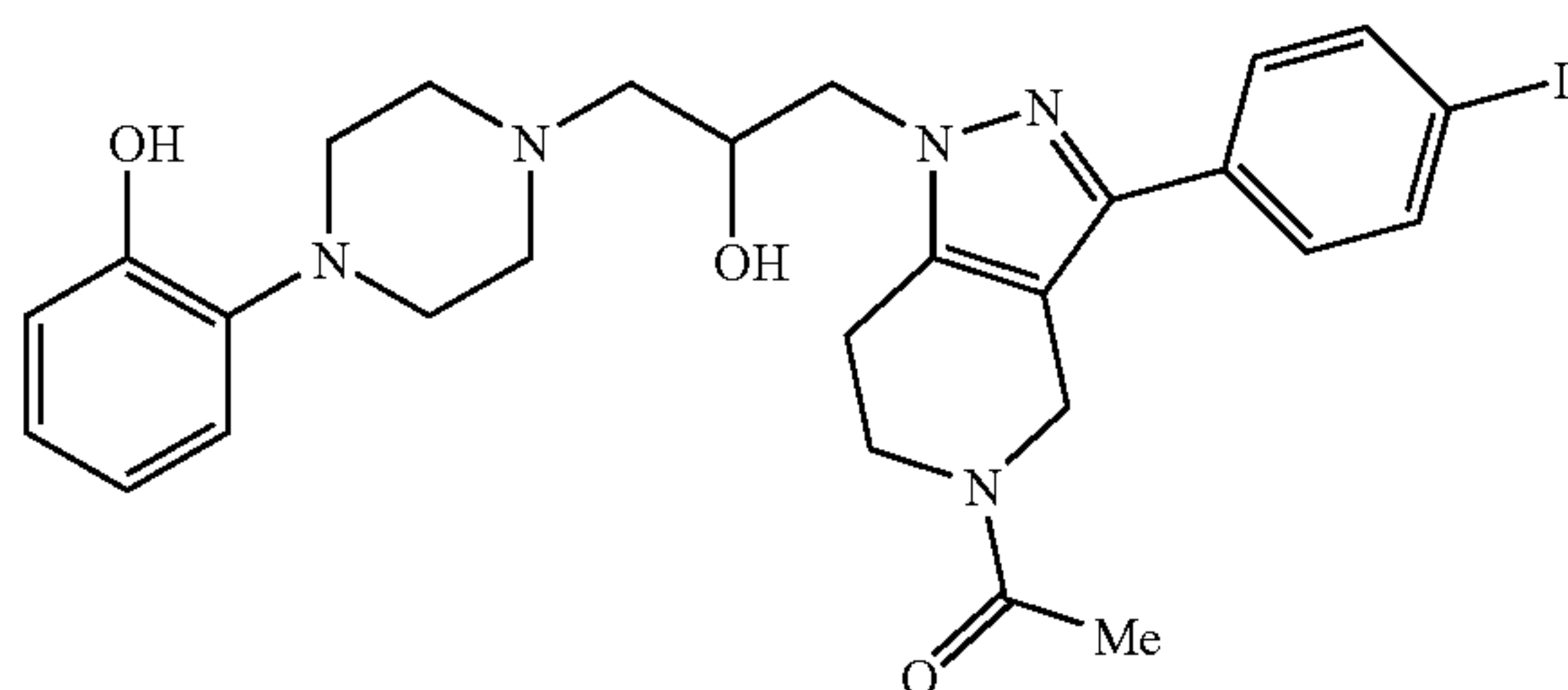
1-[1-{2-Hydroxy-3-[4-(2-hydroxy-phenyl)-piperazin-1-yl]-propyl}-3-(4-iodo-phenyl)-1,4,6,7-tetrahydro-pyrazolo[4,3-c]pyridin-5-yl]-ethanone
