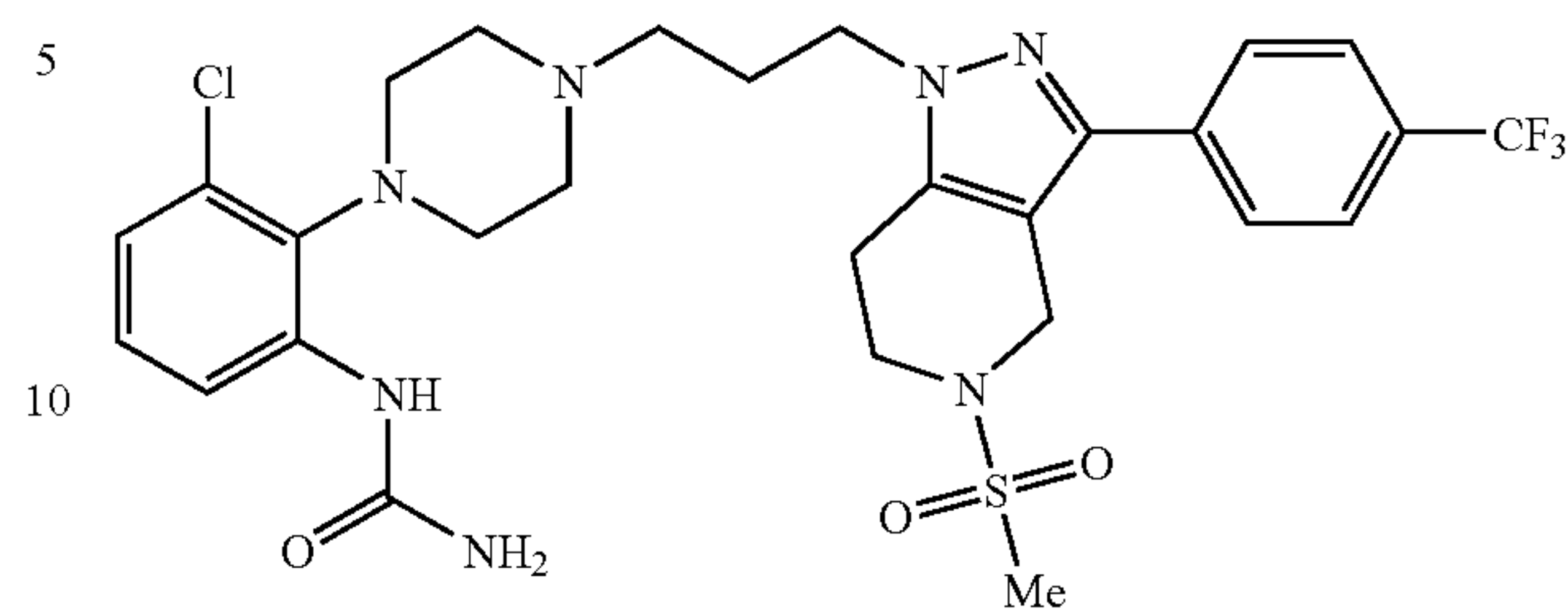
1-[3-Chloro-2-(4-{3-[5-methanesulfonyl-3-(4-trifluoromethyl-phenyl)-4,5,6,7-tetrahydro-pyrazolo[4,3-c]pyridin-1-yl]-propyl}-piperazin-1-yl)-phenyl]-3-methyl-urea
