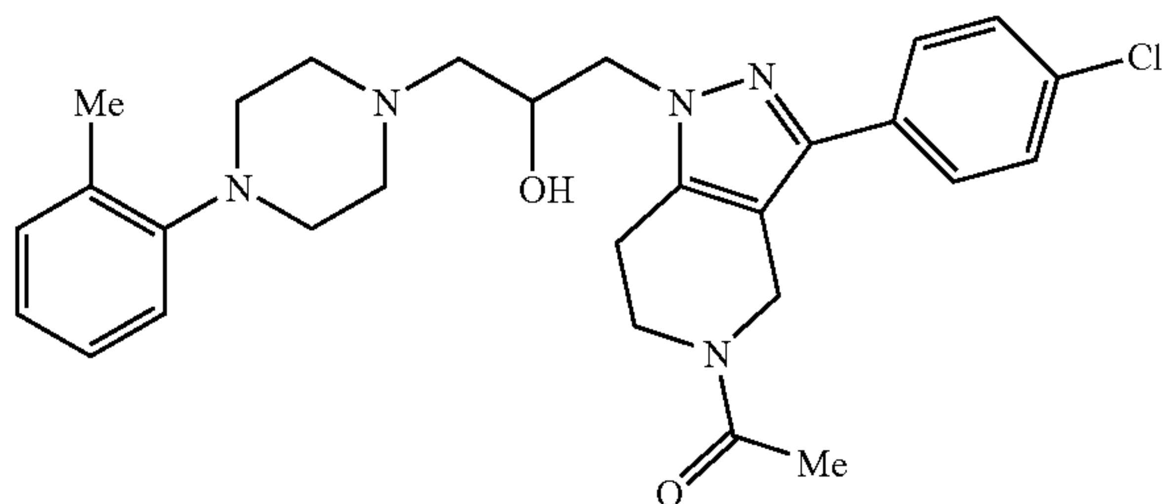
1-[3-(4-Chloro-phenyl)-1-[2-hydroxy-3-(4-o-tolyl-piperazin-1-yl)-propyl]-1,4,6,7-tetrahydro-pyrazolo[4,3-c]pyridin-5-yl]-ethanone
