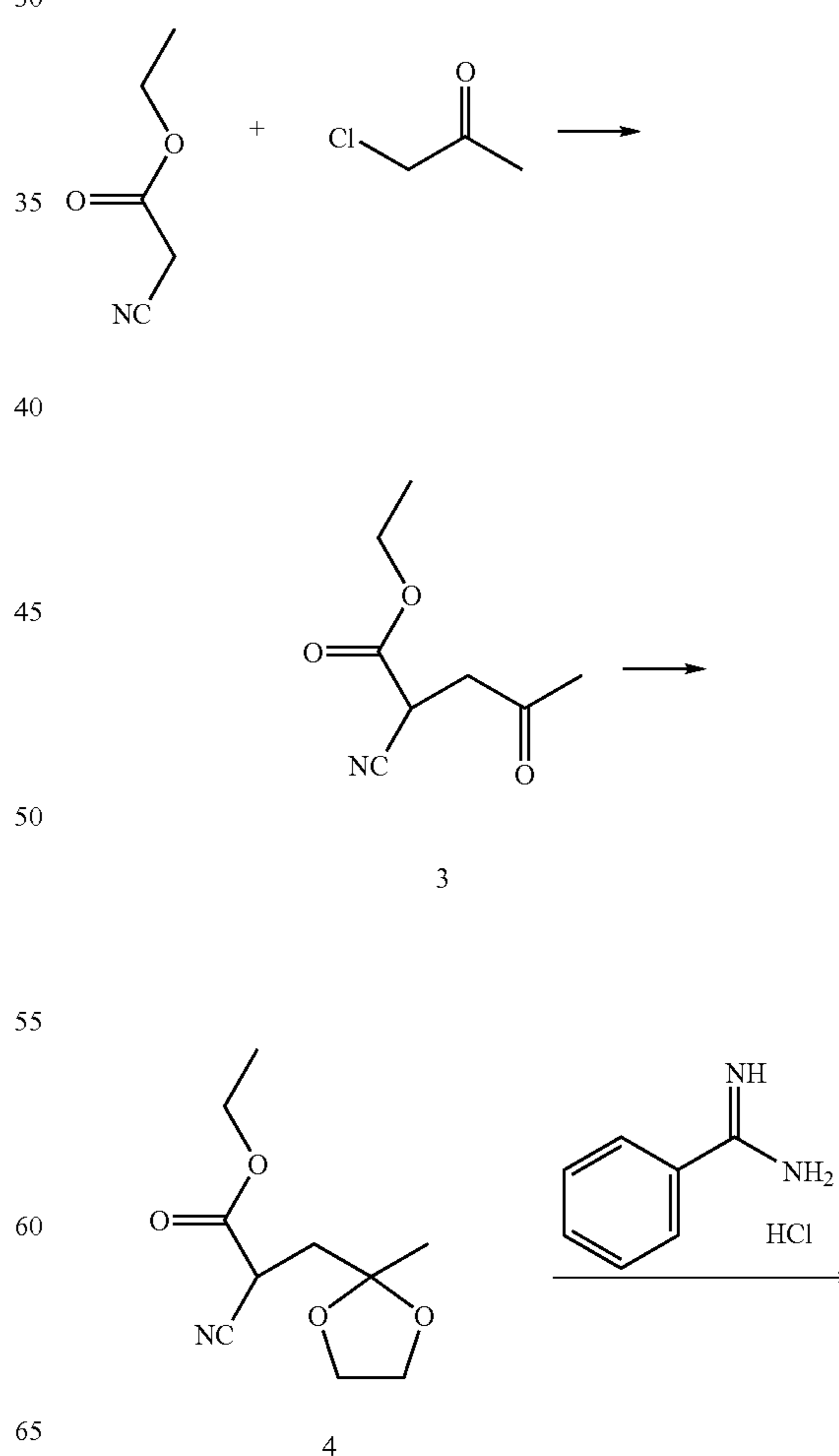
Scheme IV
