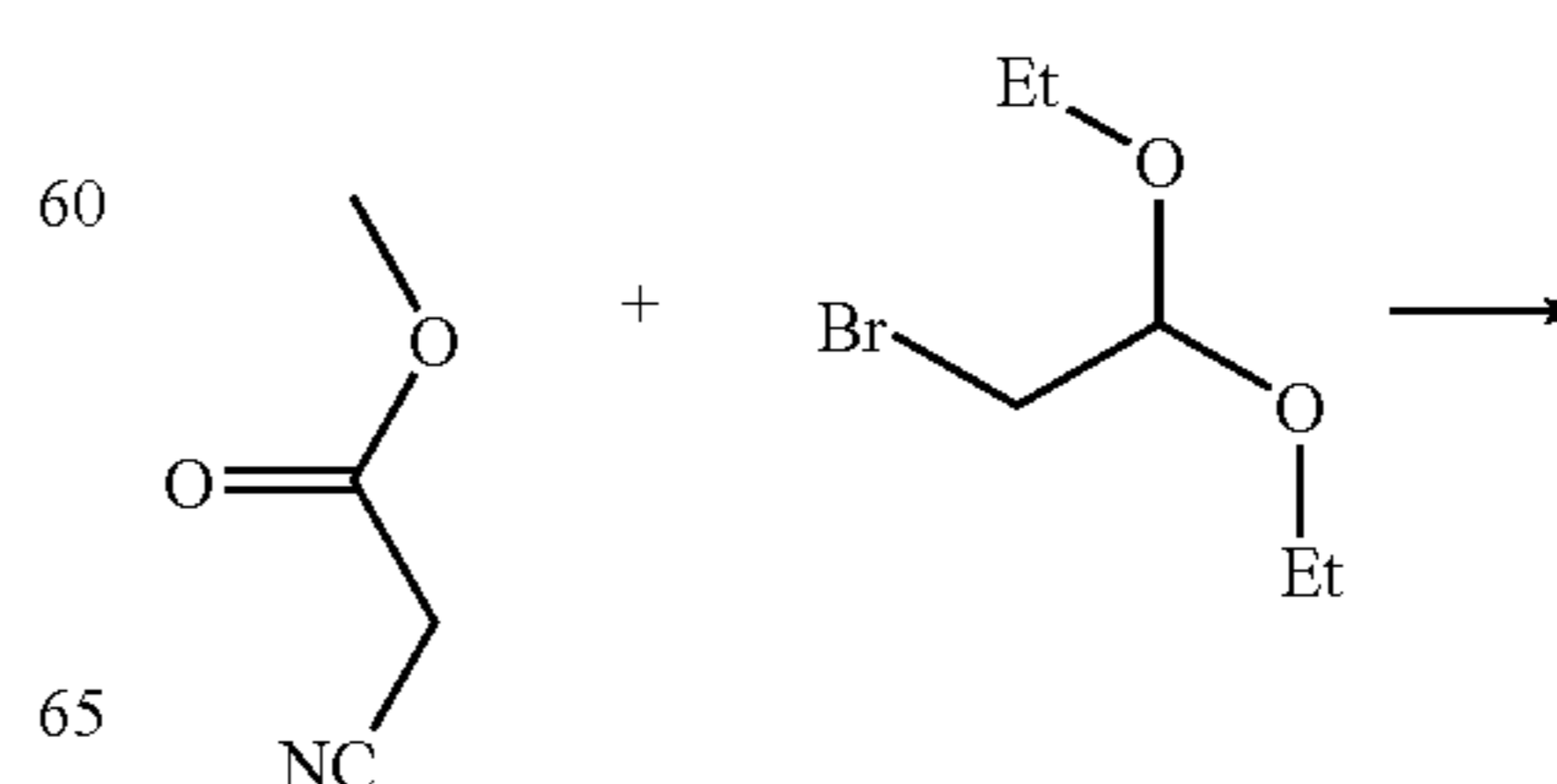
Scheme VII
