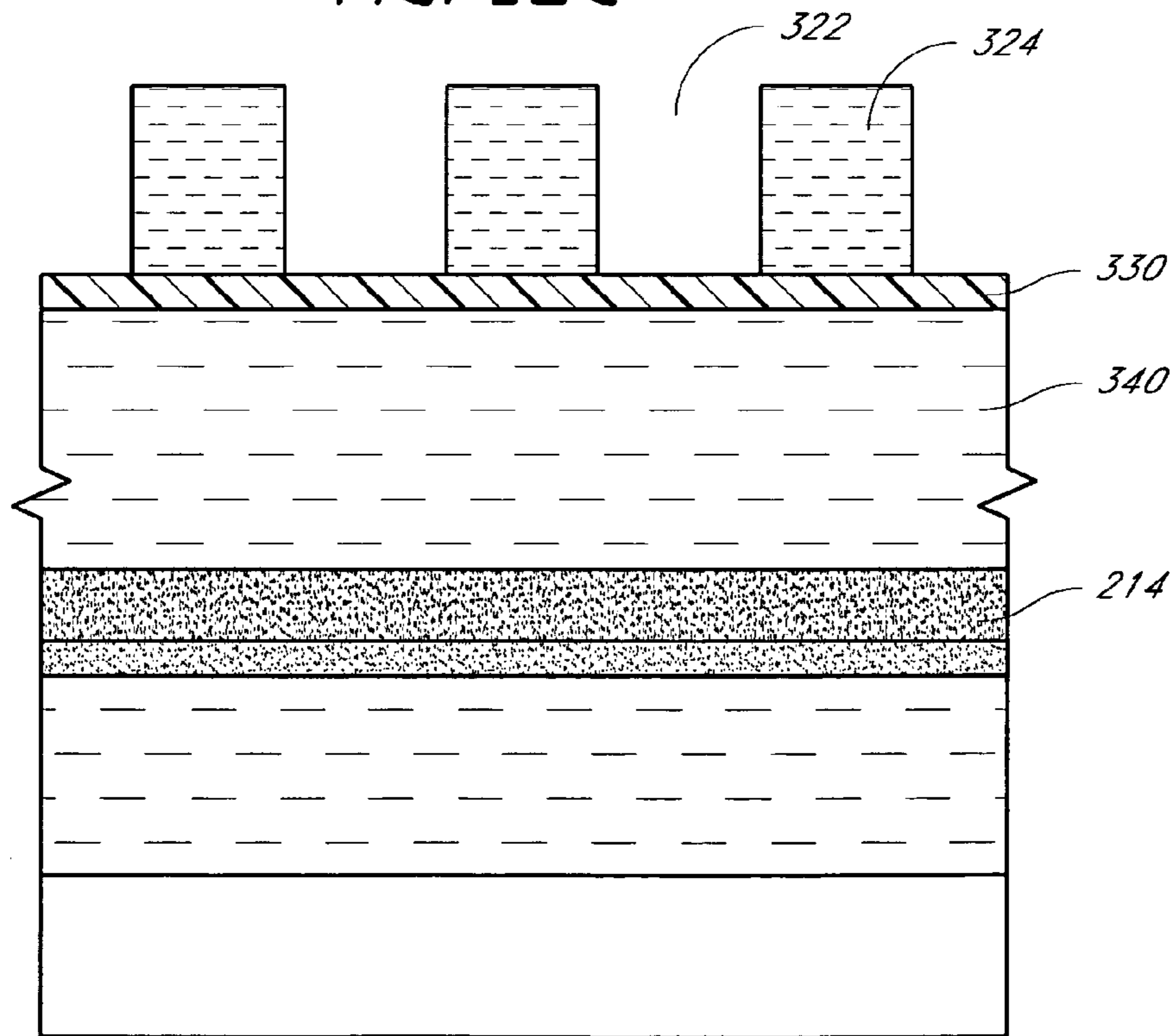
FIG. 12D
