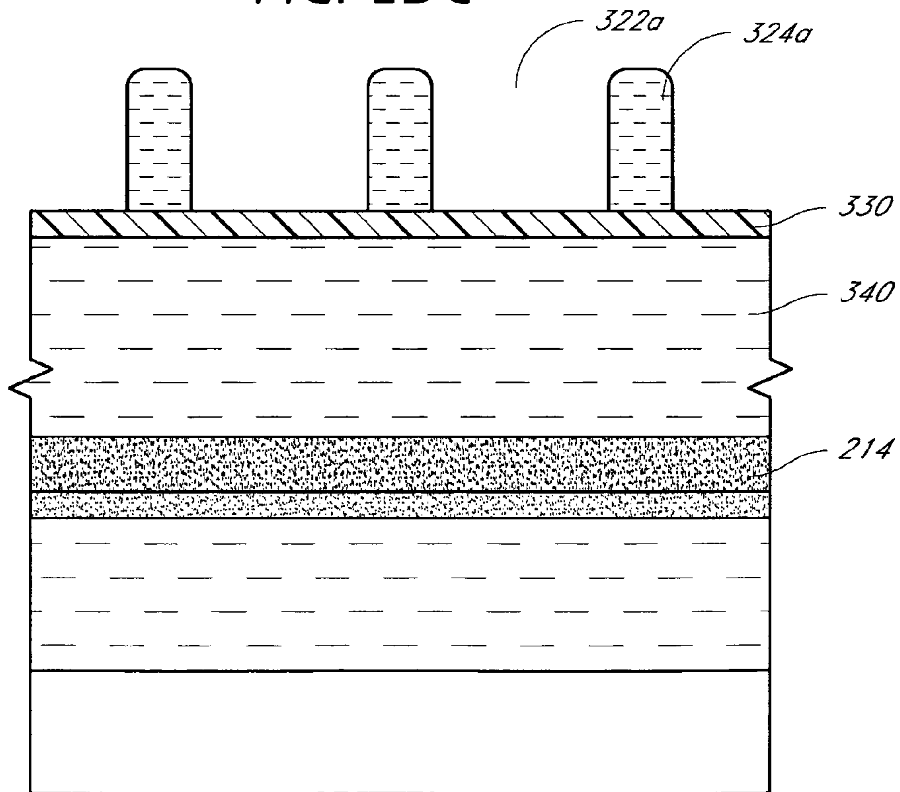
FIG. 13D
