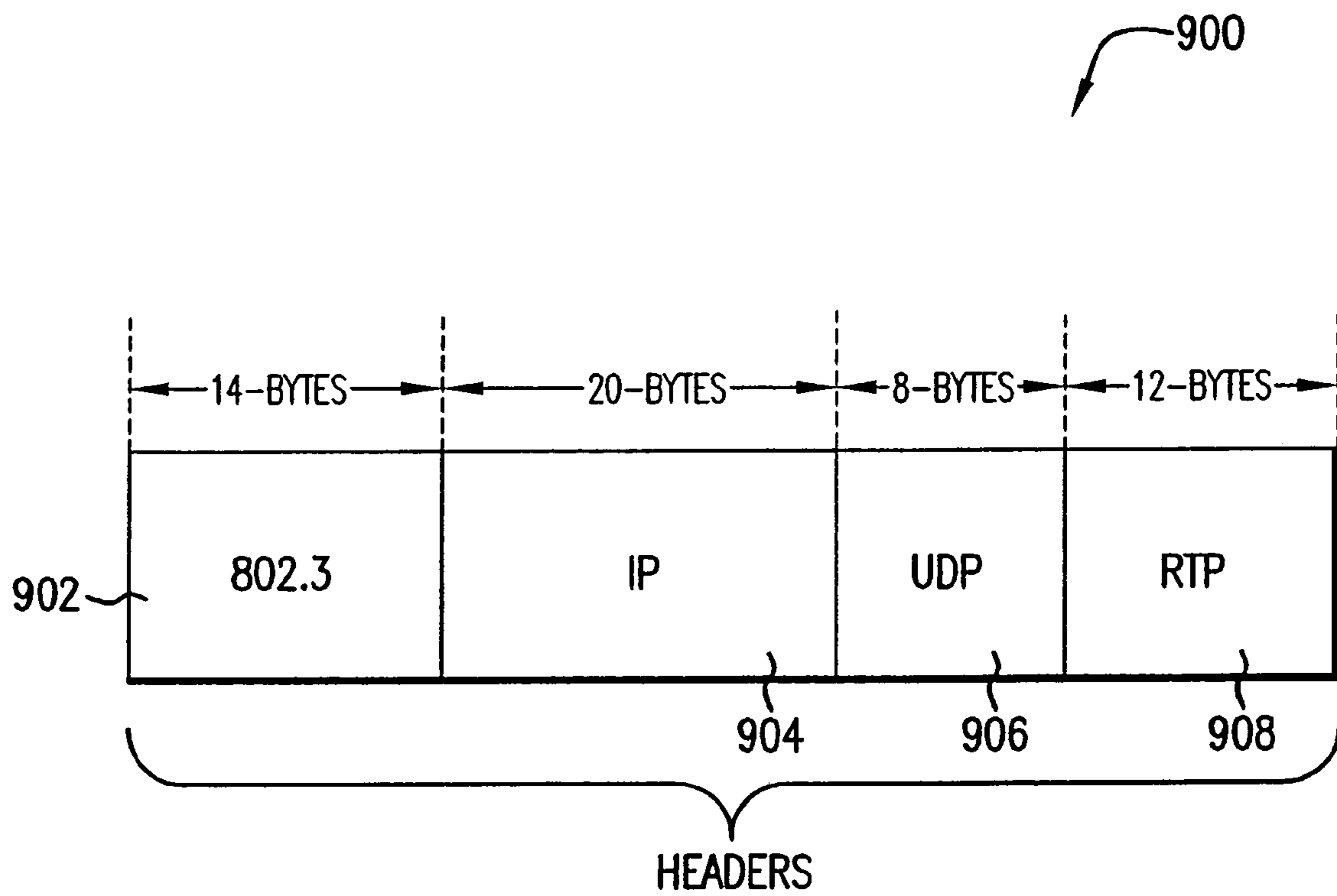
FIG.9A
