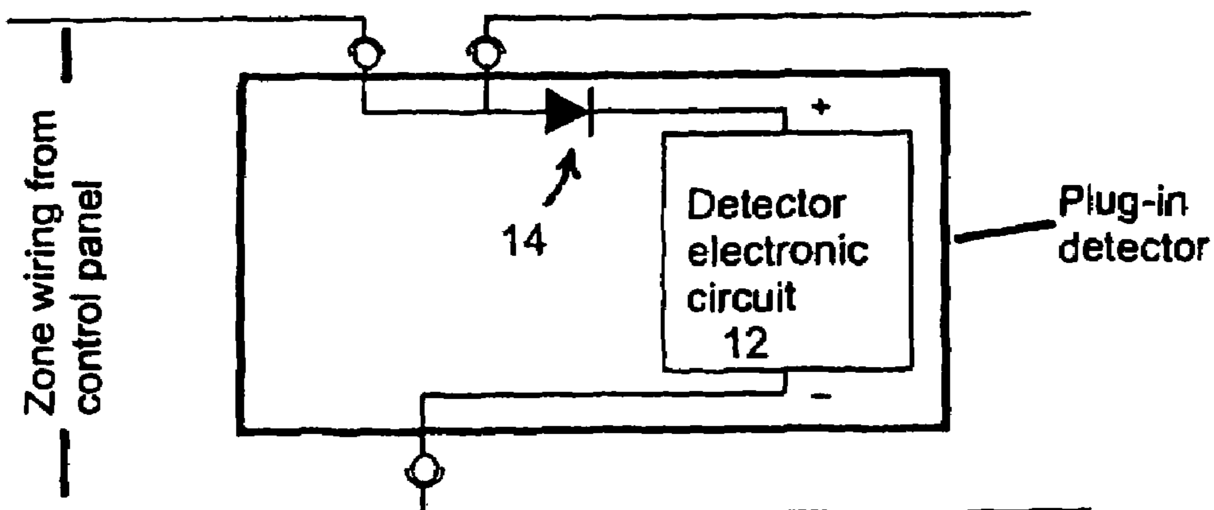
Fig 3 Polarity protection using series diode
