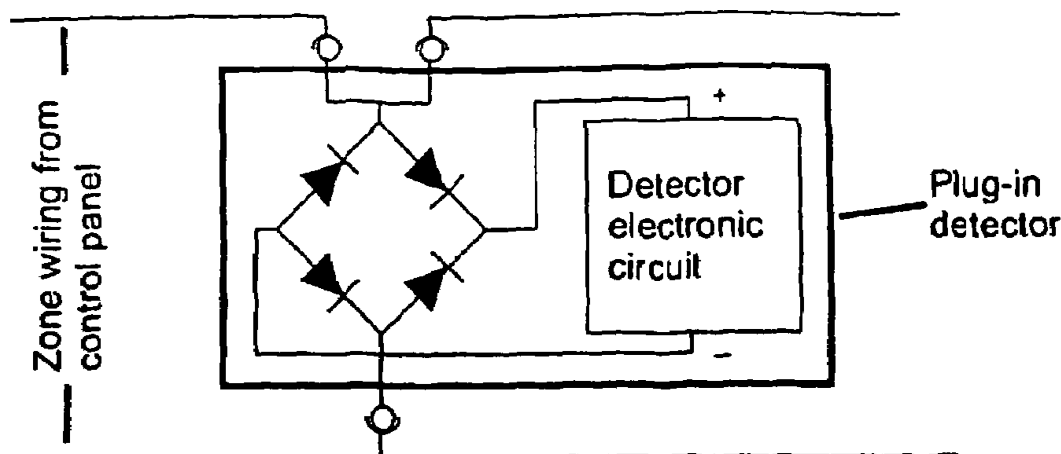
Polarity protection using diode bridge
