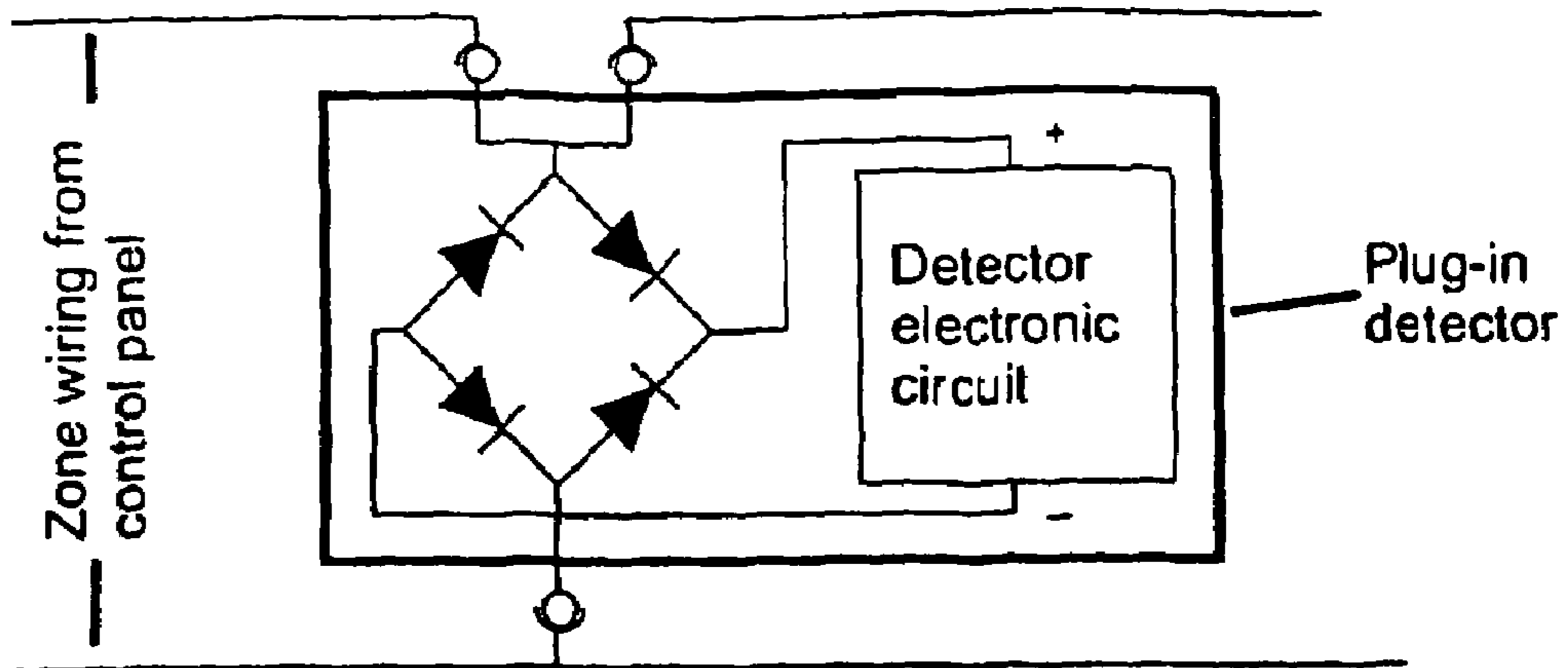
Fig 1 Polarity protection using diode bridge
