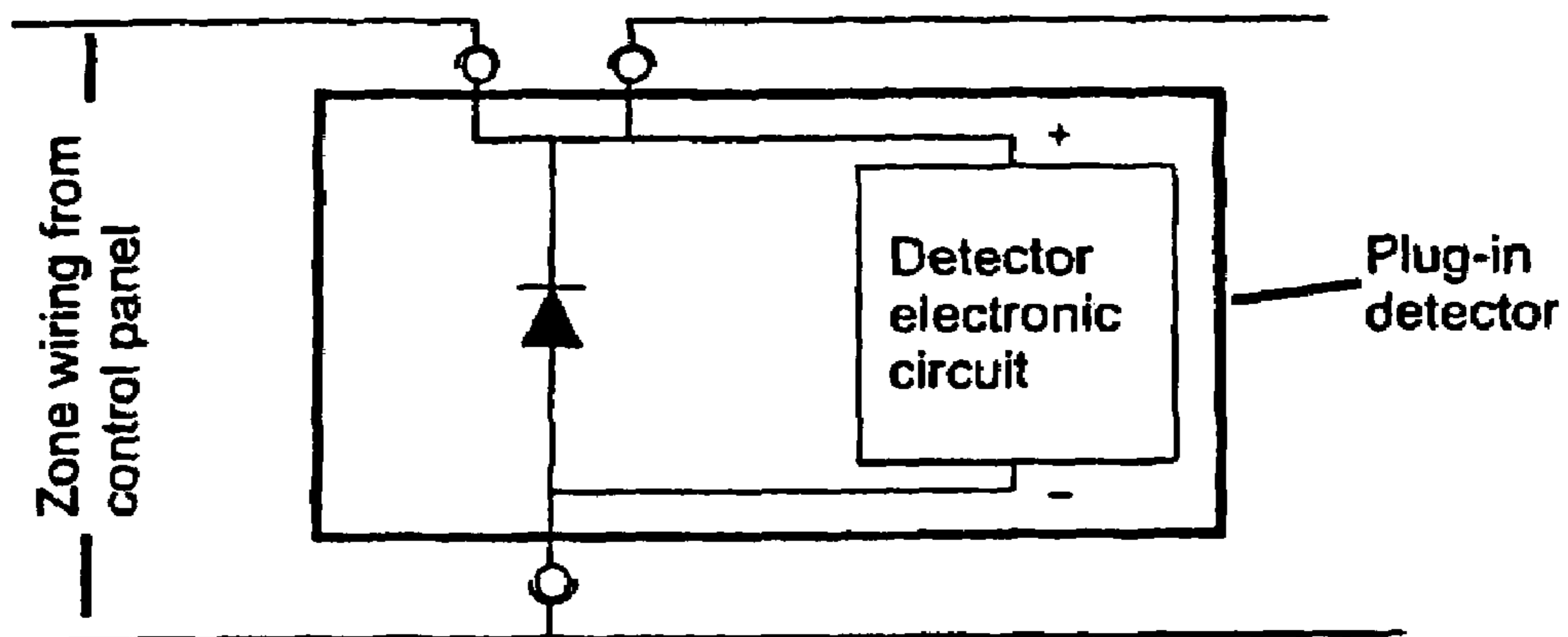
Fig 2 Polarity protection using shunt diode
