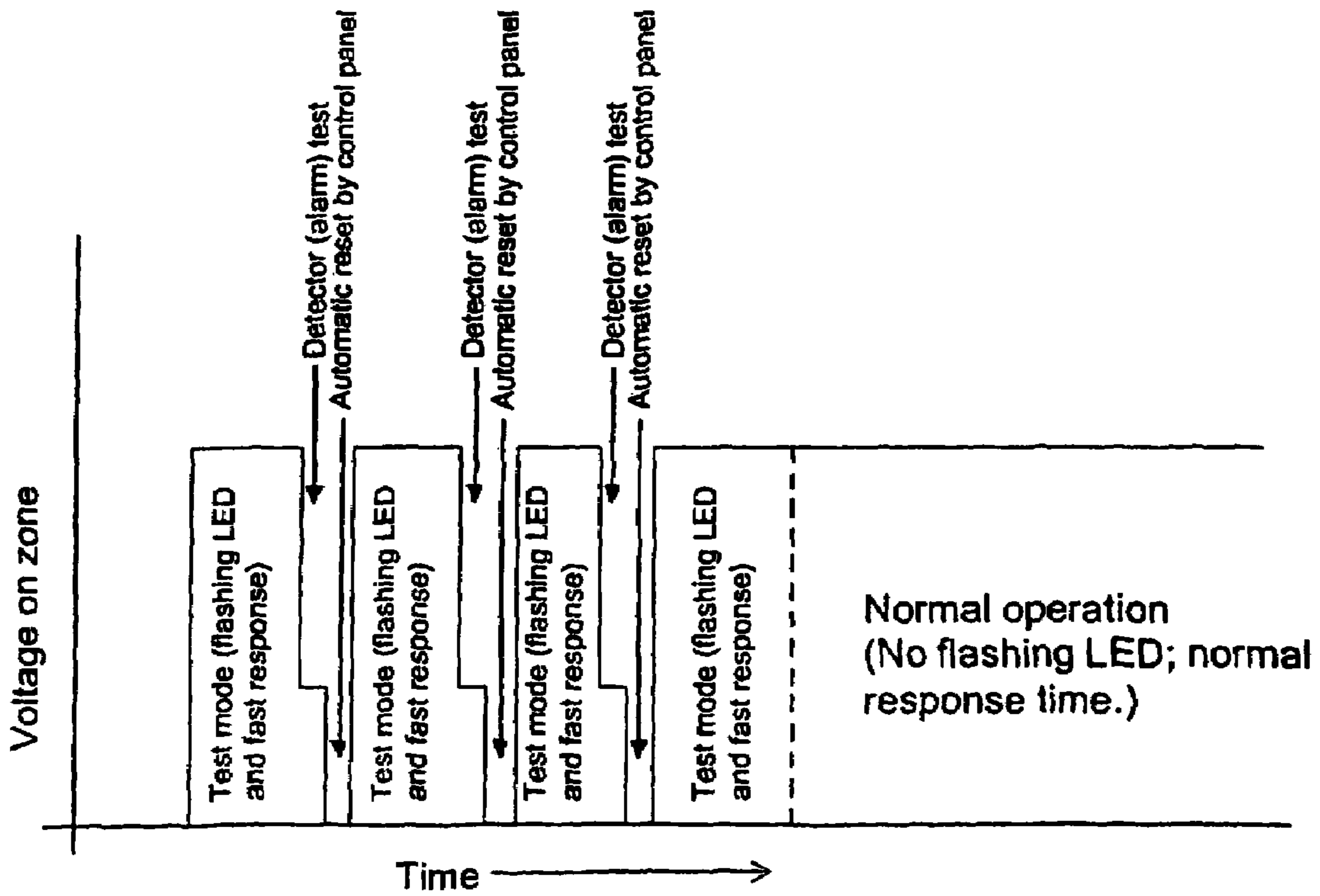
Fig 5 Special test mode on power-up
