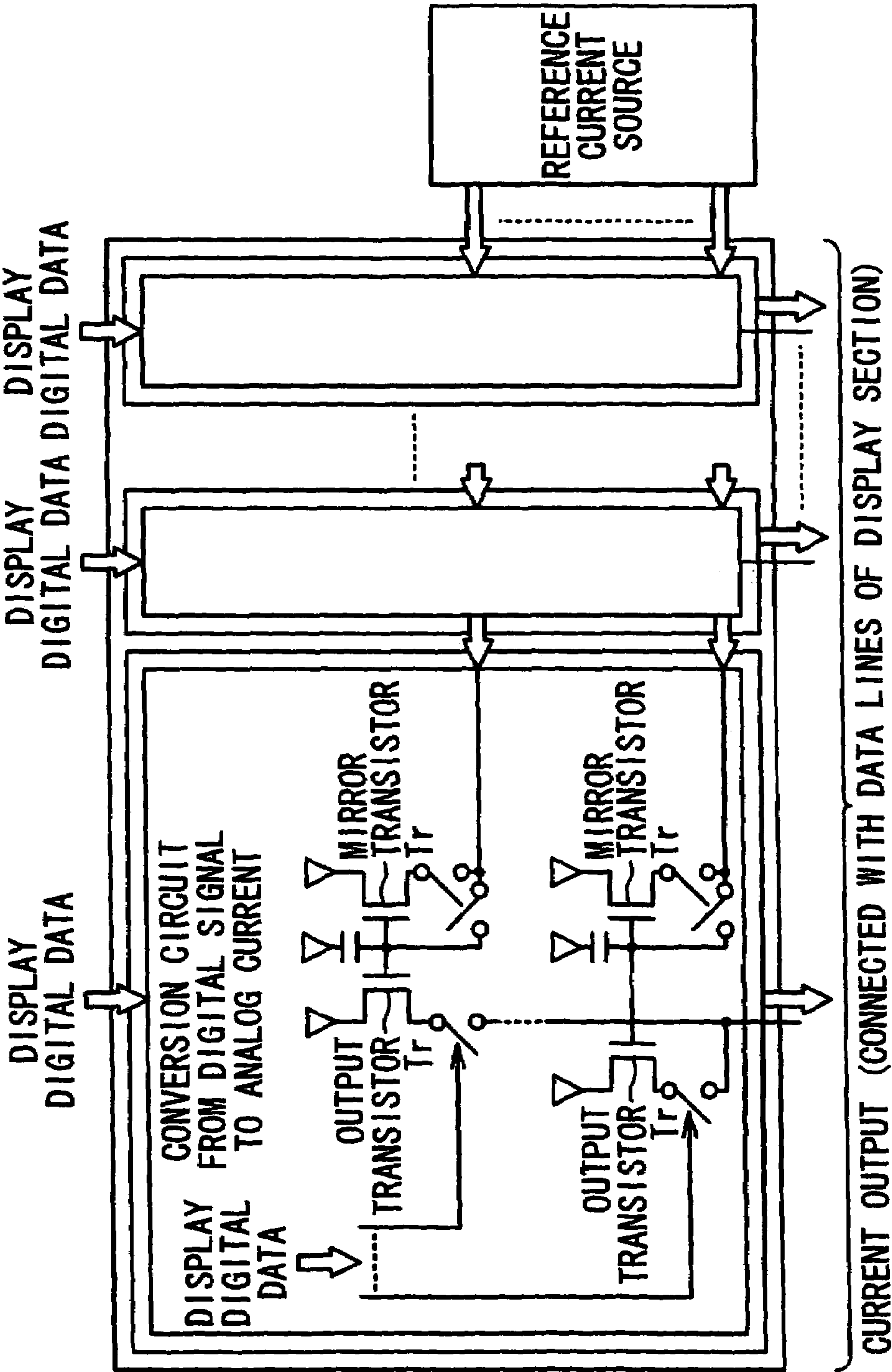
Fig. 5 (RELATED ART)
