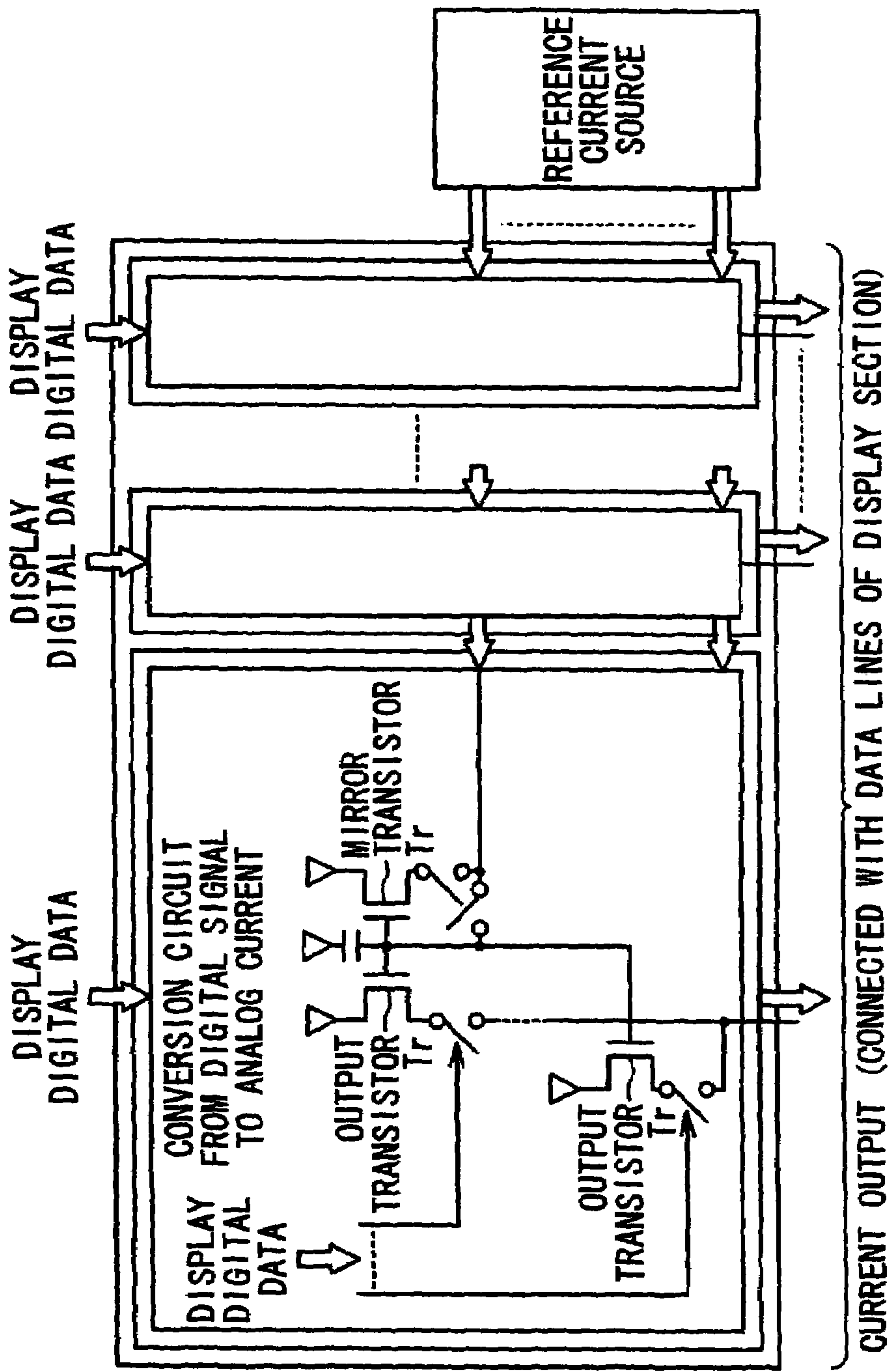
Fig. 4 (RELATED ART)
