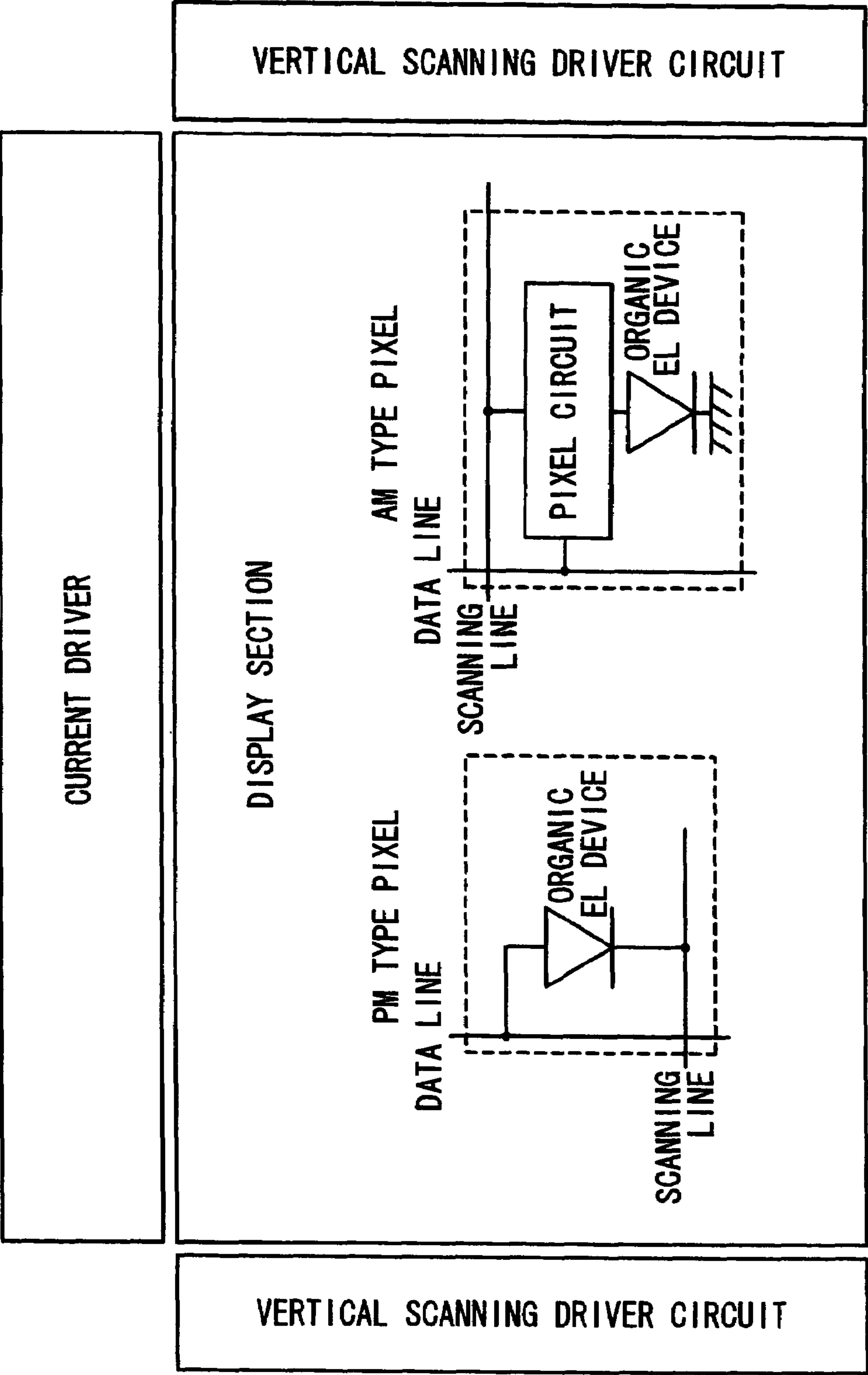
Fig. 1 (RELATED ART)
