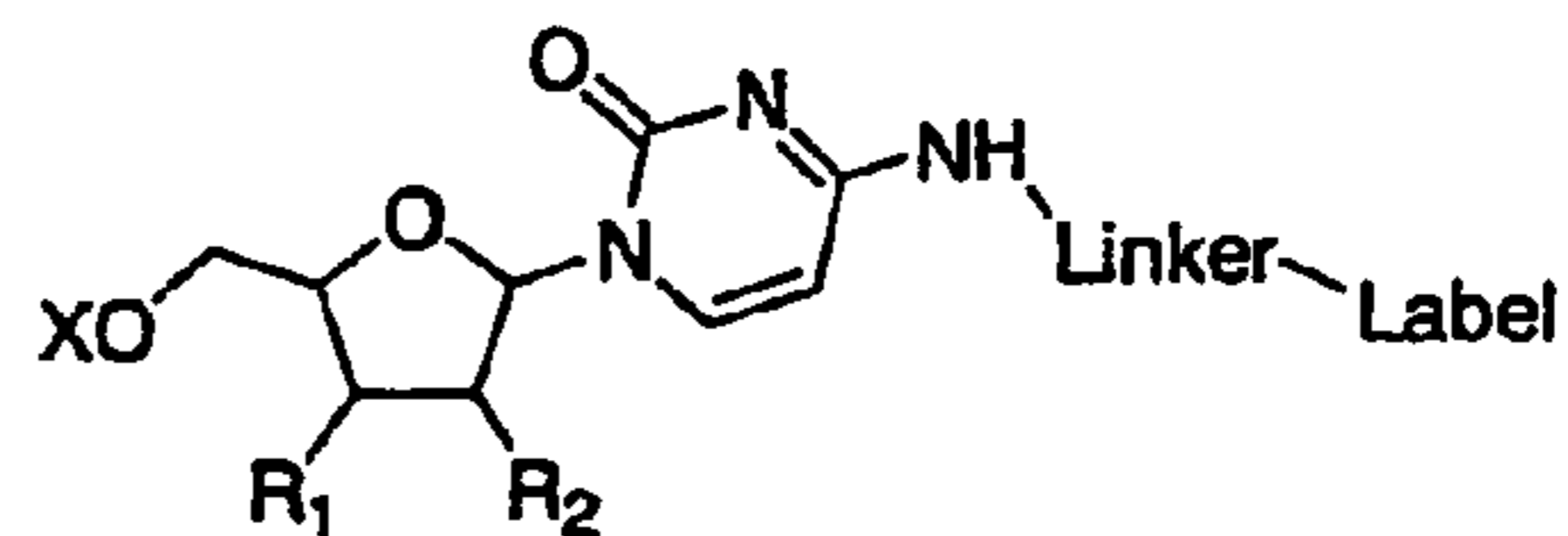
Cytidine N4-linker
