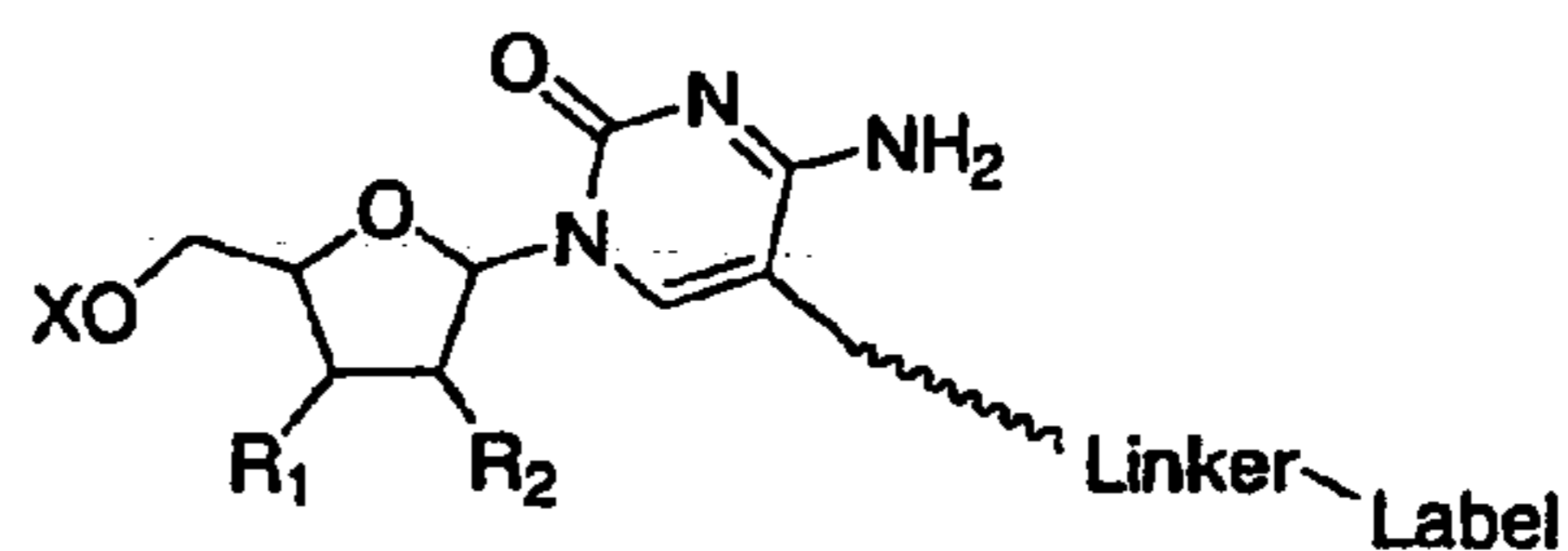
Cytidine C5-linker
