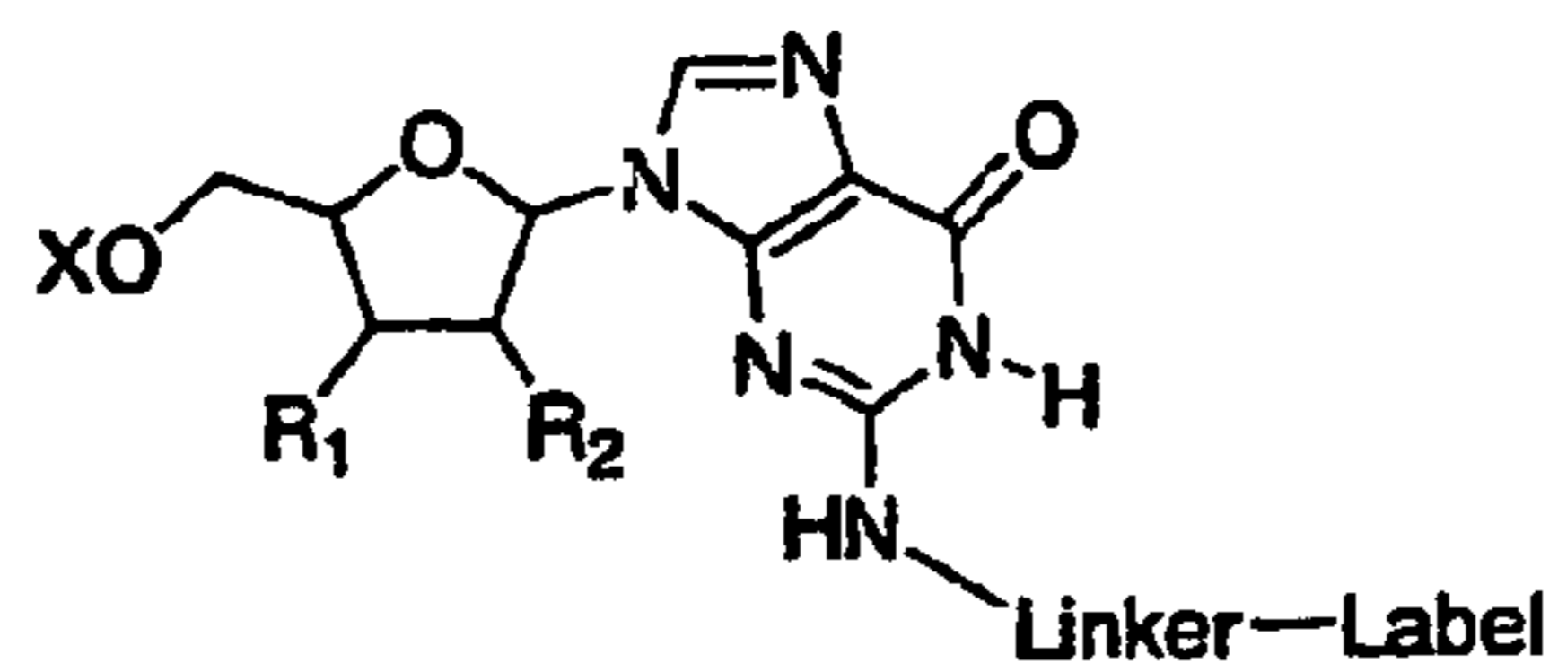
Guanosine N2-linker
