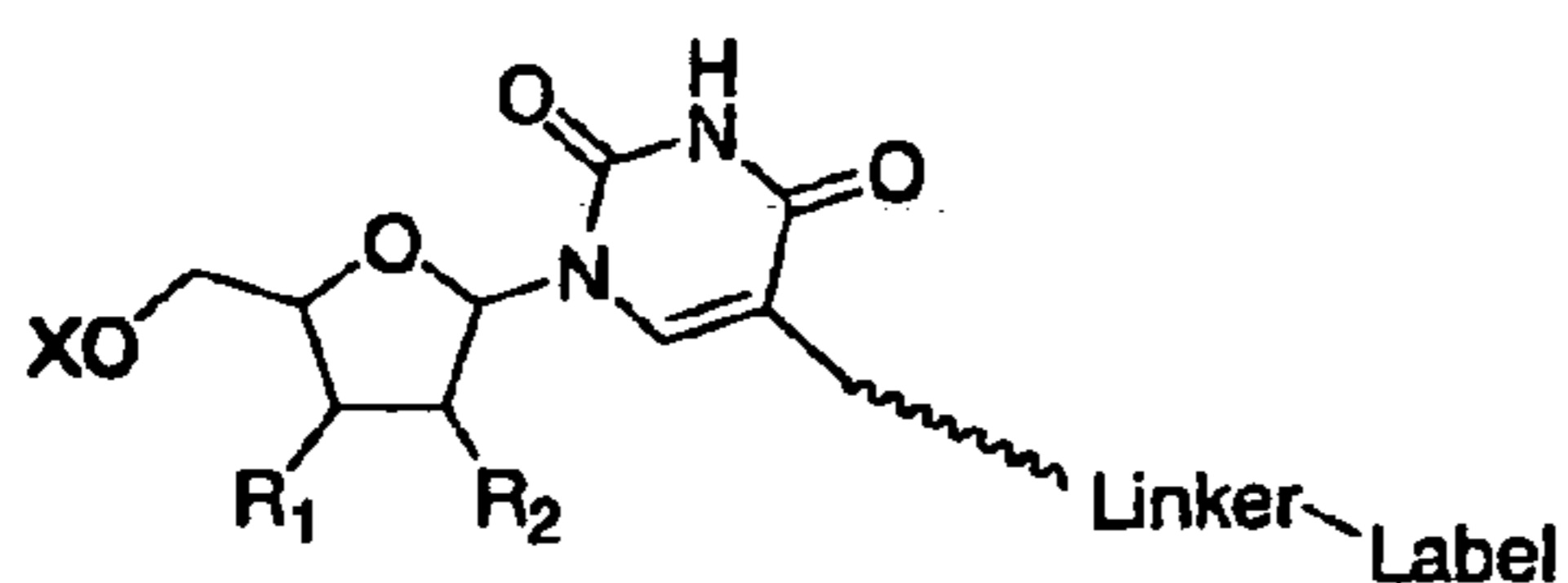
Uridine C5-linker
