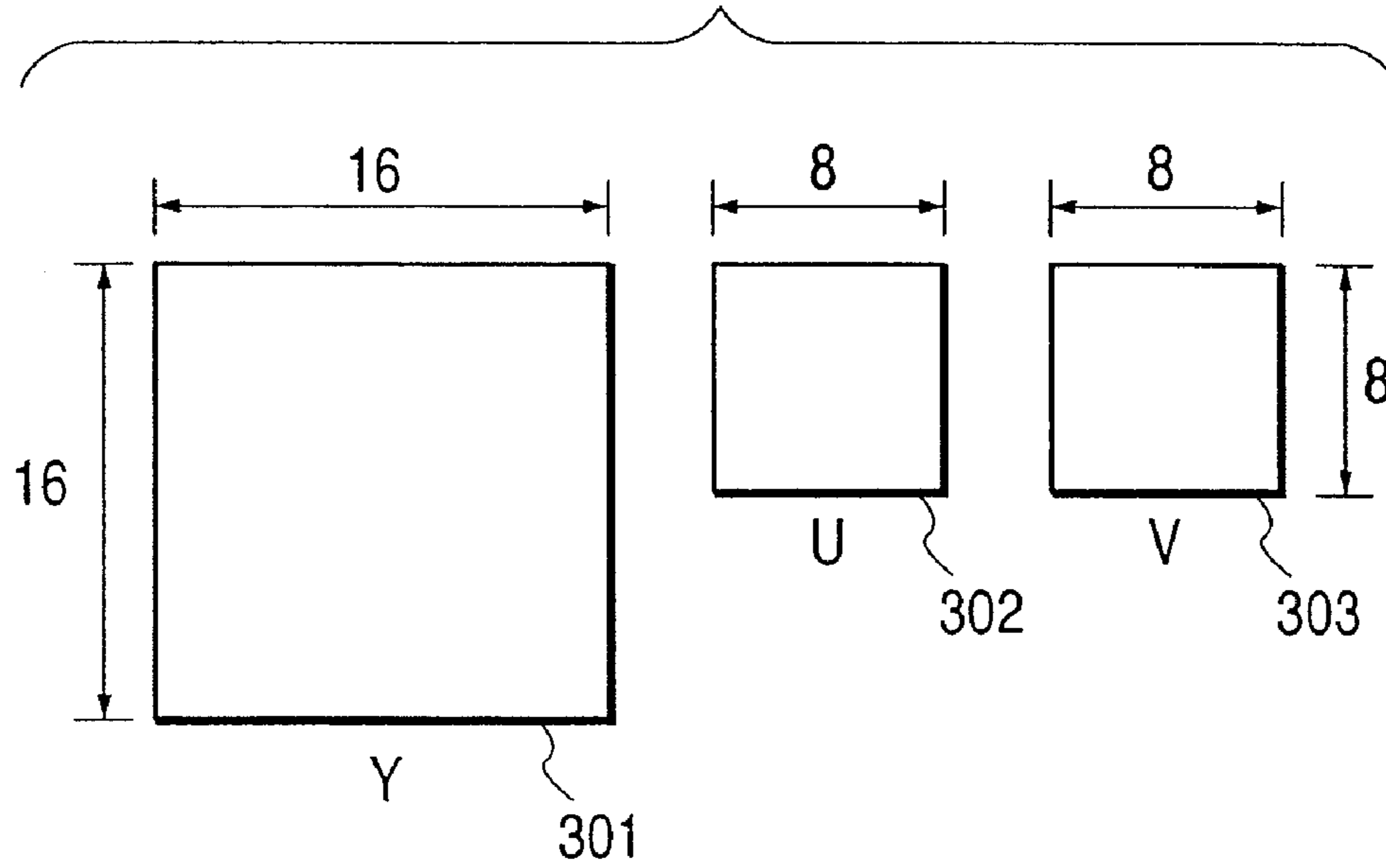
FIG. 3 (PRIOR ART)
