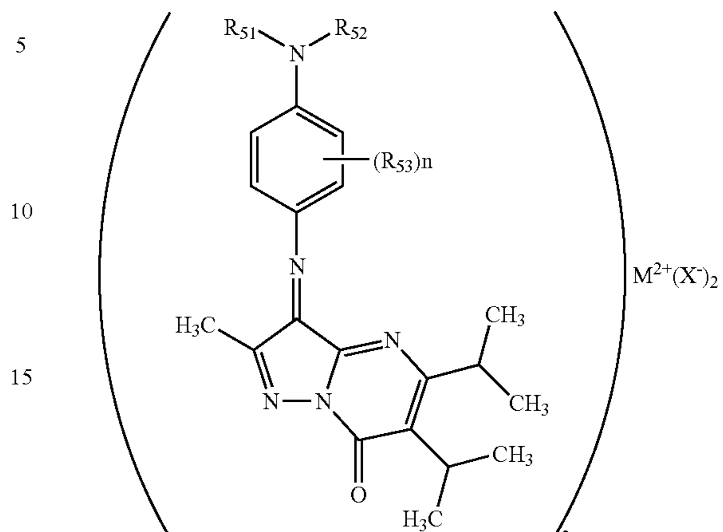
General formula (6)
