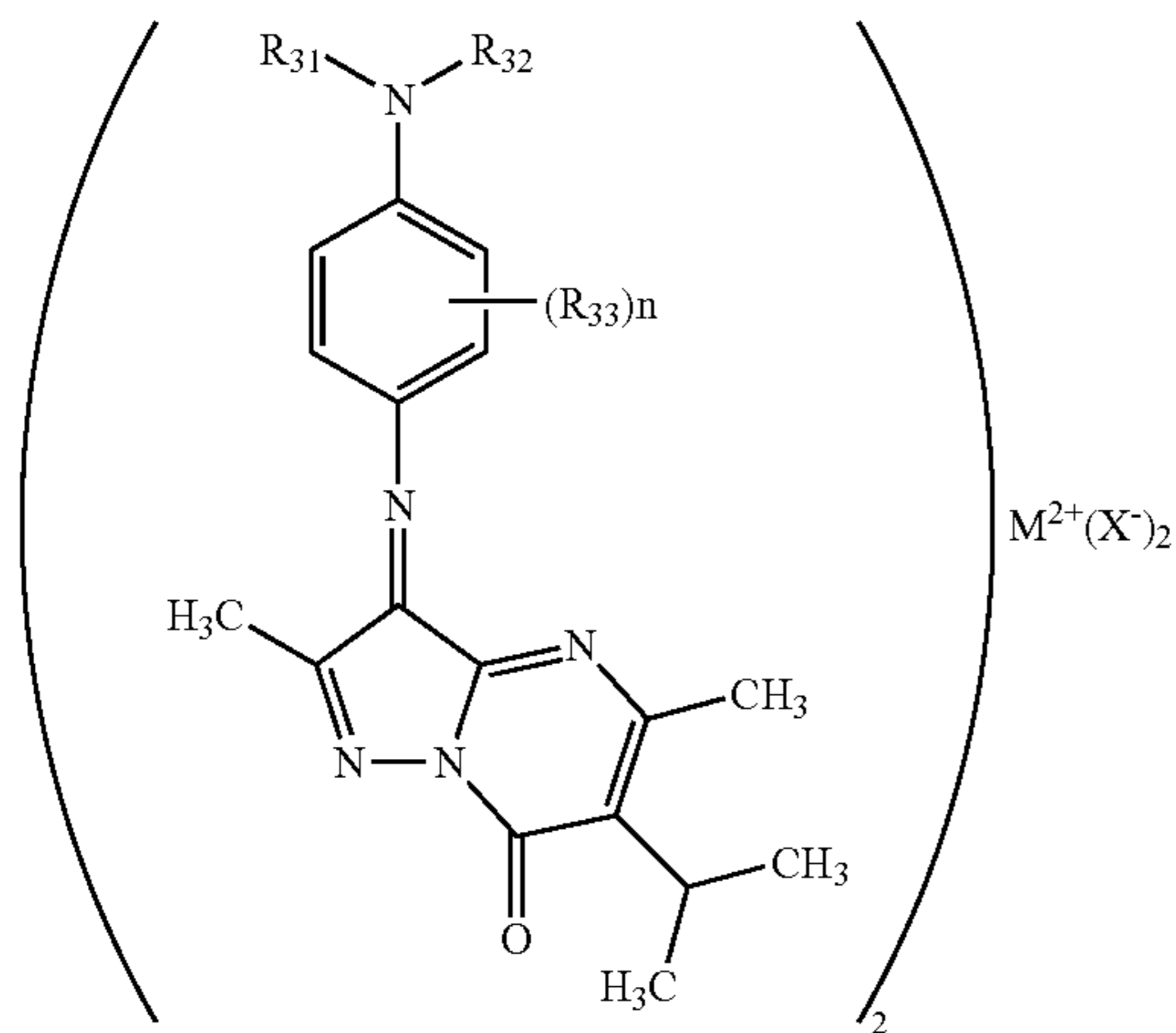
General formula (3)
