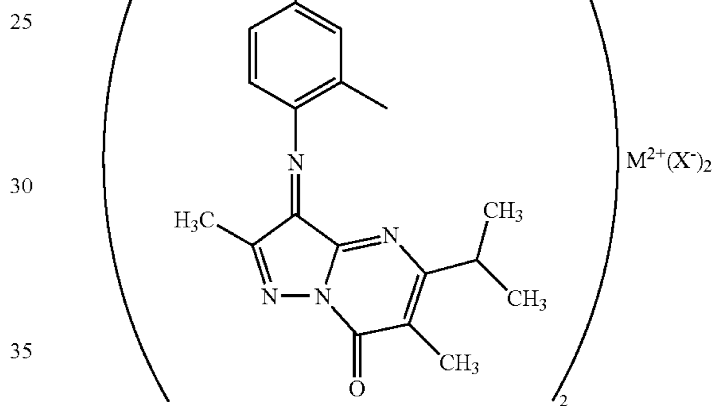
General formula (3)
