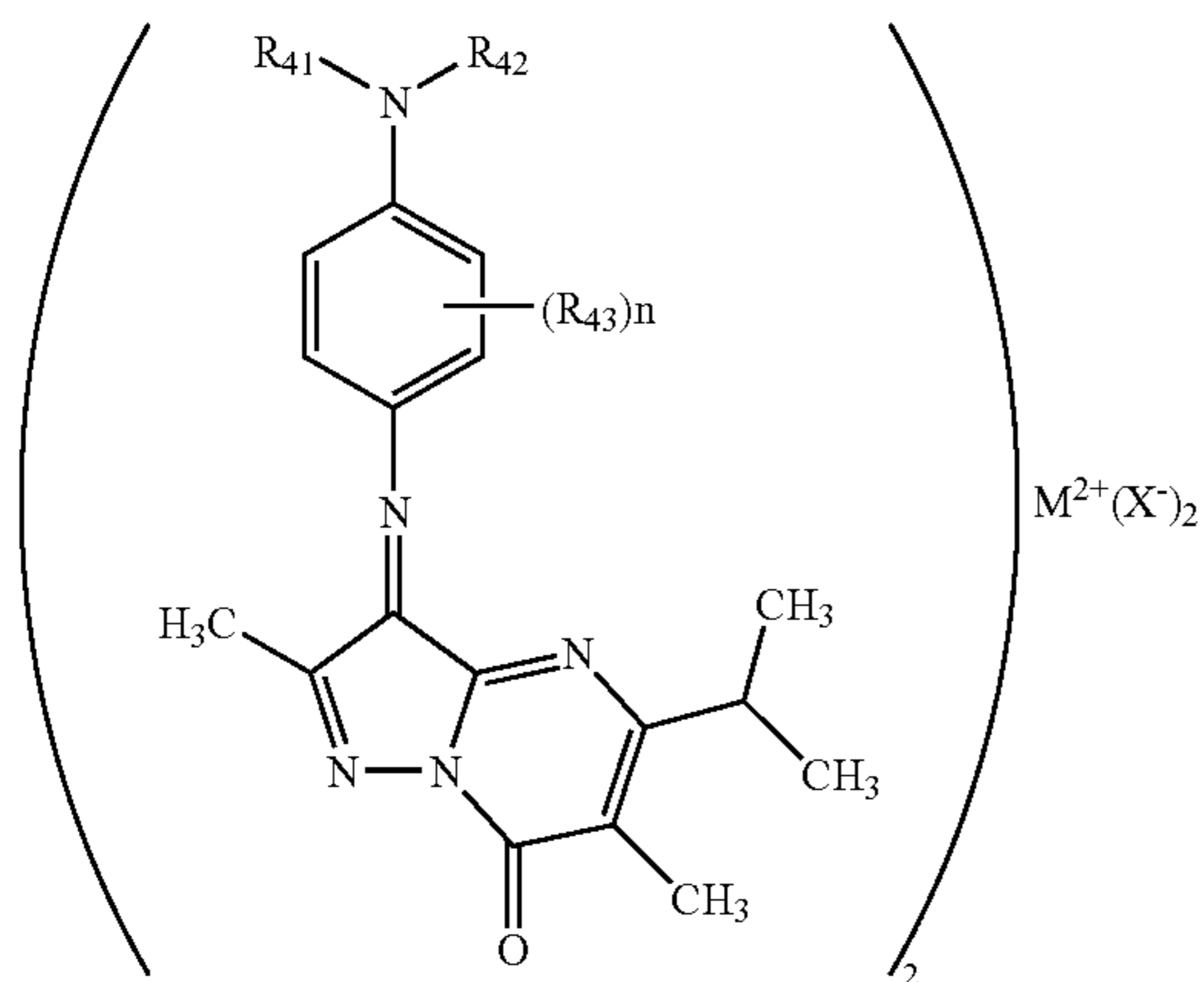
General formula (4)
