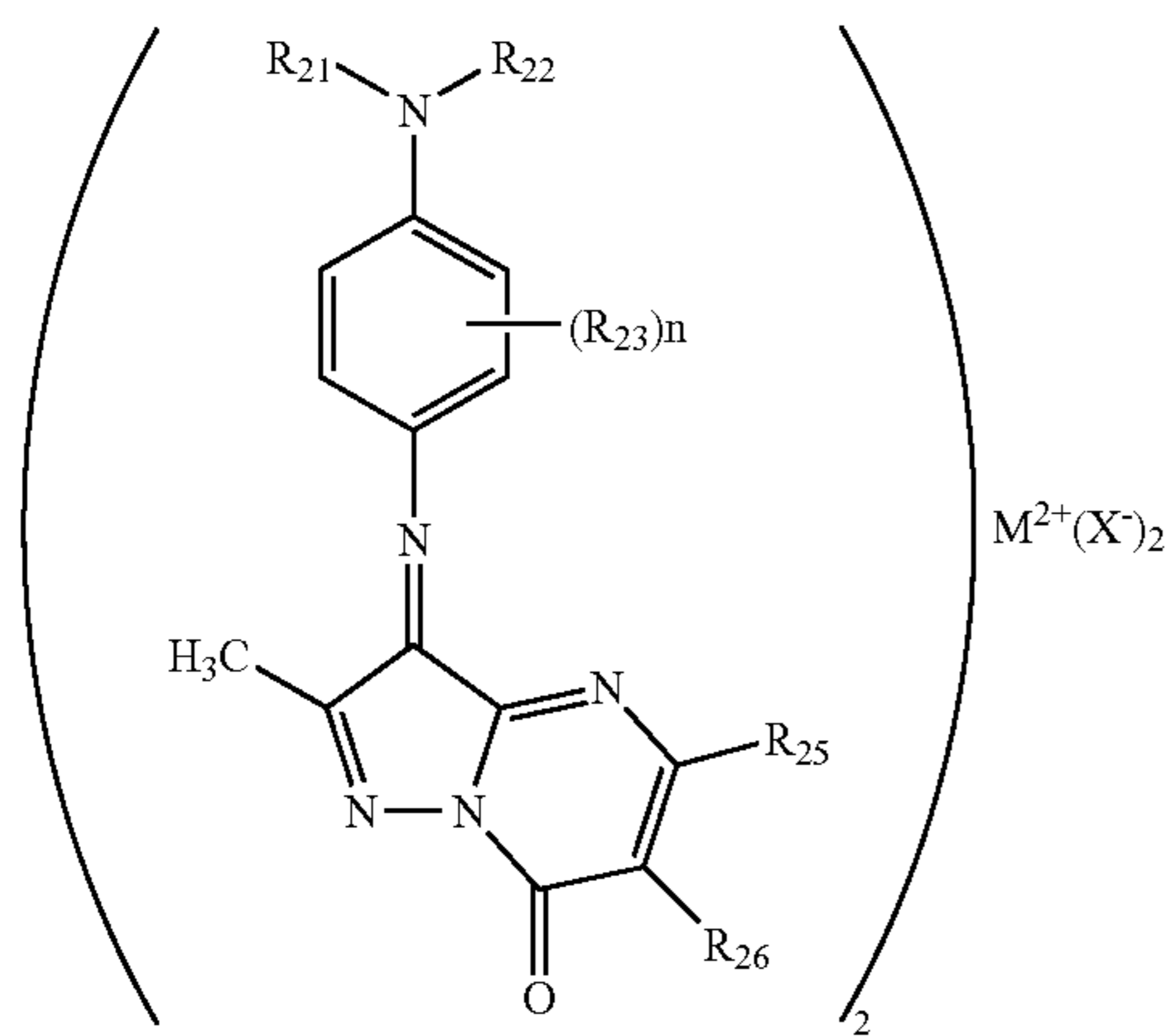
General formula (2)
