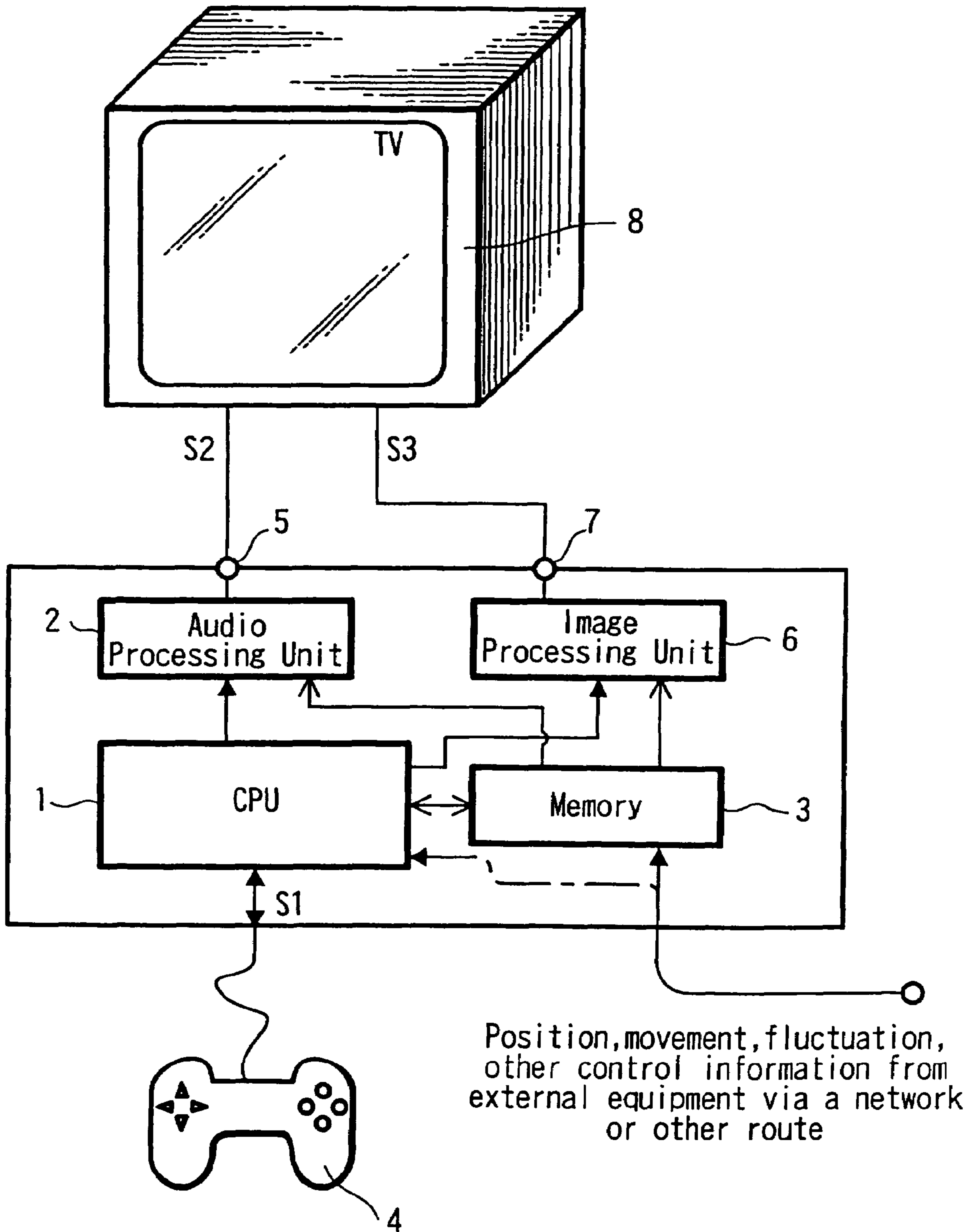
FIG. 4 (PRIOR ART)
