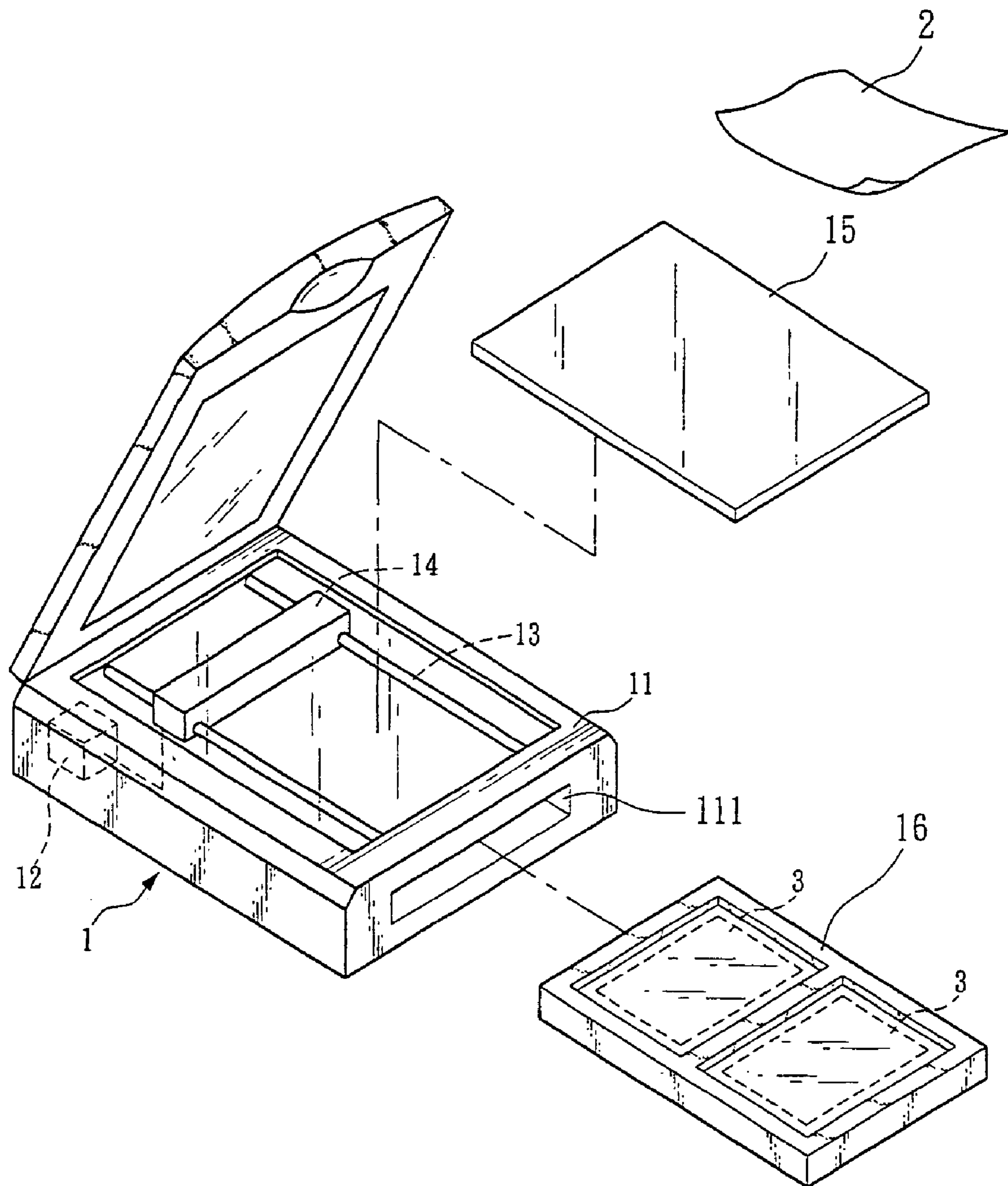
FIG. 2 (PRIOR ART)
