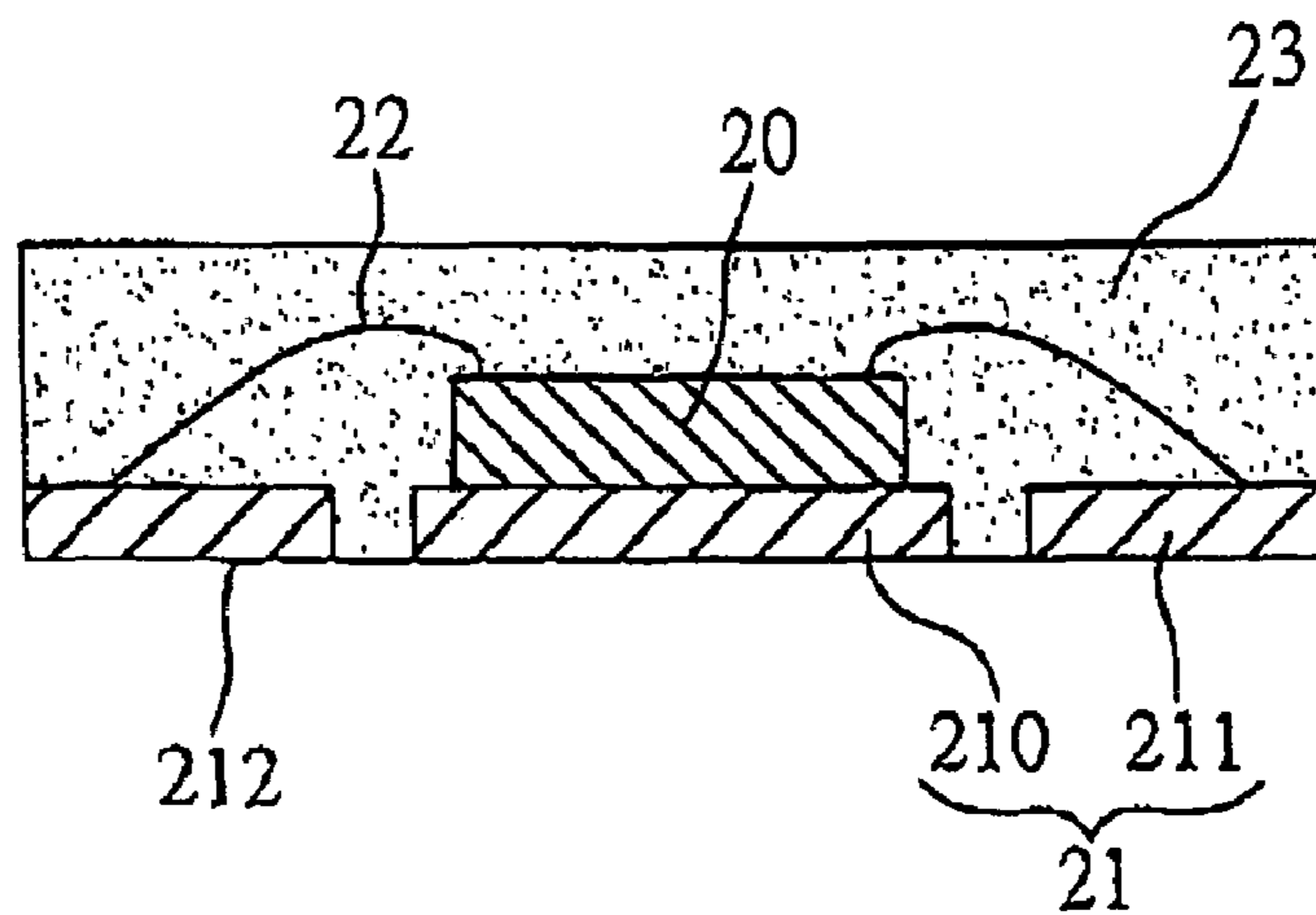
FIG. 6 (PRIOR ART)
