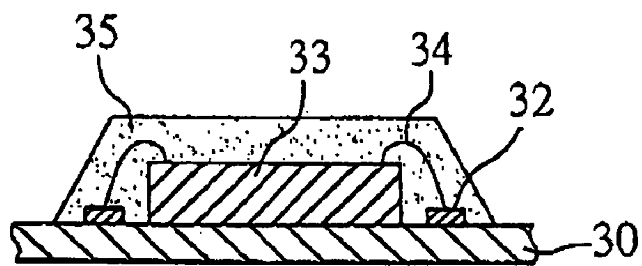
FIG. 9C (PRIOR ART)
