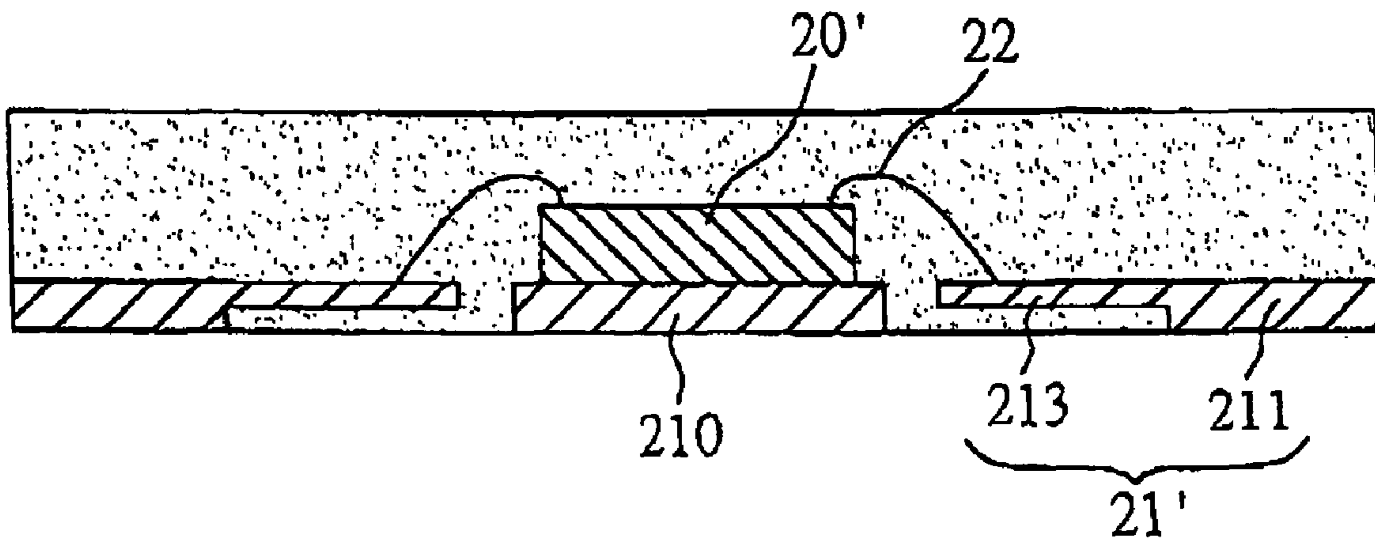
FIG. 8 (PRIOR ART)
