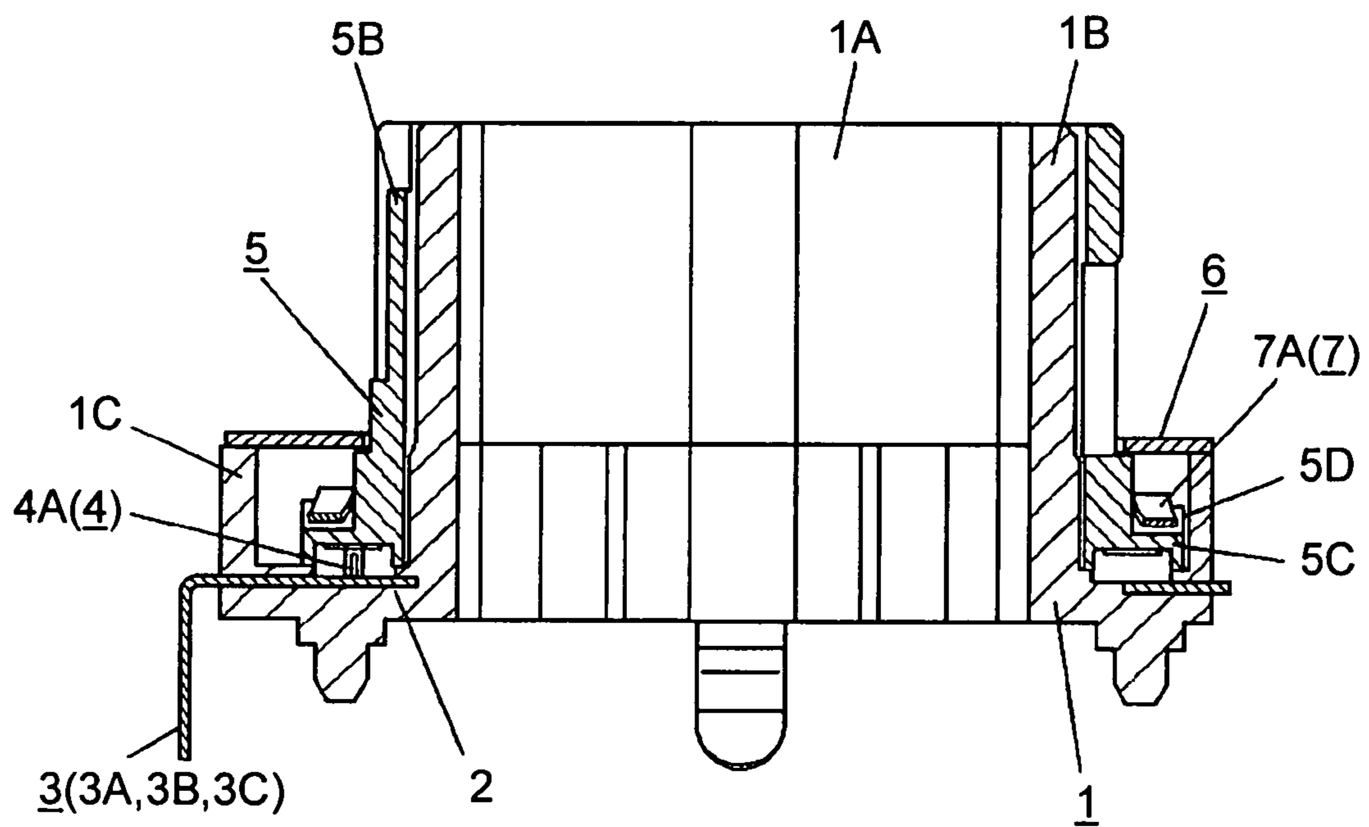
FIG. 12 PRIOR ART
