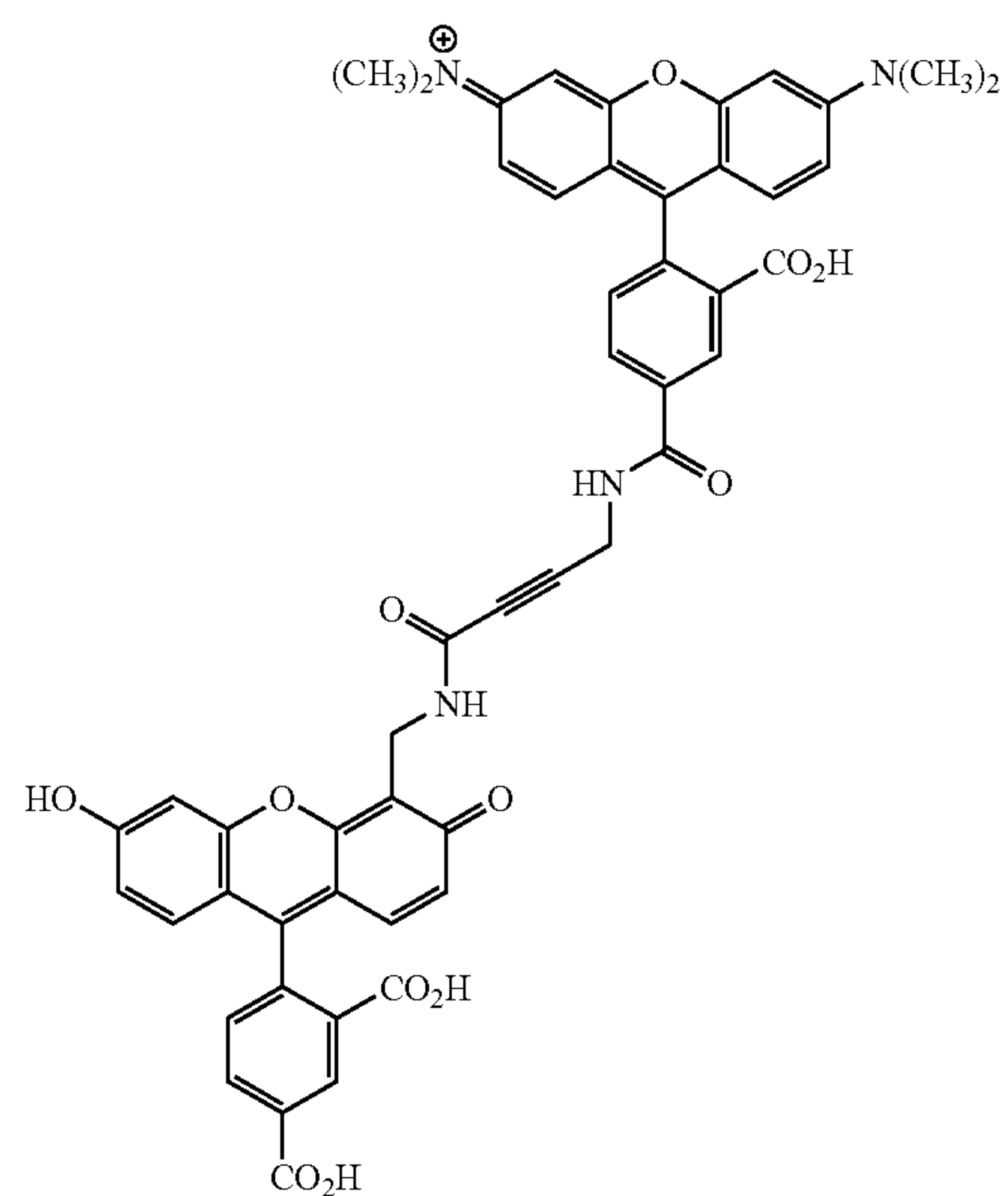
5-TMR-A-CF
