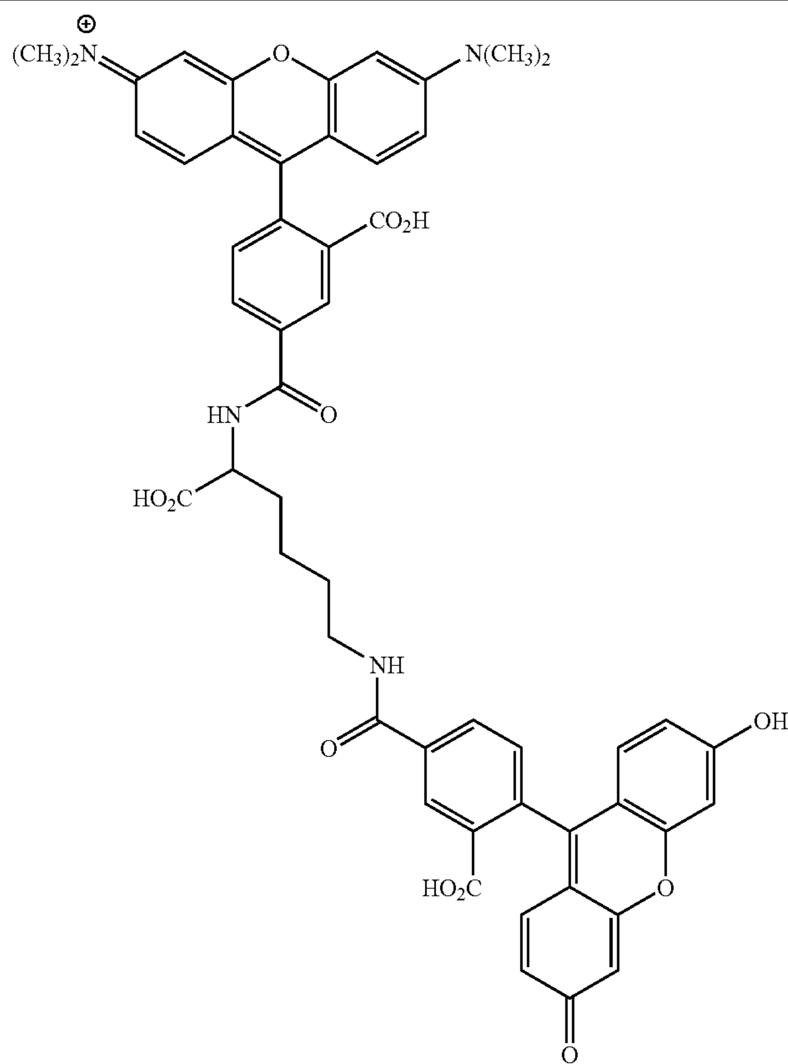
5TMR-lys-5FAM
