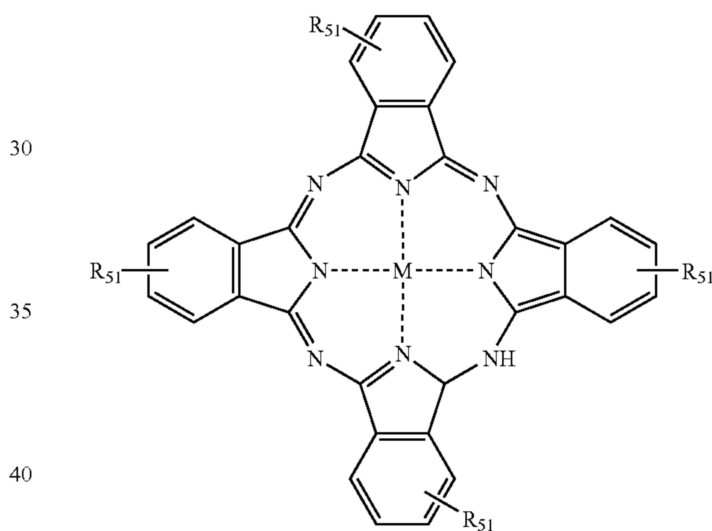
PHTHALOCYANINE
