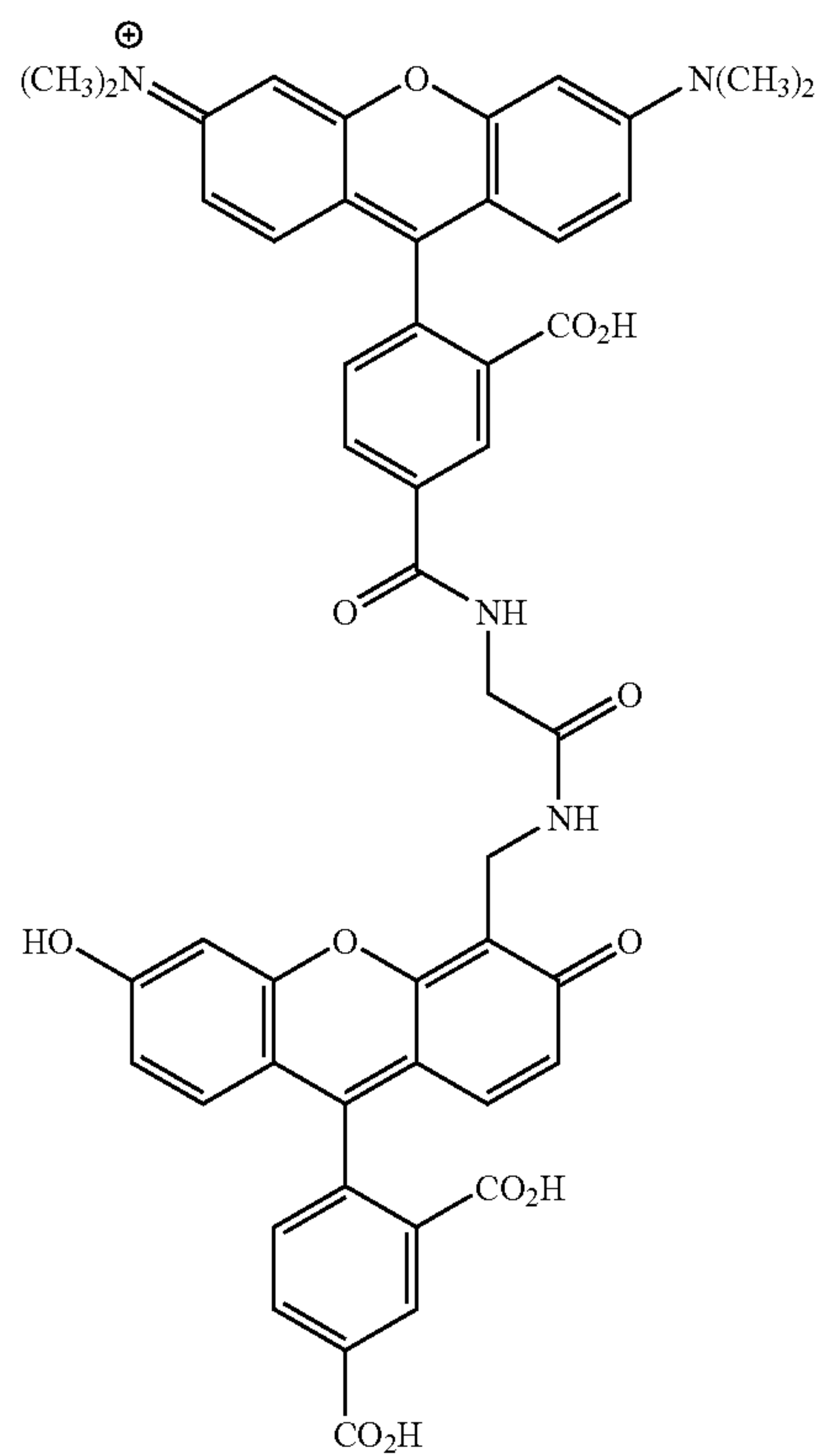
5TMR-gly-CF
