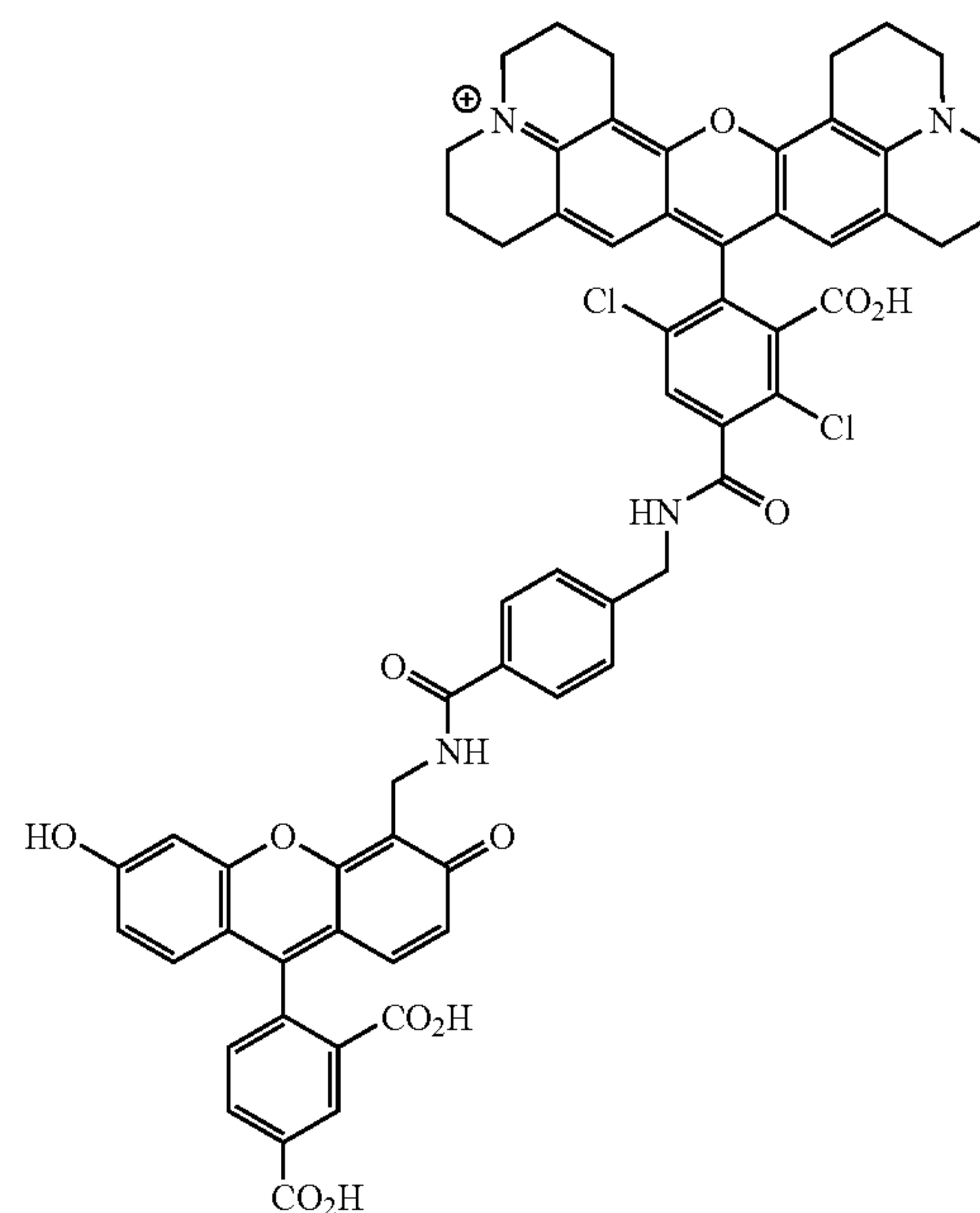
5-CFB-DROX-2
