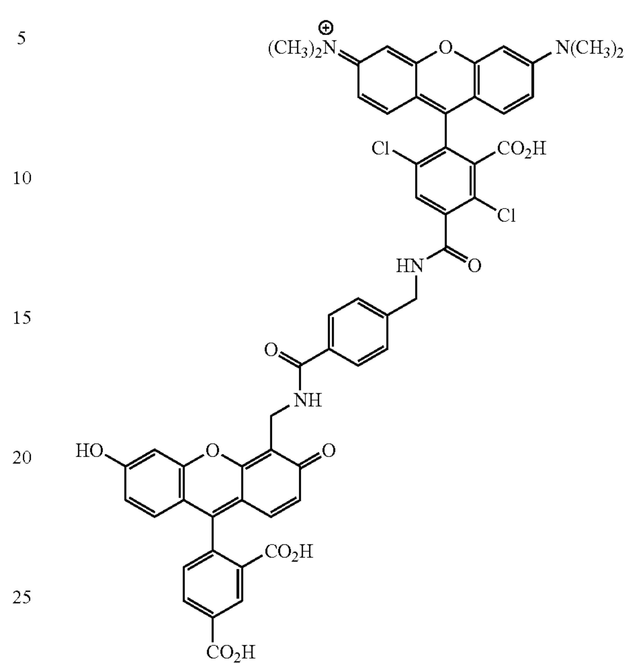
5-DTMR-B-CF
