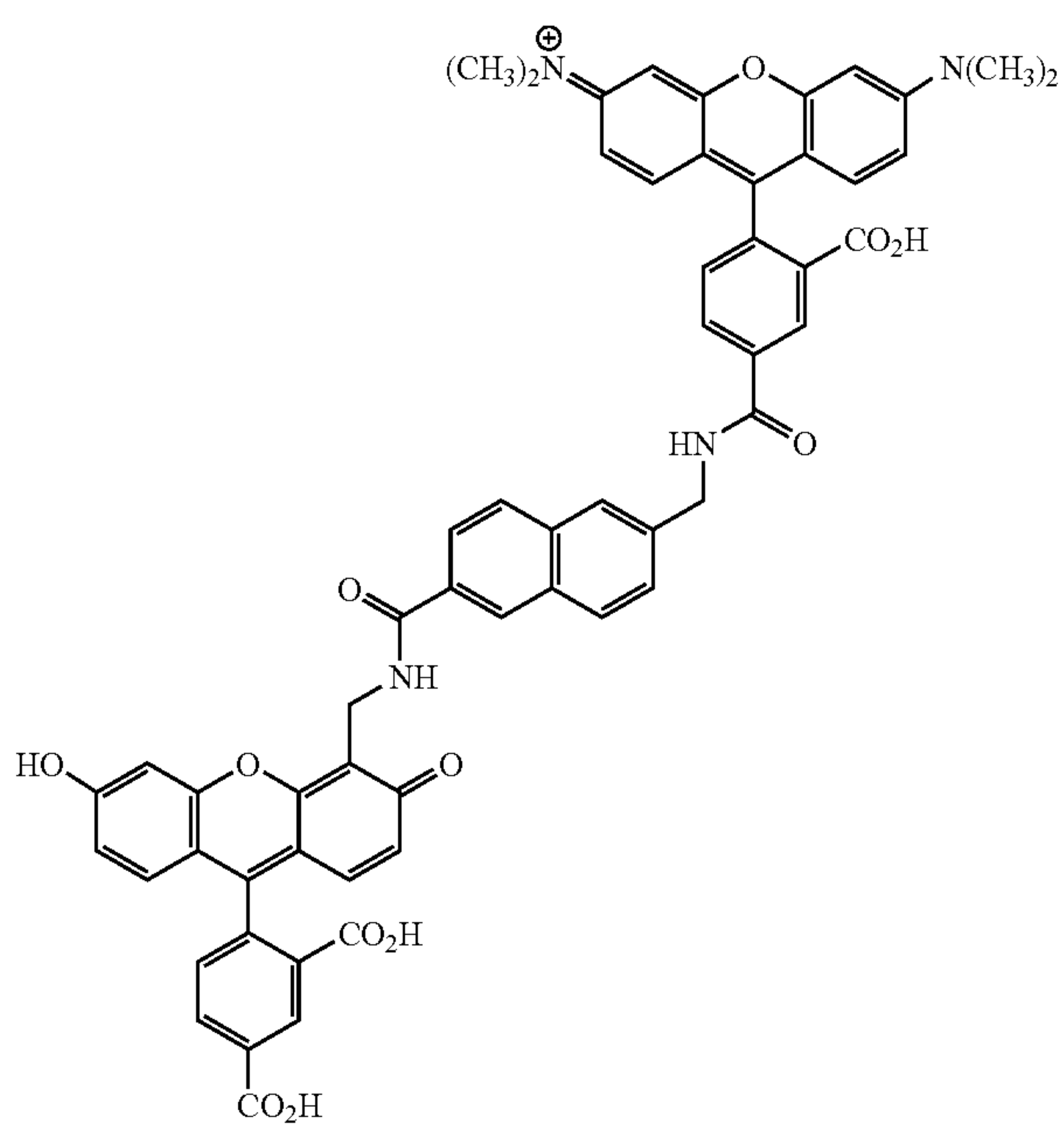
5-TMR-N-CF
