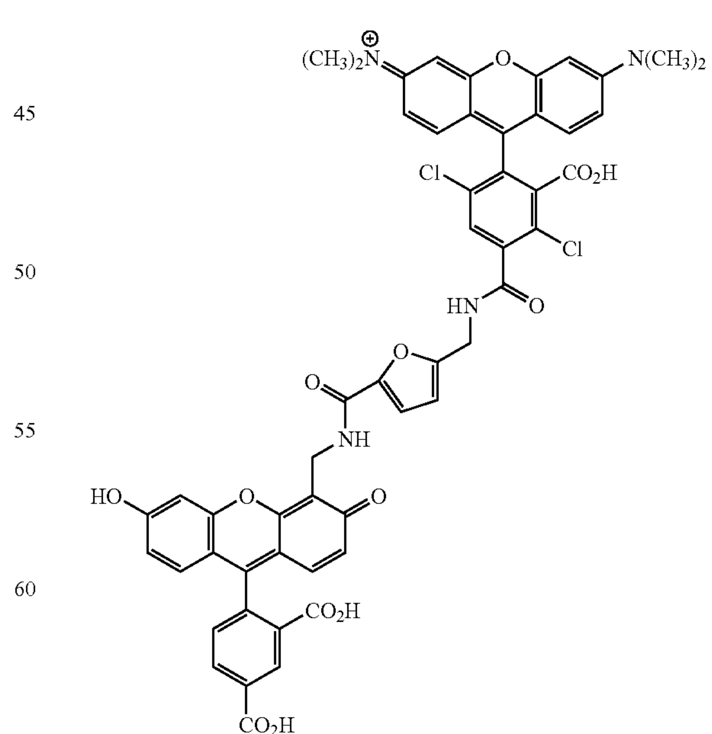
5-DTMR-F-CF
