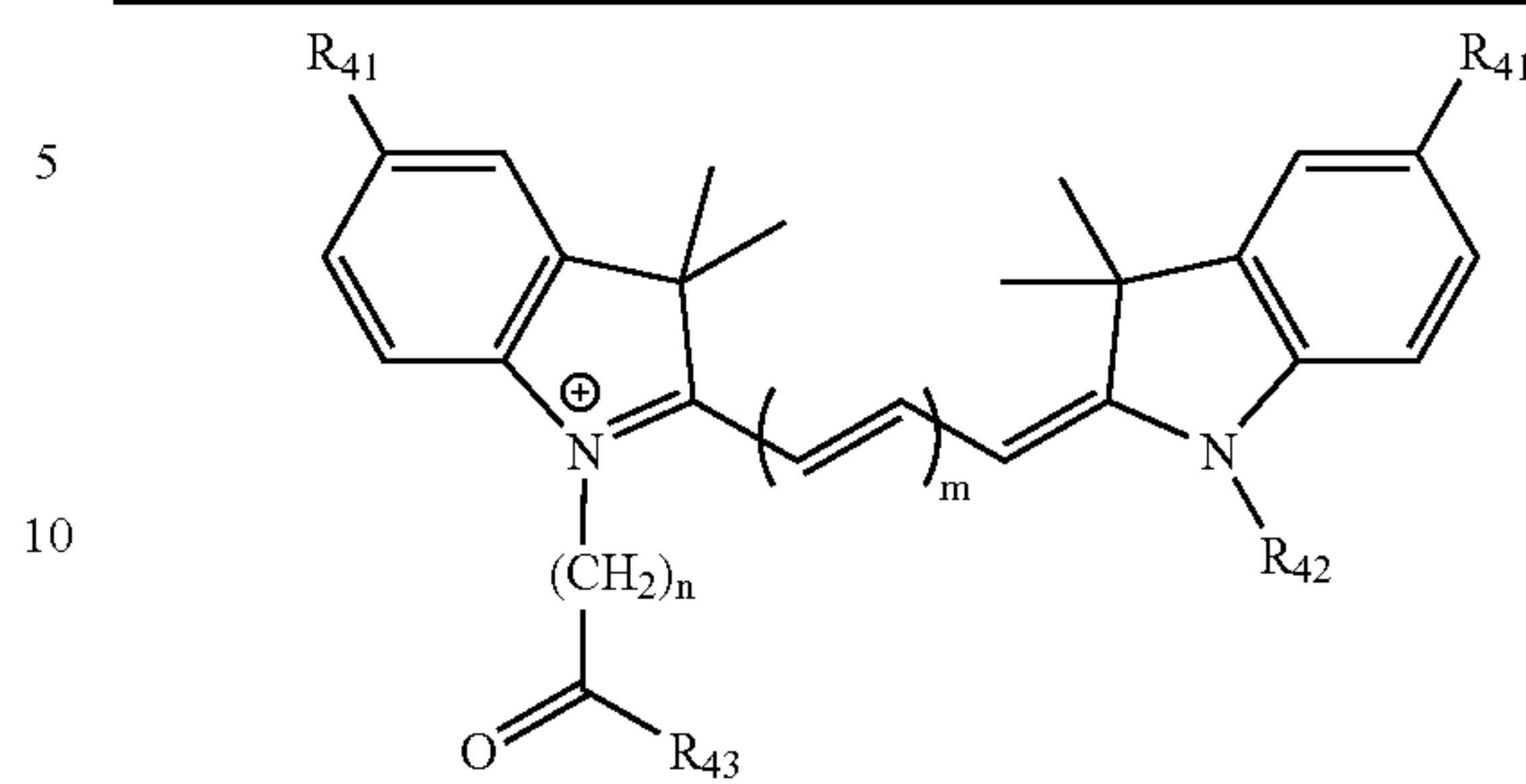
CYANINE
