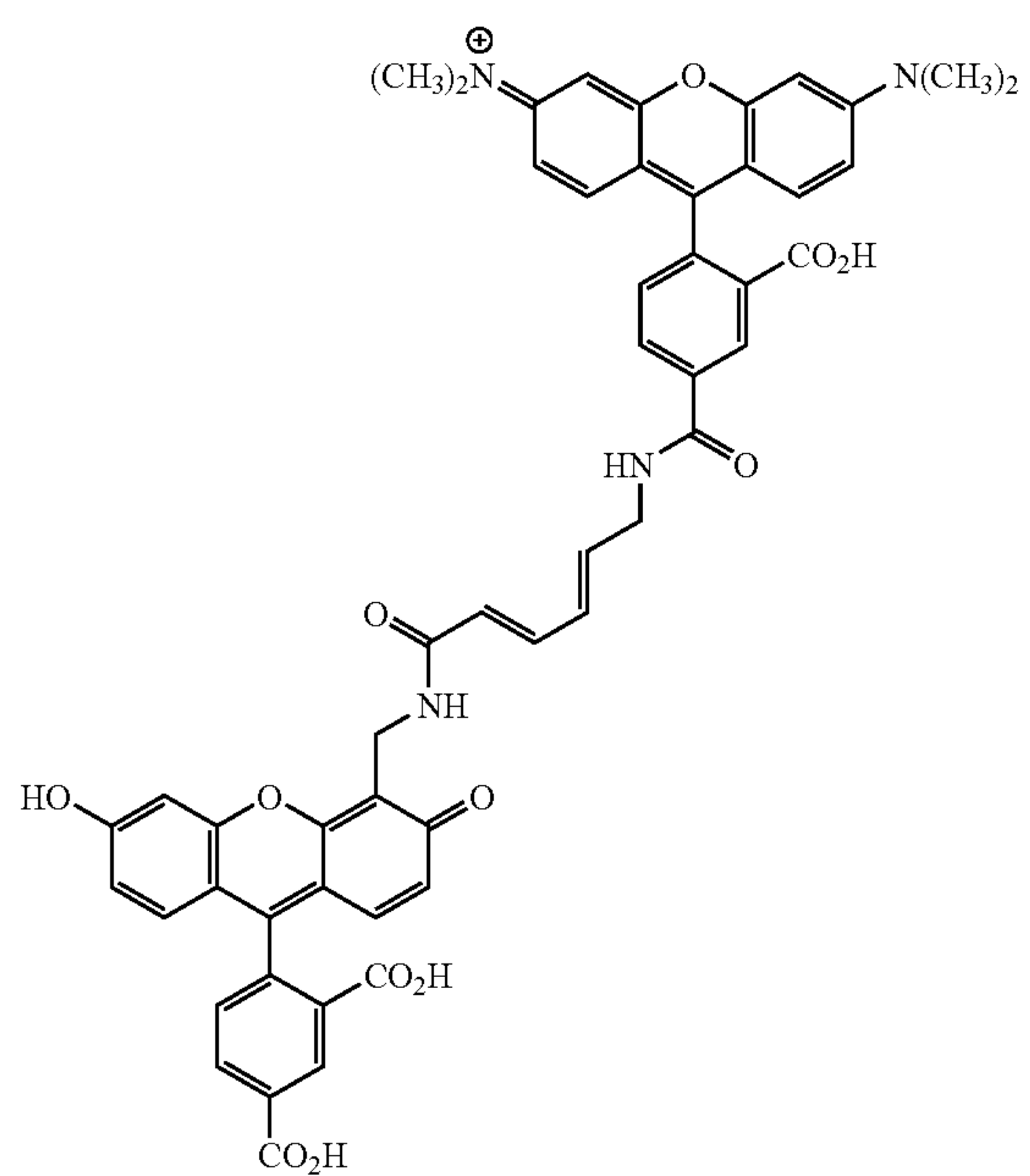
5-TMR-D-CF
