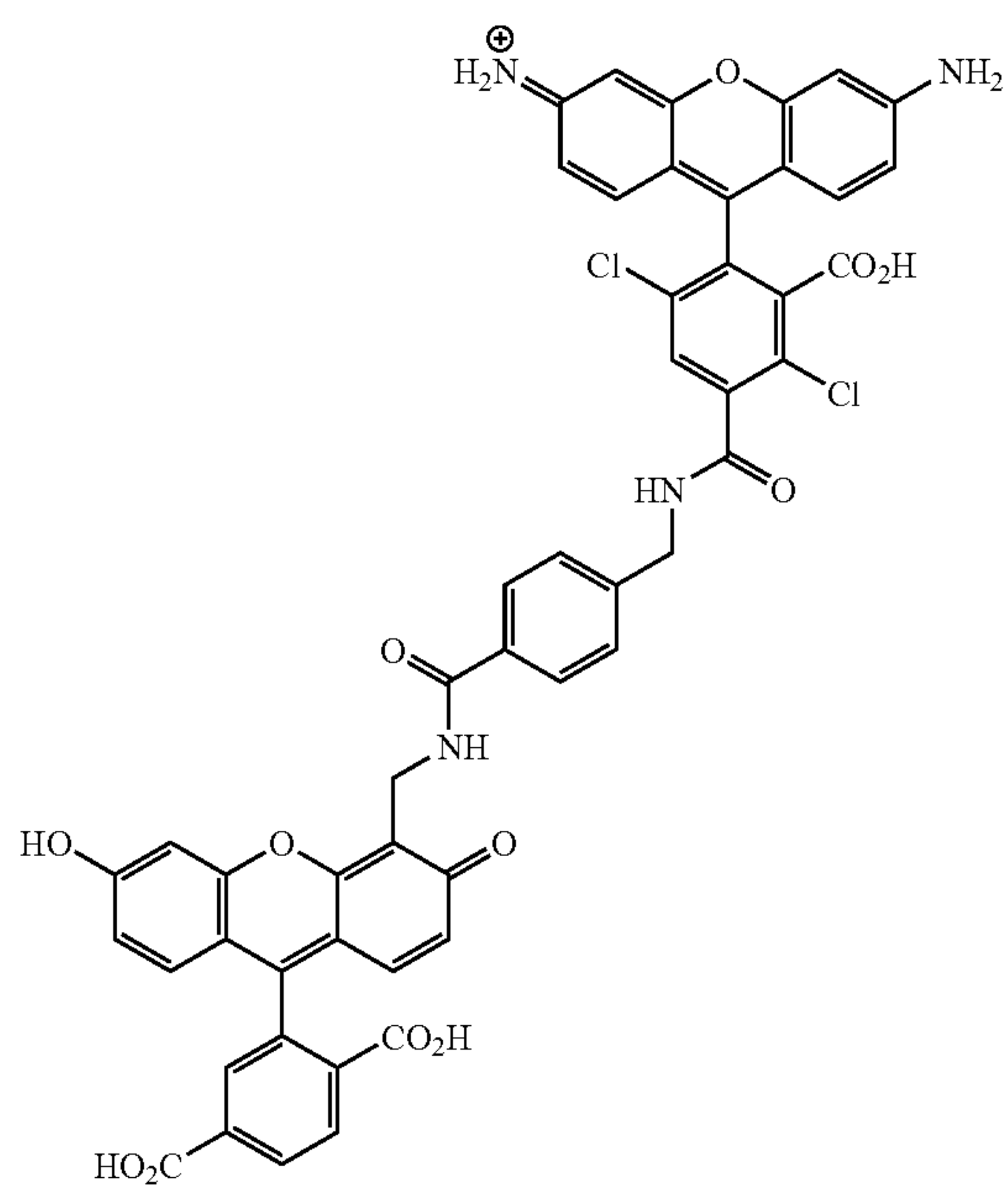
6-CFB-DR110-2
