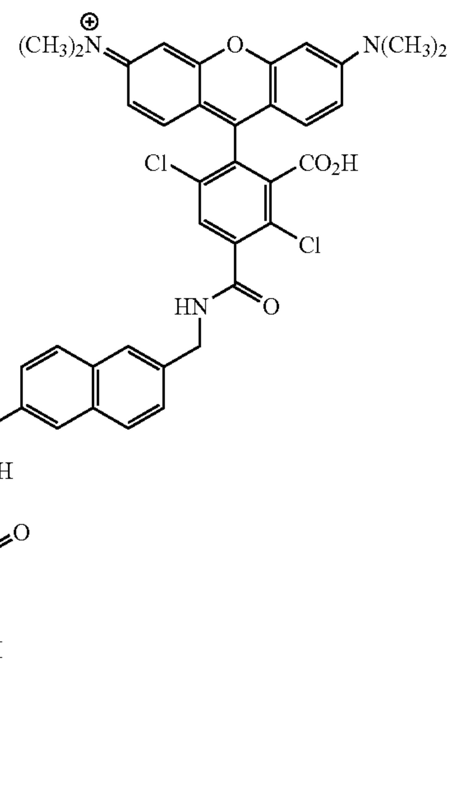
5-DTMR-N-CF
