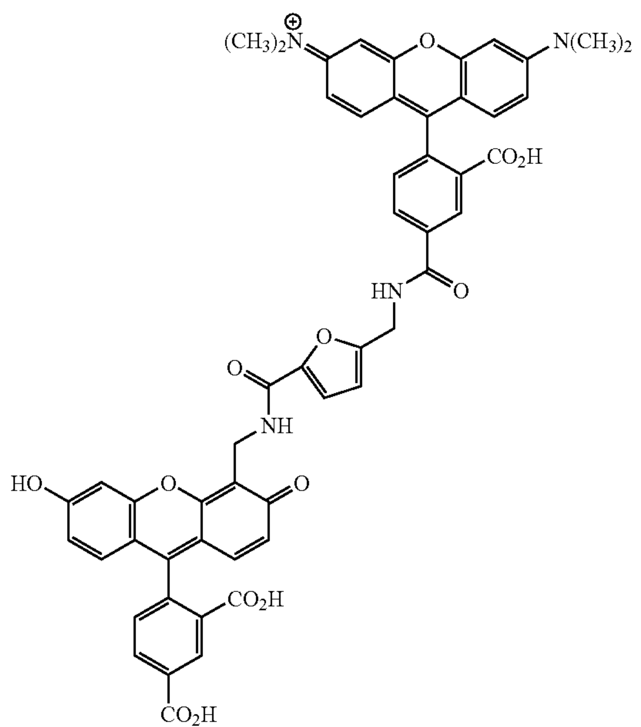
5-TMR-F-CF
