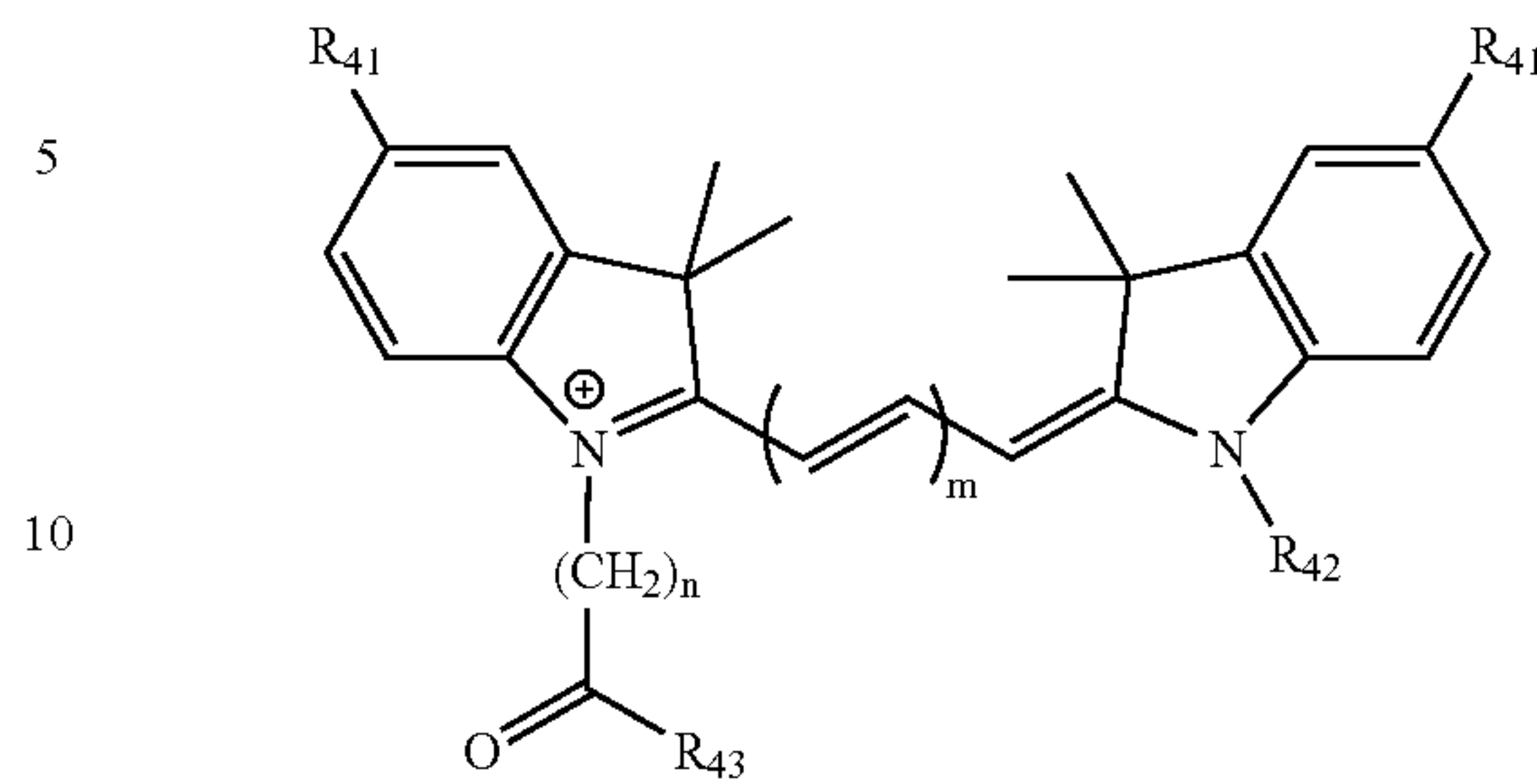
CYANINE
