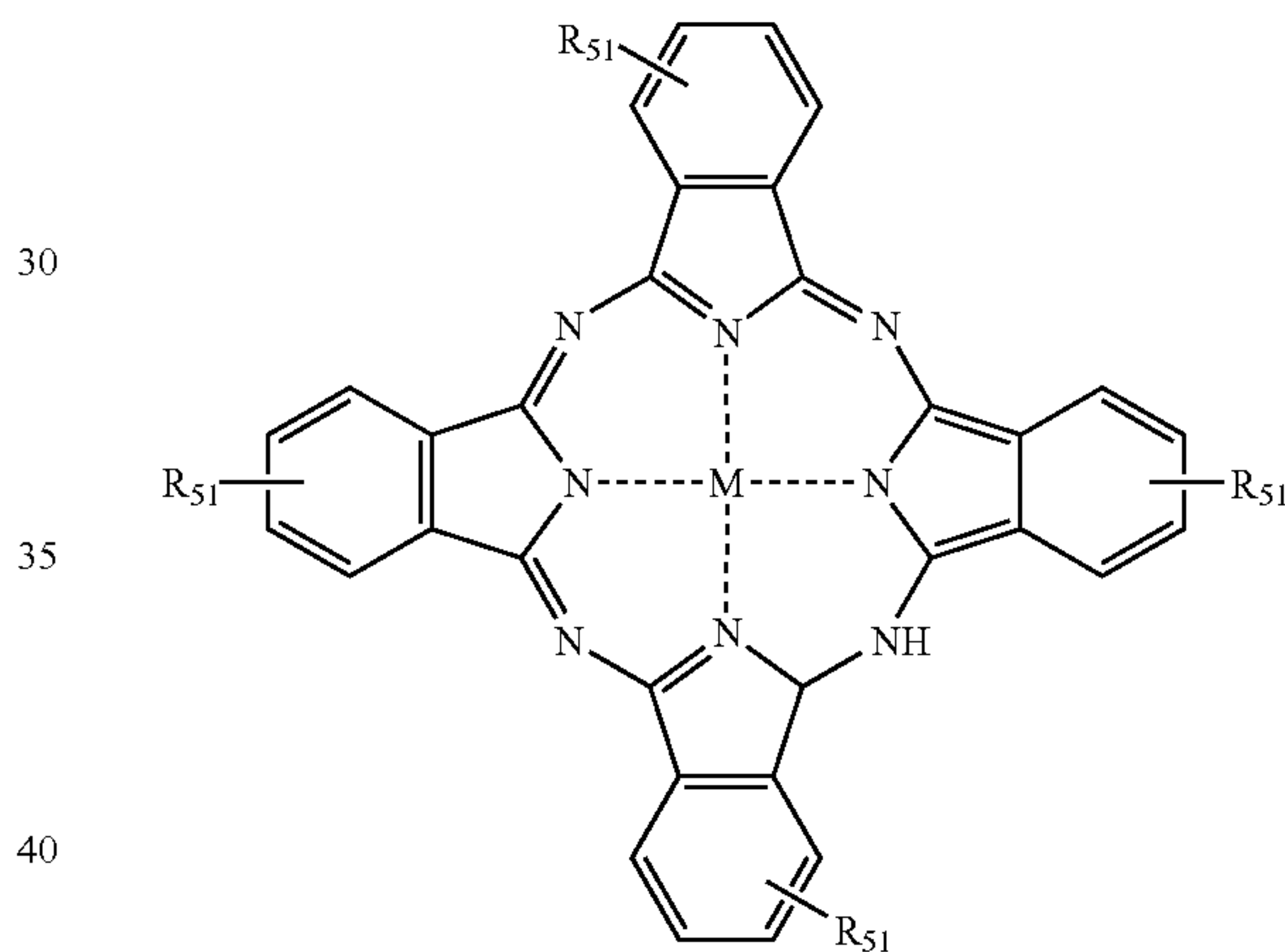
PHTHALOCYANINE
