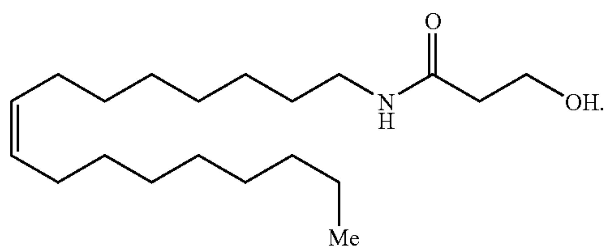
Reverse OEA
