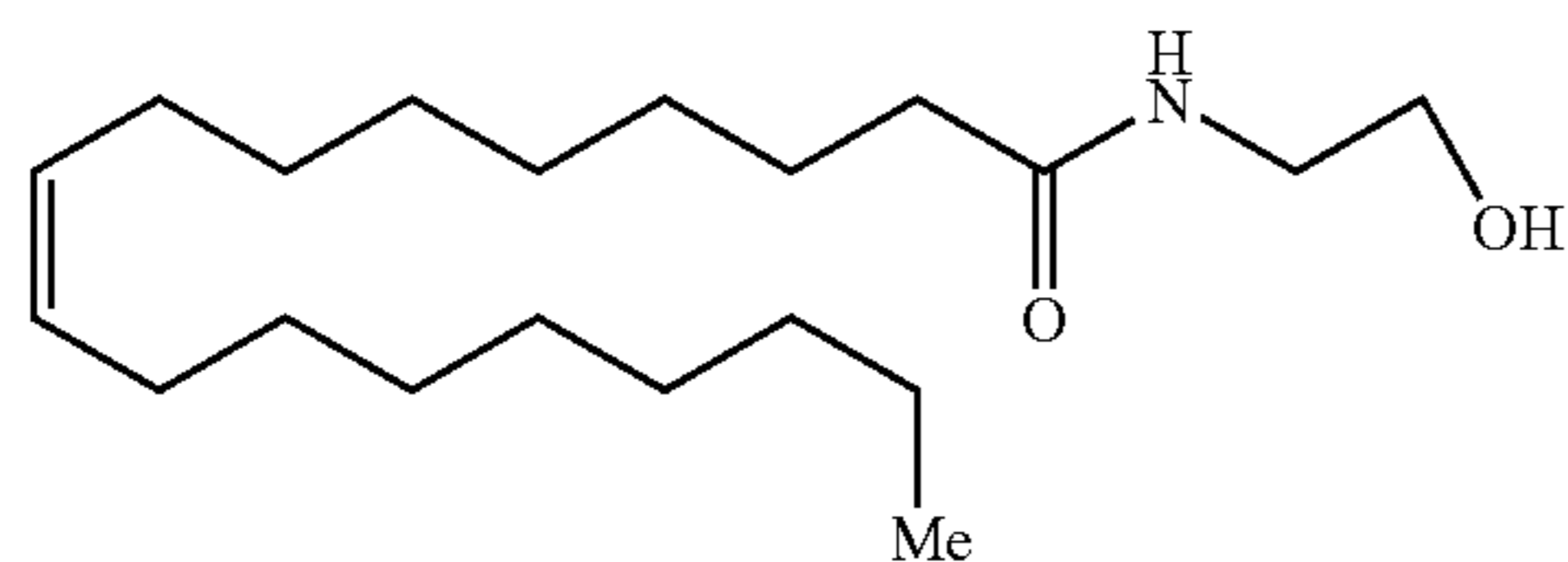
Oleylethanolamide
