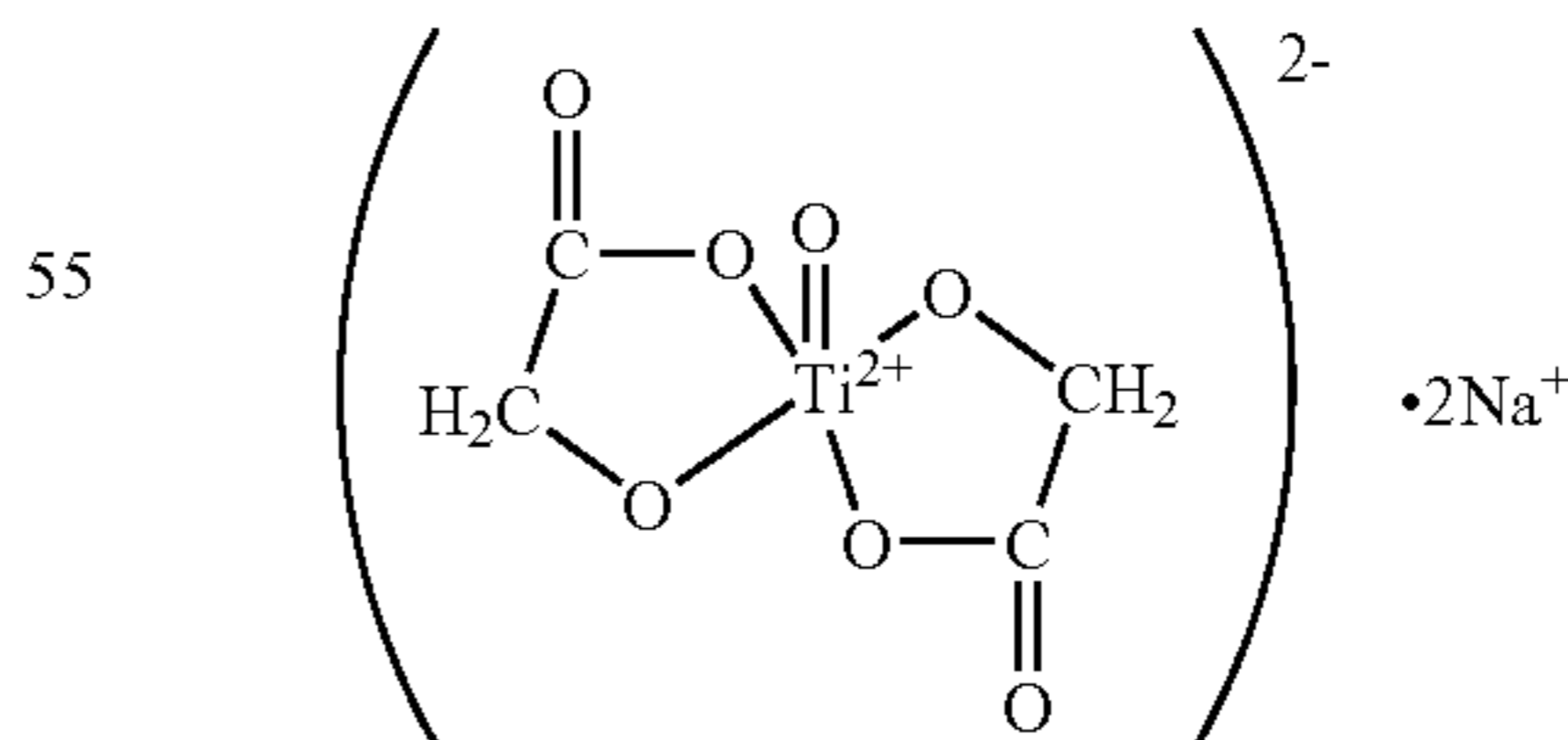
Ti Chelate Compound (11)
