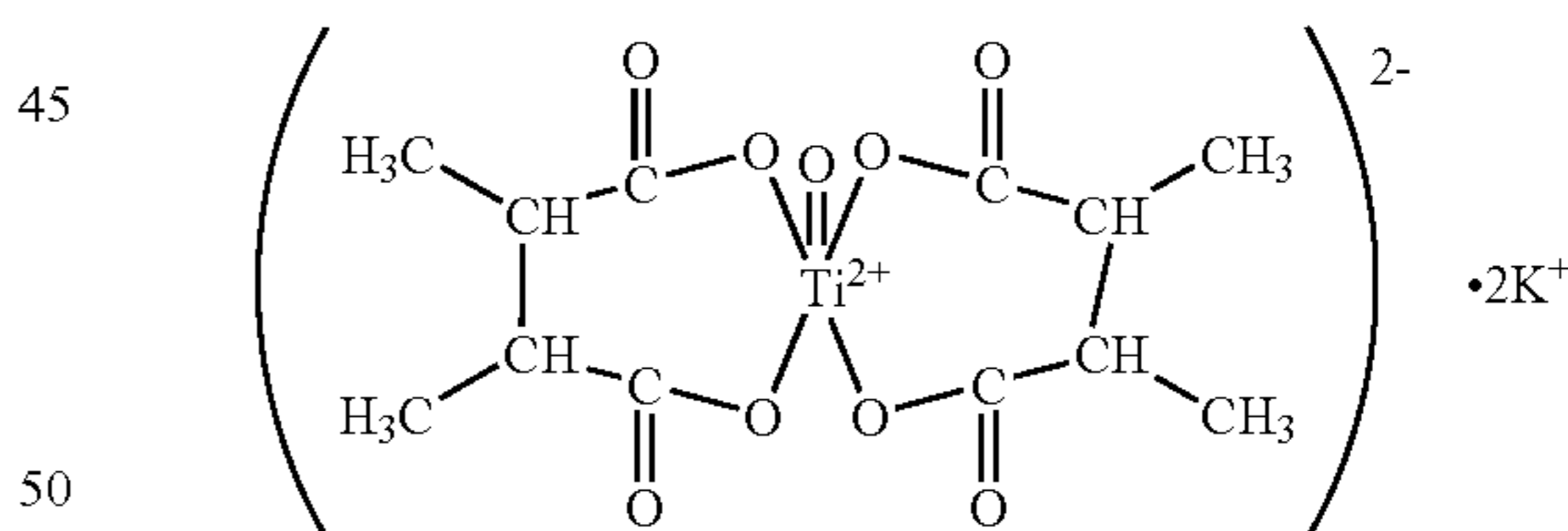
Ti Chelate Compound (11)
