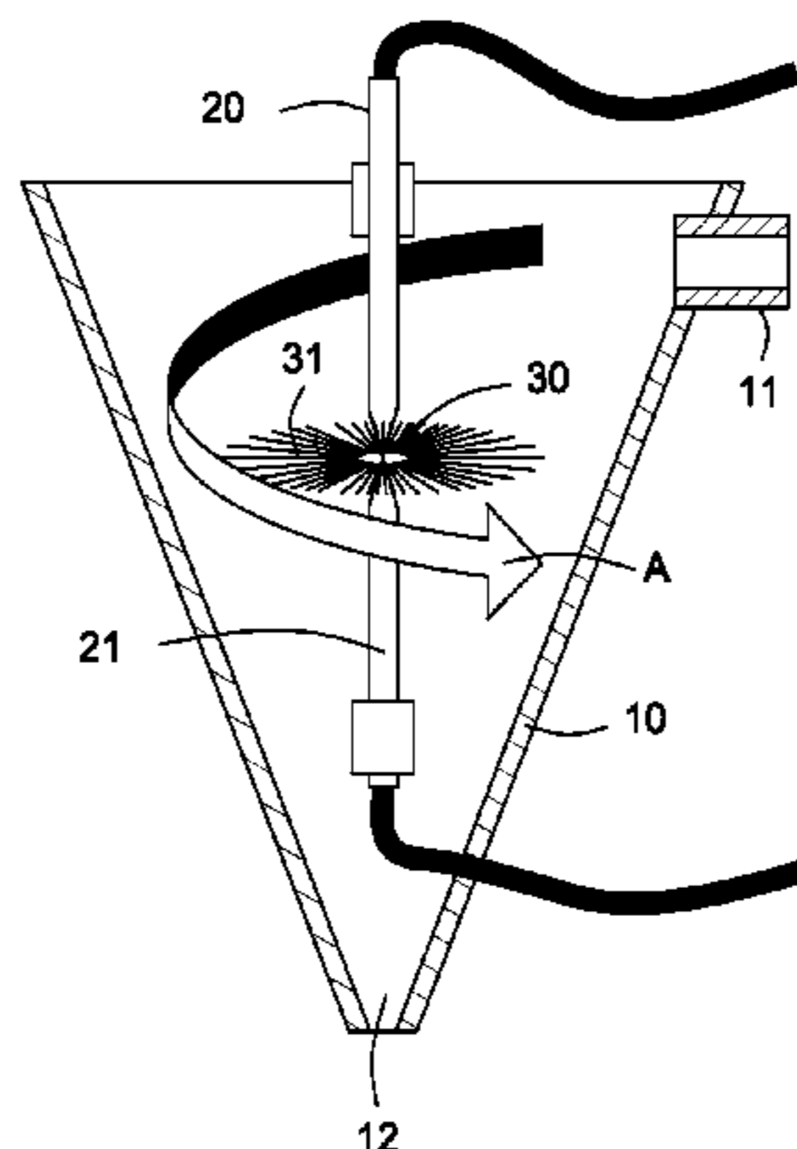
Treatment of Fluids With Carbon Arc
