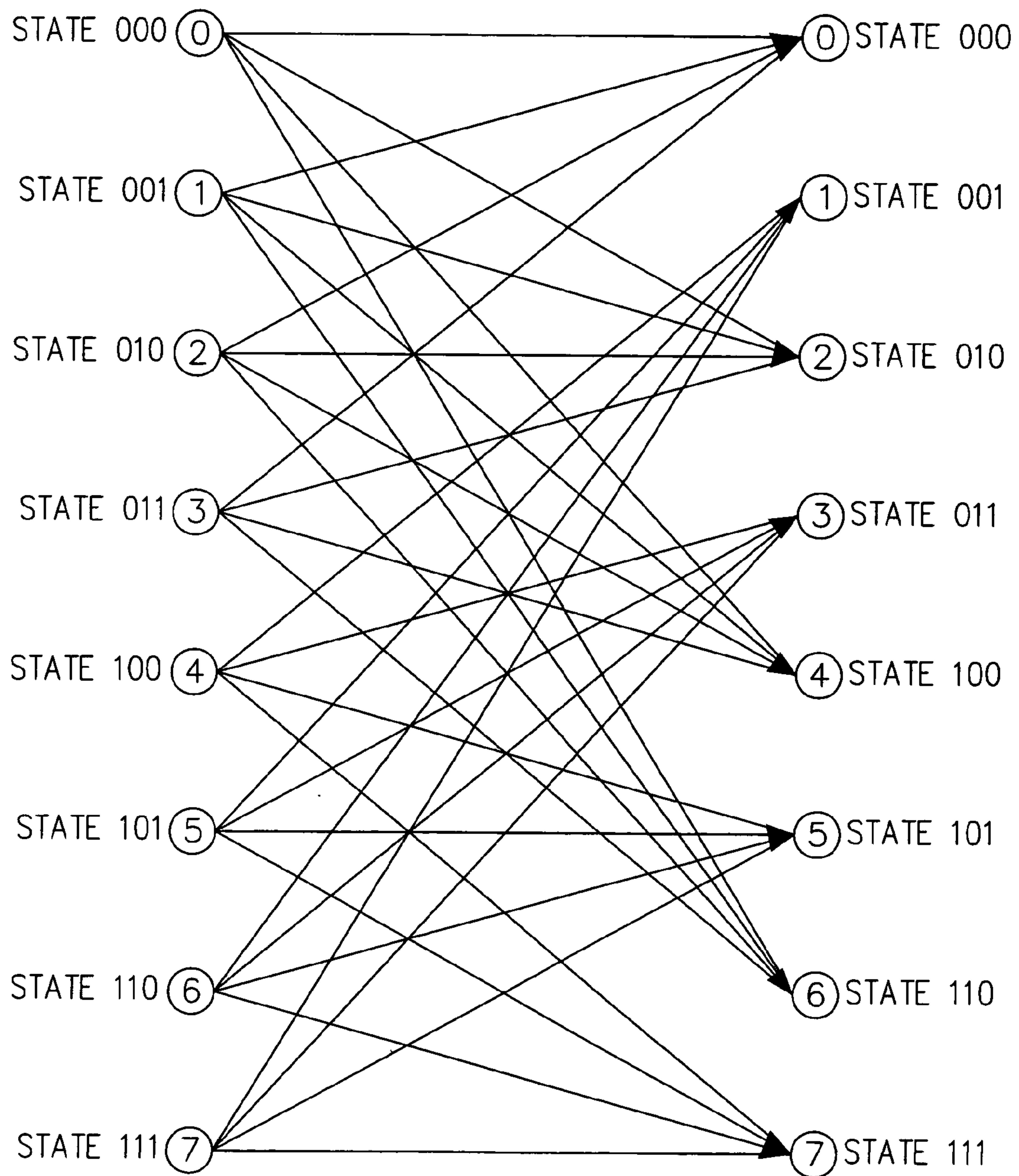
RATE 2/3 BASIC CONSTITUENT ENCODER
