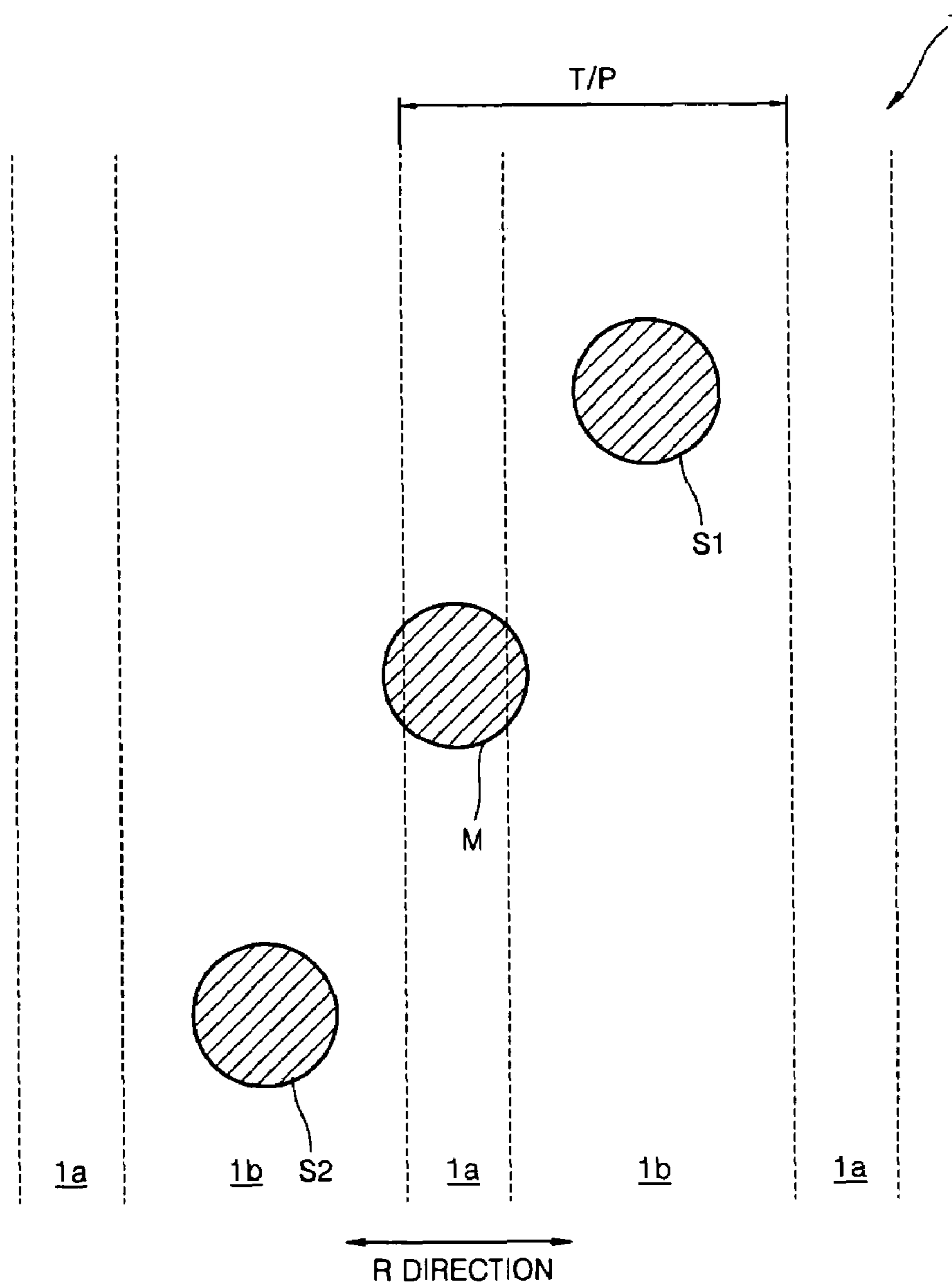
FIG. 1 (PRIOR ART)
