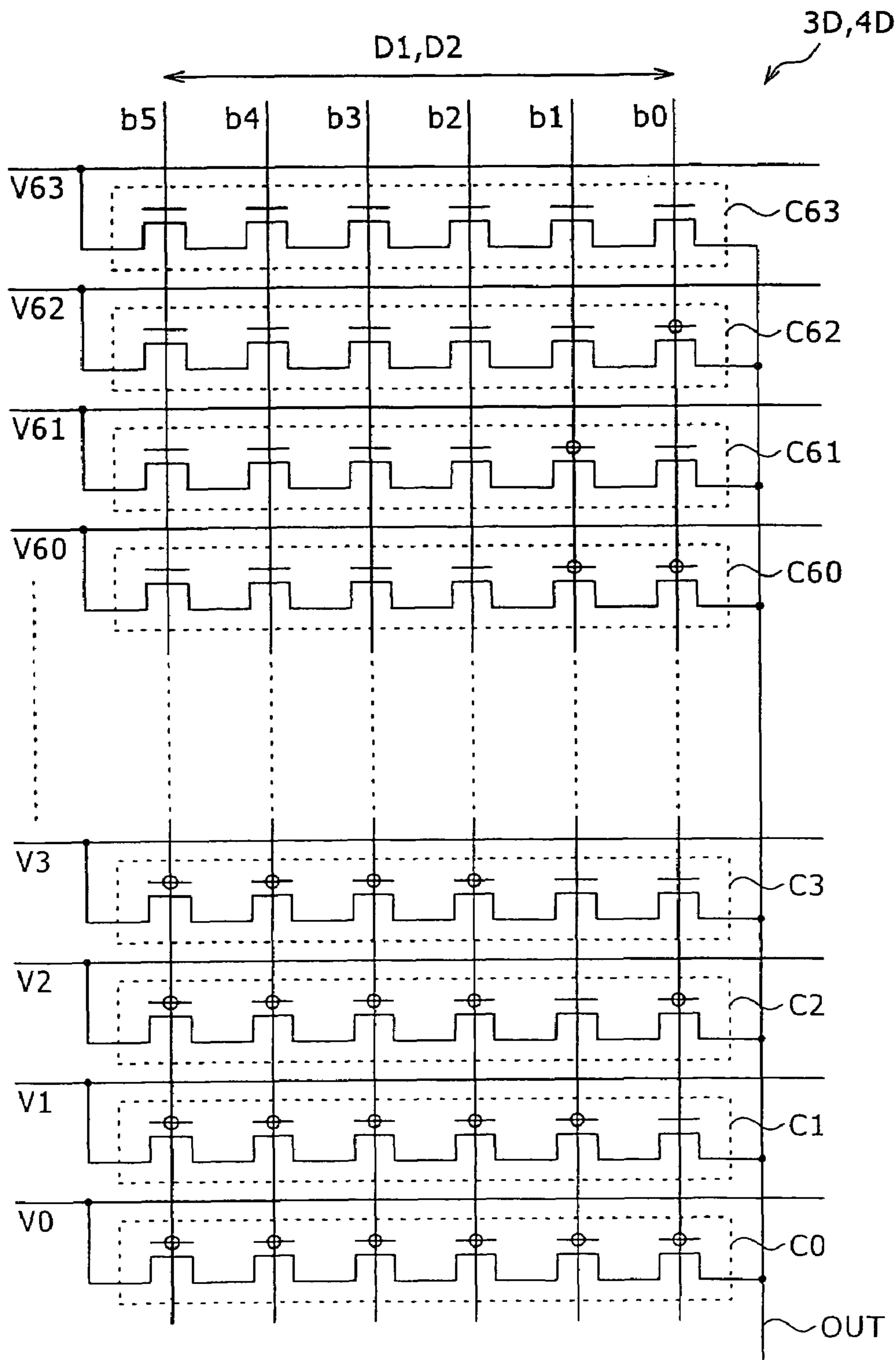
FIG. 3 (PRIOR ART)
