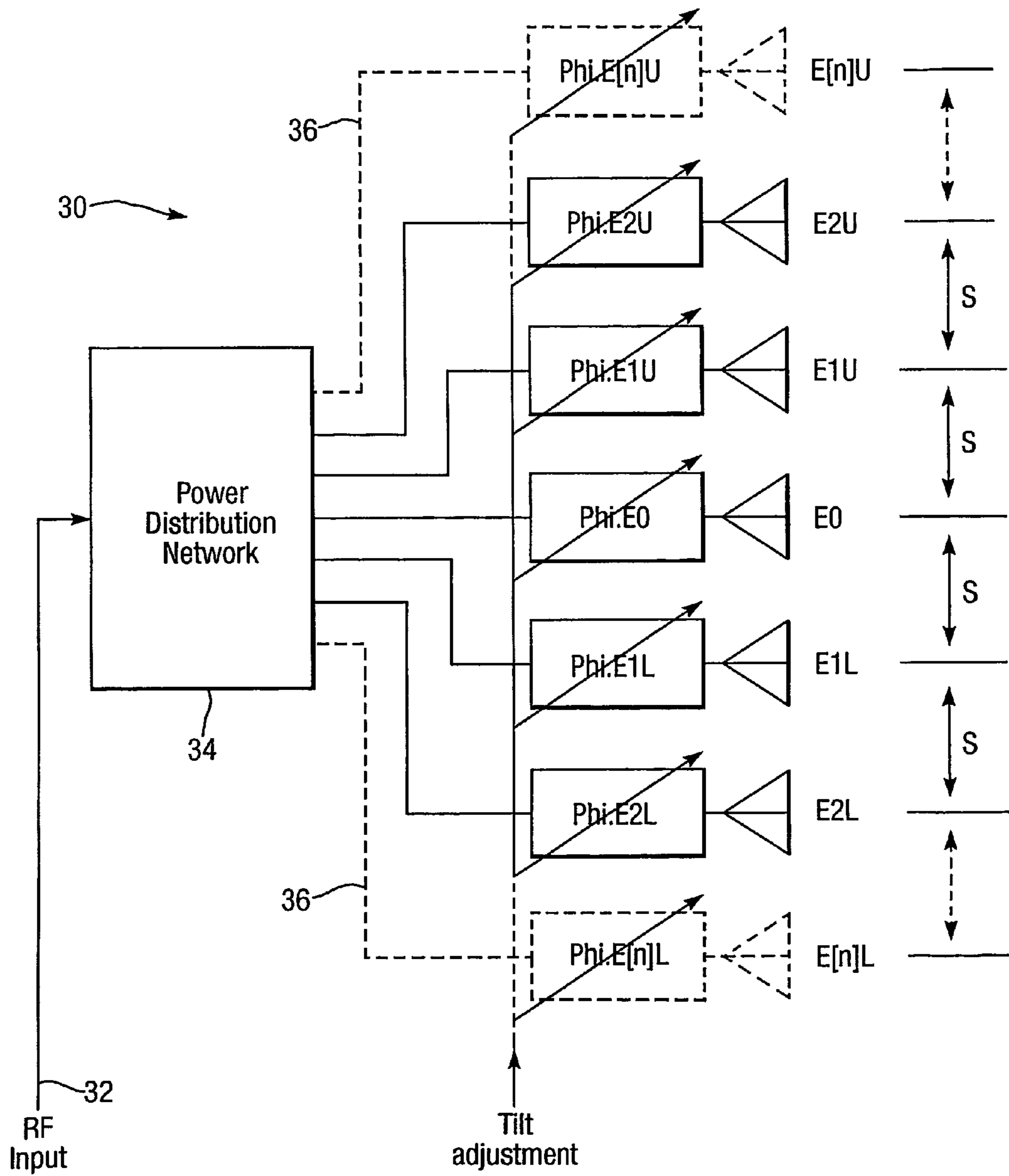
Fig.2. (Prior art)
