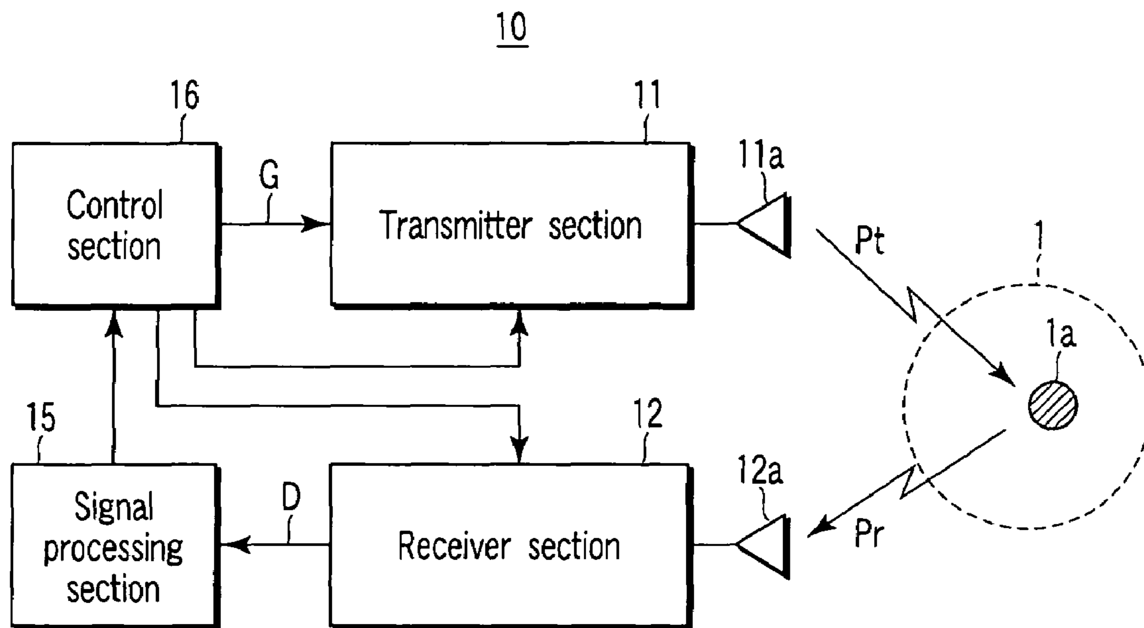
FIG. 10 (PRIOR ART)
