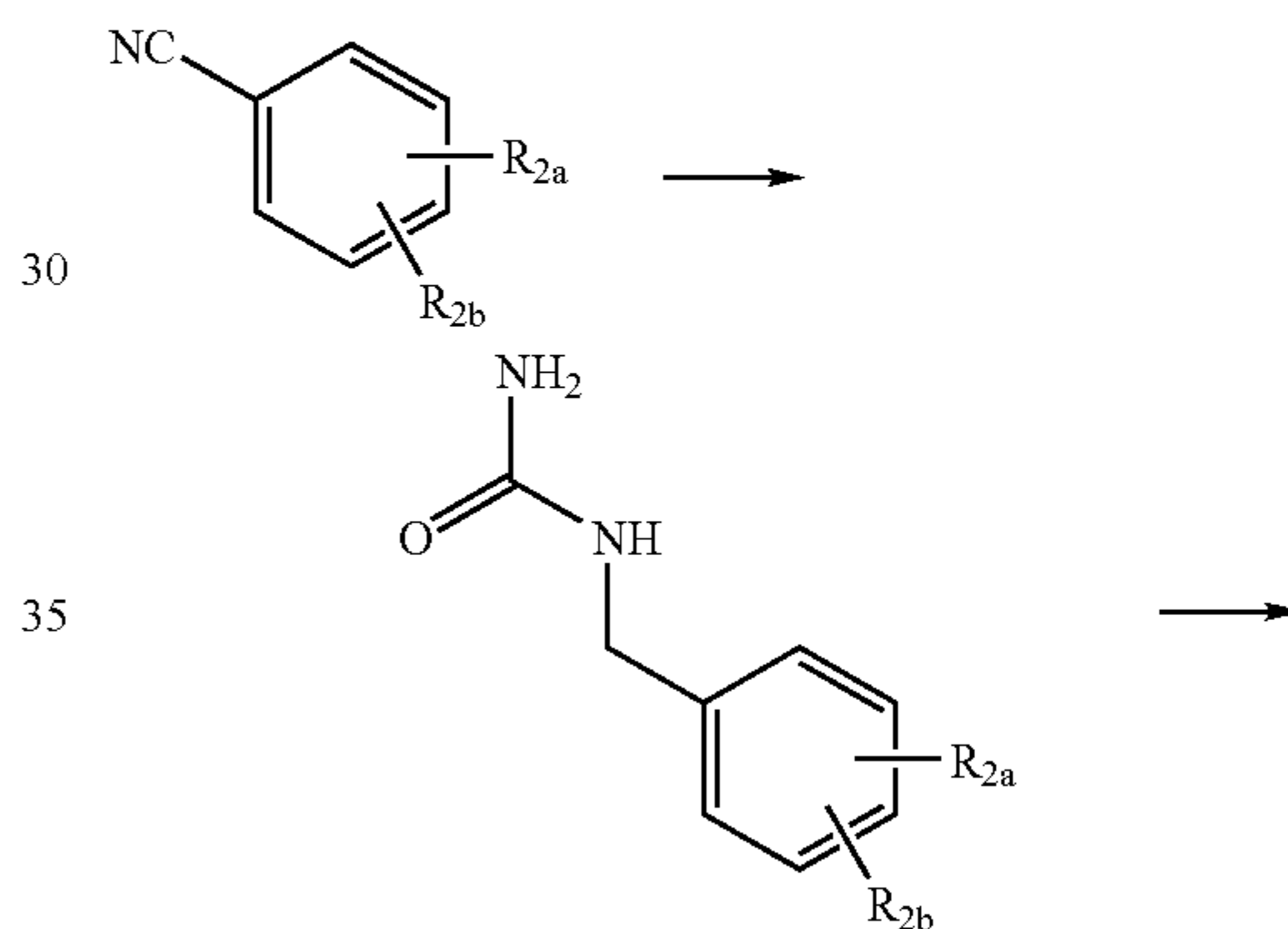
Reaction Scheme 1
