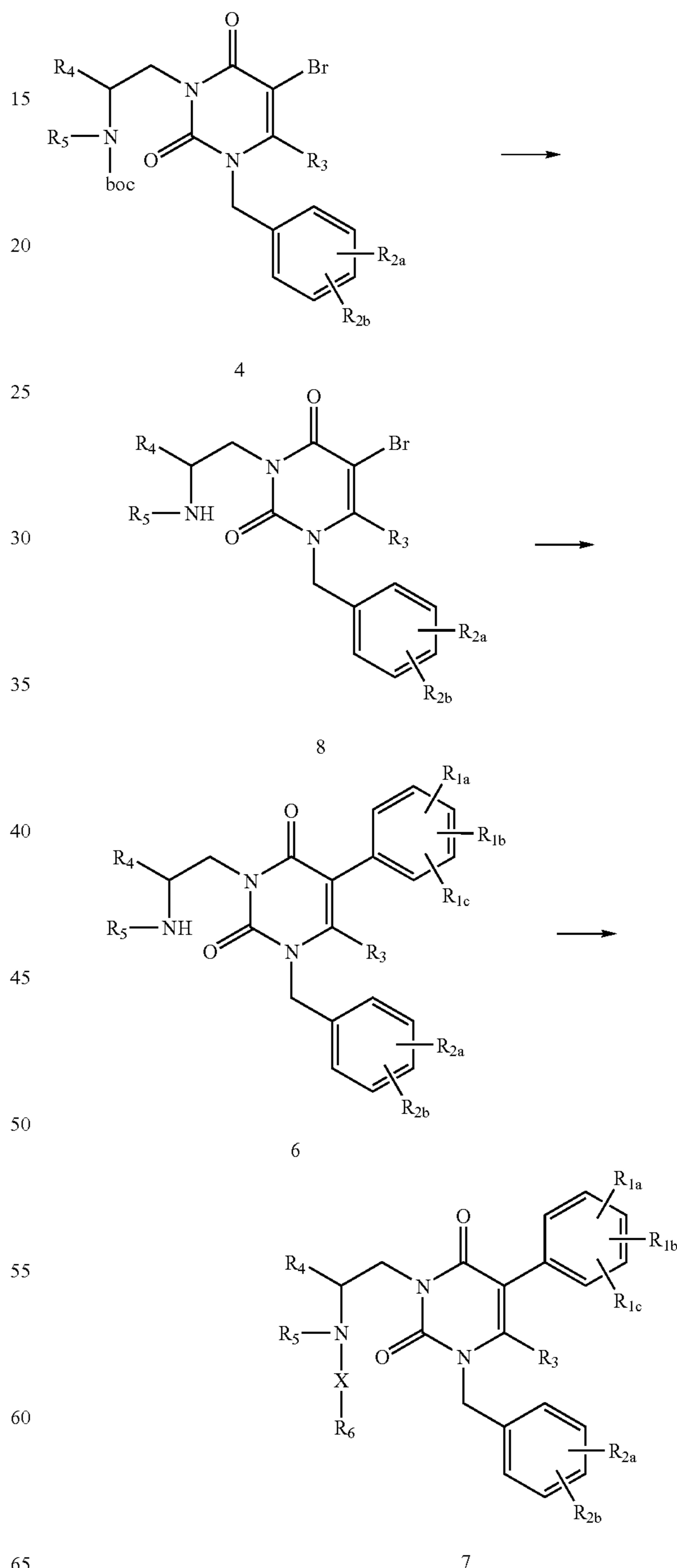
Reaction Scheme 2
