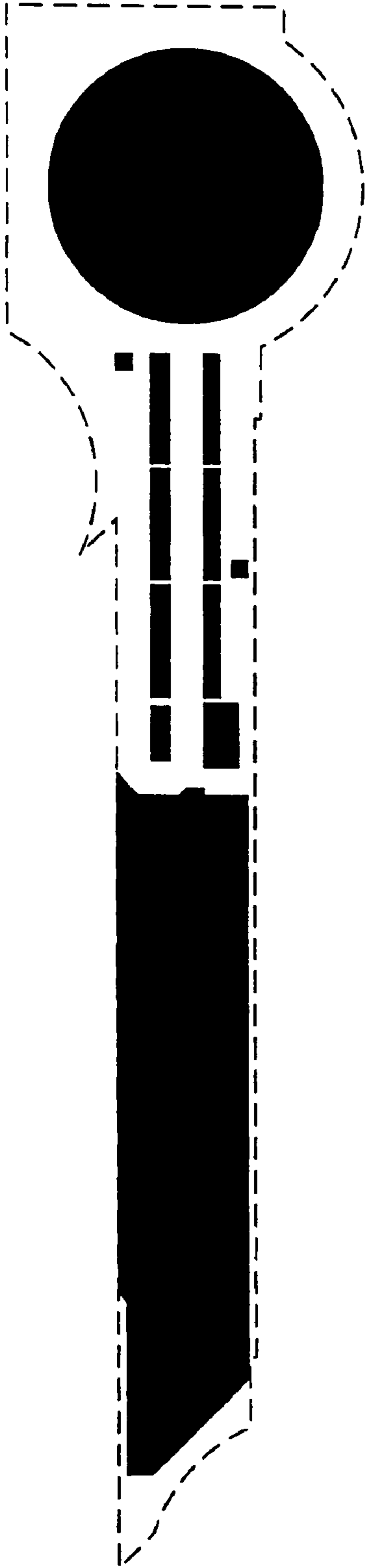
Active mask
