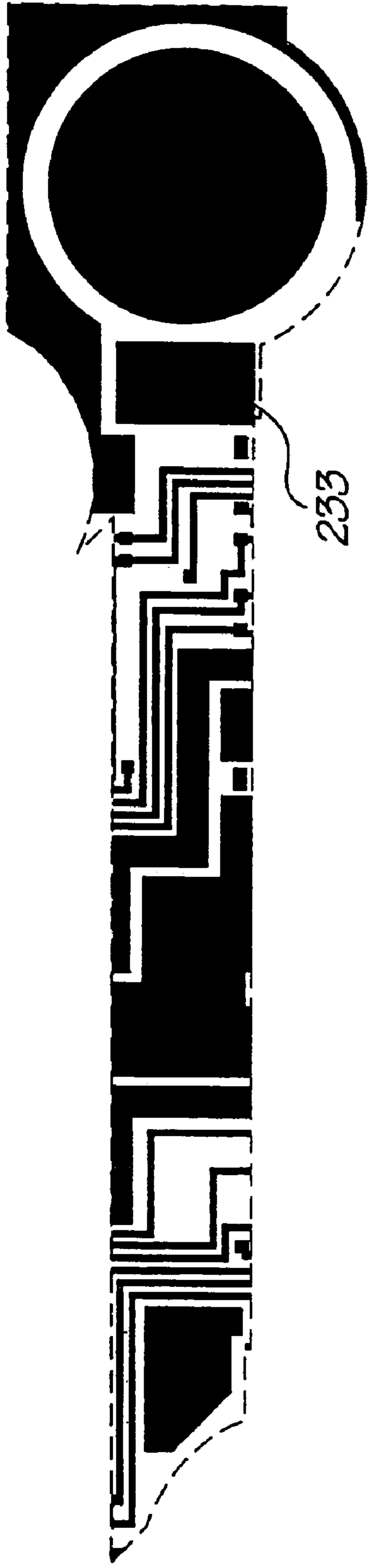
Metal 2 mask
