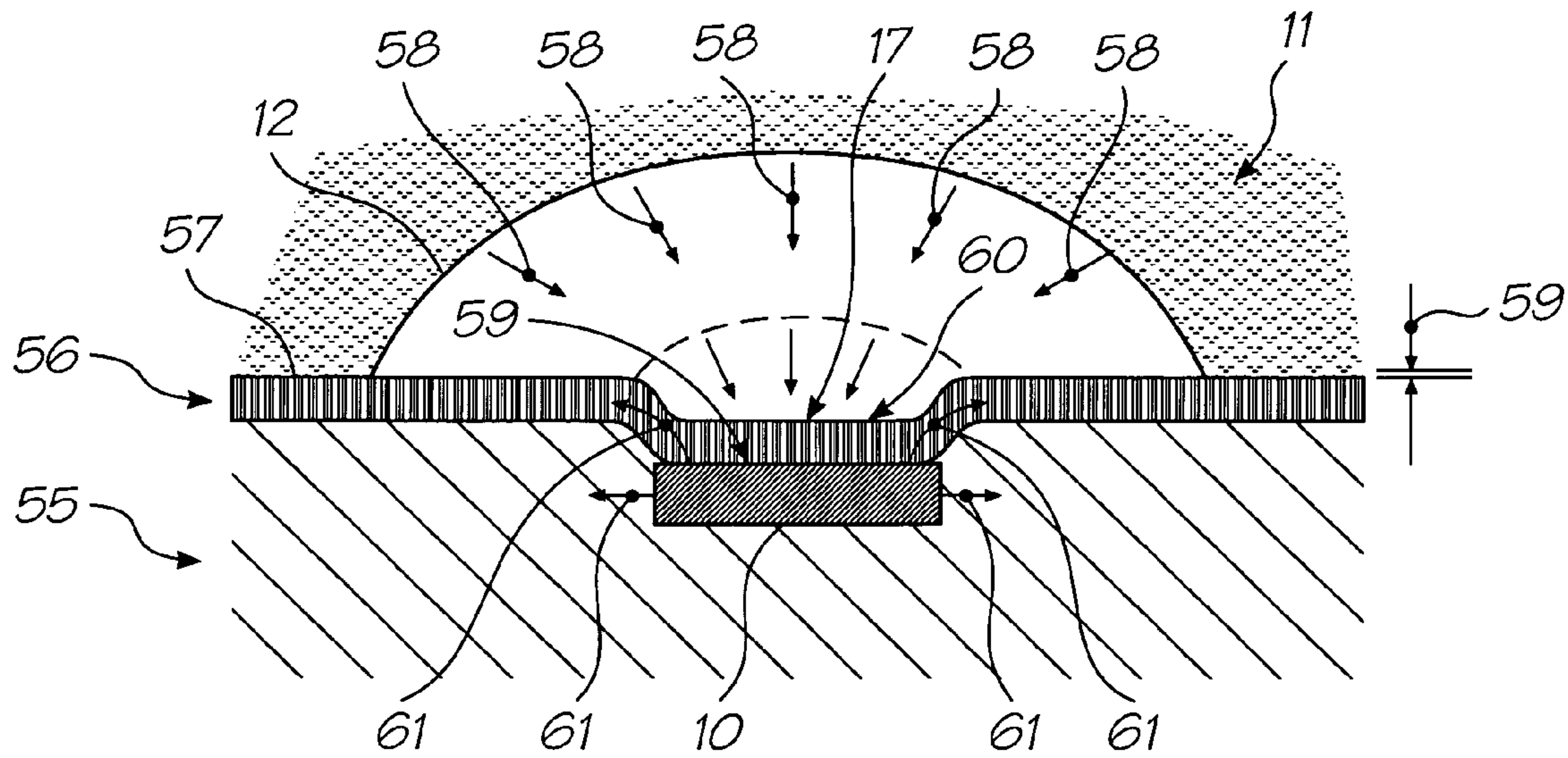
FIG. 57 (PRIOR ART)
