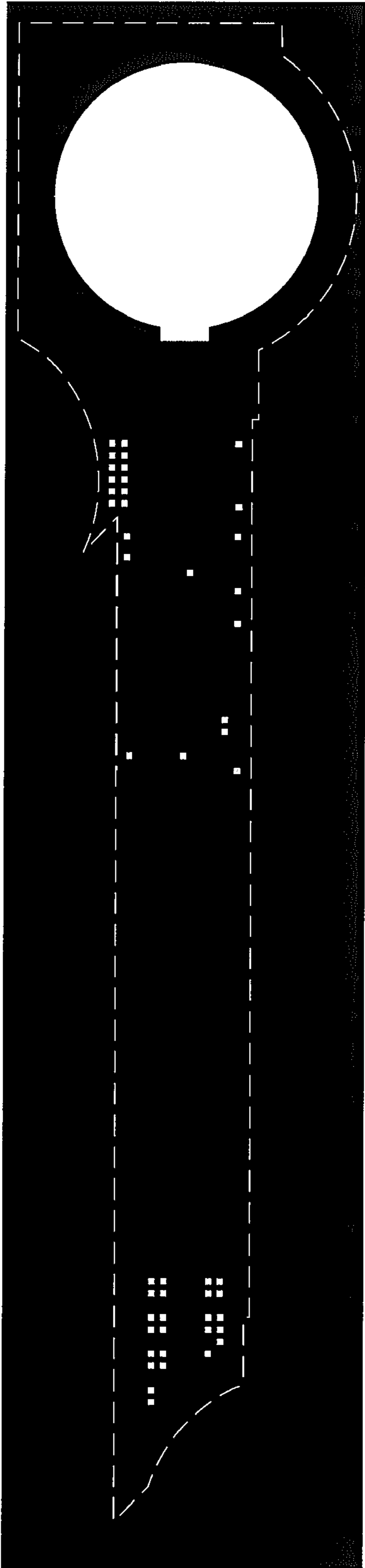
Via 1 mask
