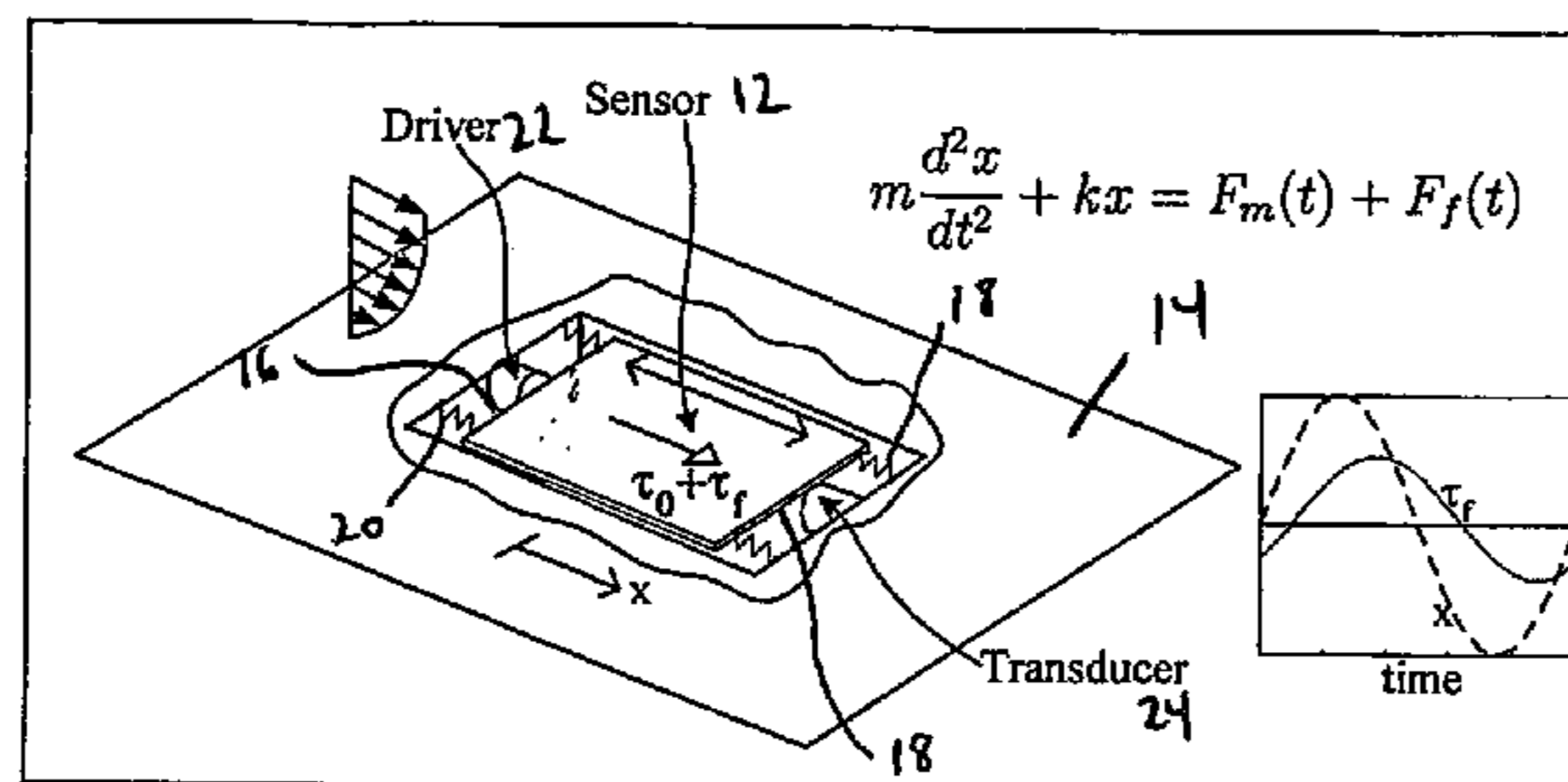
Schematic of dynamic resonant shear stress sensor with the governing equation and a time history of the fluctuating shear force on the sensor (from a simulation). A cutaway view of the sensor is shown to display components below the surface.
