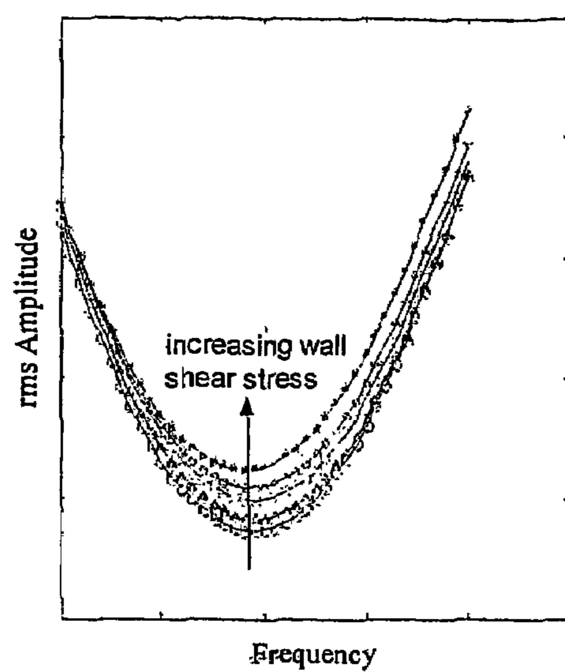
Fig. 4 - Experimental data showing the performance of an closed loop, periodic, resonant wall shear stress sensor. The dependence of the driving mechanism amplitude on frequency is shown.
