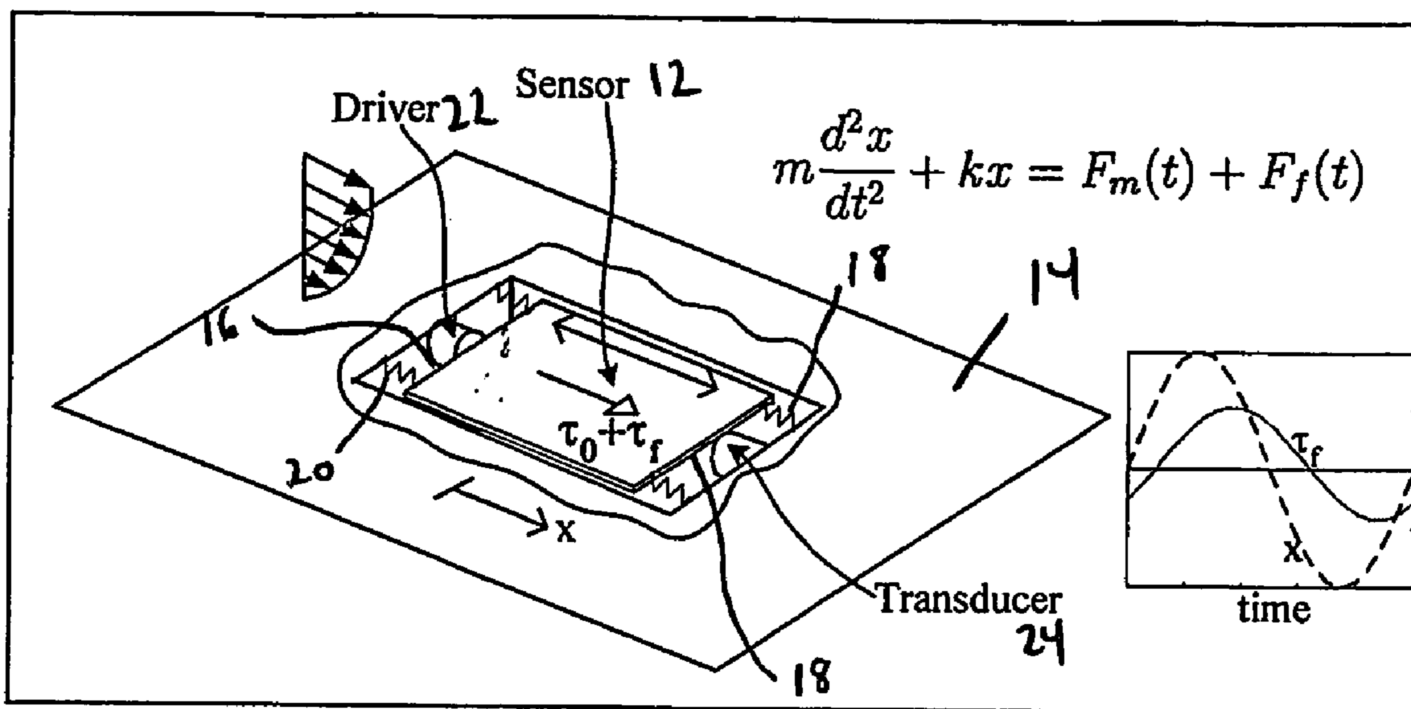
Fig. 1 - Schematic of dynamic resonant shear stress sensor with the governing equation and a time history of the fluctuating shear force on the sensor (from a simulation). A cutaway view of the sensor is shown to display components below the surface.
