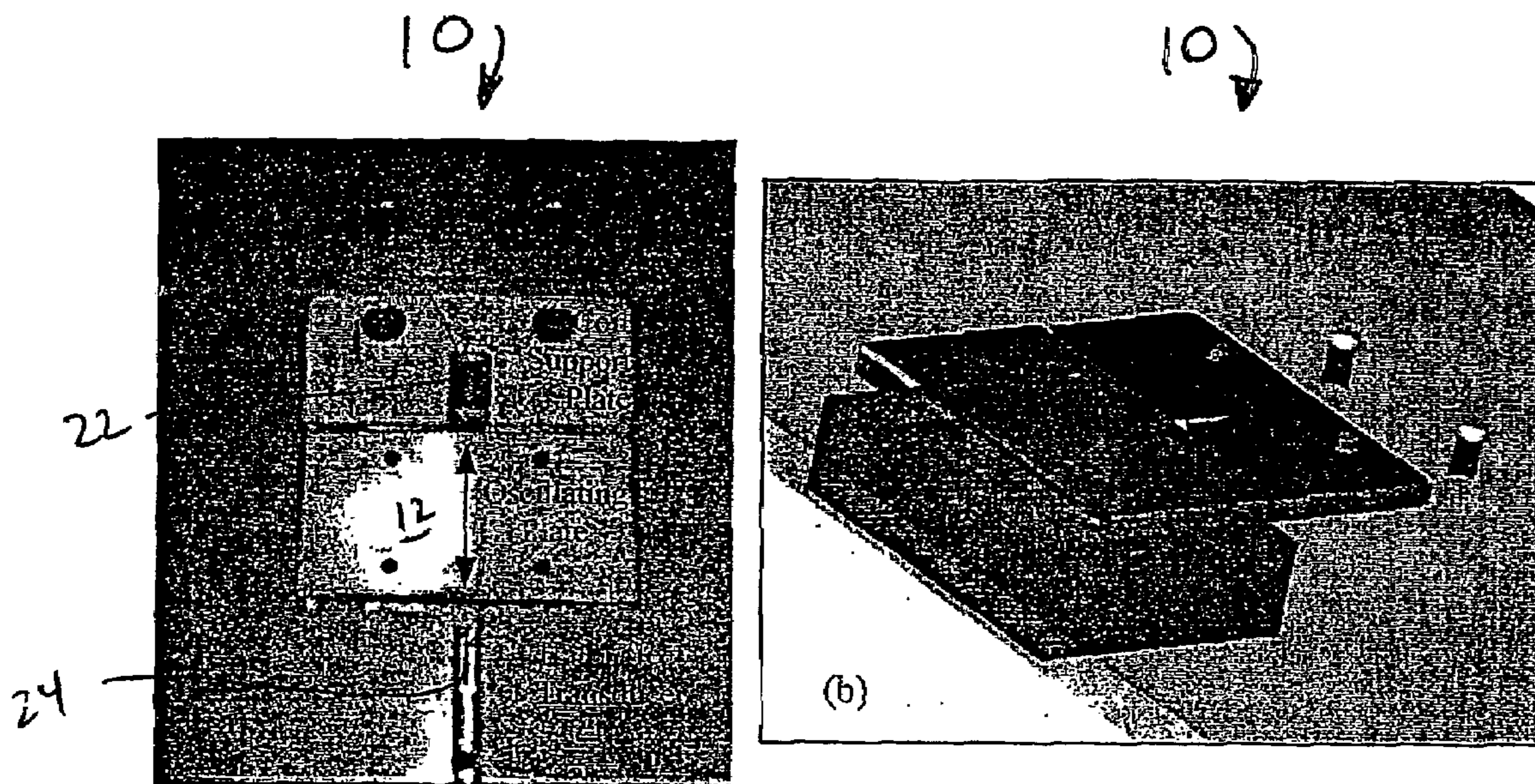
Fig. 2 - Large-scale prototype surface shear stress sensor: (a) image of the sensor, and (b) three-dimensional schematic.
