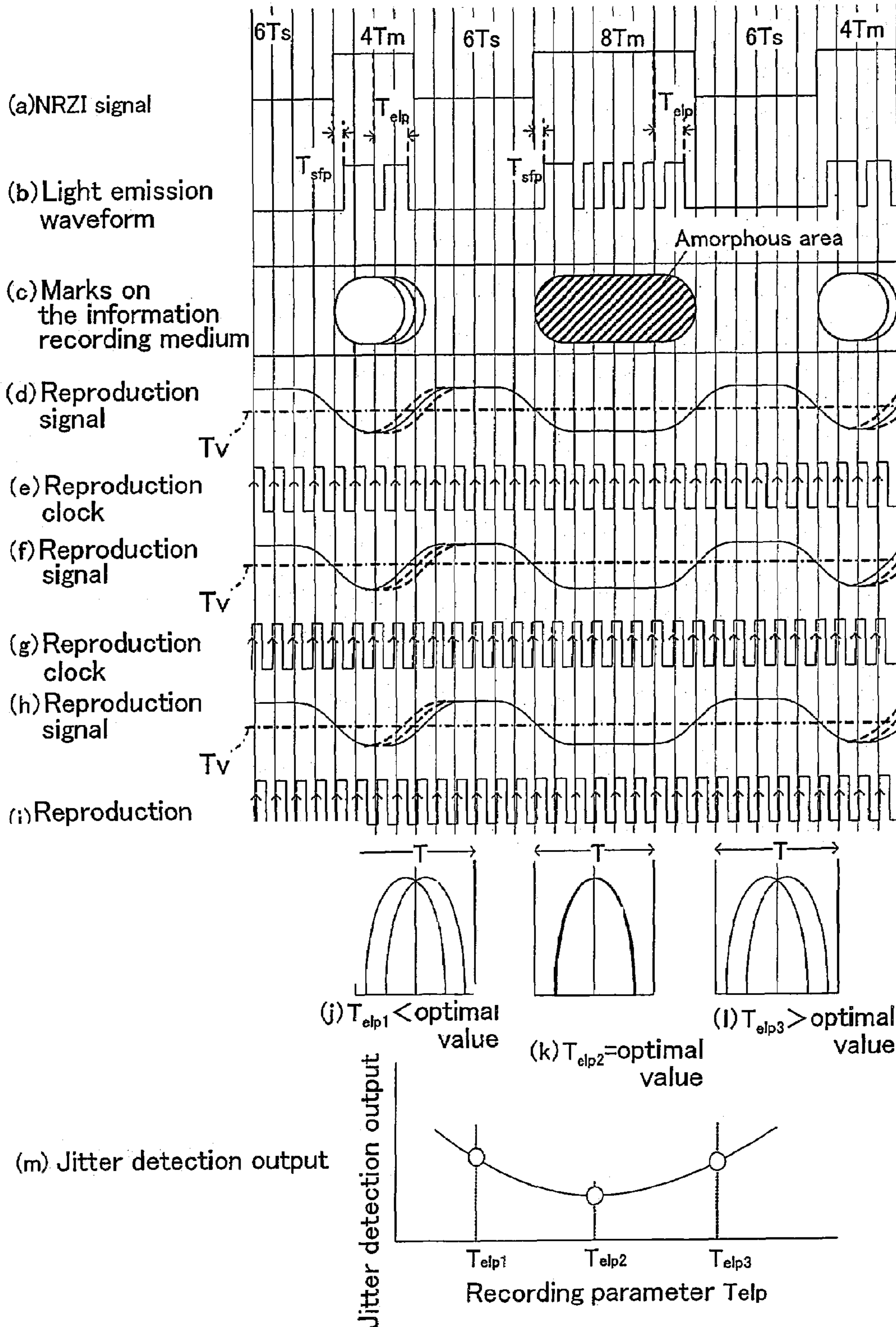
FIG. 15 CONVENTIONAL ART
