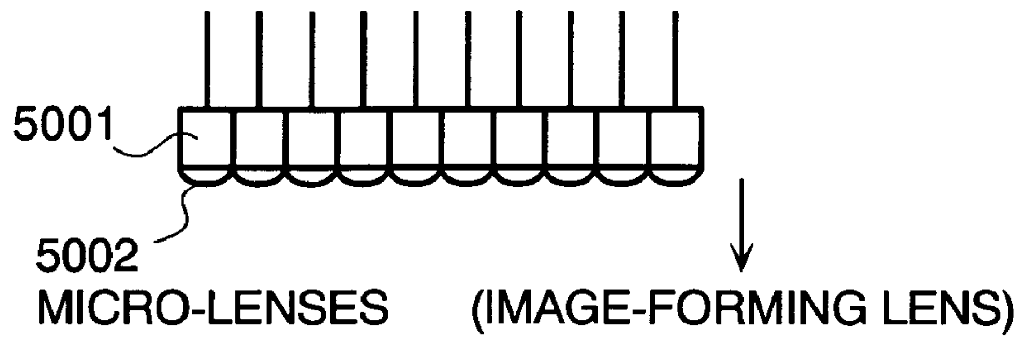
SIDE VIEW
