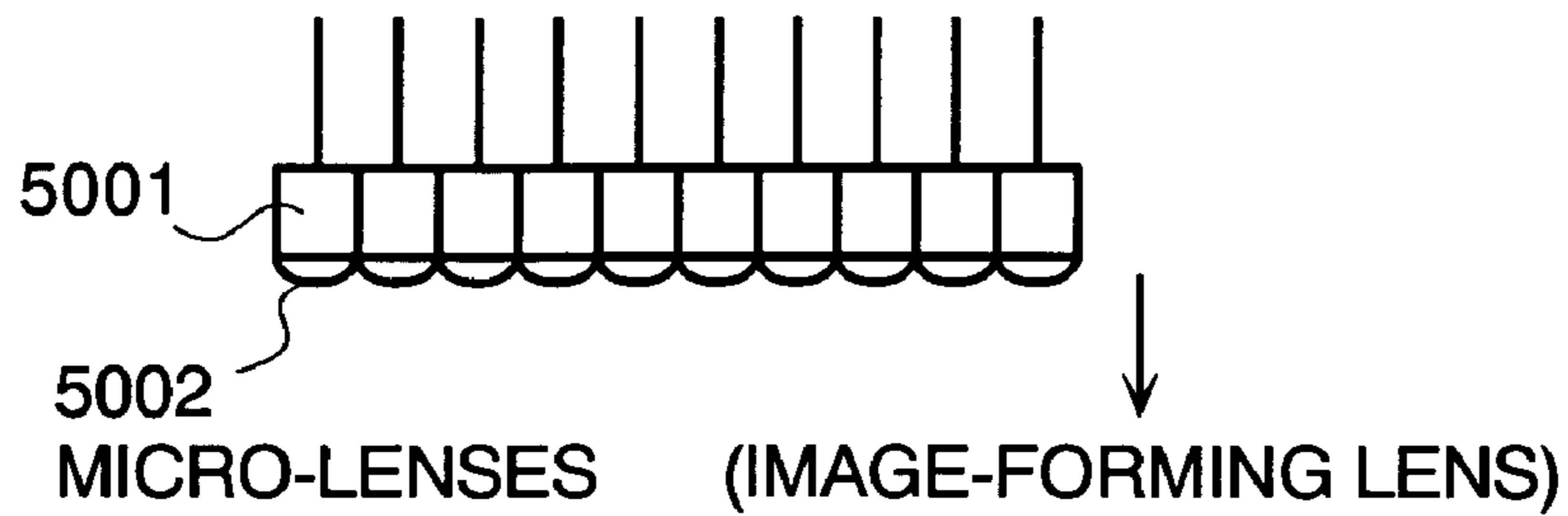
SIDE VIEW
