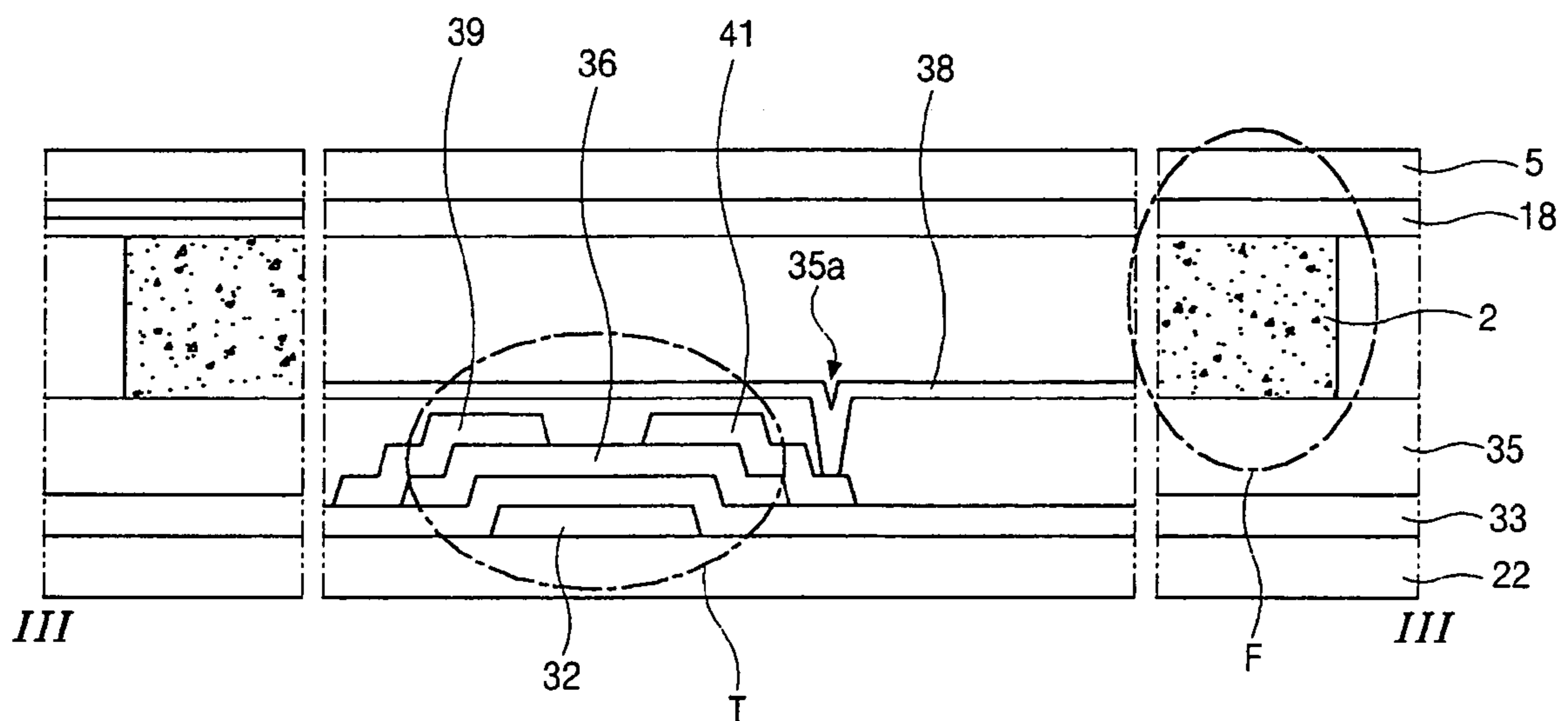
FIG. 3 (BACKGROUND ART)
