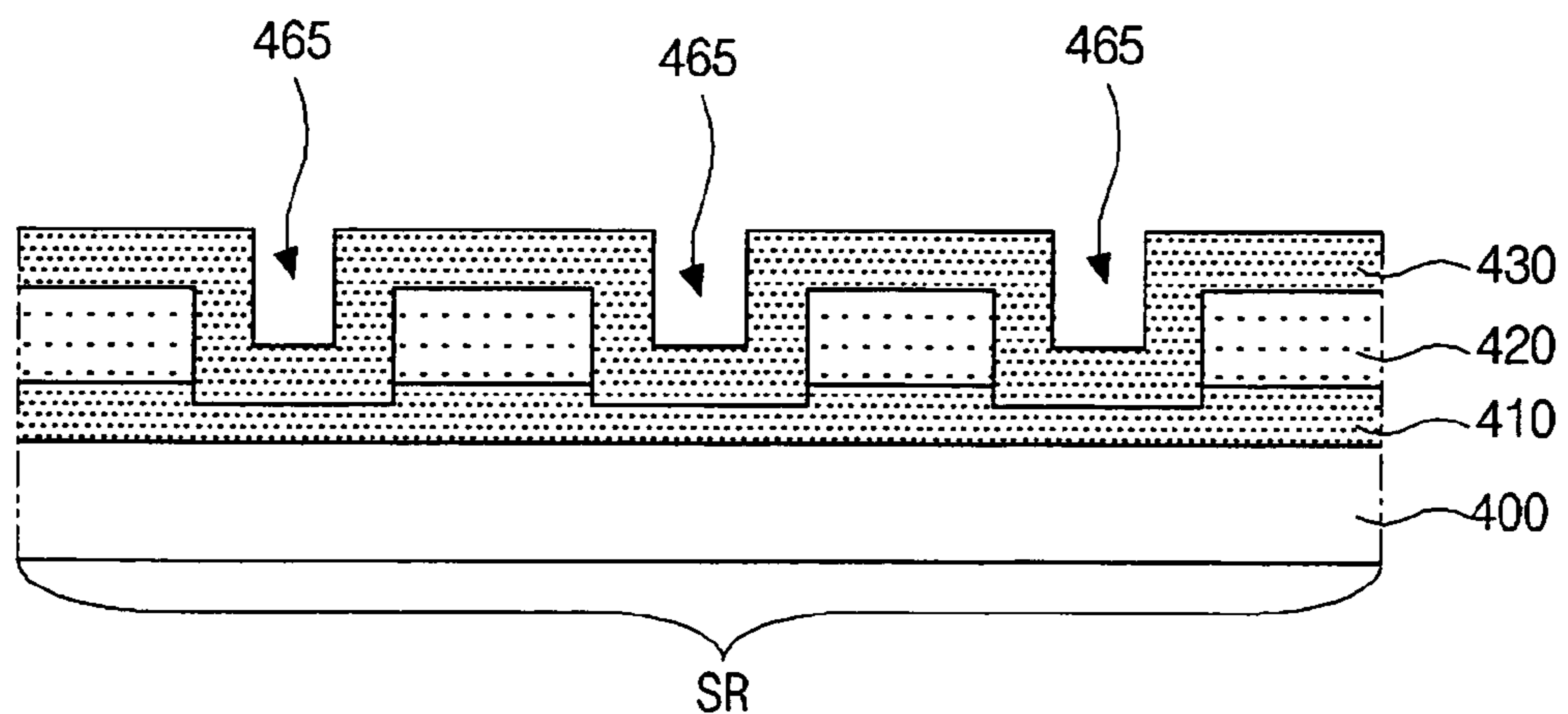
FIG. 12D
