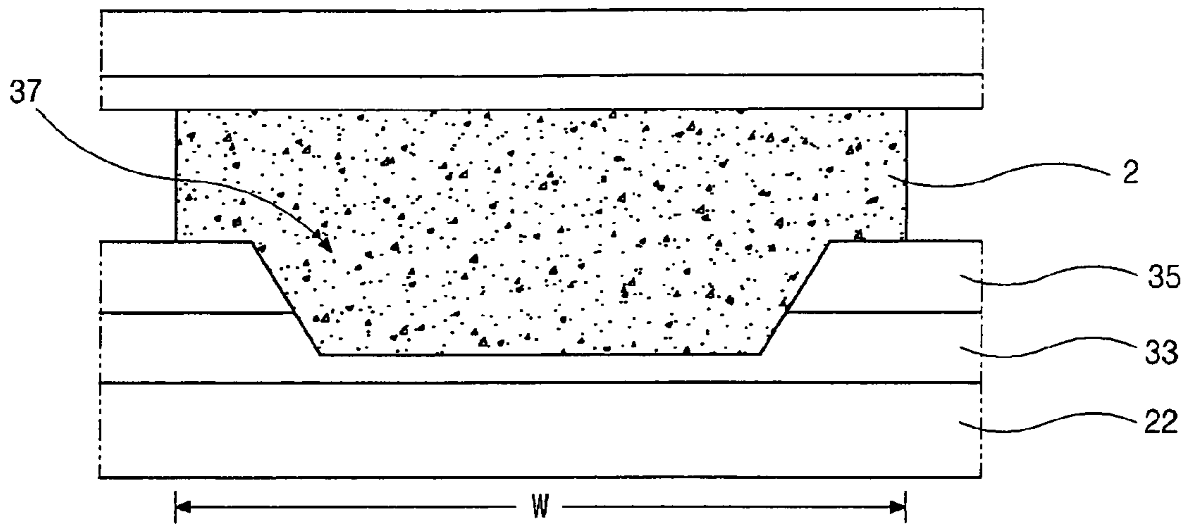
FIG. 4 (BACKGROUND ART)
