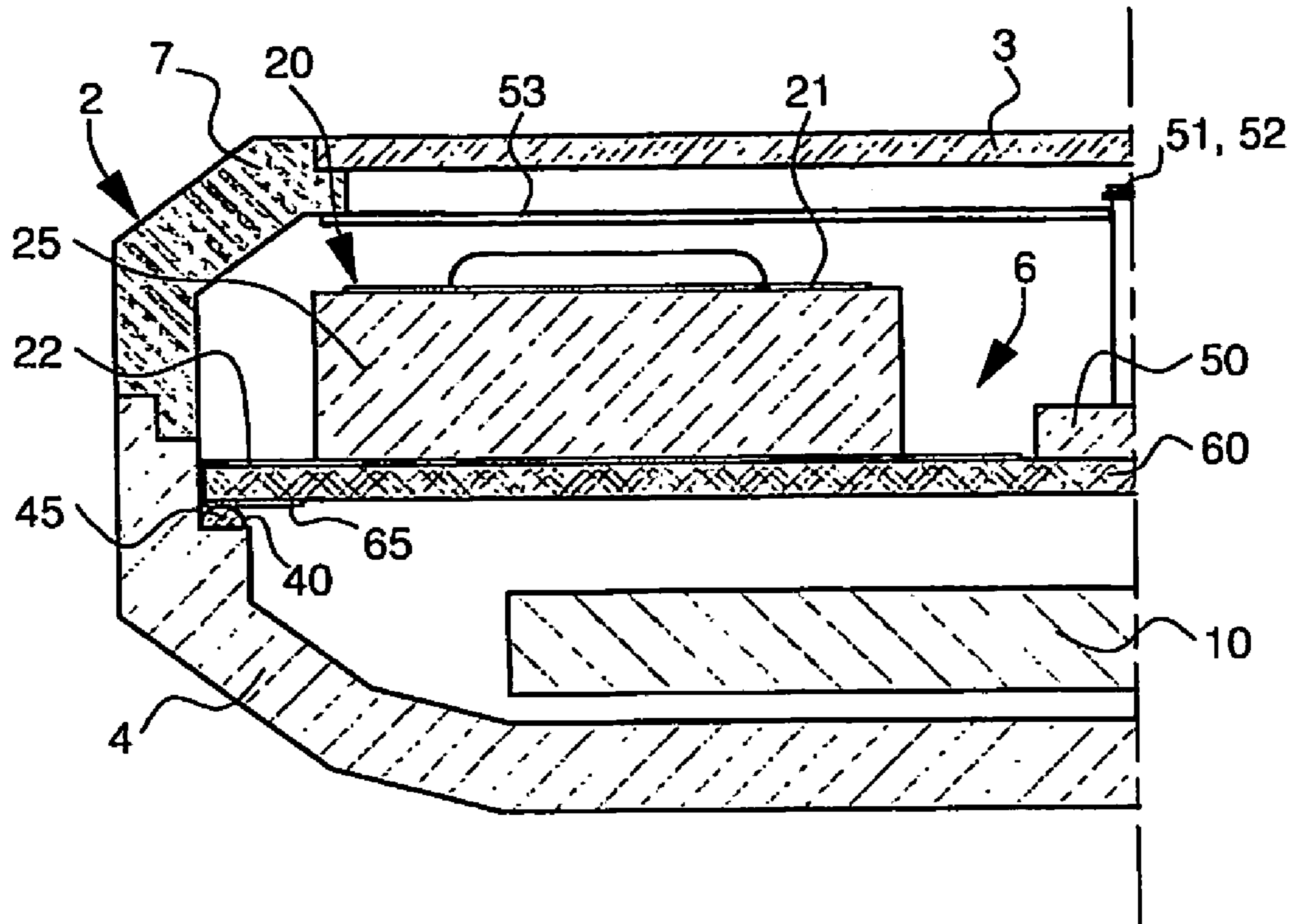
Fig.2 SECTION A-A
