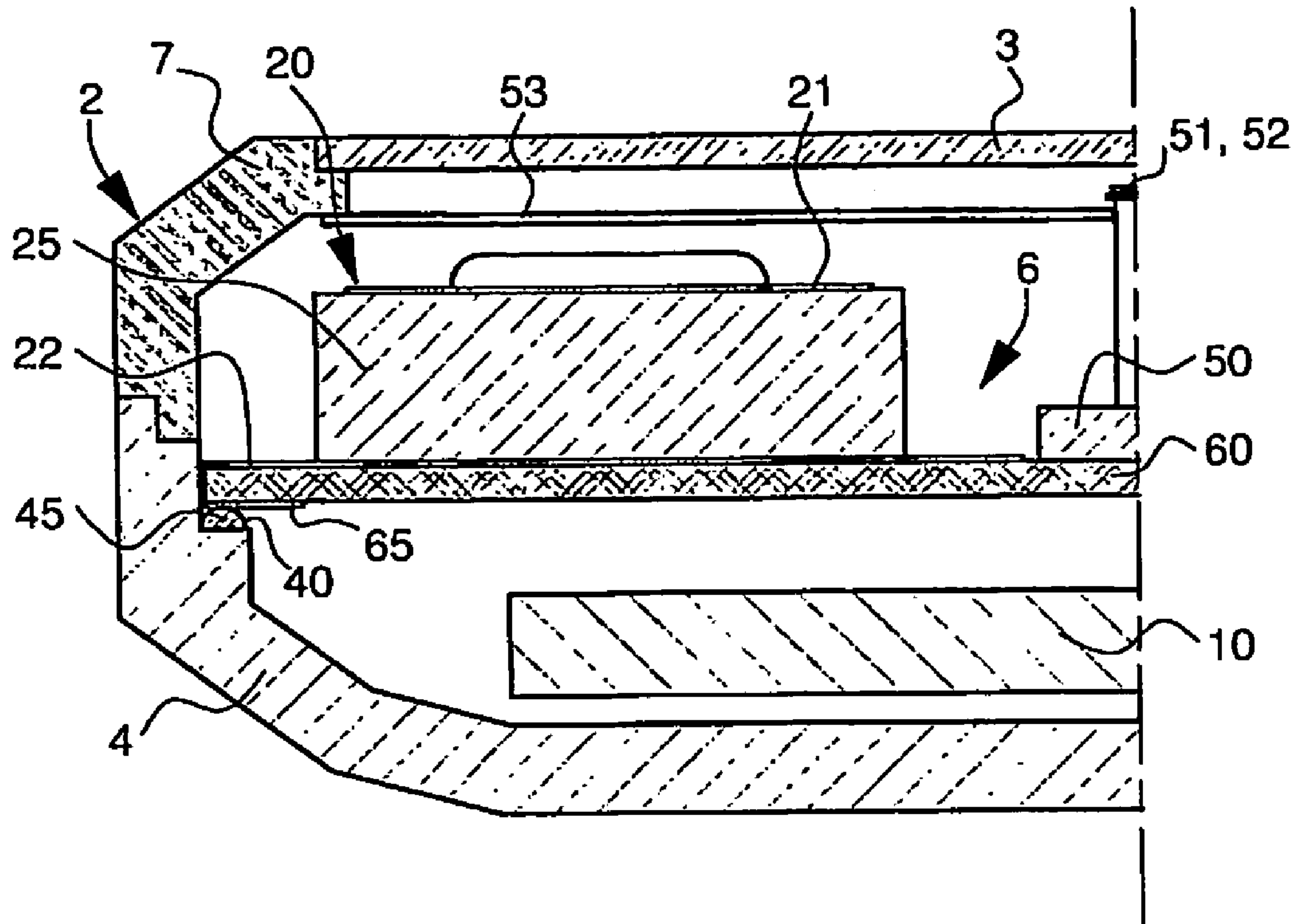
Fig.2 SECTION A-A
