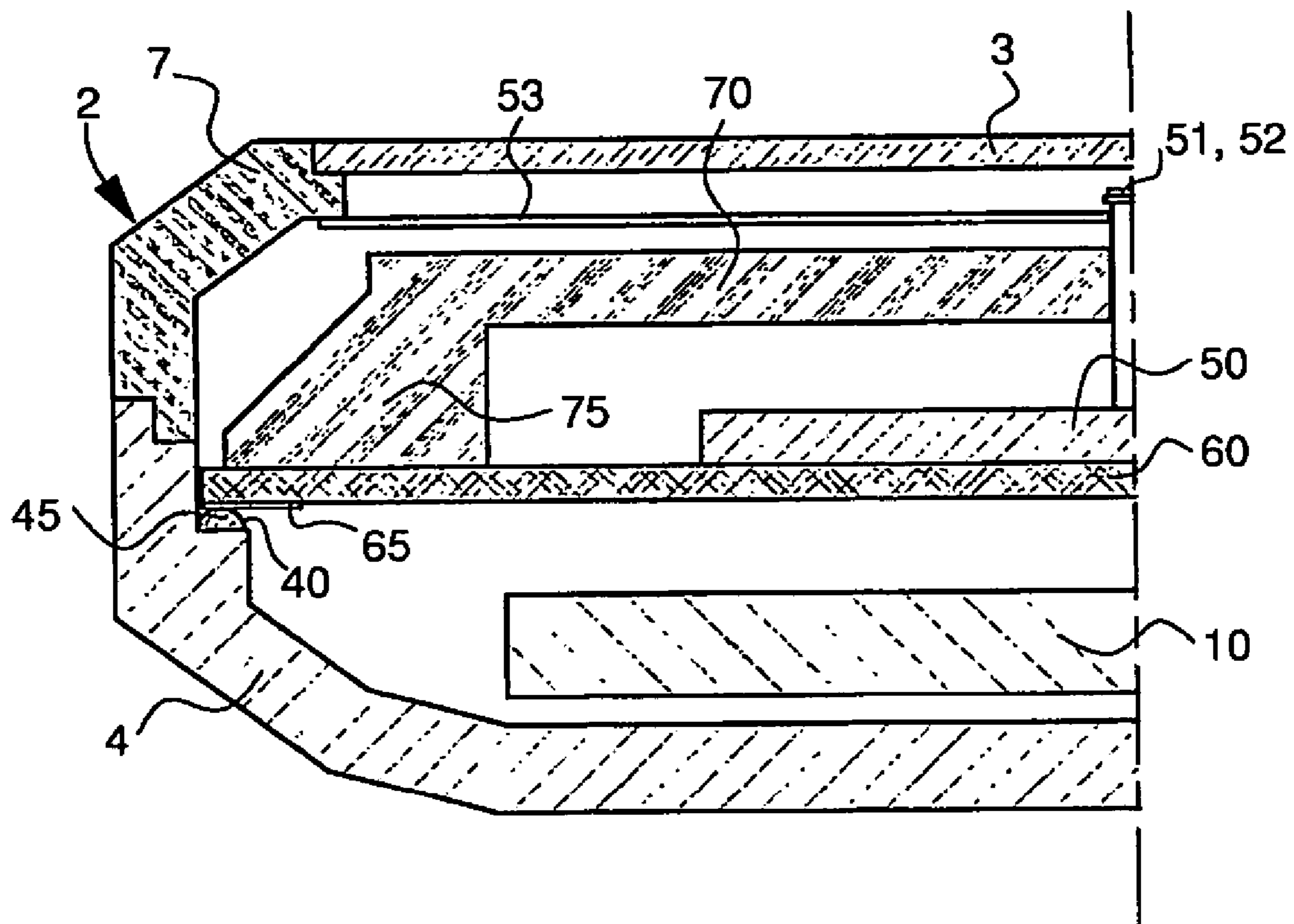
Fig.4 SECTION B-B
