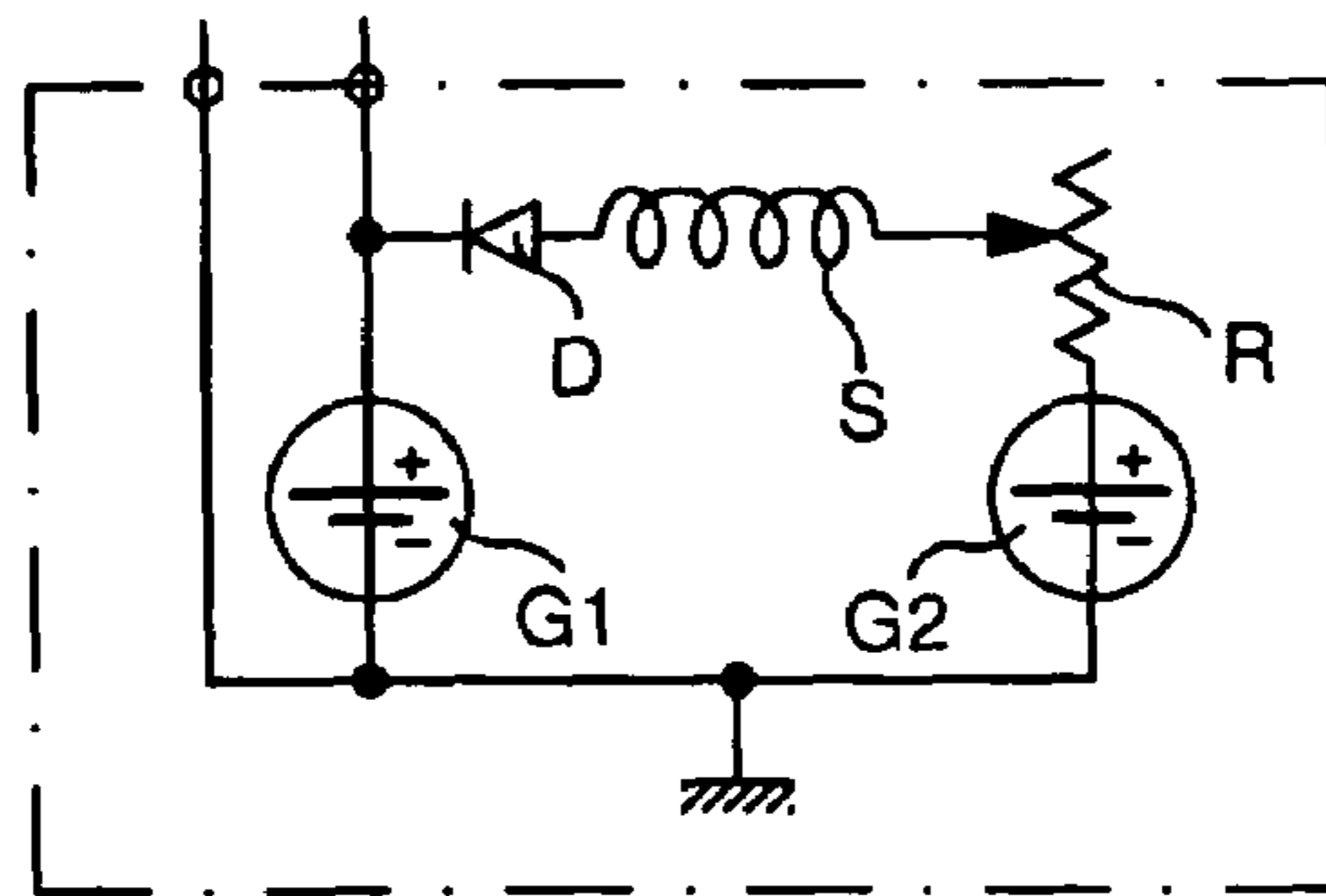
Fig. 1 PRIOR ART
