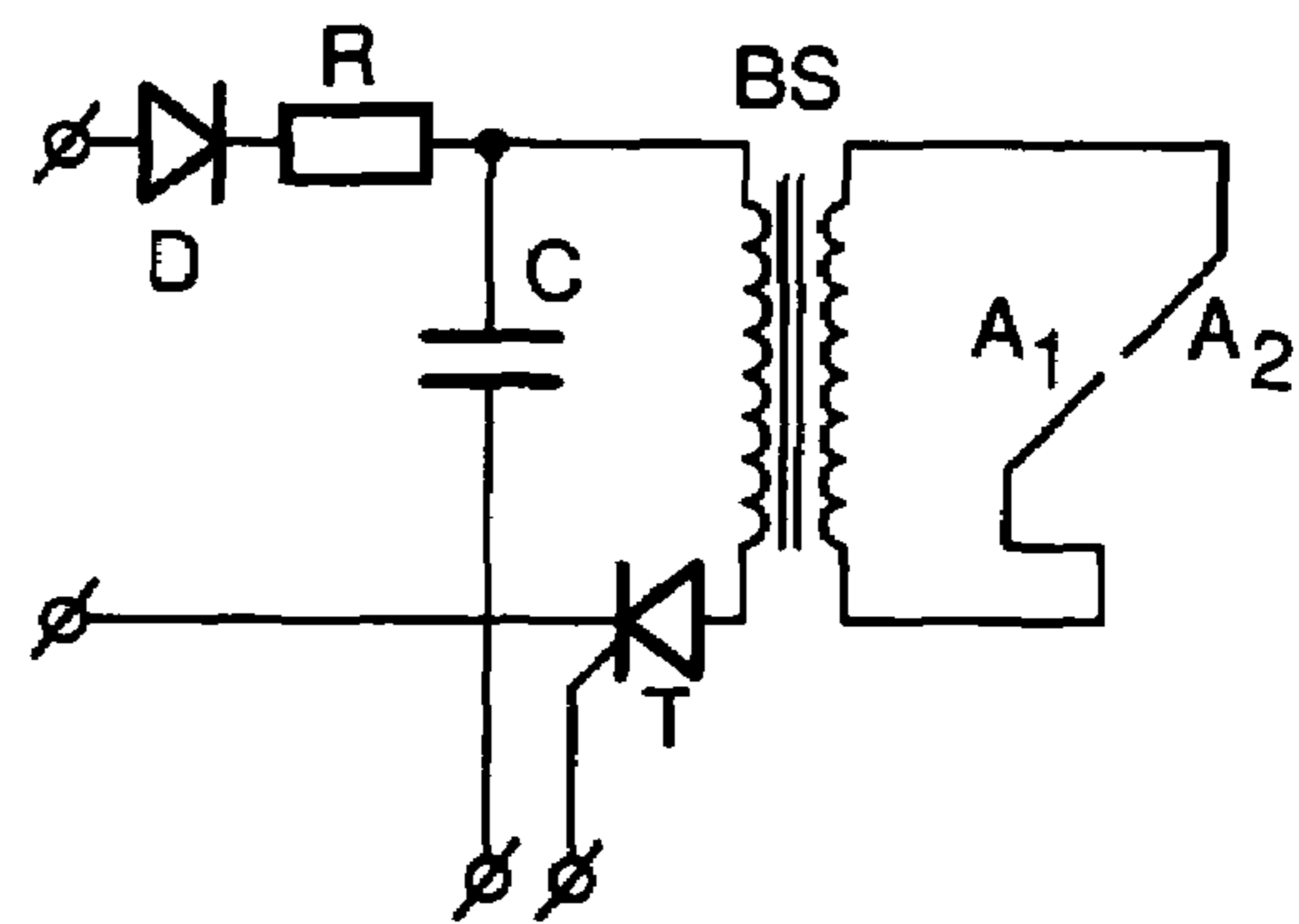
Fig. 6 PRIOR ART
