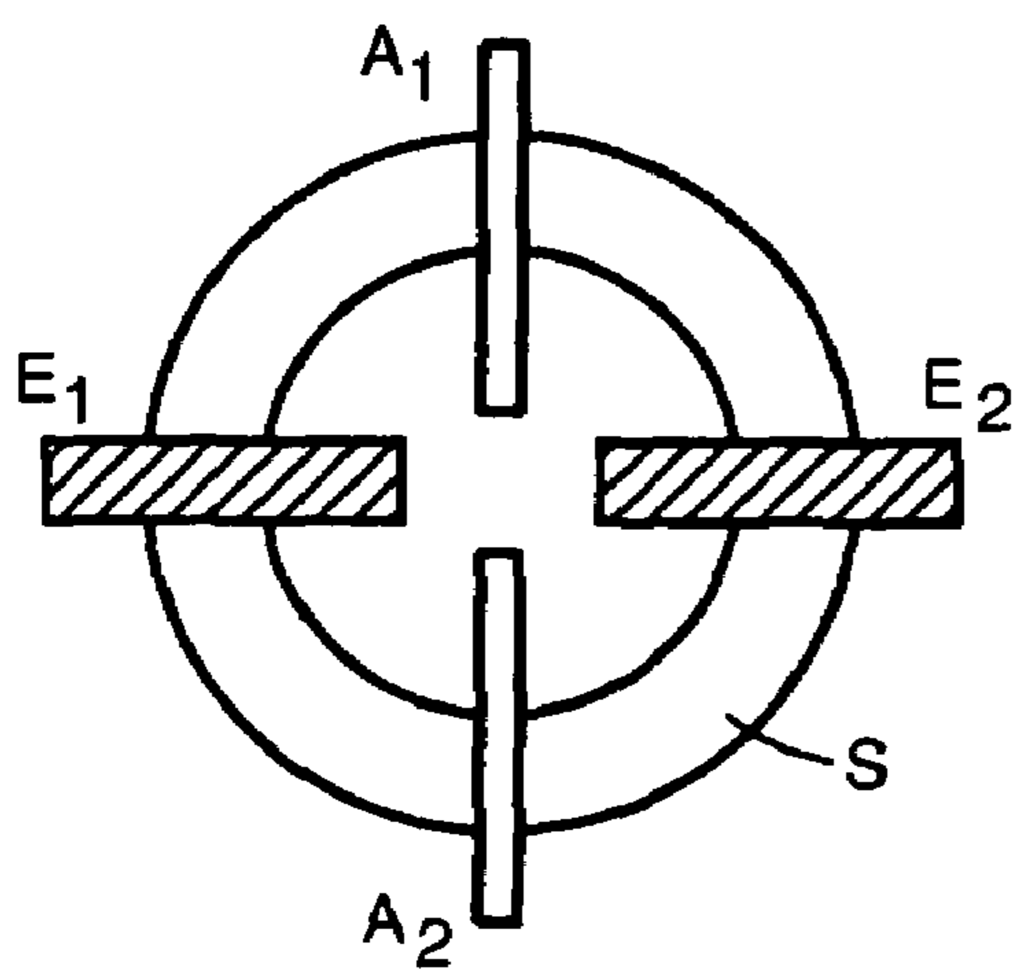
Fig. 5 PRIOR ART
