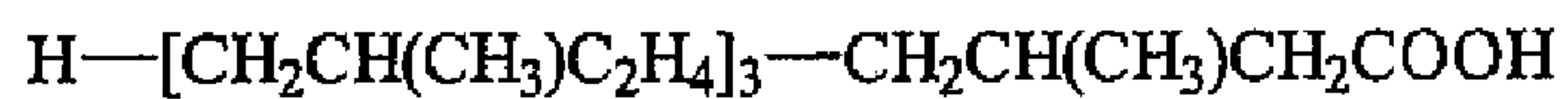
Phytanic acid
