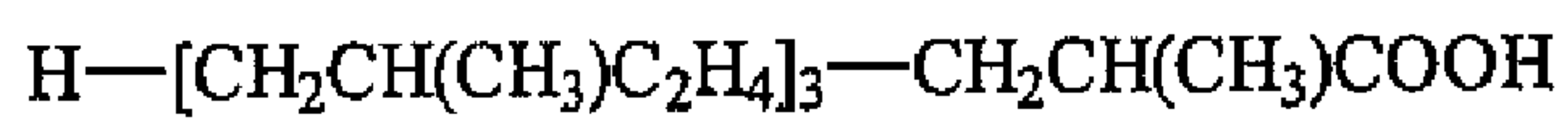
Pristanic acid
