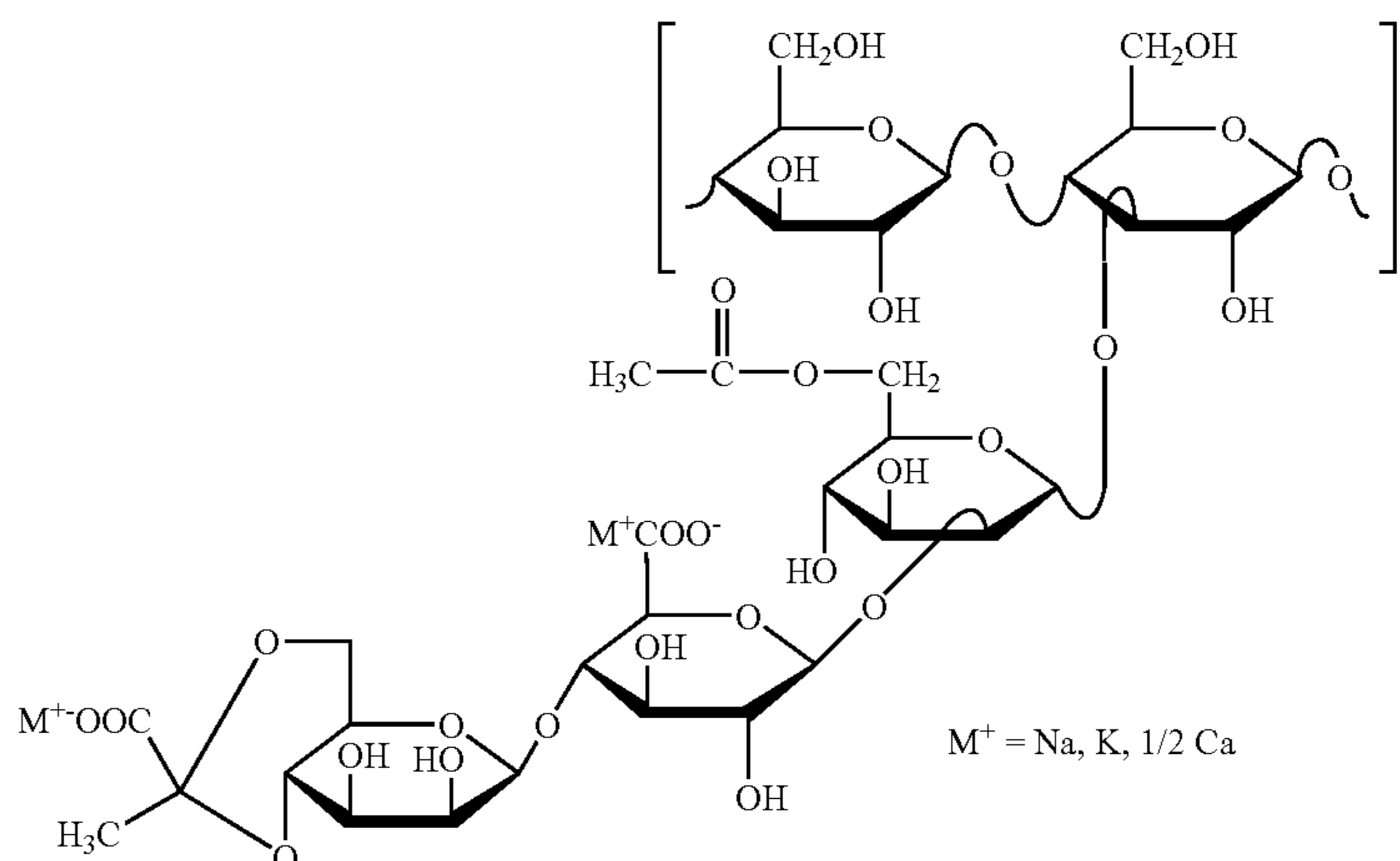
Basic unit of xanthan
