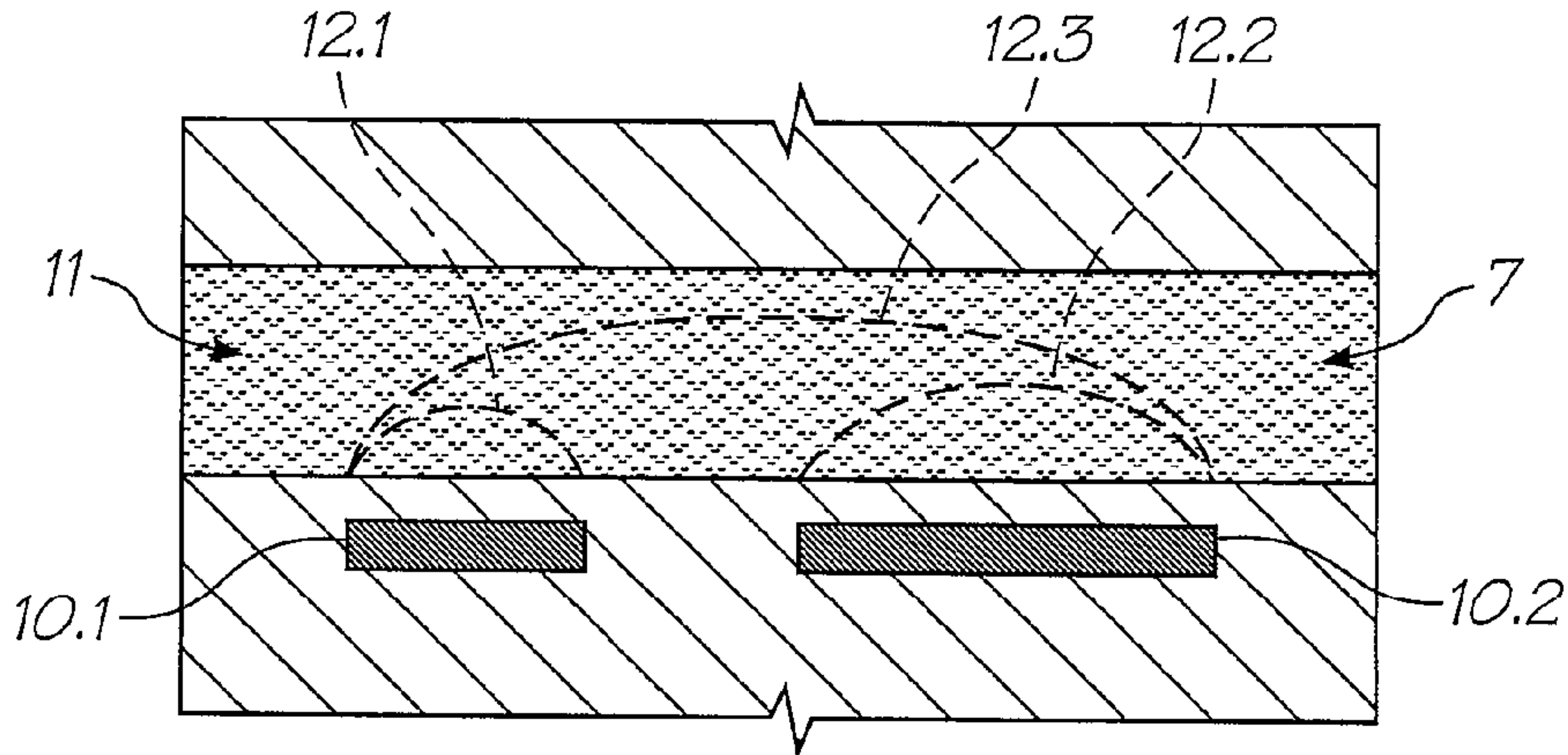
FIG. 52 (PRIOR ART)
