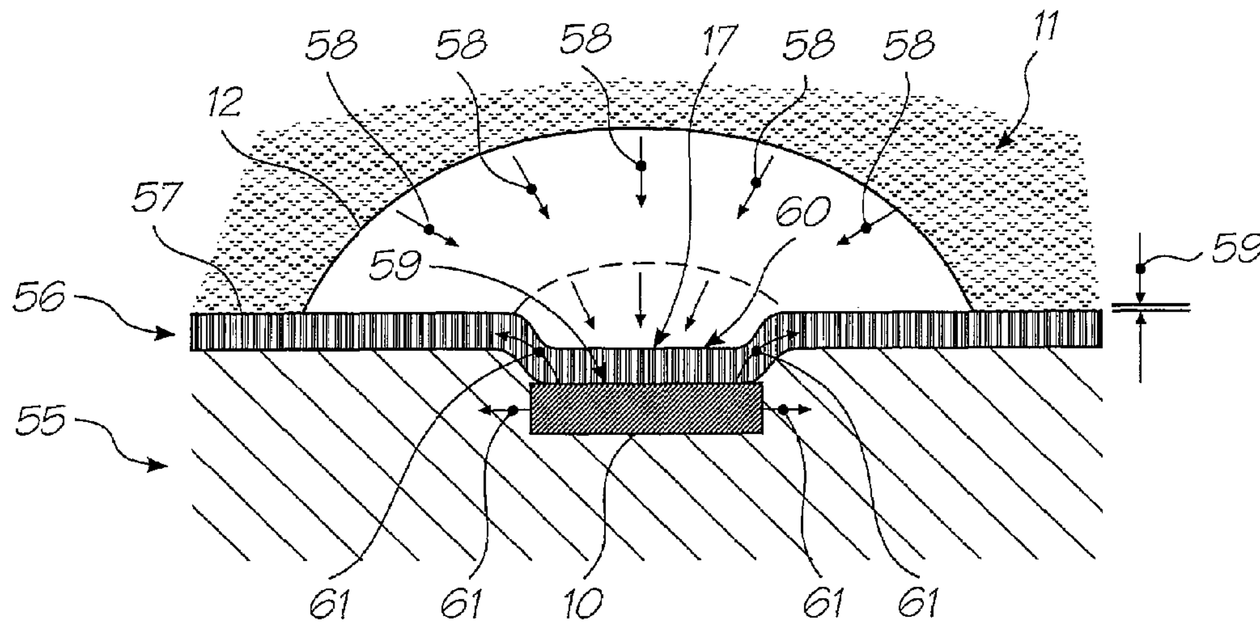
FIG. 47 (PRIOR ART)
