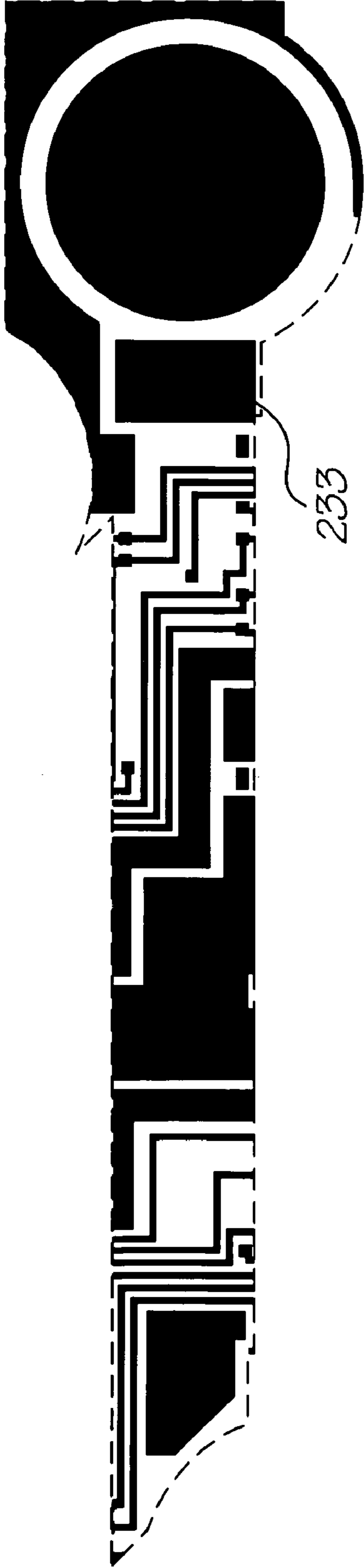
Metal 2 mask
