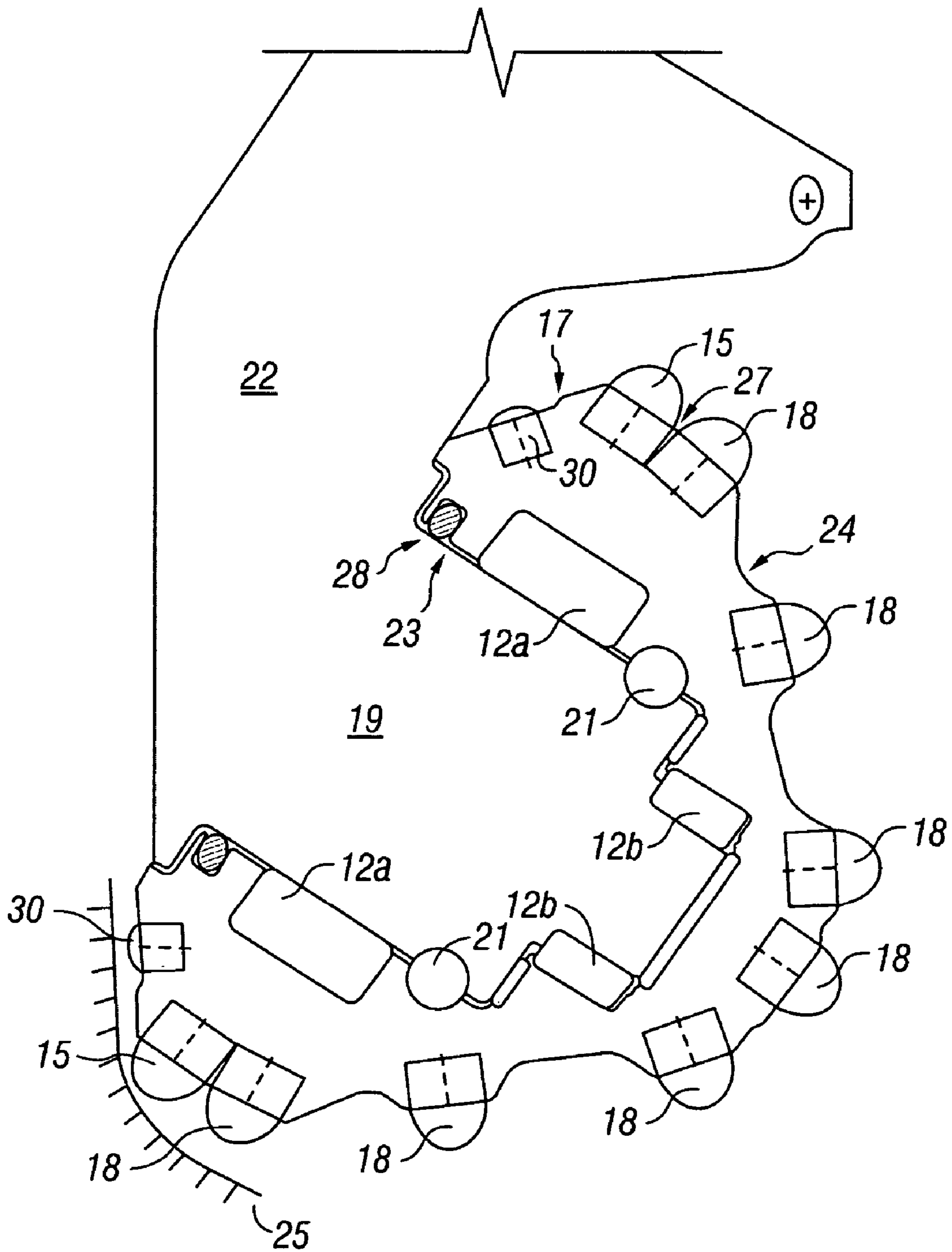
FIG. 2 (Prior Art)
