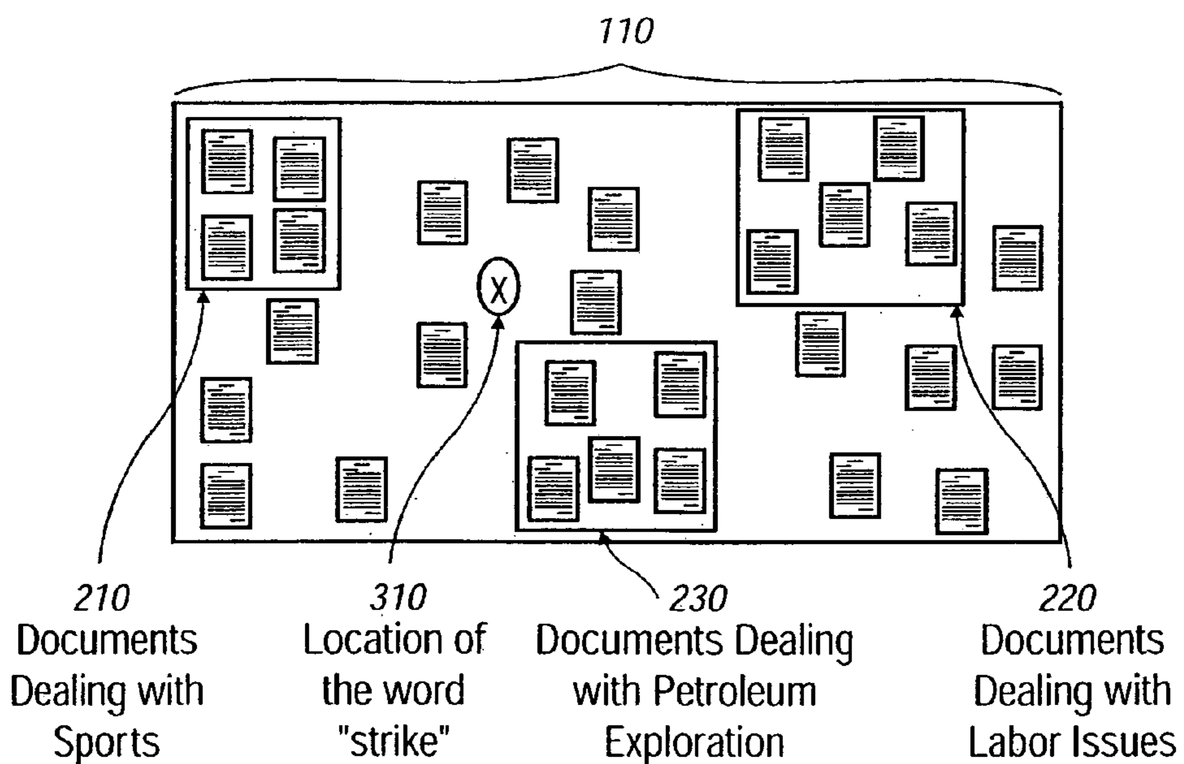
Location of the Word Strike in the LSI Space FIG. 6
