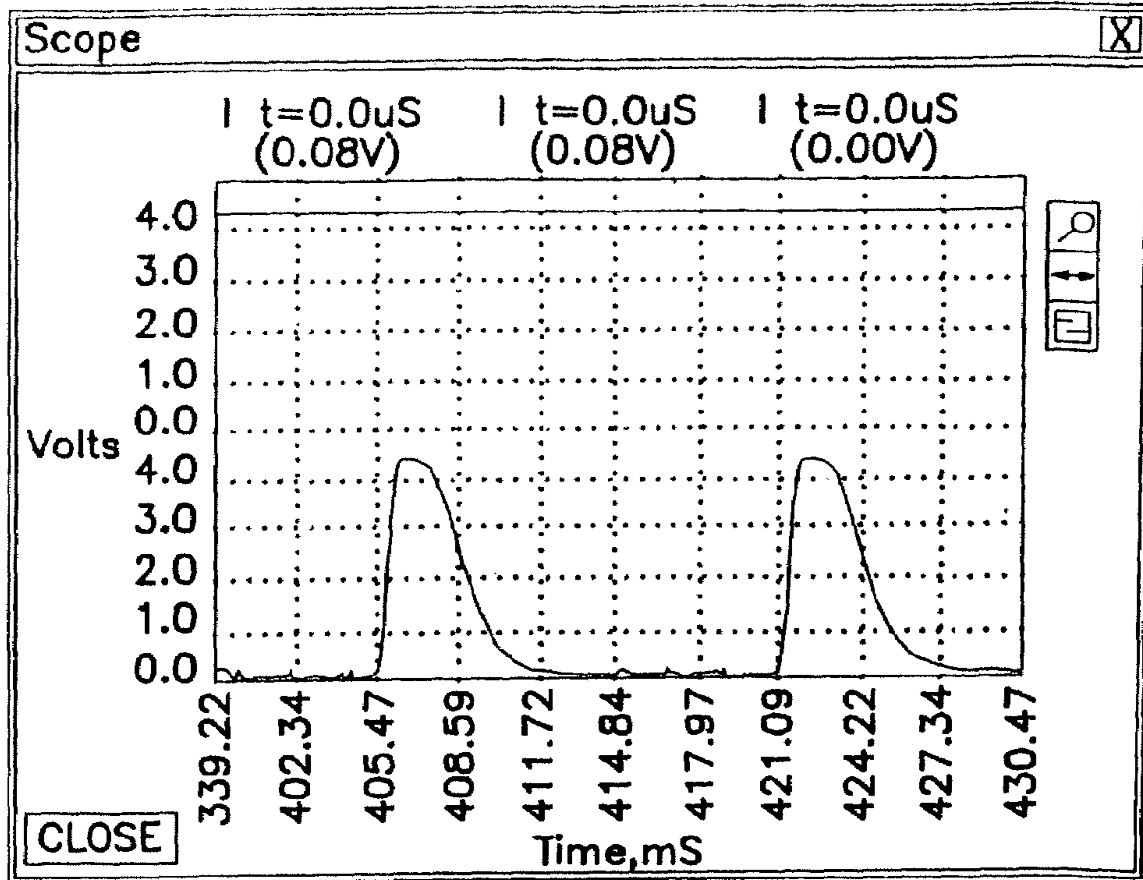
CRT photoresponse
