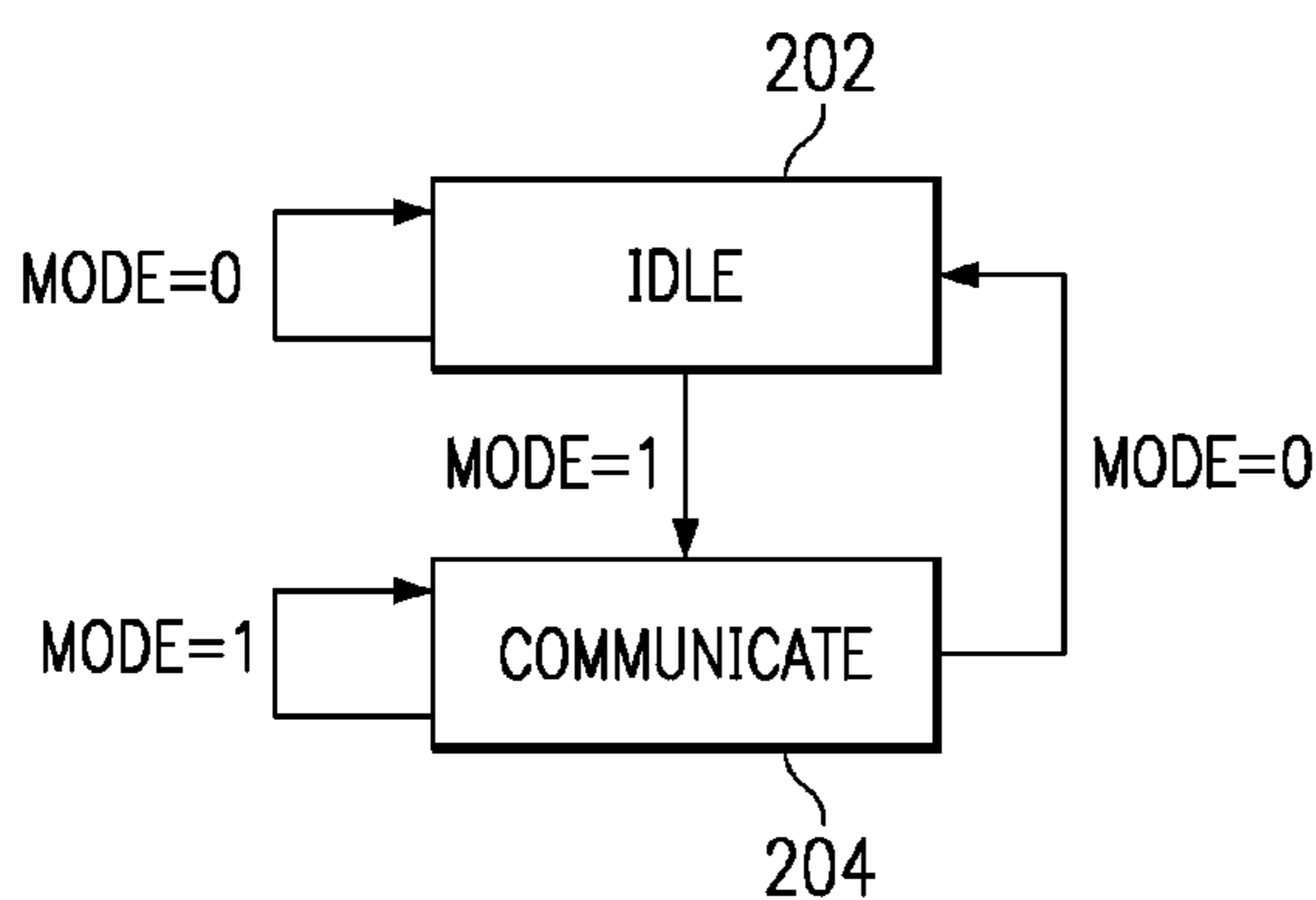
FIG. 2 (PRIOR ART)
